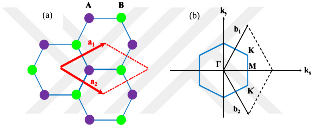
Figure 3.1 schematic of lattice structure of graphene (a) Honeycomb crystal structure of graphene with a unit cell consisting of two carbon atoms. (b) The first Brillouin zone of graphene with hexagonal shape where all corners of the hexagon are Dirac points. The unit cell of graphene includes two inequivalent atoms with primitive lattice vectors \mathbf{a}_1 and \mathbf{a}_2 as shown in the Figure 3.1(a).
