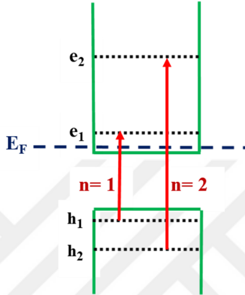
Figure 2.4 The first and second allowed interband optical transitions in accordance with selection rules in a quantum well.
