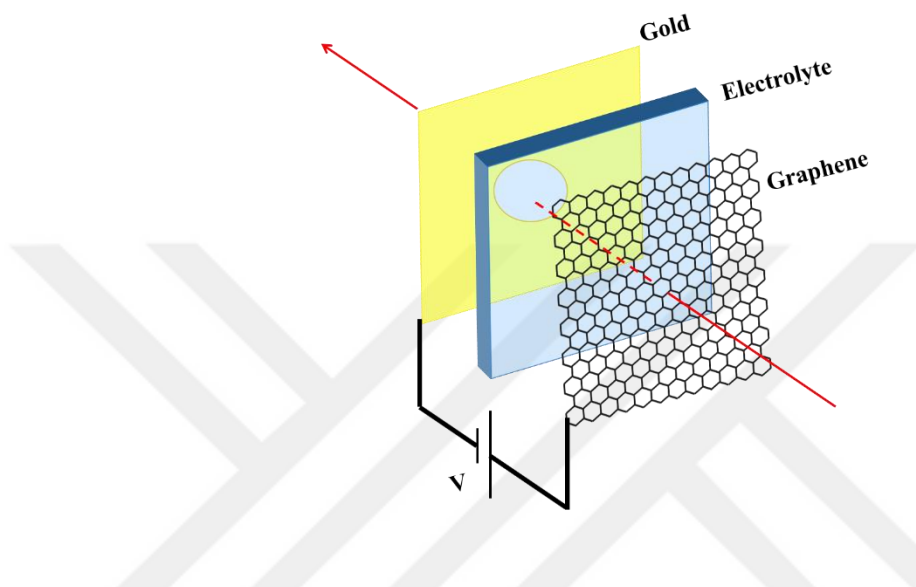
Figure 3.14 schematic of device structure. The device is composed of gold electrode, graphene on a substrate and ionic liquid in between as a gating medium. By applying voltage, ionic liquid gets polarized generating ELD and induce electric field.
