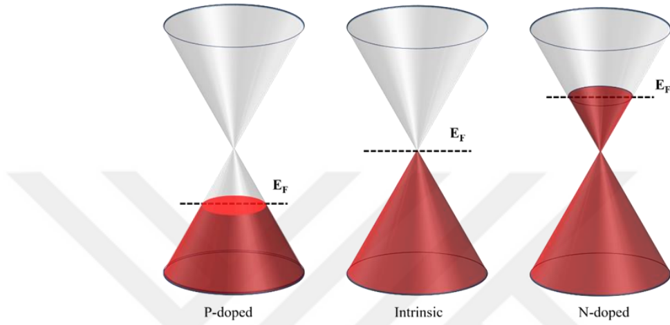
Figure 3.3 Graphene's Dirac cones in three different cases. P-doped graphene is obtained by introducing holes to the graphene and therefore, Fermi energy shifted down. In the pristine graphene, Fermi level is at the Dirac point. The n-doped graphene is electron injected and Fermi energy is shifted up.
