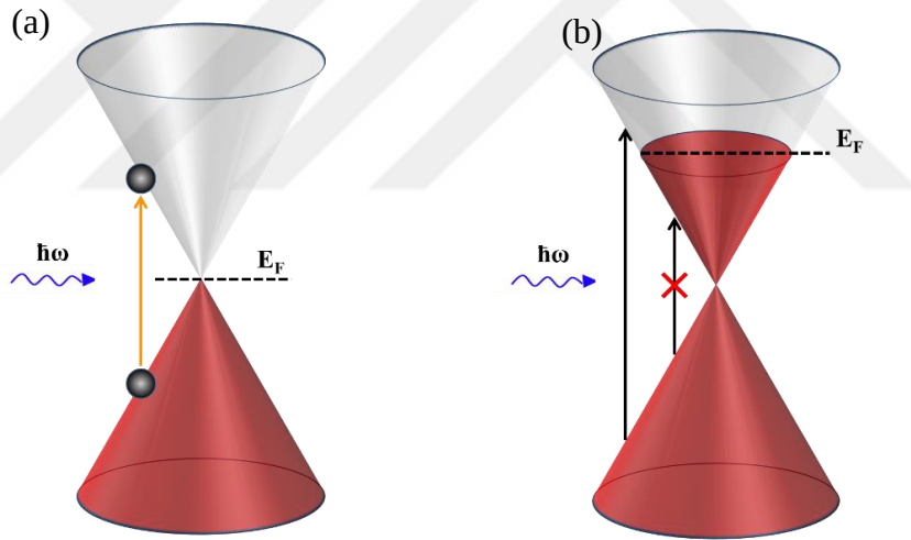
Figure 3.5 Interband transitions. (a) A photon with energy of 2E_F or more is absorbed by an electron exciting it from valence band to conduction band. (b) Optical transitions for energies less than 2E_F are blocked.
