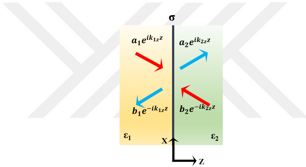
Figure 4.1 Schematic of optical response of monolayer graphene with conductivity of \sigma sandwiched between two dielectric media with dielectric constants of \epsilon_1 and \epsilon_2 . Forward and backward propagating electromagnetic waves with field coefficients of a_1 , a_2 , b_1 and b_2 , respectively.
