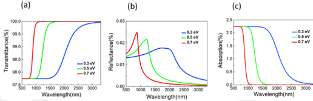
Figure 4.2 Optical response of free standing graphene at different fermi energies. (a) Transmittance of graphene is about 97.7% considering negligible reflectance yields 2.3% absorption. (b) Reflectance spectrum of graphene is inconsiderable and does not have significant effect on the graphene's absorption. (c) Absorption of graphene is about 2.3% in this region.
