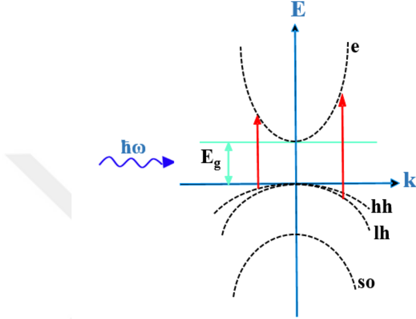
Figure 2.2 Schematic diagram of band structure of direct gap III-V semiconductors near to the center of Brillouin zone.
