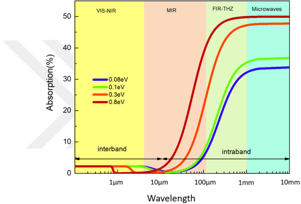
Figure 3.4 Wide-range optical response of graphene illustrated from visible to microwave spectrum. Graphene absorbs 2.3% of light at visible-near infrared region in which interband transitions arise from high energy photons. However, the absorption reaches 50% due to intraband transitions for low energy photons at terahertz and microwave area.
