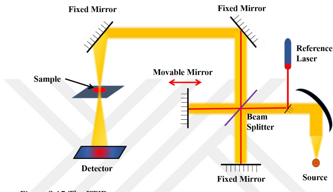
Figure 3.15 The FTIR spectrometer setup
