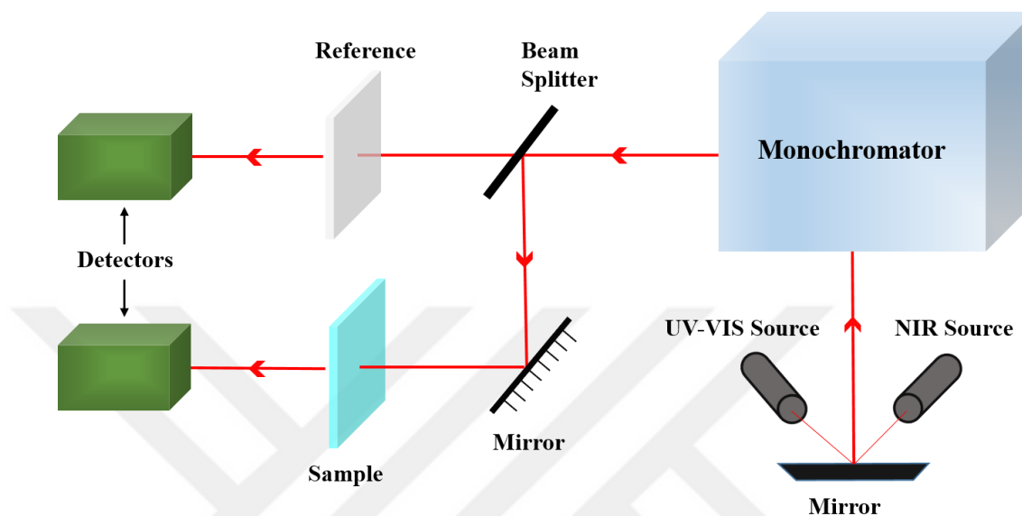
Figure 4.6 Simplified schematic of UV-Vis-NIR spectrophotometer. Light provided by source proceeds to monochromator and the narrow bandwidth outgoing beam of light splits into two beams by beam splitter. One of the beams is transmitted via the reference and the other passes through the sample. The ratio intensity of beams after detection by photo diodes is processed and the spectrum (transmittance vs wavelength) appears on display.
