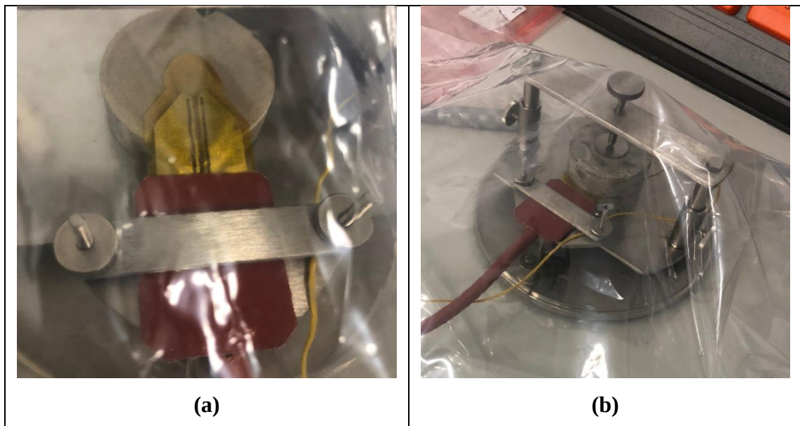
Figure 3. (a) and (b) Sensor position between grout samples.
