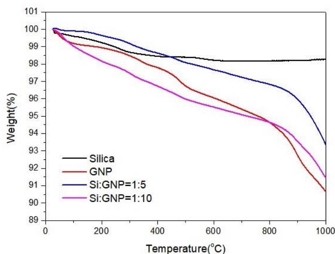
Figure 10. TGA curves of silica, GNP, Si:GNP=1:5 and Si:GNP=1:10 hybrid materials.
