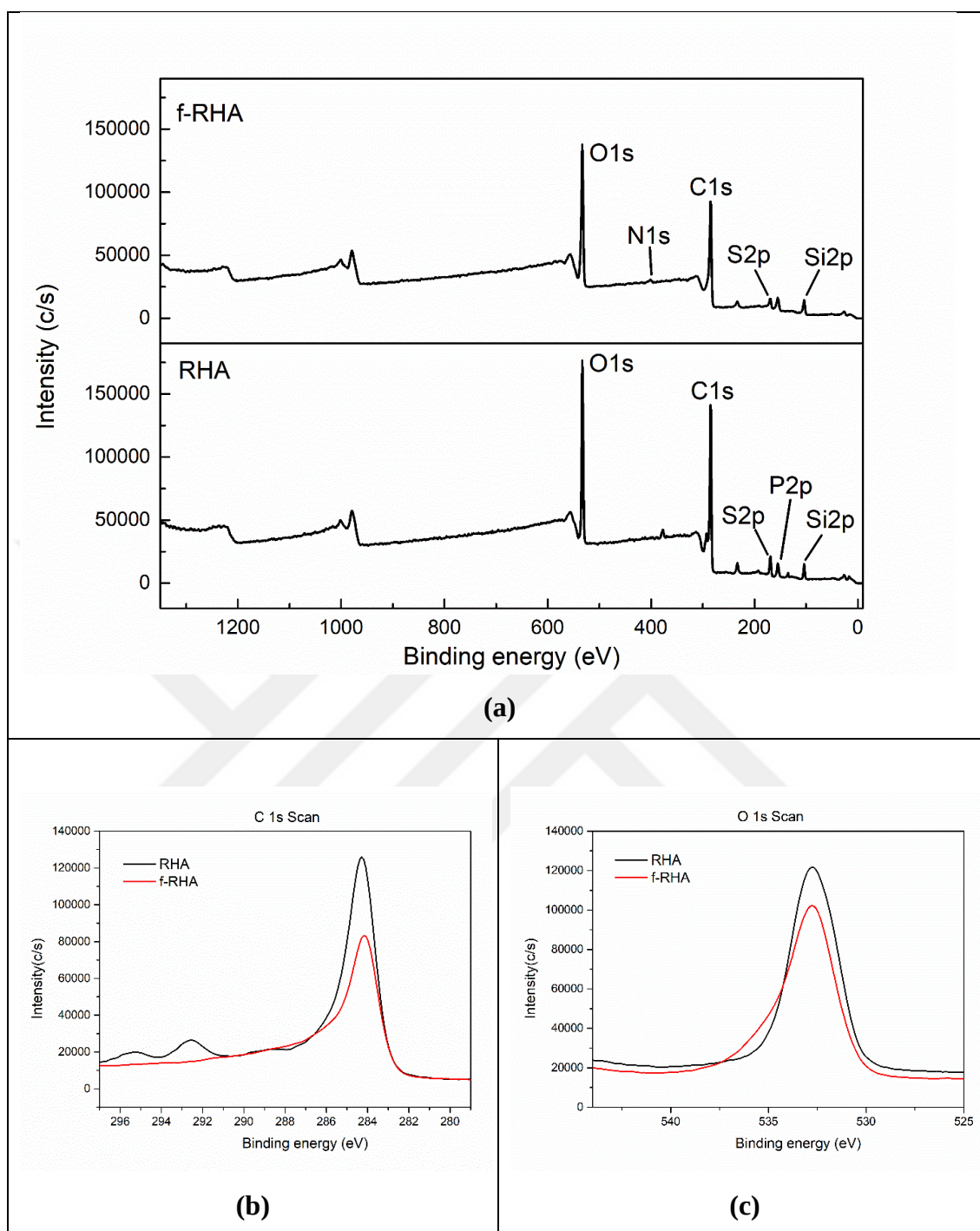
Figure 21. (a) XPS survey scan spectra, (b) C1s spectra and (c) O1s spectra of RHA and f-RHA.
