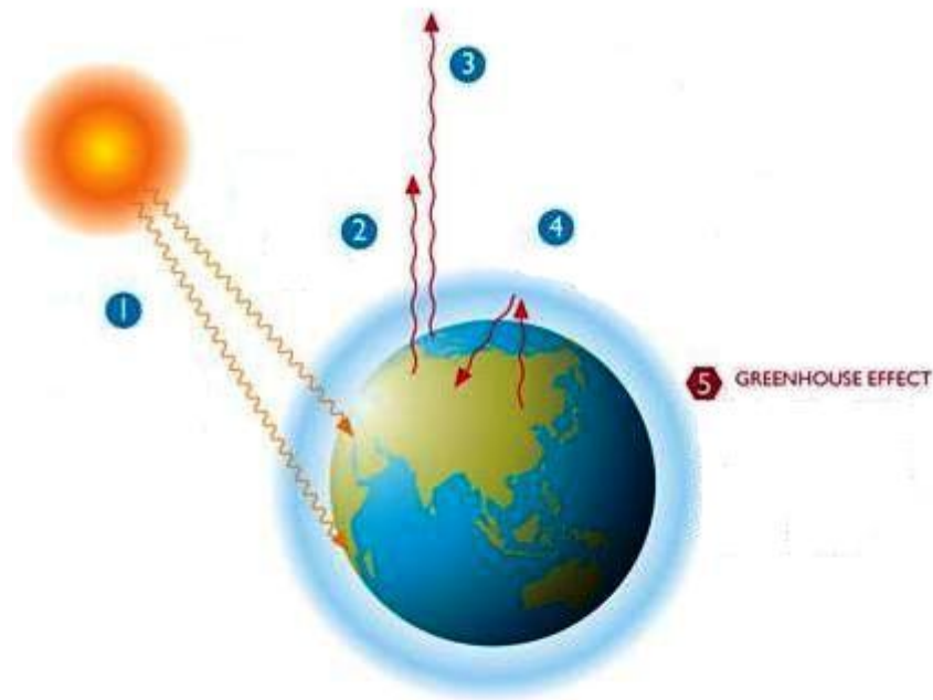
Figure 2.1 Greenhouse effect
