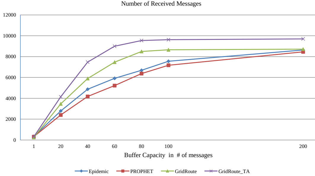
Figure 4.25: Number of received messages, CBMM, node count: 50, transmission range: 50 m, hop limit: 11.
