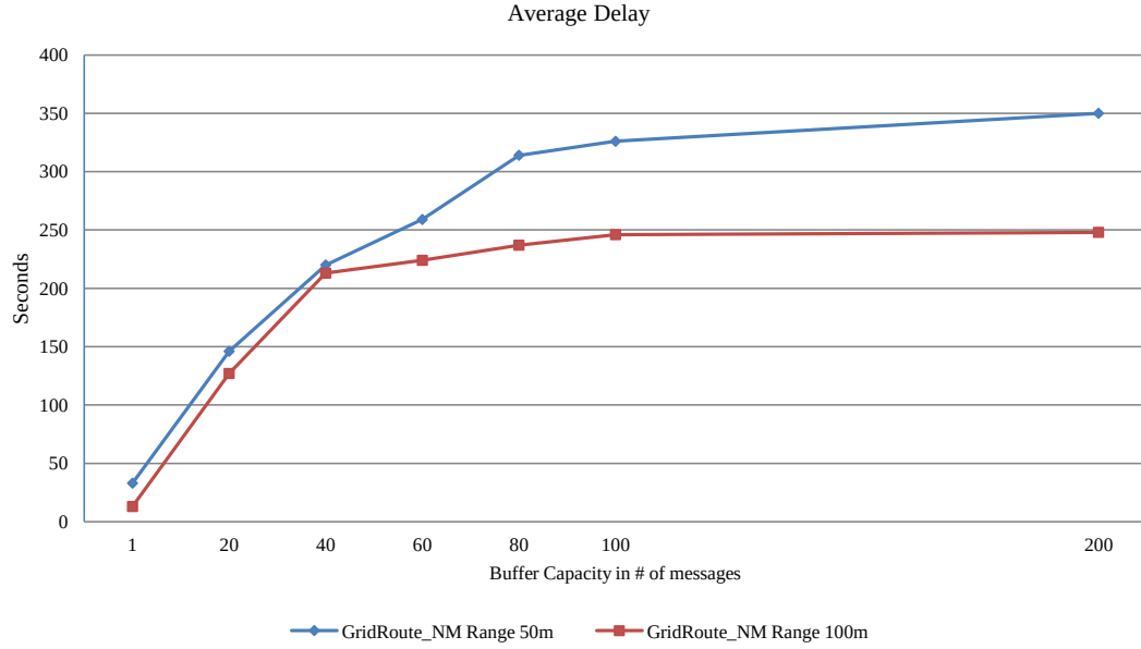
Figure 4.18: Average delay, GridRoute_NM, gateway simulation, range: 50 m, hop limit: 11.
