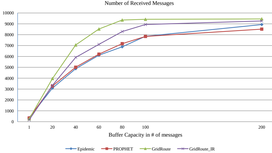
Figure 4.22: Number of received messages, CBMM, buffer size: 50 messages, node count: 50, transmission range: 100 m, hop limit: 11.
