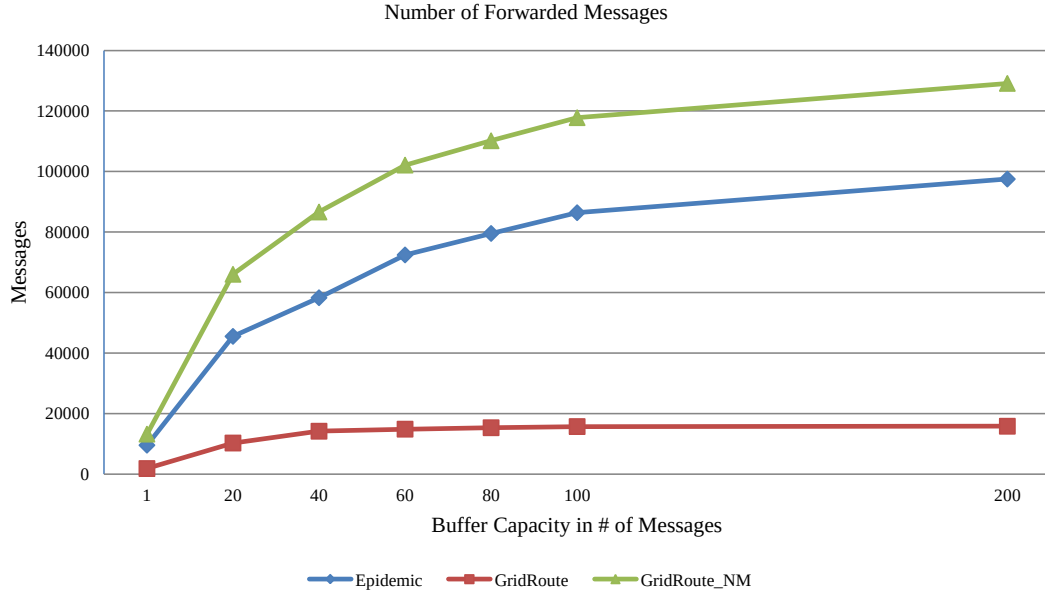
Figure 4.20: Number of forwarded messages, GridRoute_NM, CBMM simulation, range: 100 m, hop limit: 11.
