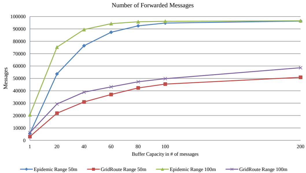
Figure 4.5: Number of forwarded messages, RWMM, hop limit: 11.
