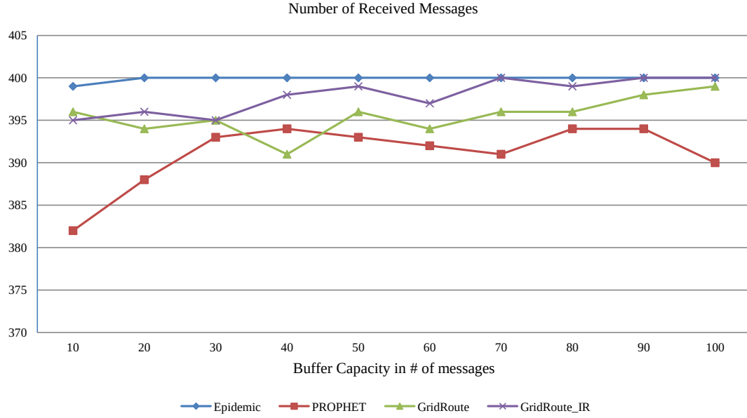
Figure 4.28: Number of received messages, CBMM, node count: 50, transmission range: 100 m, hop limit: 11.
