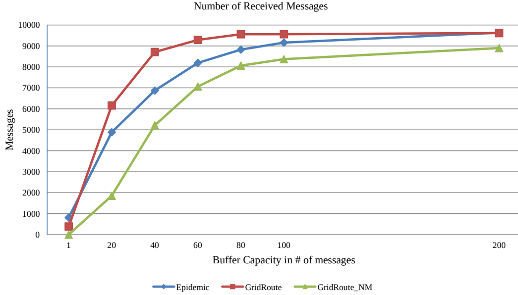
Figure 4.19: Number of received messages, GridRoute_NM, CBMM simulation, range: 100 m, hop limit: 11.
