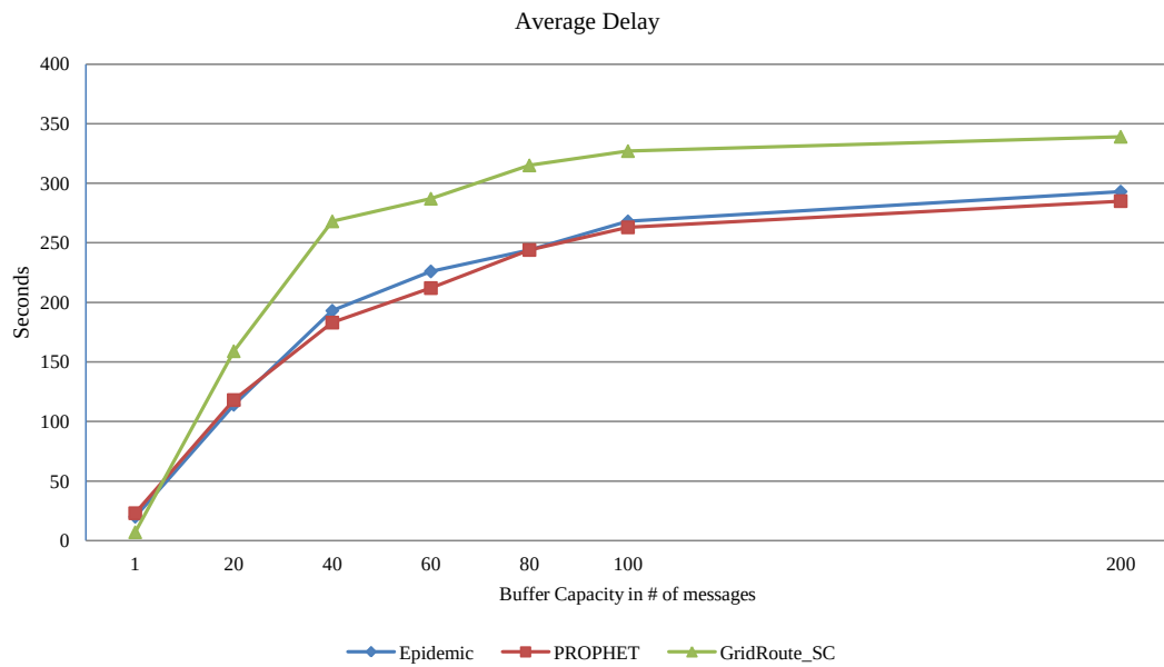
Figure 4.13: Average delay, CBMM, range: 100 m.
