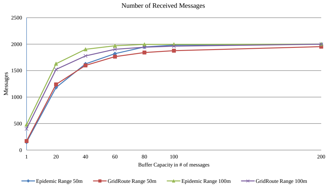
Figure 4.3: Number of received messages, RWMM, hop limit: 11.
