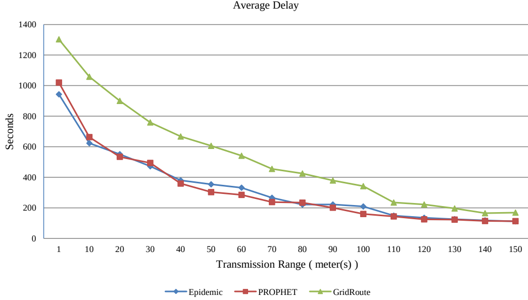
Figure 4.36: Average delay, CBMM, buffer size: 50 messages, node count: 50, hop limit: 11.
