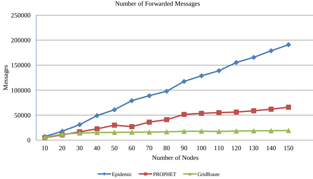
Figure 4.38: Number of forwarded messages, CBMM, buffer size: 50 messages, transmission range: 100 m, hop limit: 11.
