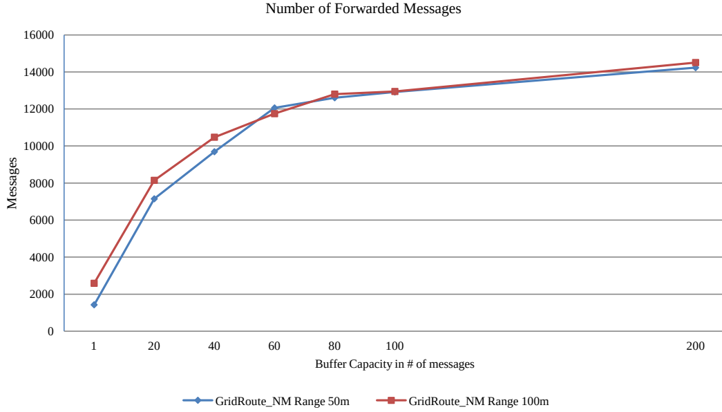
Figure 4.17: number of forwarded messages, GridRoute_NM, gateway simulation, range: 50 m, hop limit: 11.
