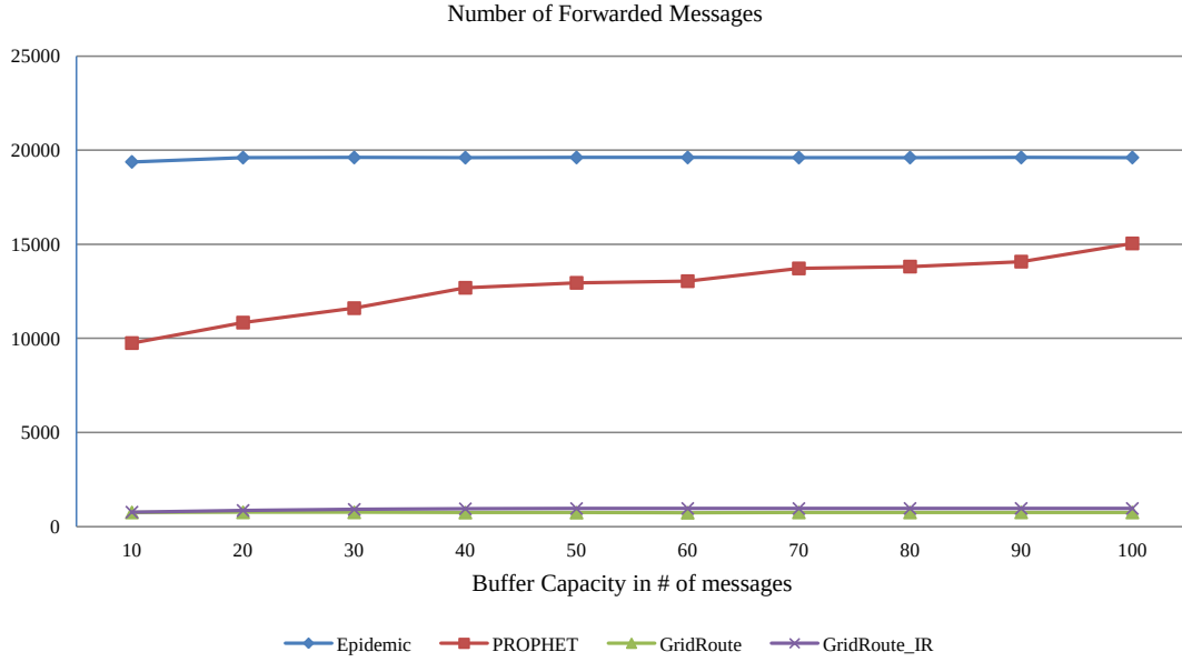
Figure 4.29: Number of received messages, CBMM, node count: 50, transmission range: 100 m, hop limit: 11.
