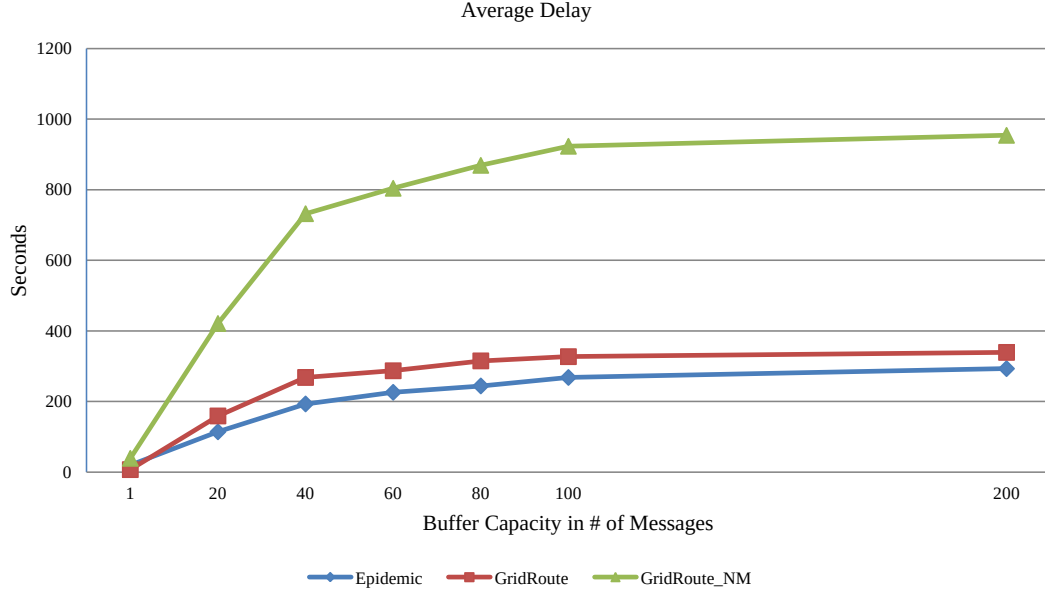
Figure 4.21: Average delay, GridRoute_NM, CBMM simulation, range: 100 m, hop limit: 11.
