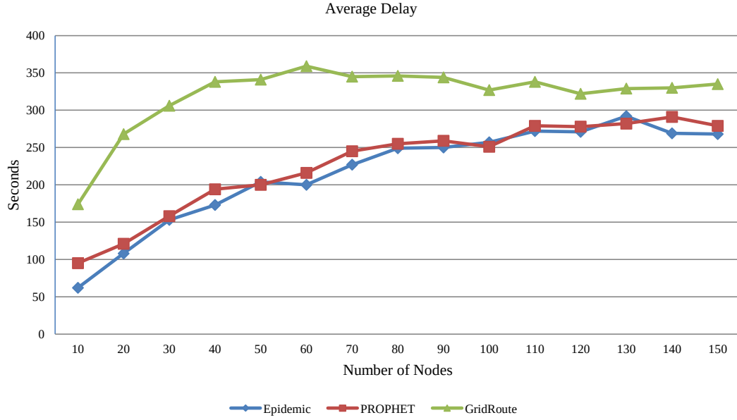
Figure 4.39: Average delay, CBMM, buffer size: 50 messages, transmission range: 100 m, hop limit: 11.
