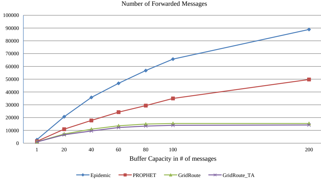
Figure 4.26: Number of received messages, CBMM, node count: 50, transmission range: 50 m, hop limit: 11.
