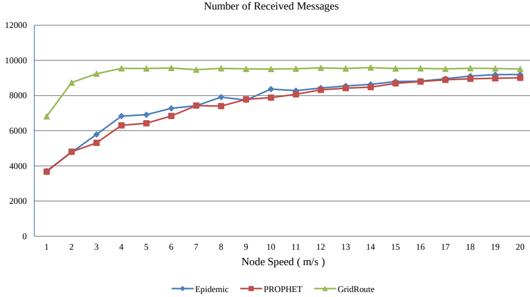
Figure 4.40: Number of received messages, CBMM, node count: 50, buffer size: 50 messages, transmission range: 100 m, hop limit: 11.
