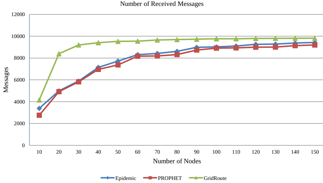
Figure 4.37: Number of received messages, CBMM, buffer size: 50 messages, transmission range: 100 m, Hop Limit: 11.
