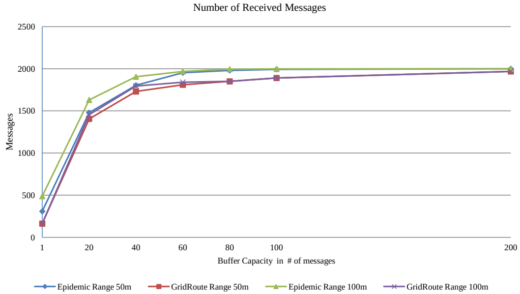
Figure 4.2: Number of received messages, RWMM, hop limit: 3.
