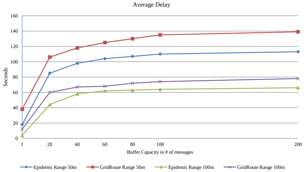
Figure 4.6: Average delay, RWMM, hop limit: 3.
