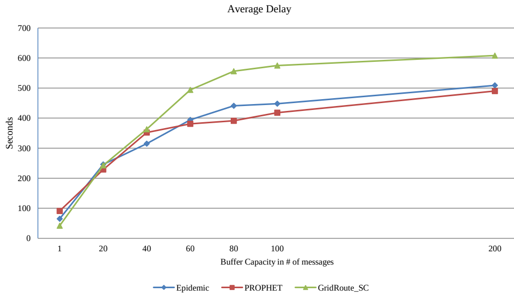
Figure 4.12: Average delay, CBMM, range: 50m.
