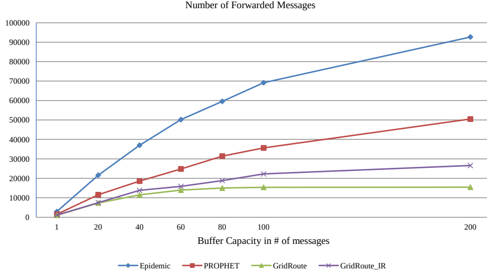
Figure 4.23: Number of received messages, CBMM, node count: 50, transmission range: 50 m, hop limit: 11.
