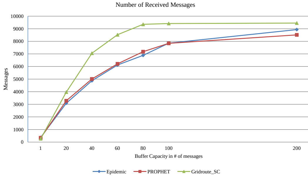
Figure 4.8: Number of received messages, CBMM, range: 50 m.
