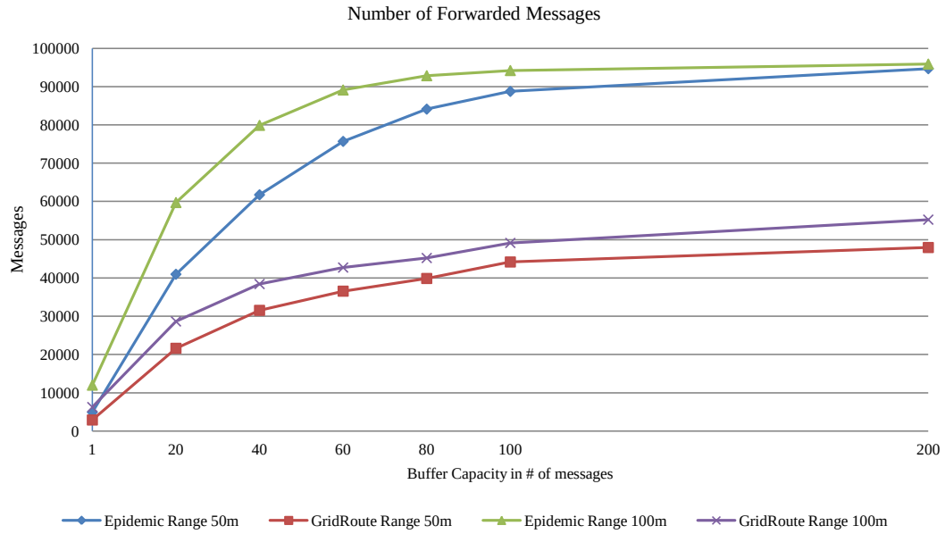
Figure 4.4: Number of forwarded messages, RWMM, hop limit: 3.
