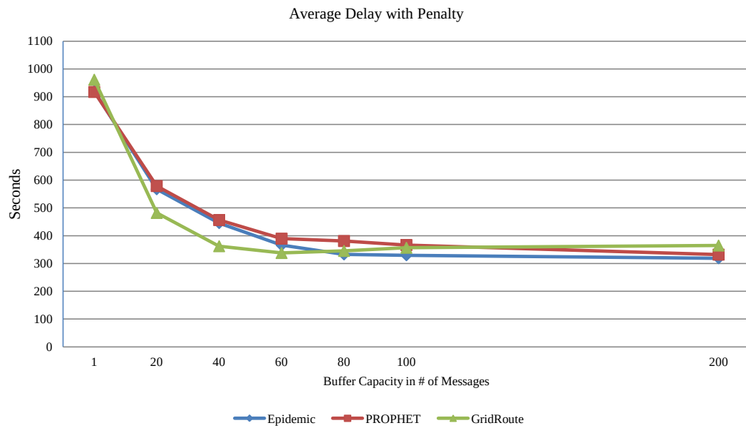
Figure 4.15: Average delay with undelivery penalty, CBMM, range: 100 m.
