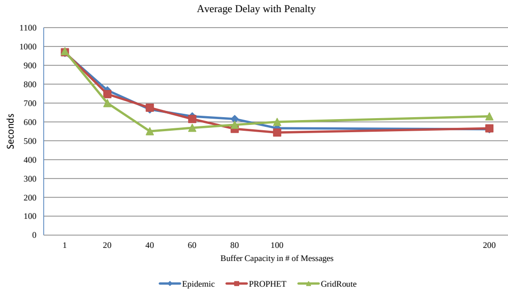
Figure 4.14: Average delay with undelivery penalty, CBMM, range: 50 m.
