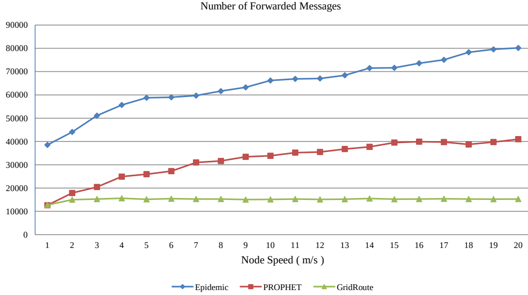
Figure 4.41: Number of forwarded messages, CBMM, node count: 50, buffer size: 50 messages, transmission range: 100 m, hop limit: 11.
