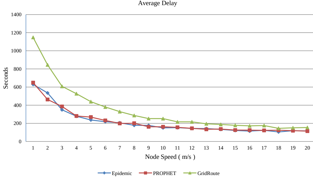
Figure 4.42: Average delay, CBMM, node count: 50, buffer size: 50 messages, transmission range: 100 m, hop limit: 11.
