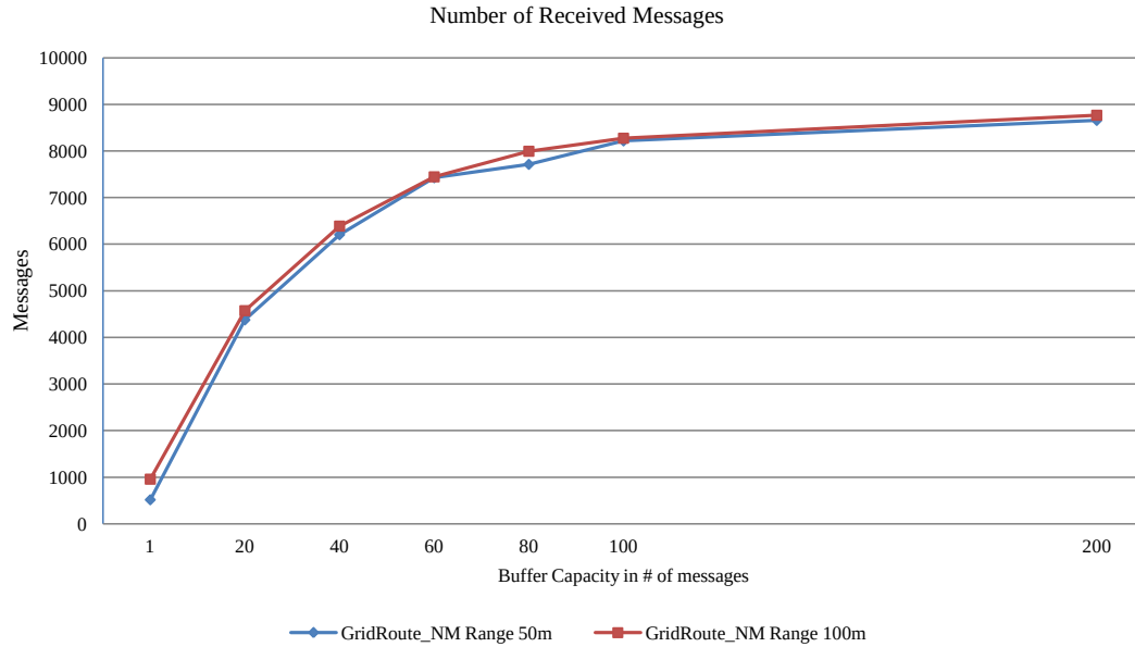
Figure 4.16: Number of received messages, GridRoute_NM, gateway simulation, range: 50 m, hop limit: 11.
