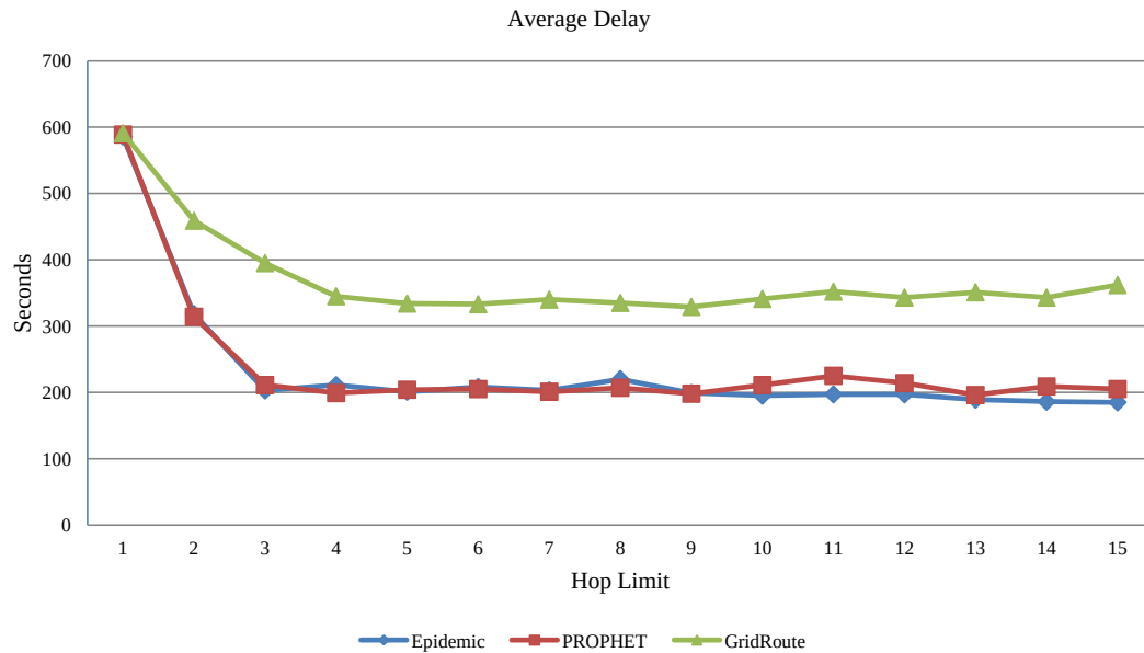
Figure 4.33: Average delay, CBMM, buffer size: 50 messages, node count: 50, transmission range: 100 m.
