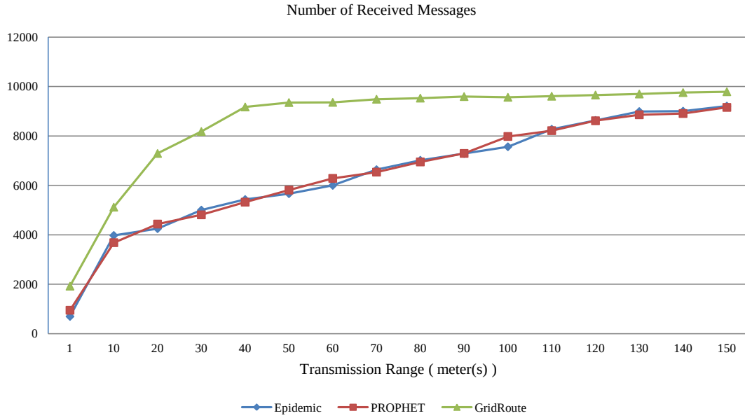
Figure 4.34: Number of received messages, CBMM, buffer size: 50 messages, node count: 50, hop limit: 11.
