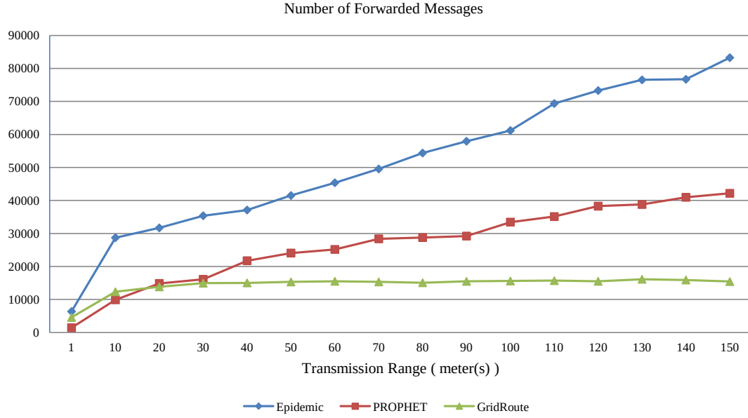
Figure 4.35: Number of forwarded messages, CBMM, buffer size: 50 messages, node count: 50, hop limit: 11.
