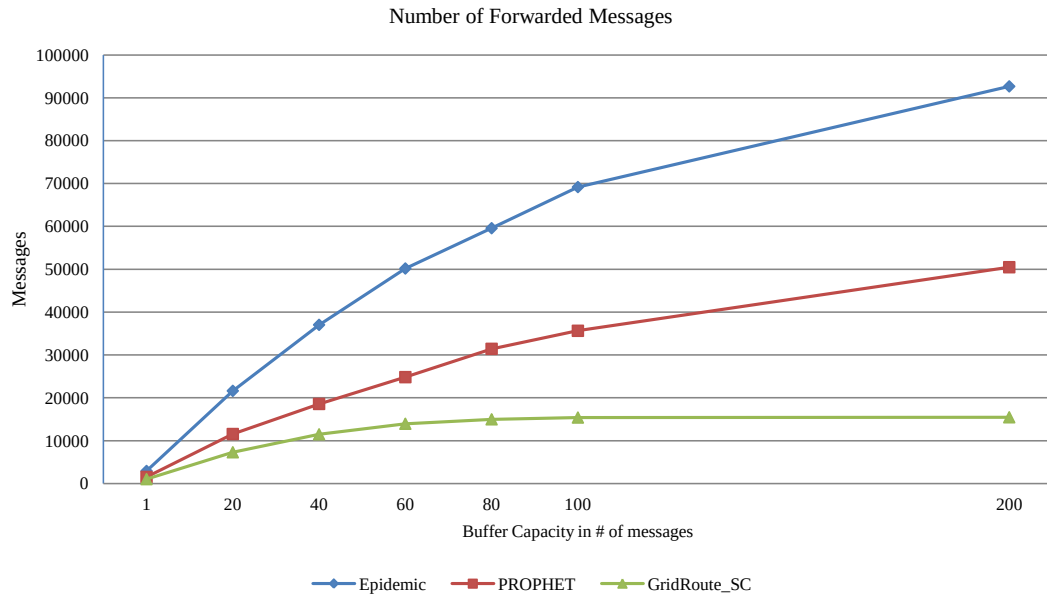
Figure 4.10: Number of forwarded messages, CBMM, range: 50 m.
