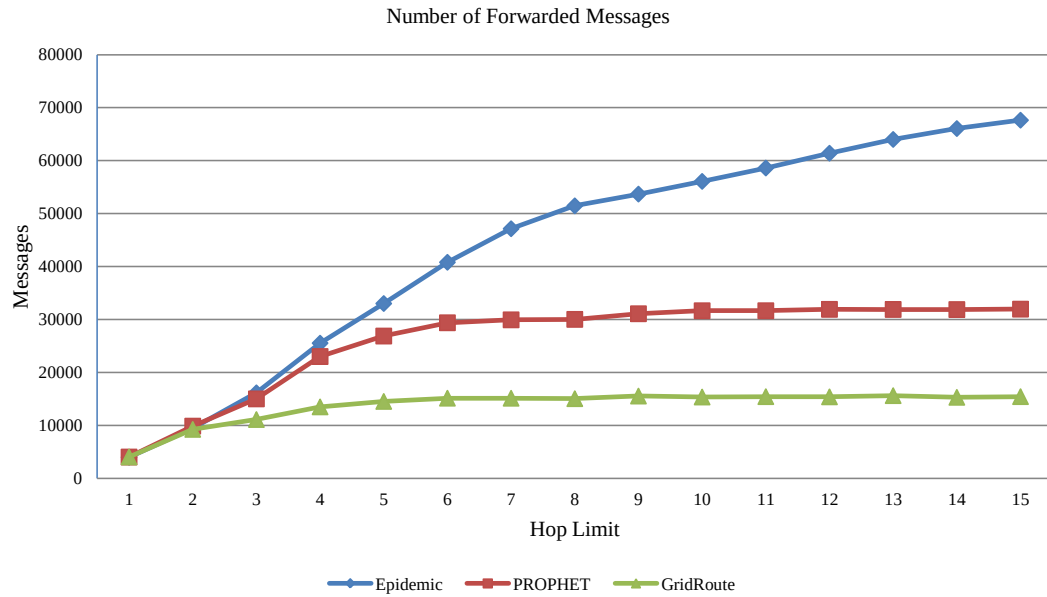
Figure 4.32: Number of forwarded messages, CBMM, buffer size: 50 messages, node count: 50, transmission range: 100 m.
