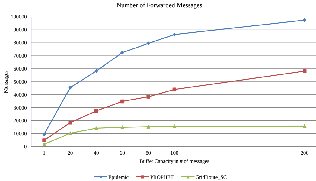
Figure 4.11: Number of forwarded messages, CBMM, range: 100 m.
