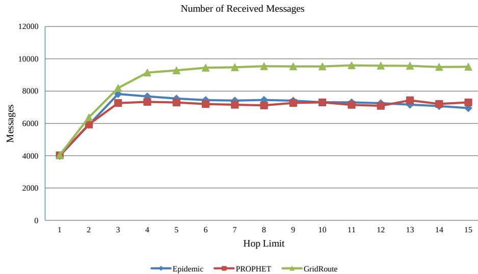
Figure 4.31: Number of received messages, CBMM, node count: 50, transmission range: 50 m.
