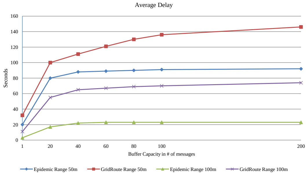
Figure 4.7: Average delay, RWMM, hop limit: 11.
