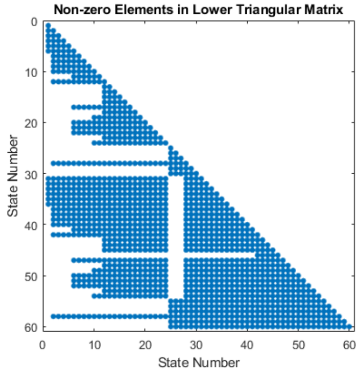
Figure 4.4: The lower triangular matrix of the gain matrix in Figure 2.3
