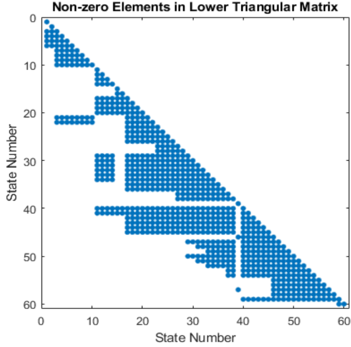
Figure 4.7: The lower triangular matrix of the Gain matrix after the decomposition process
