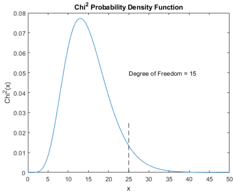
Figure 2.4: Probability density function for \chi^2 .
