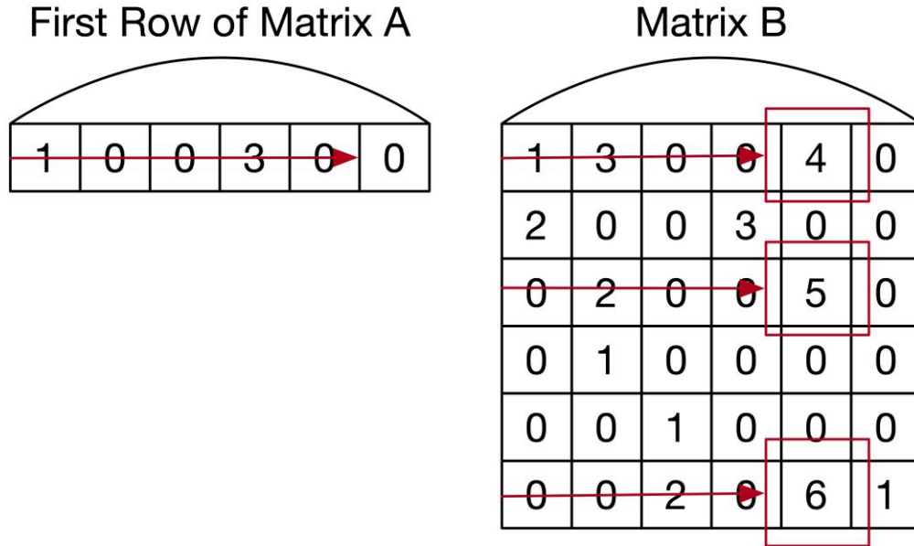
Figure 4.2: The linked list search of row order “Knuth’s Method” in the multiplication of the first row of Matrix A and fifth column of Matrix B
