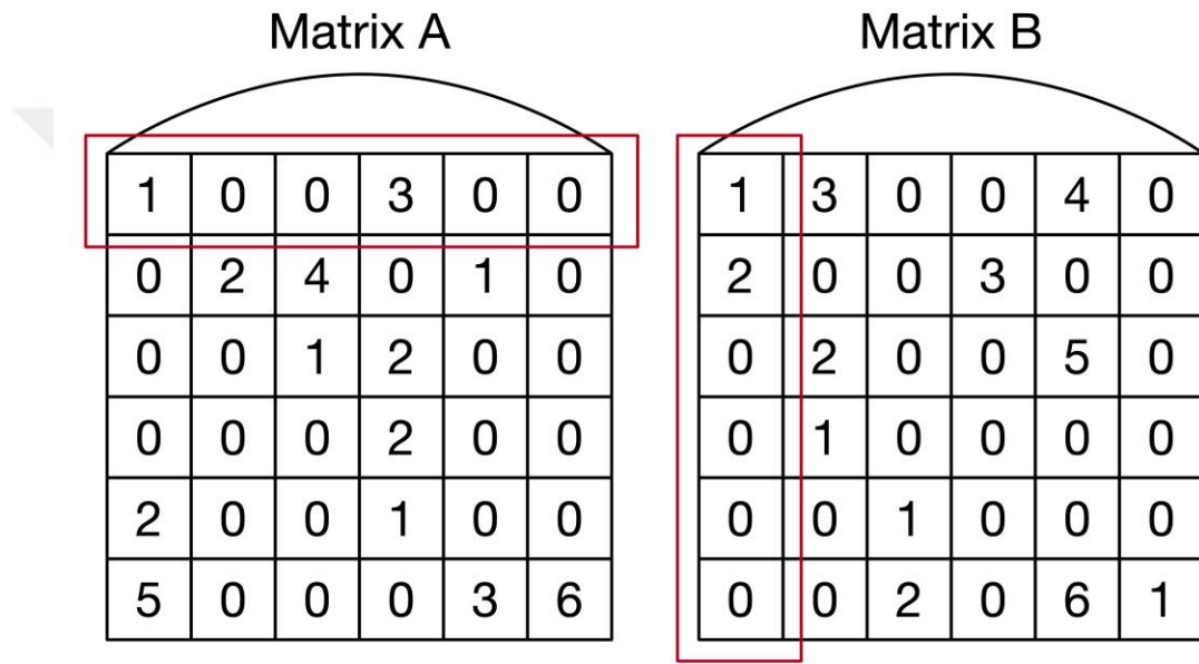
Figure 4.1: The visualization of matrix multiplication for first row first column
