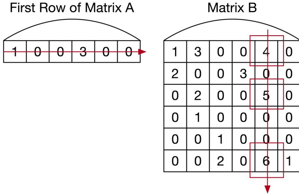
Figure 4.3: The linked list search of the proposed method in the multiplication process of the first row of Matrix A and fifth column of Matrix B
