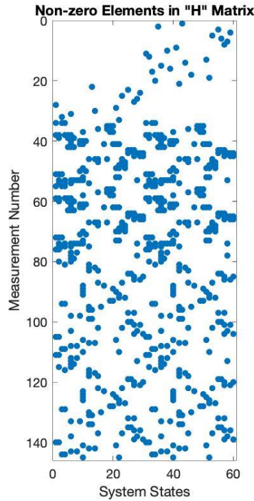
Figure 2.2: The “ H ” matrix sparse structure.
