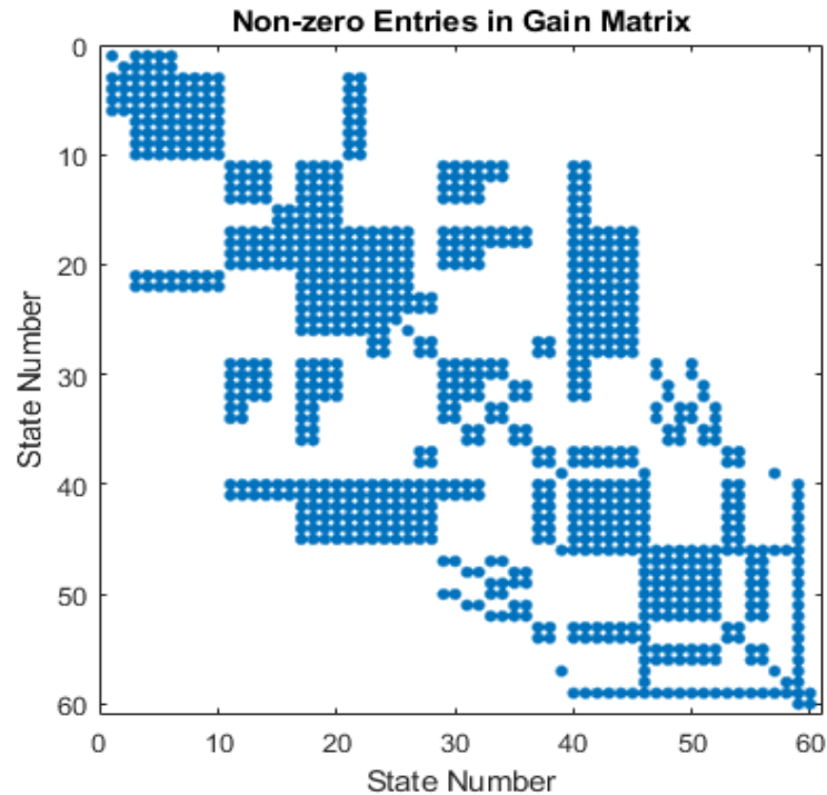
Figure 4.6: The Gain matrix after Reverse Cuthill McKee algorithm applied
