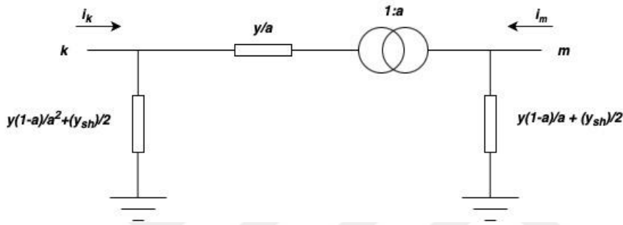
Figure 2.1: The generalized \pi model of a transformer.
