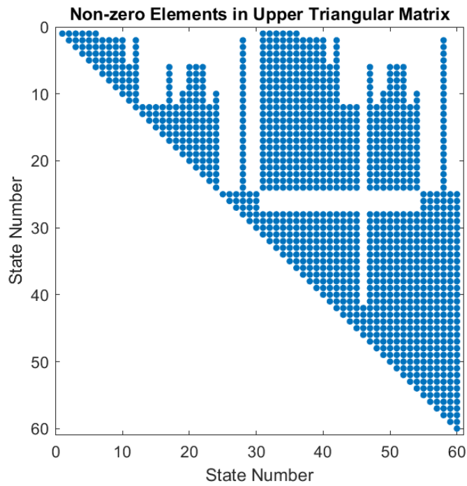
Figure 4.5: The upper triangular matrix of the gain matrix in Figure 2.3
