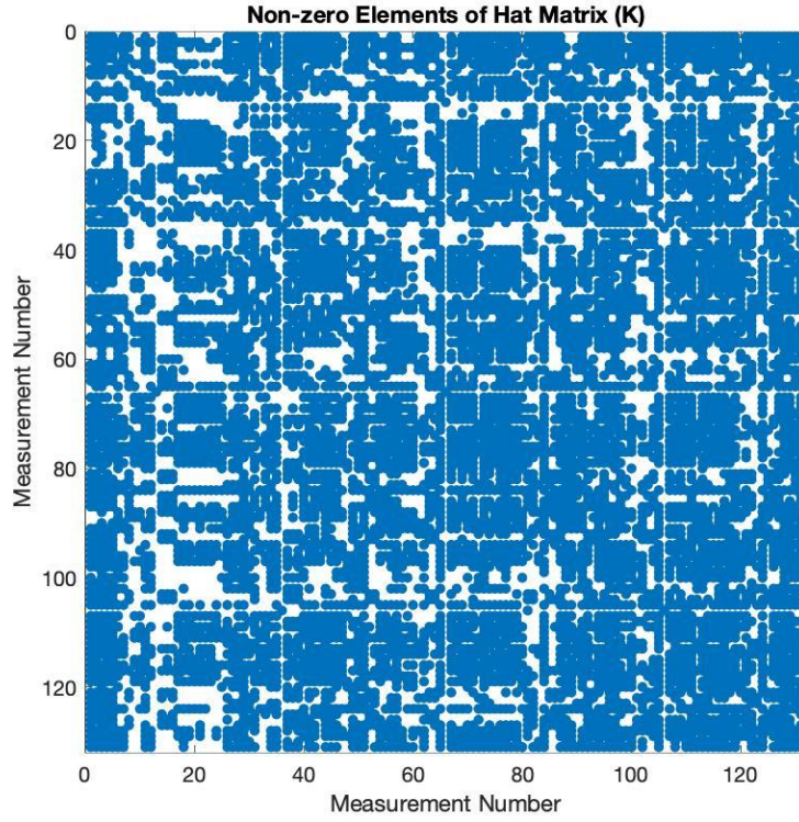
Figure 2.6: The structure of the hat matrix ( K ).
