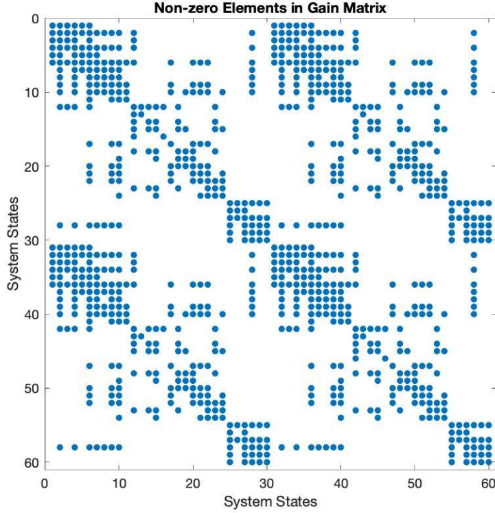
Figure 2.3: The Gain Matrix sparse structure.
