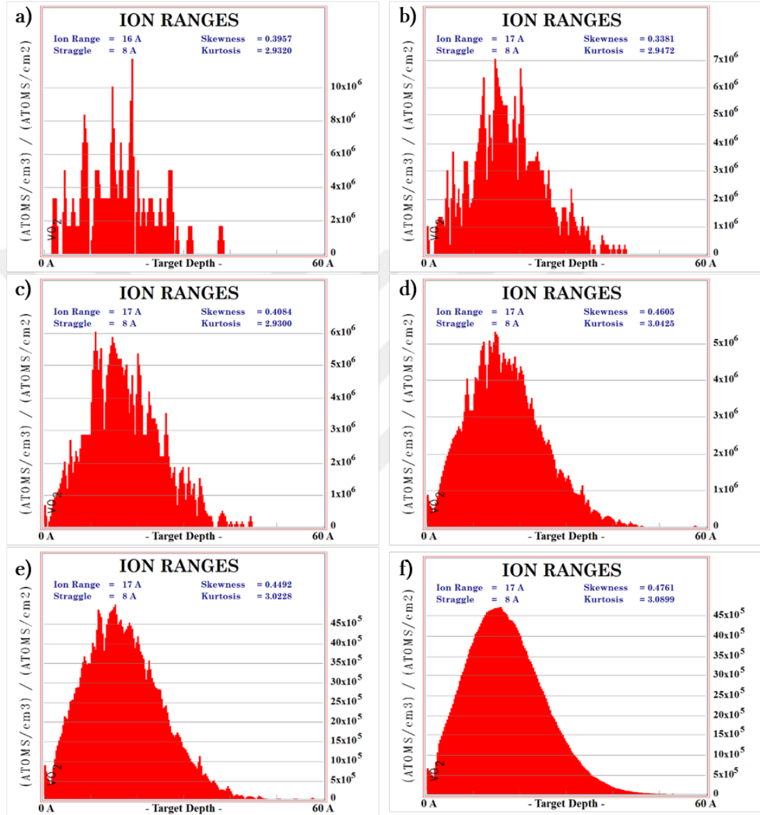
Figure 3.3: Evolution of the Ar-ion distribution in the VO 2 crystal. Majority of the ions are located at 1.7 nm from the surface of the crystal.
