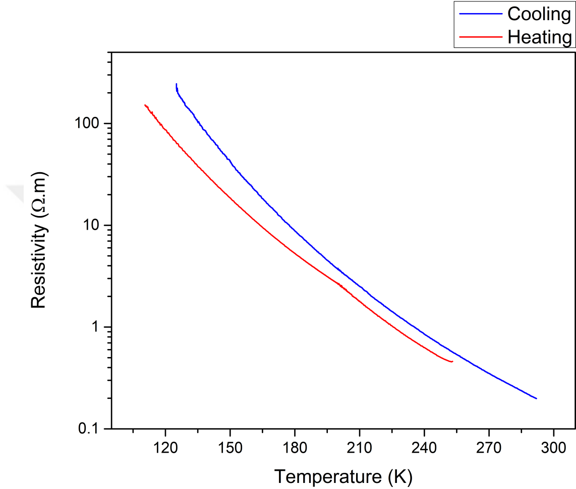
Figure 3.12: Resistivity vs. temperature curve of the 119 nm thick VO 2 device. The device failed while it reached 255 K during the heating cycle.
