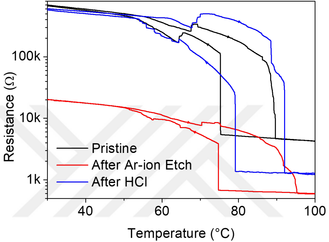
Figure 3.5: Resistance vs temperature cycle of pristine, milled and HCl treated VO 2 . The milled VO 2 has reduced resistance response due to being in series connection with the ion-beam induced damaged layer. The nanobeam retrieves its pristine electrical properties after HCl treatment. Taken from ref. [32].
