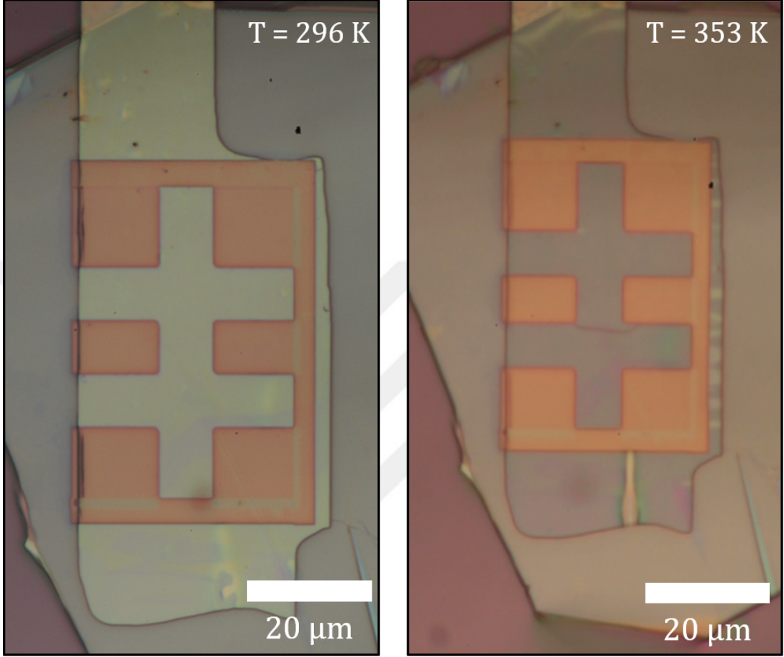
Figure 3.7: A 174 nm thick \text{VO}_2 crystal shaped into Hall-bar geometry cracks during the MIT as a result of the stress introduced by the structural phase transition.
