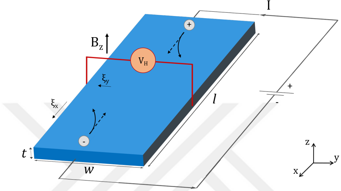
Figure 1.1: An illustration of a simple Hall effect measurement system.
