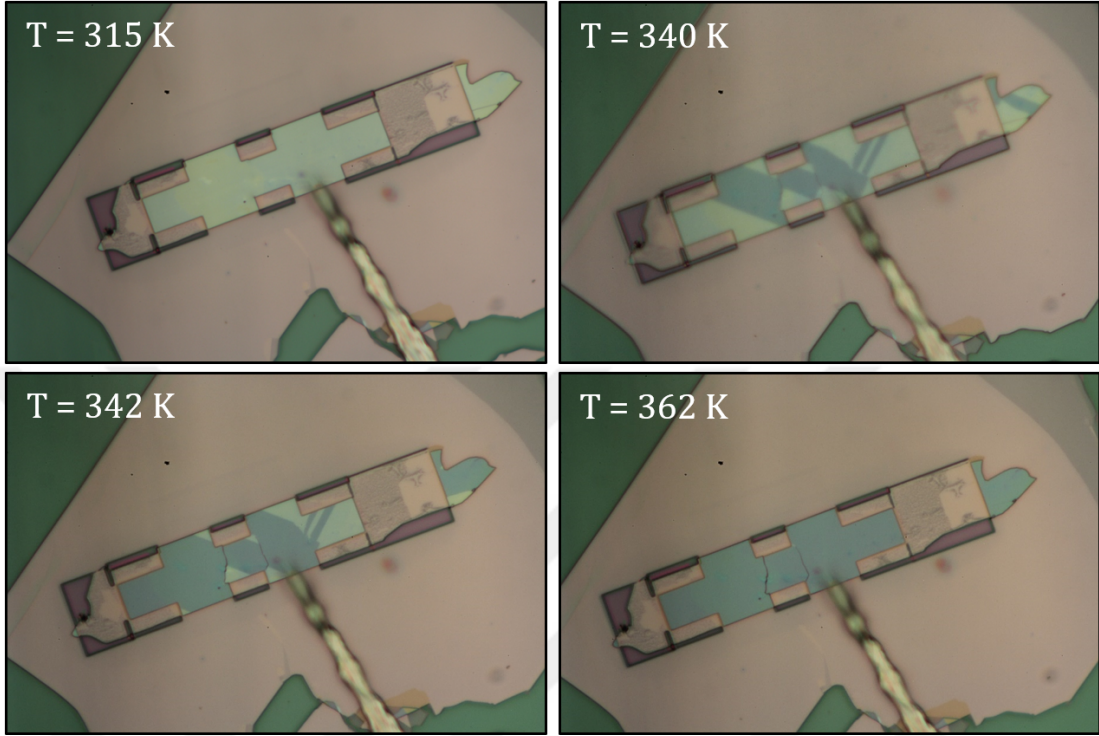
Figure 3.6: Two cracks appear on a 160 nm thick Hall-bar shaped \text{VO}_2 crystal during the MIT as a result of the stress introduced by the structural phase transition.
