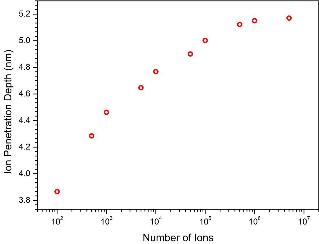
Figure 3.2: SRIM results showing the Ar-ion damage on the \text{VO}_2 crystal with increasing number of ions. The maximum depth of implanted ions converge to 5.2 nm from the surface of the crystal.
