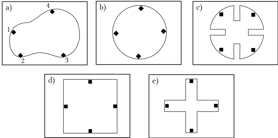
Figure 1.2: Lamella-type van der Pauw structures.
