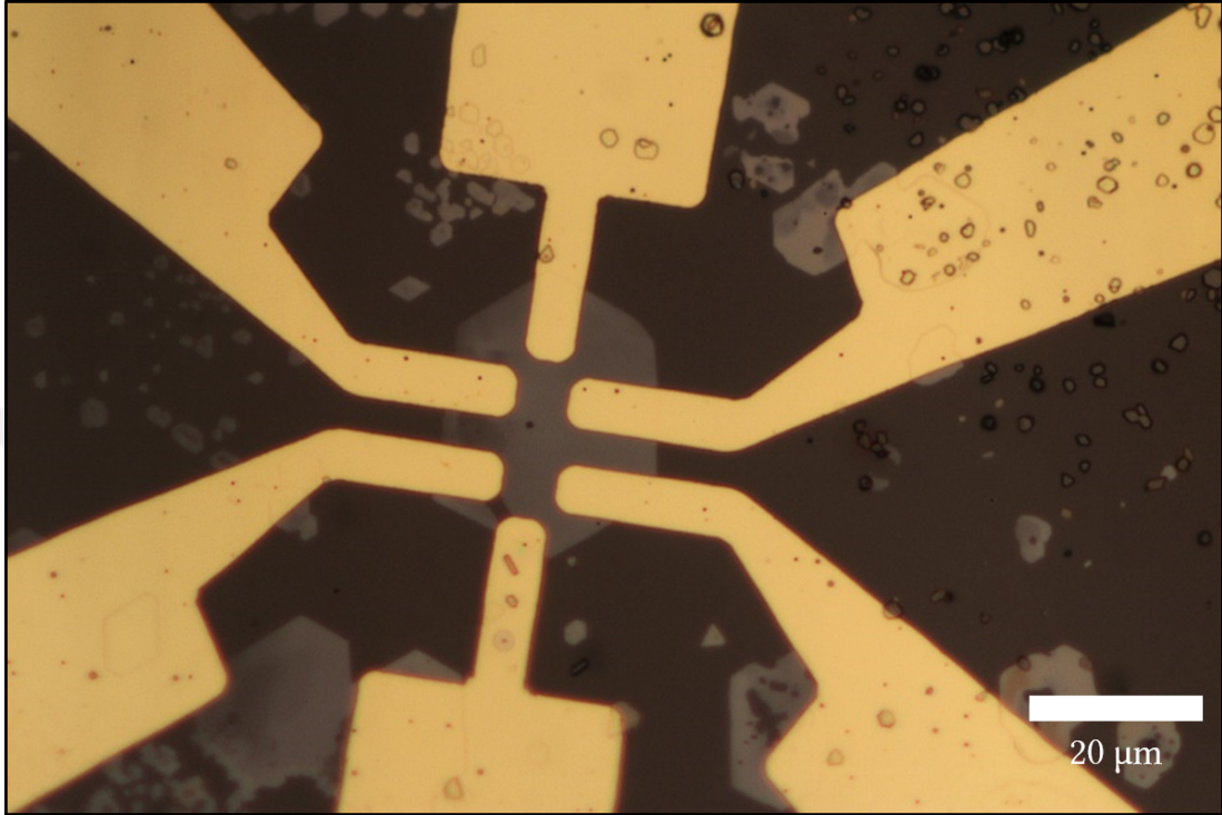
Figure 3.14: Optical image of a 6-terminal \text{V}_2\text{O}_3 device used to investigate the magnetotransport properties.
