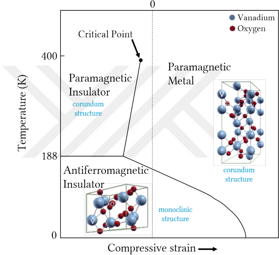
Figure 1.8: The phase diagram of V_2O_3 based on reference [22]. The paramagnetic metal (PM) and insulator (PI) phases have corundum structure, while the antiferromagnetic insulator phase (AFI) has a monoclinic structure.
