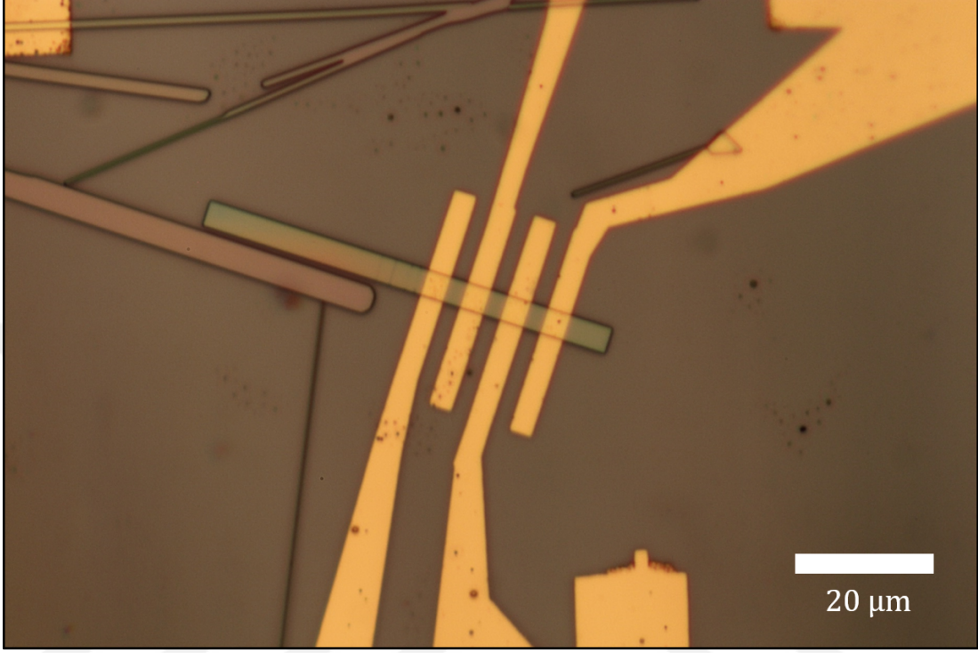
Figure 3.11: Optical image of a 4-terminal VO 2 device used in magnetoresistance measurements.
