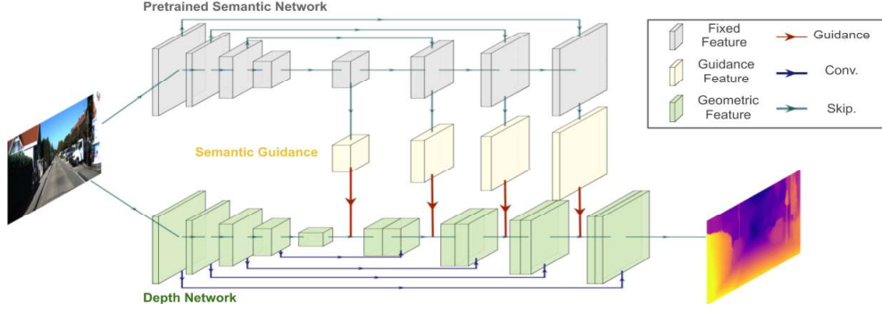
Figure 3.7: A diagram of the semantically guided depth estimation network proposed by [9]. Figure source: Guizilini et al. [9].
