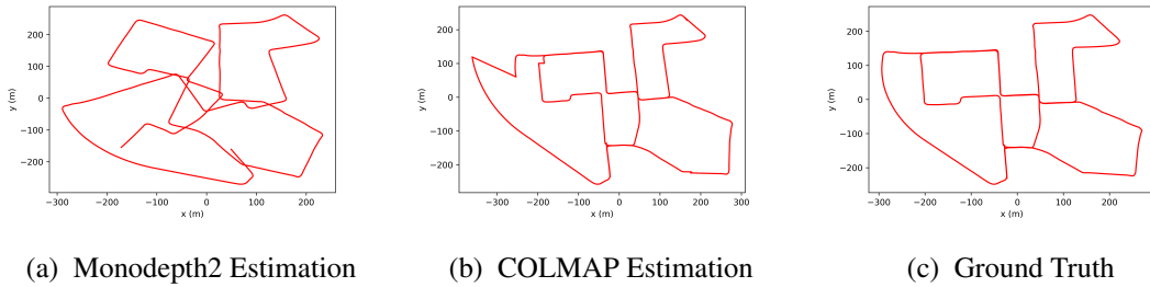
Figure A.1: Trajectory estimations with Monodepth2 and COLMAP on Sequence-0 of KITTI Odometry Dataset
