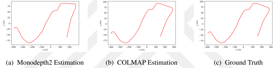
Figure A.9: Trajectory estimations with Monodepth2 and COLMAP on Sequence-10 of KITTI Odometry Dataset
