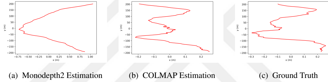
Figure A.4: Trajectory estimations with Monodepth2 and COLMAP on Sequence-4 of KITTI Odometry Dataset
