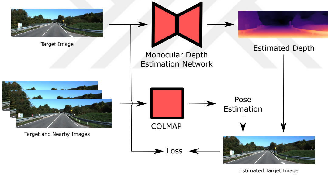
Figure 4.3: Schematic diagram of the training methodology. During training, relative poses are computed by using COLMAP instead of a pose estimator DNN.
