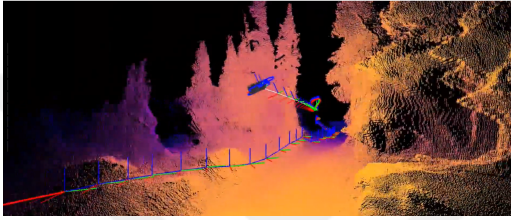
(c) Skydio 2 [17]
