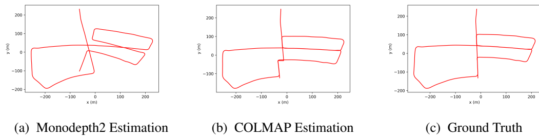
Figure A.5: Trajectory estimations with Monodepth2 and COLMAP on Sequence-5 of KITTI Odometry Dataset
