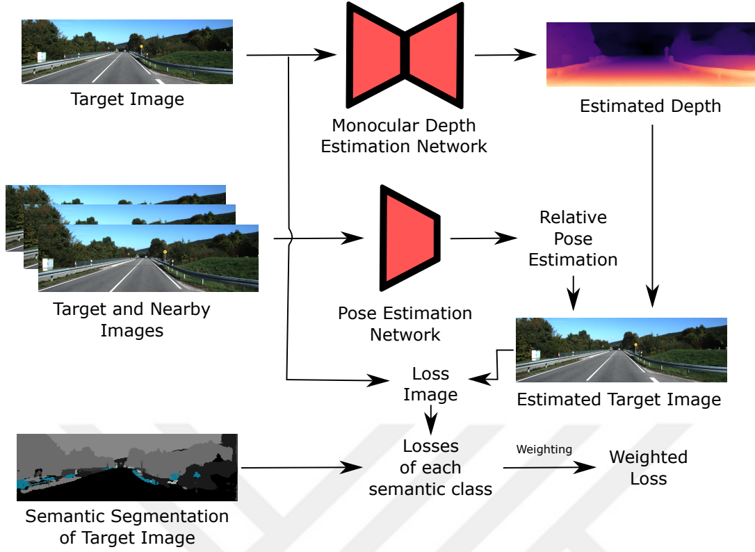
Figure 4.11: A schematic of semantic weighting process of losses of different semantic classes.
