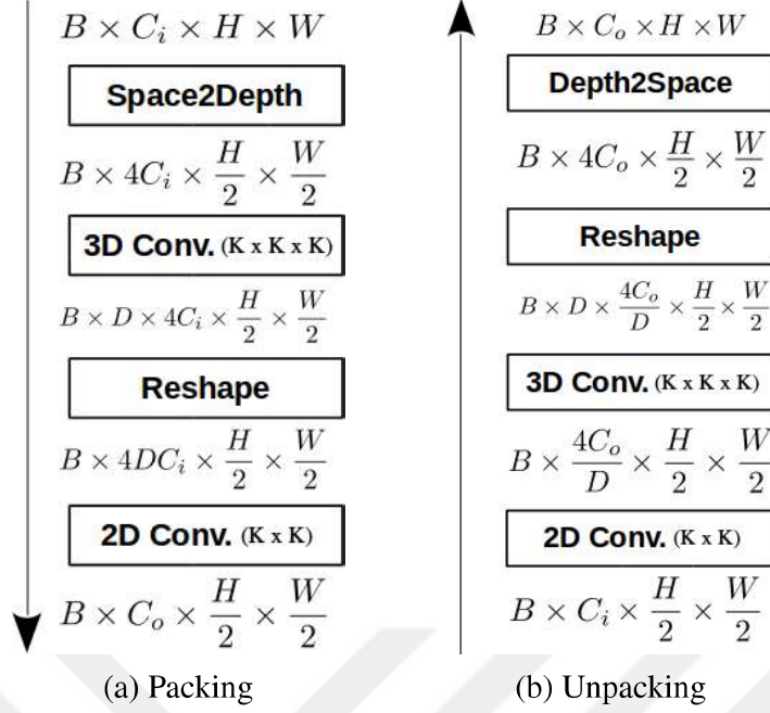
Figure 3.3: The inside architecture of the proposed packing and unpacking blocks. Figure source: [5].
