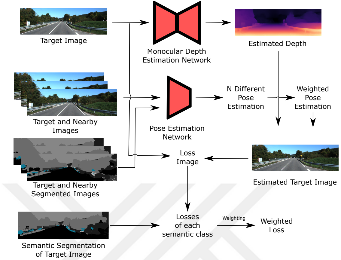
Figure 4.12: A schematic of semantic weighting process of poses of different semantic classes.
