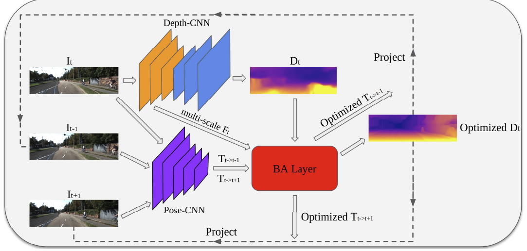
Figure 3.5: The proposed unsupervised depth and pose estimation network which adapts the differentiable BA layer [6]. Figure source: Shi et al. [7].
