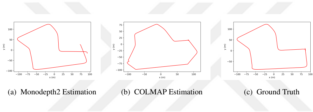
Figure A.7: Trajectory estimations with Monodepth2 and COLMAP on Sequence-7 of KITTI Odometry Dataset
