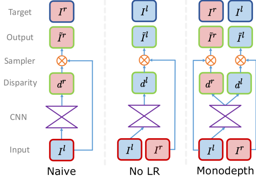
Figure 3.1: Different approaches for Monodepth to train the disparity network [4].
