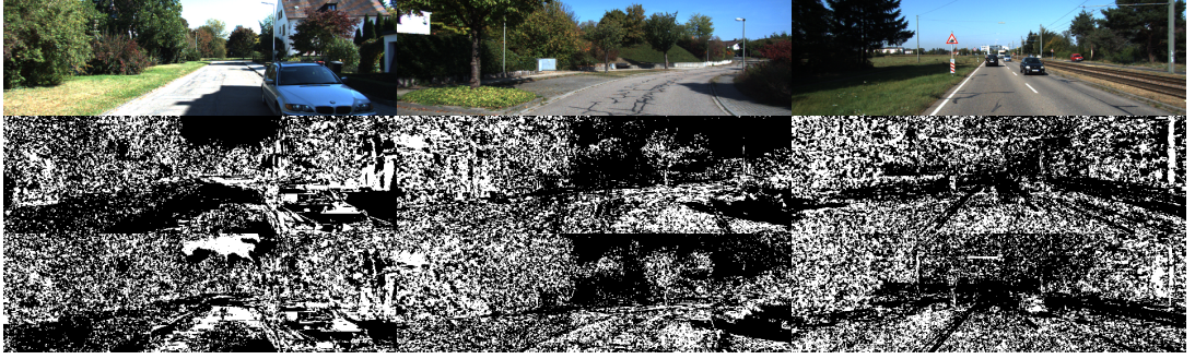
Figure 4.8: Illustration of the filtered pixels for the input images from training split proposed by Eigen et al. [10] in KITTI 2012 Dataset [2]. The input images are located in the row, the selected pixels with default setting of Monodepth2 are shown in the second row, and the selected pixels when frames taken at t_{i\pm 7} are added to training process are shown in the third row. The white pixels are selected for loss calculation and black pixels are filtered out and not being used for training.
