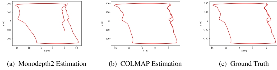
Figure A.6: Trajectory estimations with Monodepth2 and COLMAP on Sequence-6 of KITTI Odometry Dataset
