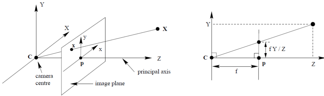
Figure 2.1: The pinhole camera projection model in [3]. The camera center is \mathbf{C} and \mathbf{p} is the principal point.
