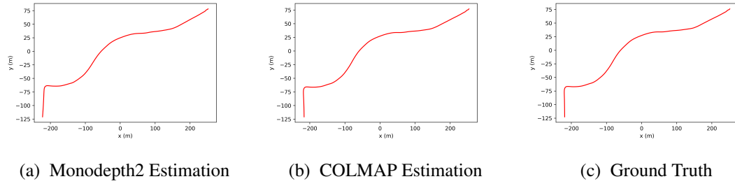
Figure A.3: Trajectory estimations with Monodepth2 and COLMAP on Sequence-3 of KITTI Odometry Dataset
