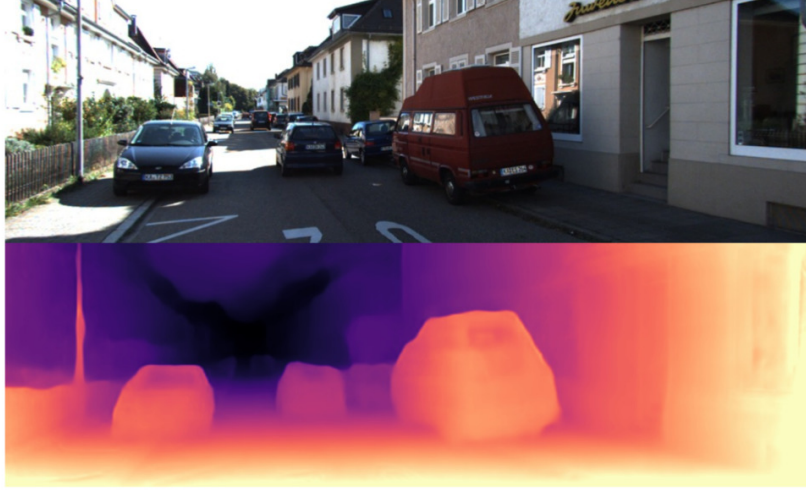
Figure 1.1: An illustration of the depth estimation concept. A depth value is predicted for each pixel in the monocular input image.
