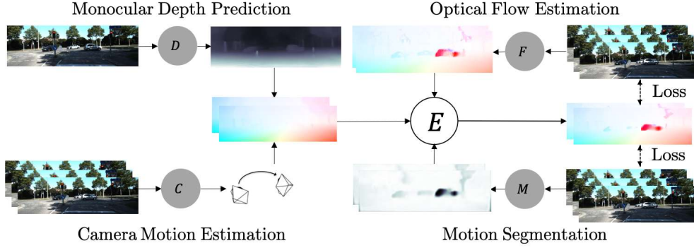
Figure 3.6: A schematic diagram of the Ranjan et al. [8]. Four different network performs dense depth estimation, relative pose estimation, optical flow estimation, and motion segmentation. Figure source: Ranjan et al. [8].
