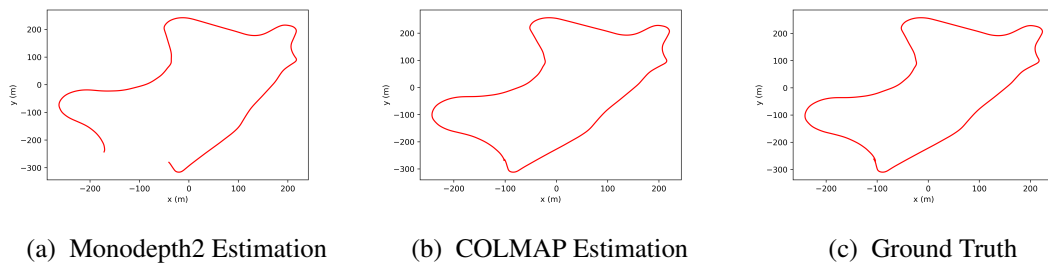
Figure A.8: Trajectory estimations with Monodepth2 and COLMAP on Sequence-9 of KITTI Odometry Dataset
