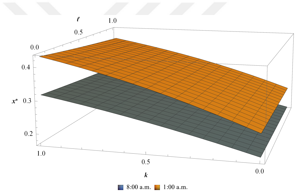
Figure 4.7: The optimal commitment value x^* for a peak (1 a.m.) and off-peak hour (8 a.m.) with respect to penalty parameters k and l
