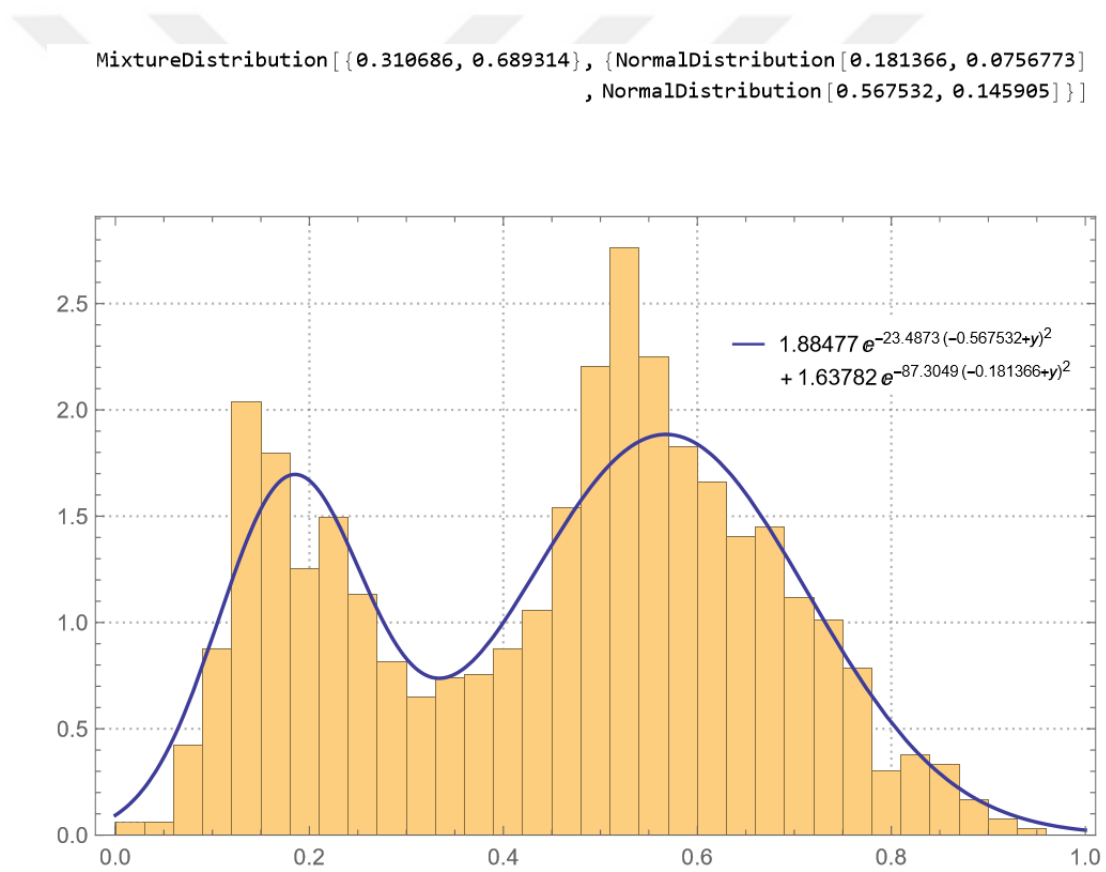
Figure B.5: The histogram and empirical distribution function of spring season
