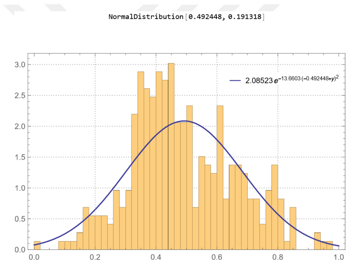
Figure 4.4: The histogram and empirical distribution function of 1 a.m.
