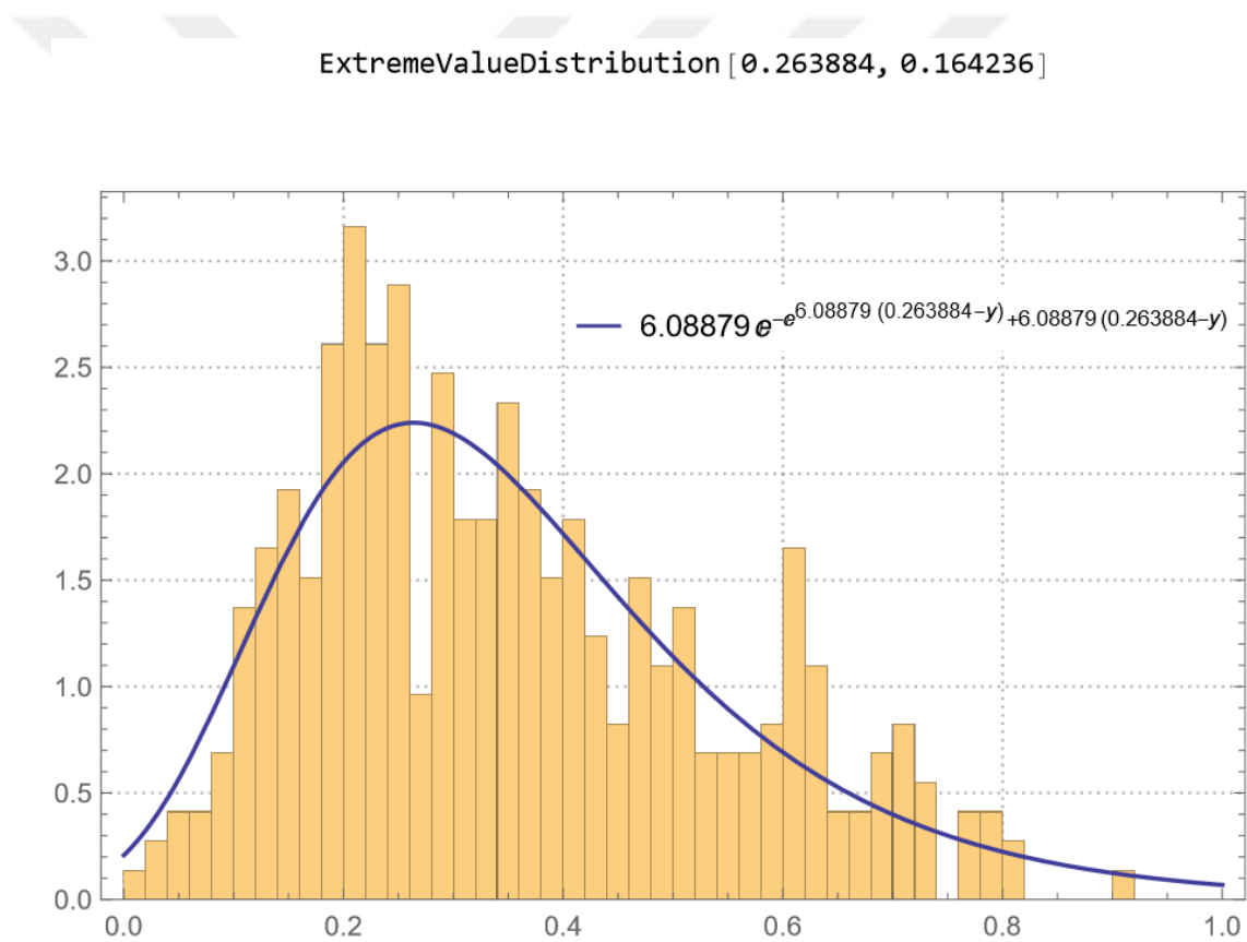
Figure 4.5: The histogram and empirical distribution function of 8 a.m.
