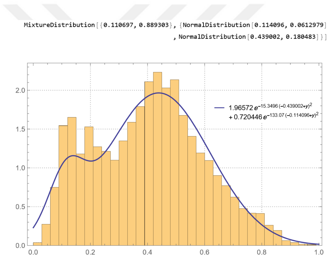
Figure B.1: The histogram and empirical distribution function of weekday
