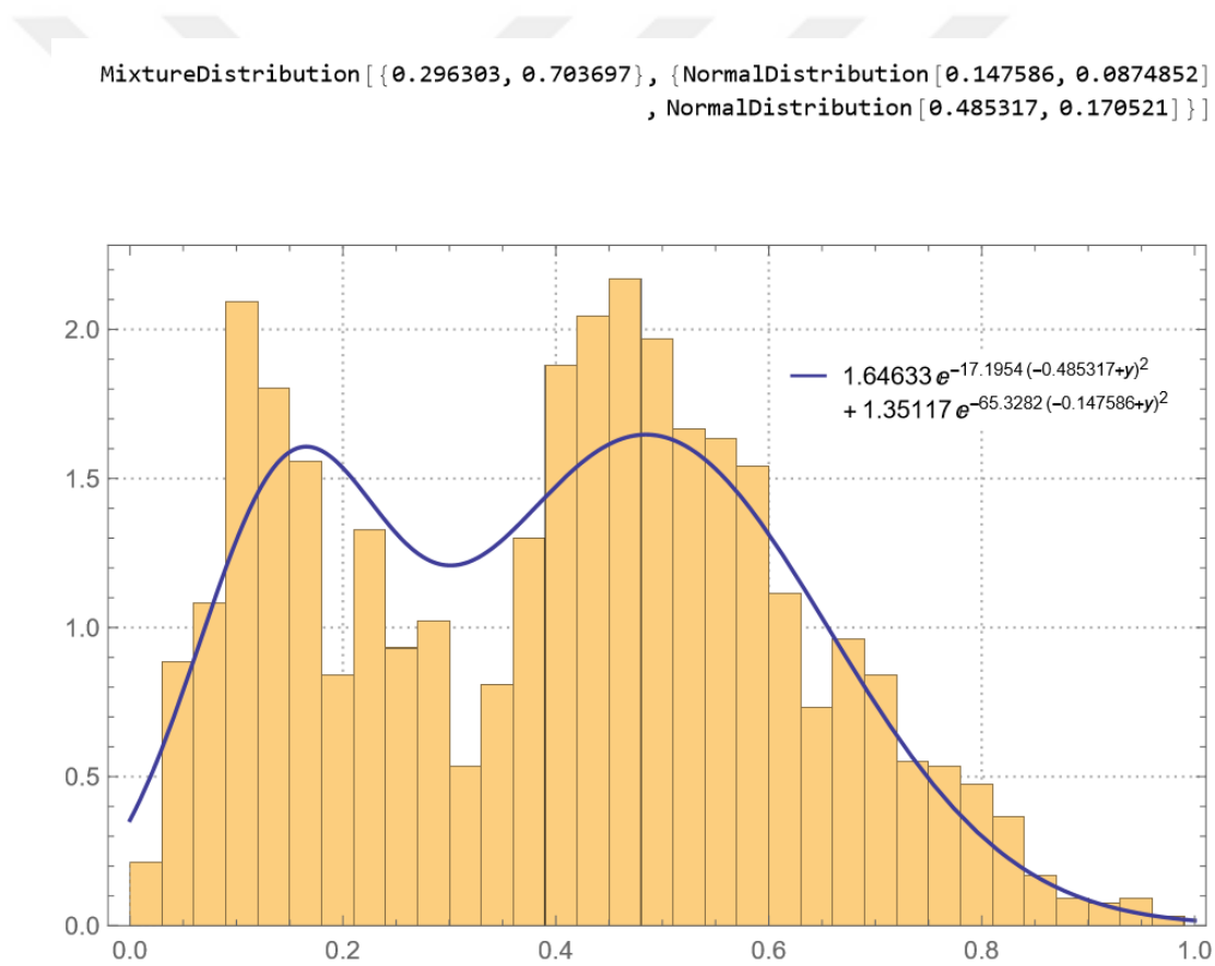
Figure B.6: The histogram and empirical distribution function of fall season
