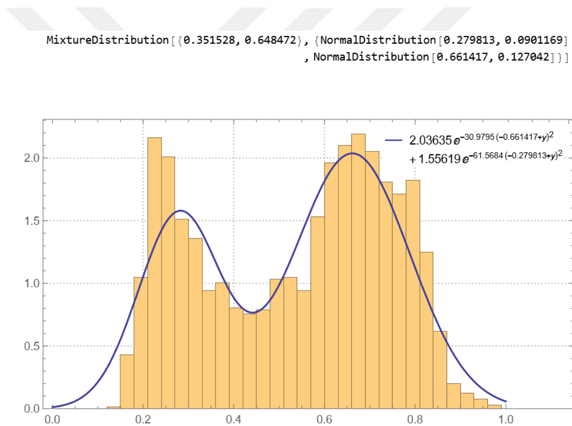
Figure B.4: The histogram and empirical distribution function of winter season
