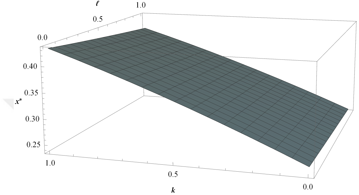
Figure 3.1: The change in optimal commitment value with respect to penalty parameters k and l , where Y \sim U(0, 1) .
