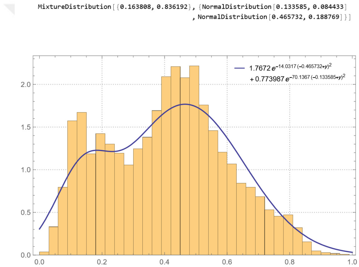
Figure B.7: The histogram and empirical distribution function of Baskent distribution region
