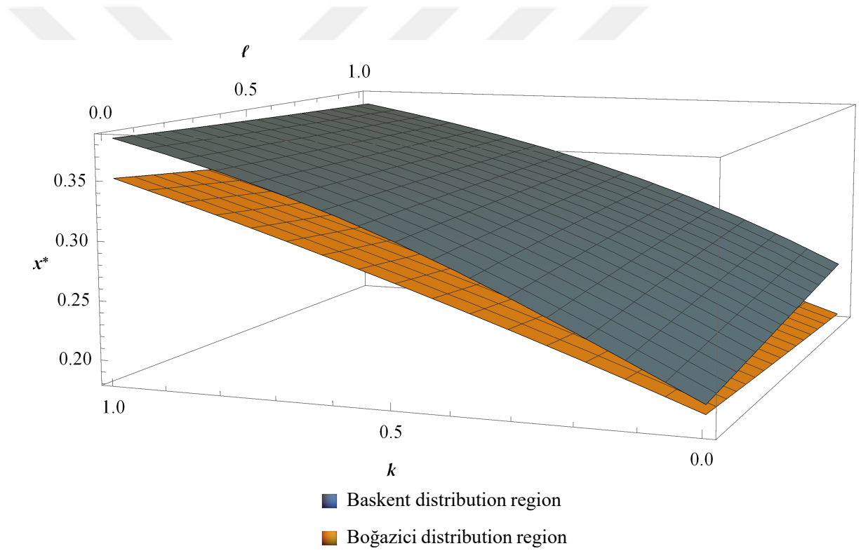
Figure 4.10: The optimal commitment value x^* for Central Anatolia Region and Marmara Region.
