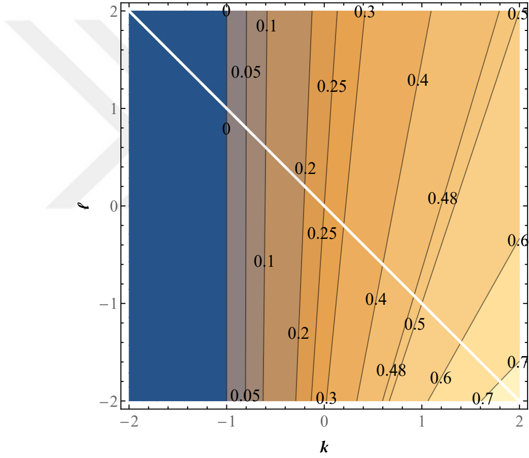
Figure 3.3: k and l combinations for different optimal commitment values where k, l \in [-2, 2] and Y \sim U(0, 1)
