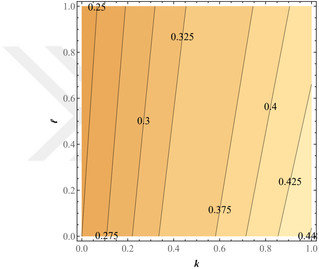
Figure 3.2: k and l combinations for different optimal commitment values where k, l \in [0, 1] and Y \sim U(0, 1)
