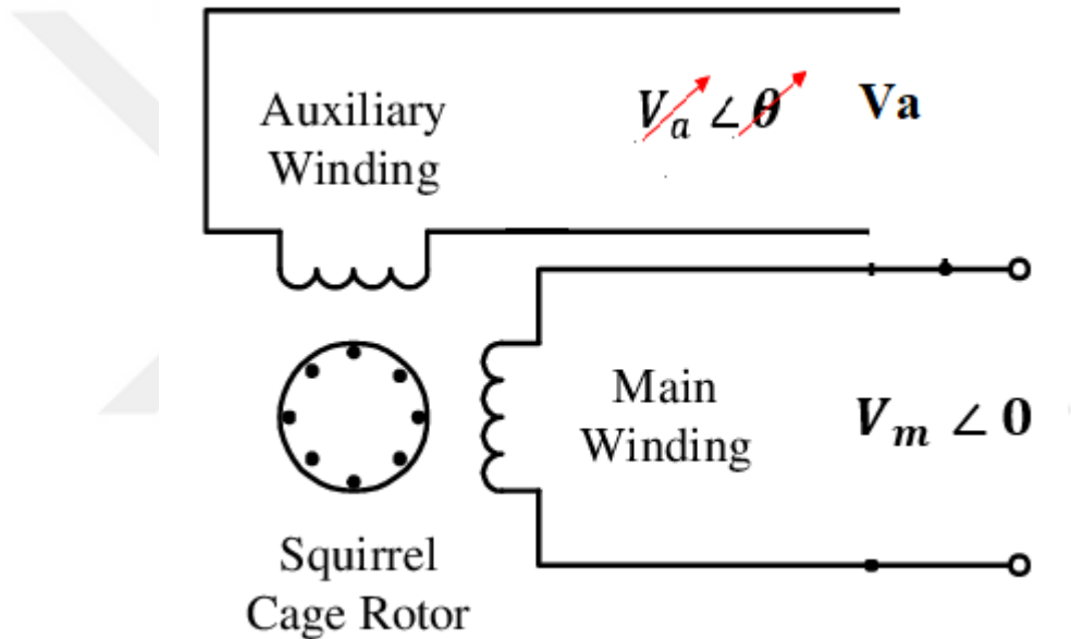
Figure 4.1. Schematic diagram of single-phase induction motor powered by two different voltage sources
