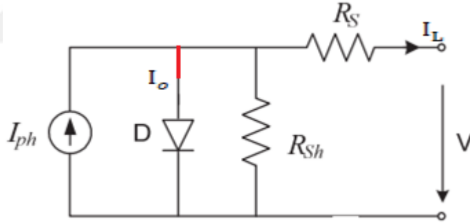
Figure 3.3. Photovoltaic equivalent circuit
