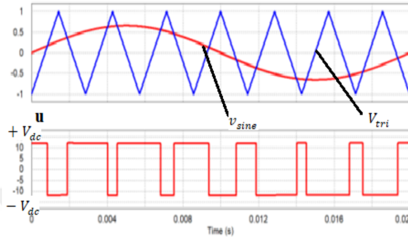
Figure 3.6. PWM signal with sine wave reference and triangle wave carrier
