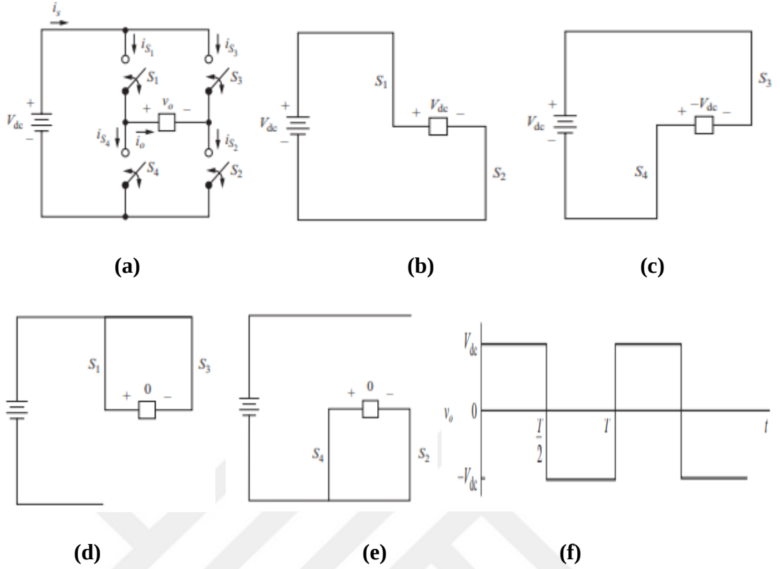
Figure 3.5. a) Full-bridge inverter; b) S_1 and S_2 closed; c) S_3 and S_4 closed; d) S_1 and S_3 closed; e) S_2 and S_4 closed; f) Output voltage of full bridge inverter
