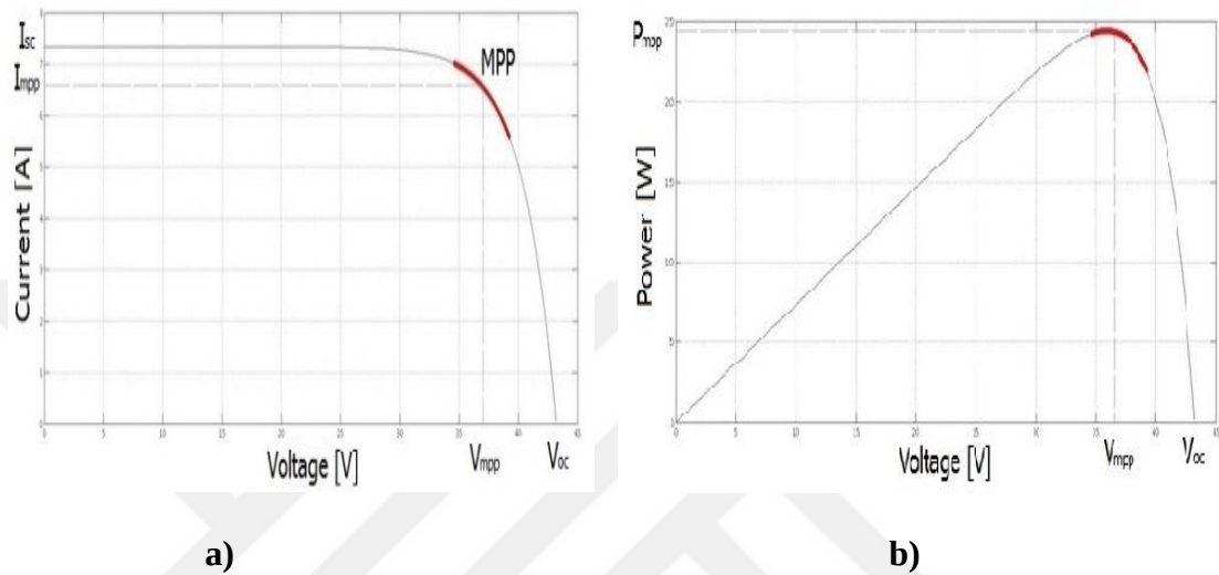
Figure 3.4. a) I-V characteristics curve; b) P-V characteristics curve
