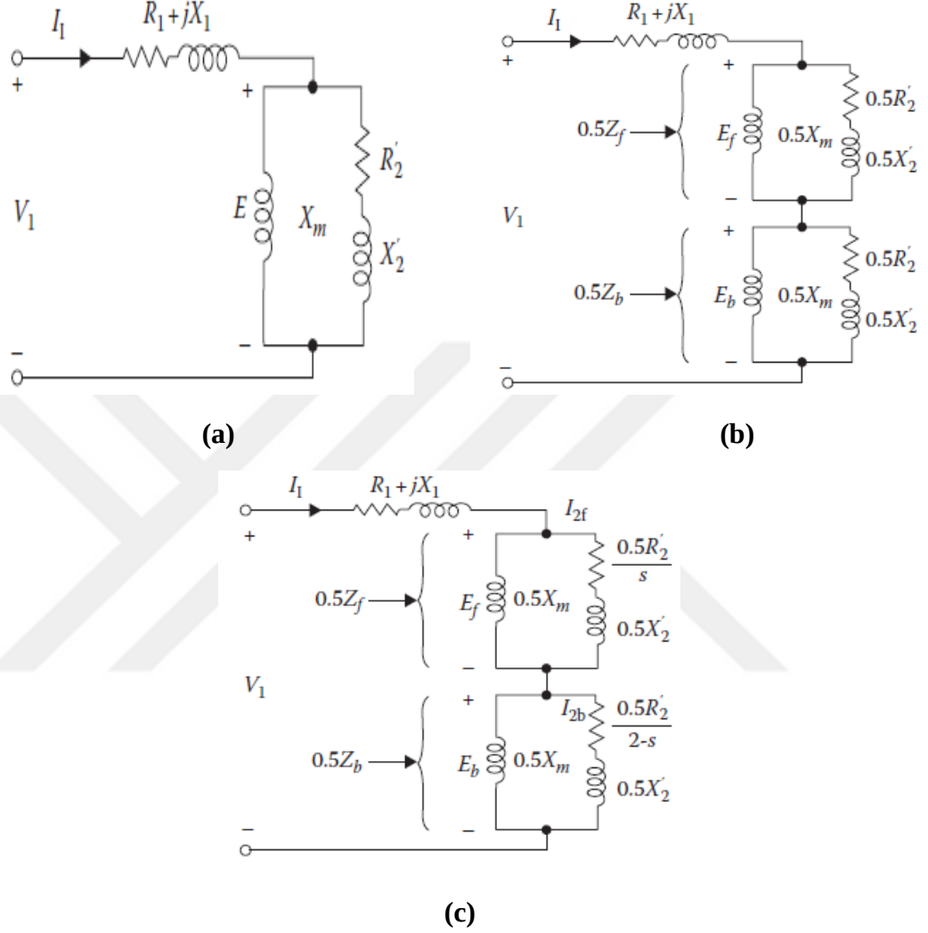
Figure 3.11. a) Equivalent circuit of SPIM; b) Configuration at standstill; c) Modified configuration at standstill
