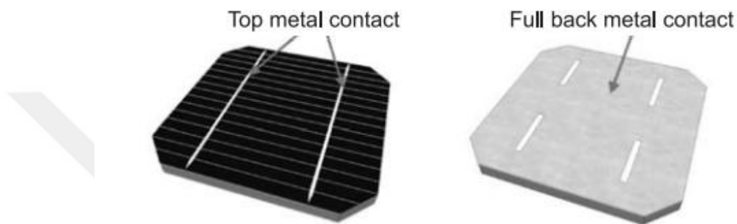
Figure 3.1. Front side and back side of a silicon solar cell
