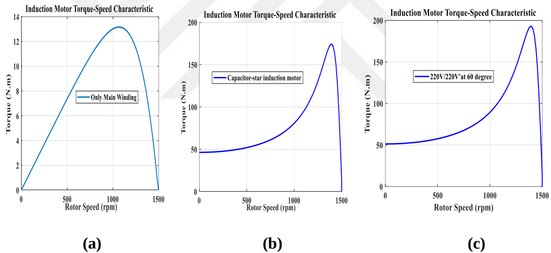
Figure 5.1. Torque speed characteristics of SPIM; a) SPIM with only main winding; b) Capacitor-star SPIM; c) SPIM with two voltage sources
