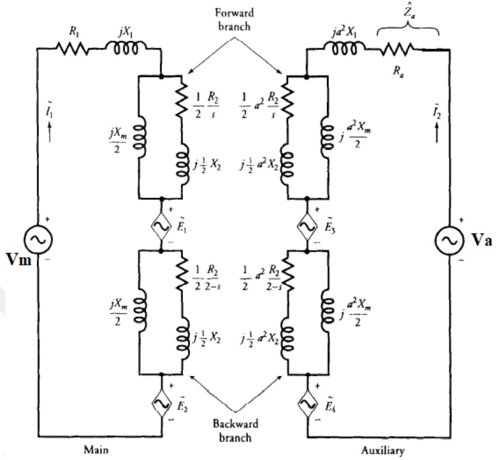
Figure 4.2. Equivalent circuit of the main winding and auxiliary windings of a single-phase induction motor
