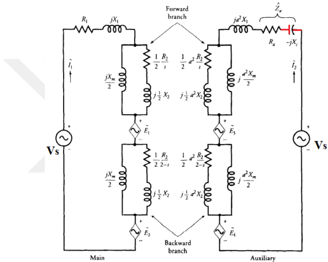
Figure 3.13. Equivalent circuit of the main winding and auxiliary windings of a capacitor-start induction motor
