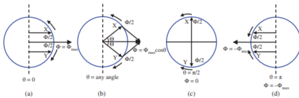
Figure 3.9. The flux that was produced in relation to the angle
