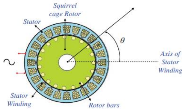
Figure 3.8. Cross-sectional view of a single-phase induction motor
