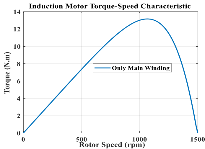
Figure 3.12. Torque-speed characteristic only main winding SPIM
