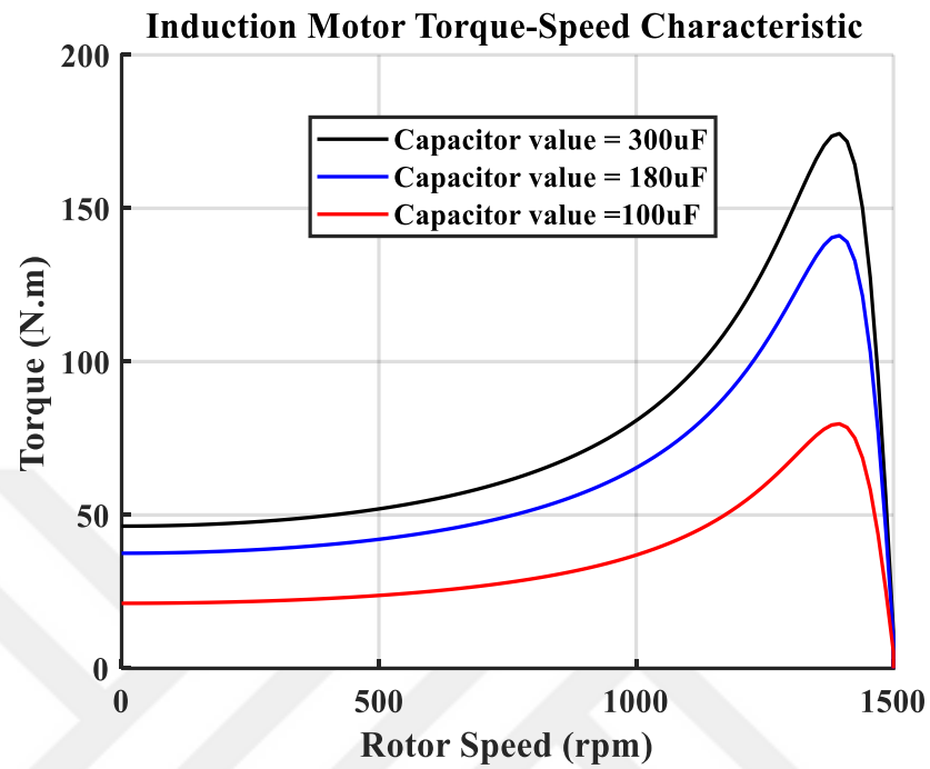
Figure 3.14. A Capacitor-start induction motor's torque-speed characteristic
