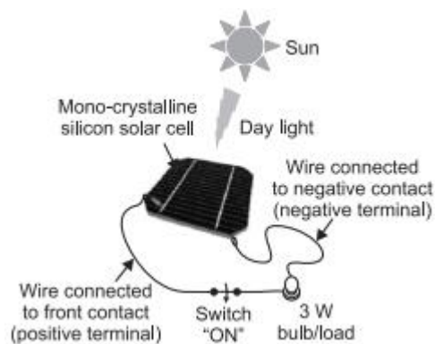
Figure 3.2. Solar cell with terminals and load
