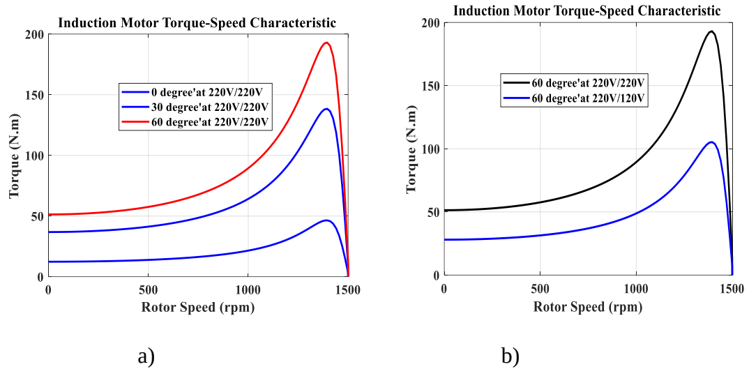
Figure 5.2. Torque speed characteristics of SPIM a) By controlling the phase angle; b) By controlling the voltage supply for the auxiliary winding
