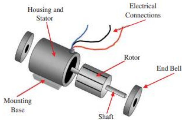
Figure 3.7. Construction of the single-phase induction motor.
