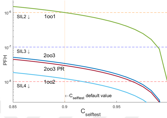
Figure 2.14: Effect of C_{selftest} variation over safety.
