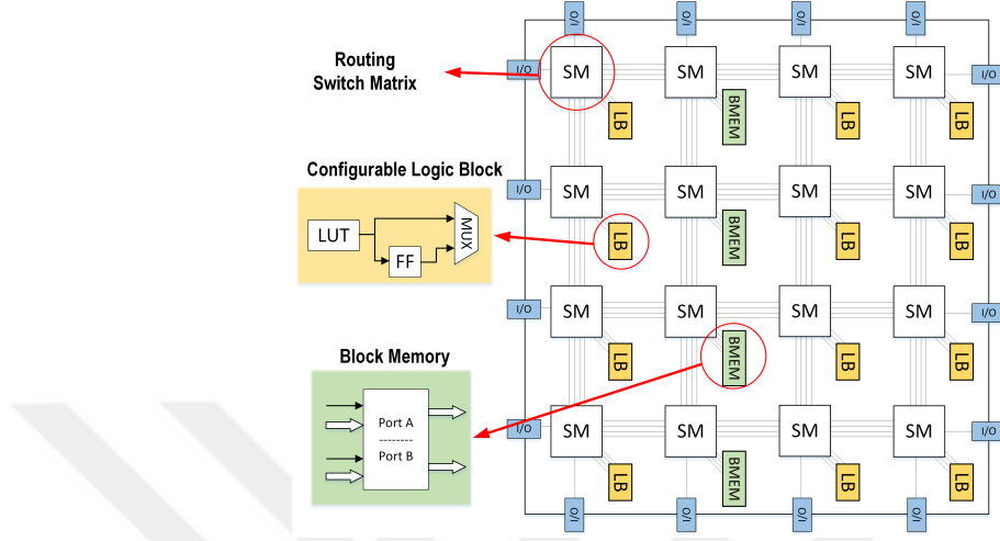
Figure 4.1: Distribution of logic blocks, on-chip memory blocks, routing switch matrices, and I/O blocks inside a generic FPGA architecture.
