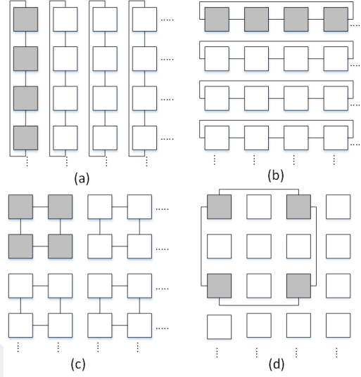
Figure 4.4: Variants of JSRAM layout.
