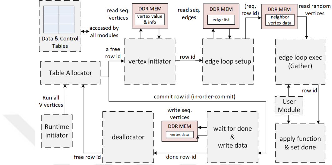
Figure 3.4: Simplified diagram of one high-throughput deeply pipelined vertex processing accelerator.
