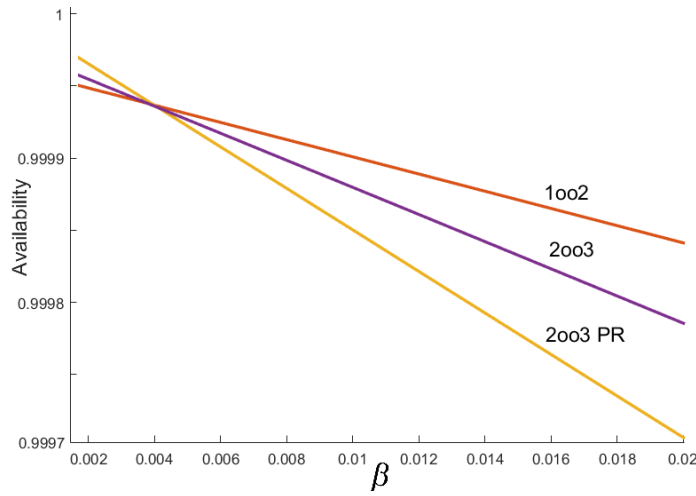
Figure 2.10: Steady state operational availability value for base systems with \beta variation (1oo1 is not shown).
