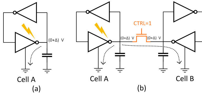
Figure 4.7: a) Hitting particle charges node capacitor and then, node voltage rises. b) Node capacitor and discharging path of cell B is added to cell A to discharge faster.
