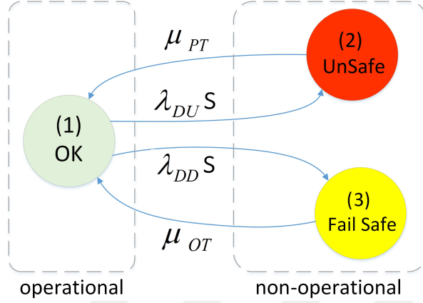
Figure 2.6: Markov model for 1oo1 (single) system.
