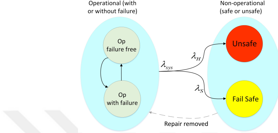
Figure 2.5: Unsafe (hazardous) and safe failure rate.
