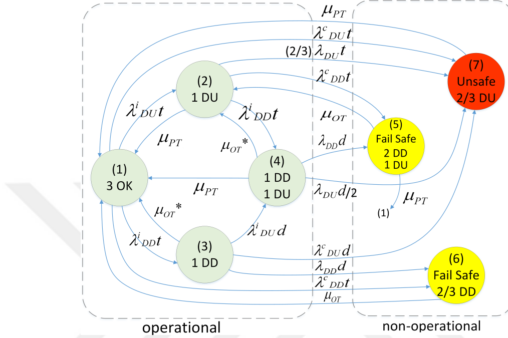
Figure 2.8: Markov model for 2oo3 system.
