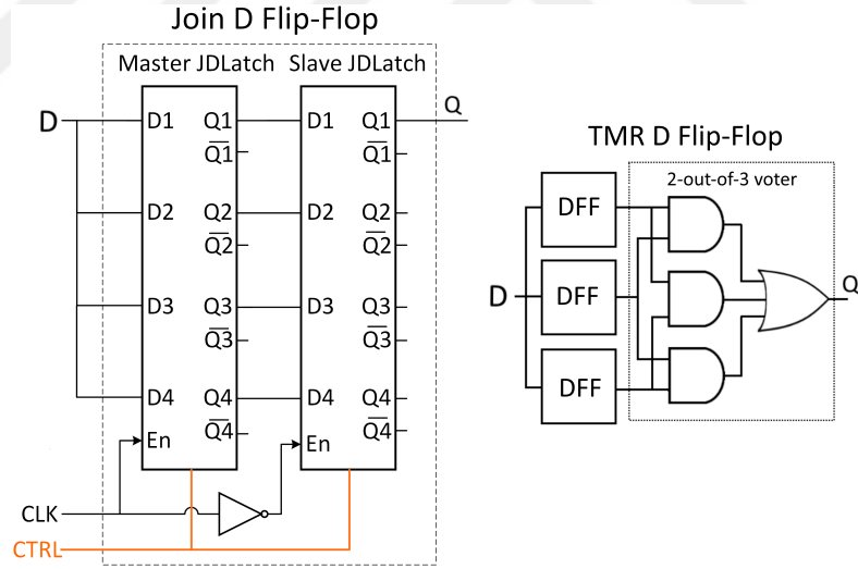
Figure 4.12: JDFF (Joint D Flip-Flop) is built from two JDLatches (Joint D Latches) on the left. This structure provides four separate normal DFF or a single radiation hardened DFF. Conventional TMR technique on the right.
