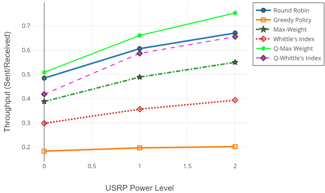
Figure 3.13: Fourth Experiment Set-Evaluation of Throughput with varying Input Gain of Second Receiver (SDR Testbed)
