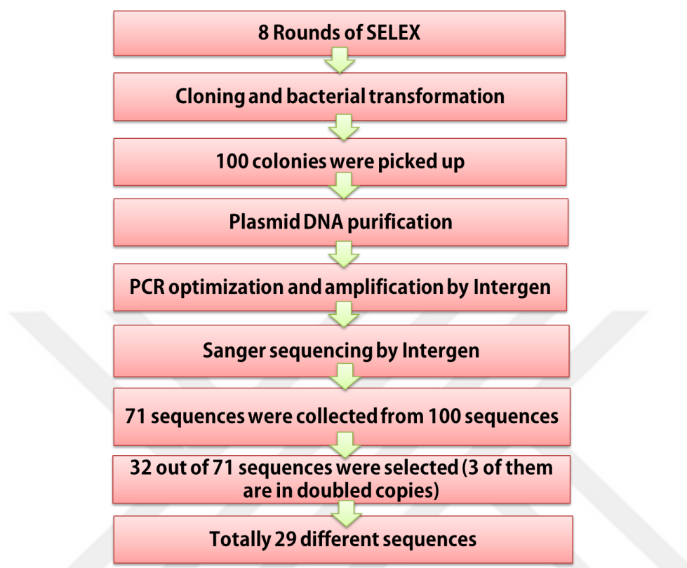
Figure 3.4. Post-SELEX methods and procedures.
