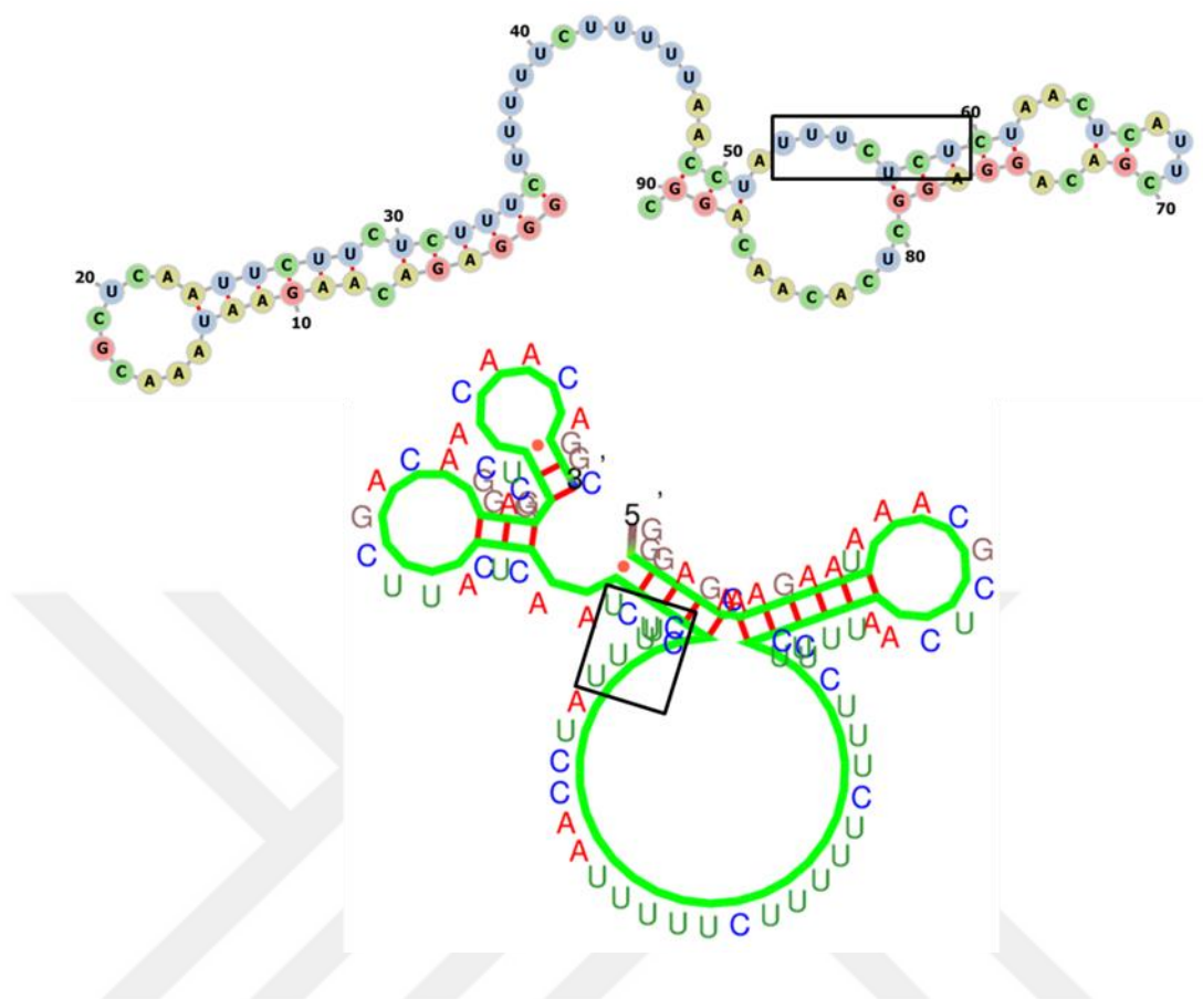
Figure 3.11. CadB85 structure. Above is RNAfold and below is KineFold.
