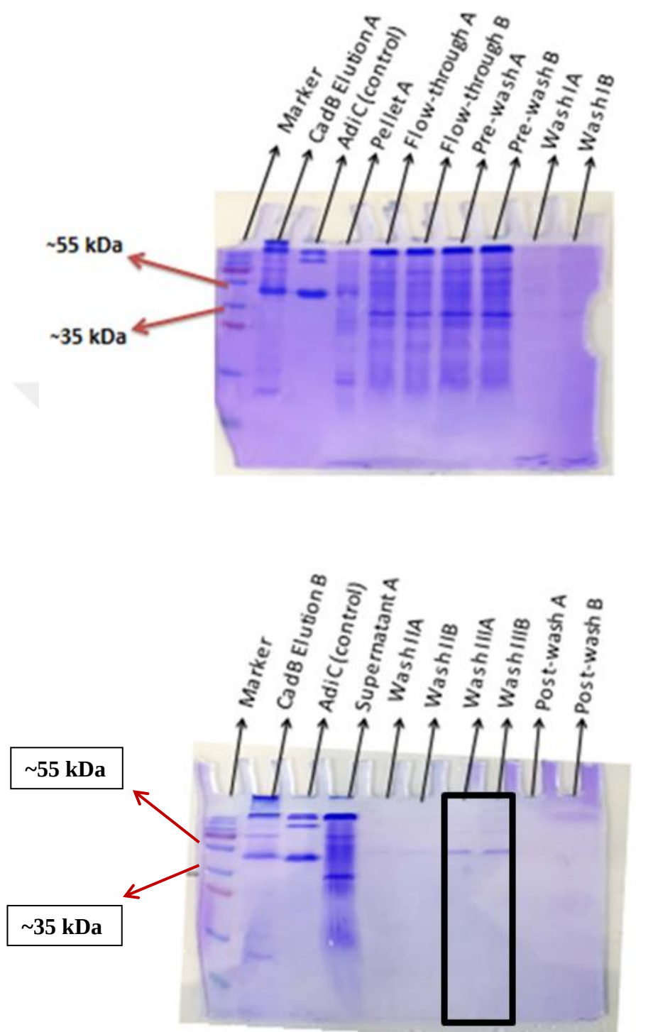
Figure 3.1. SDS-PAGE gel bands for CadB purification.
