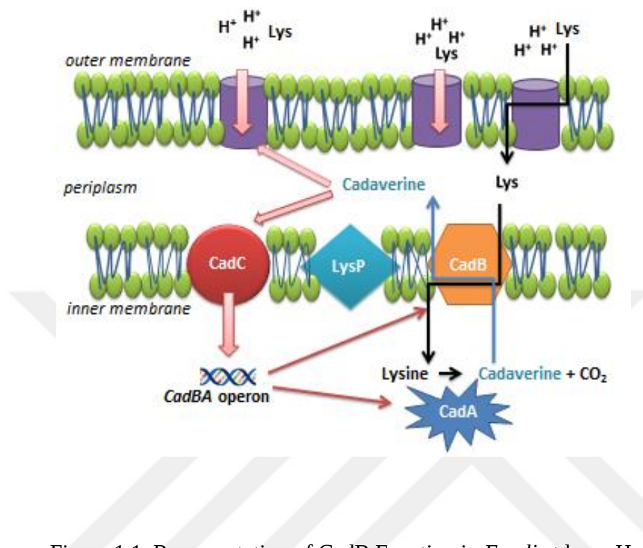
Figure 1.1. Representation of CadB Function in E.coli at low pH.
