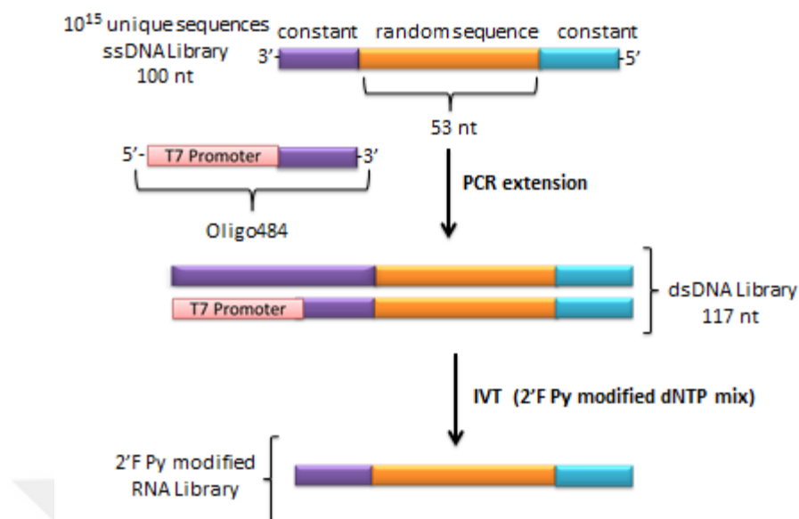
Figure 2.1. The schematic diagram of the RNA synthesis from the ssDNA pool.
