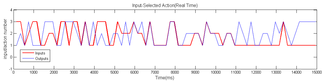
Figure 4.7: The selected actions (blue line) and the sensory inputs (red line) of the second experiment. The first input is red color, the second is yellow color and the third is blue color. The sensory stimuli are presented in random order.
