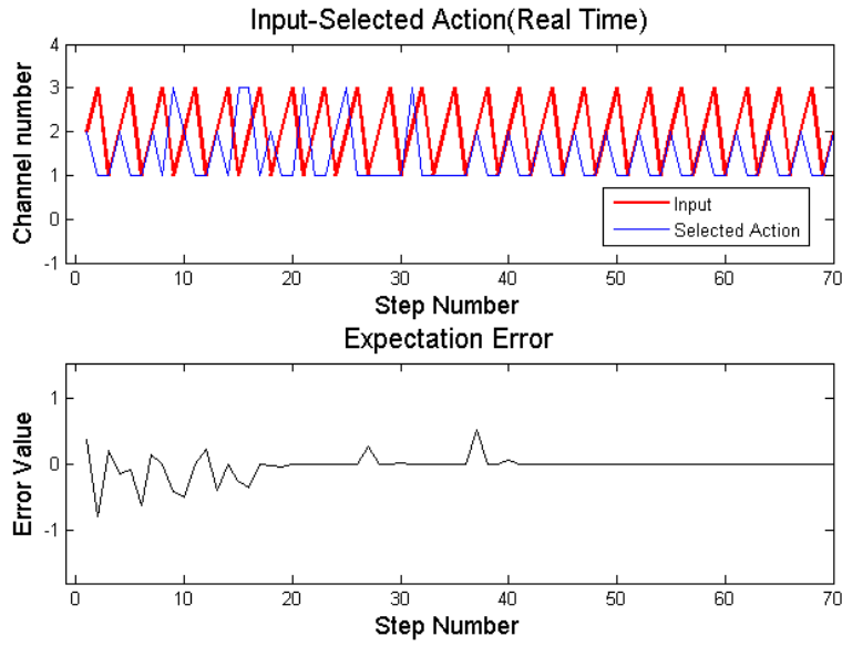
Figure 3.6: Zombie situation ( S_{max} = 1 ). The learning experiment is realized with random initial W_c and W_{rbase} is 0. The model sticks between two actions at the end of learning experiment and cannot select the third one. The expectation error is low through experiment and close to zero at the end despite it doesn't get reward.
