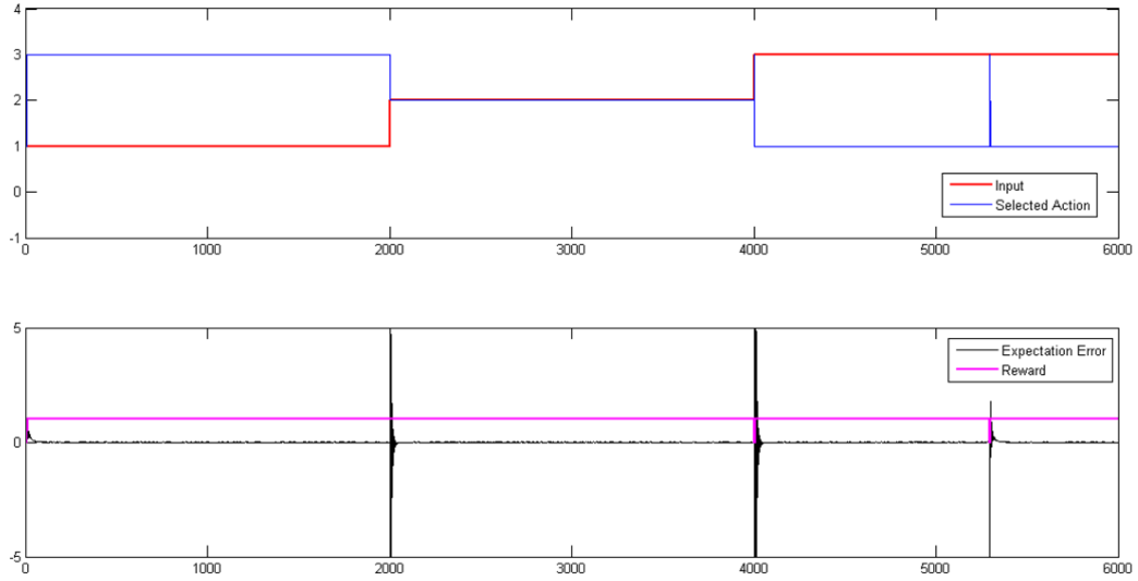
Figure 3.10: Results of rearranging the previously associated stimulus-action pairs in MATLAB environment. The upper sketch shows the relation between the inputs and actions and the lower one shows the expectation error and reward. 1 in the upper figure indicates the first stimulus or action, 2 indicates the second stimulus or action and 3 indicates the third stimulus or action with the related line colors.
