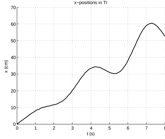
Figure 3.18: x values which are taken by the needle tip in \aleph_r for the insertion under periodic motion.
