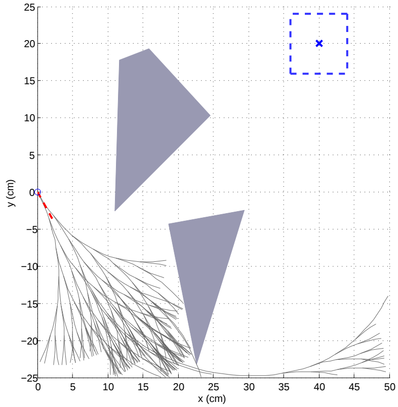
Figure 4.5: RRT generated in \aleph_c in n = 278 iterations with q_{init} = [0 \ 0 \ \frac{-\pi}{3}]^T . Entry position of the needle is shown with a blue dot and the initial angle with a red, dashed line segment. Target area is shown as a rectangular area with a cross at its center. Tree is blocked by the obstacles and the workspace boundary before it reaches the target area.
