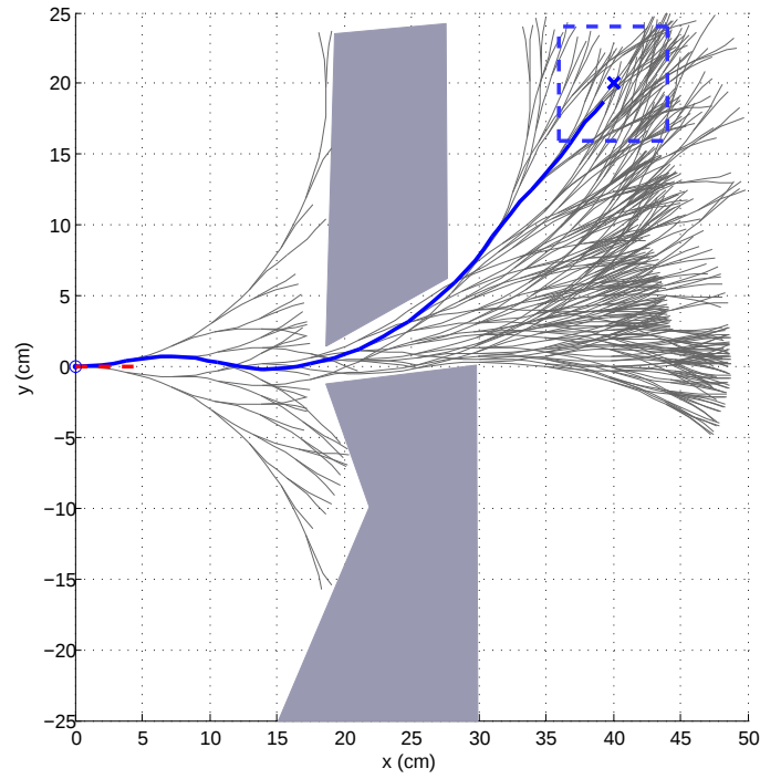
Figure 4.6: RRT generated in \mathfrak{N}_c in n = 500 iterations with q_{init} = [0 \ 0 \ 0]^T . Entry position of the needle is shown with a blue dot and the initial angle with a red, dashed line segment. Target area is shown as a rectangular area with a cross at its center. The path in the tree drawn in blue is the shortest feasible path found to drive the needle from q_{init} to the target.
