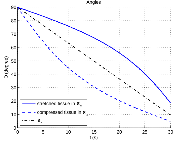
Figure 3.9: Angle of the needle tip throughout the insertion. We display the angle values for the needle in both of the representations, \aleph_c and \aleph_r , for an insertion into a stretched tissue as well as an insertion into a compressed one.
