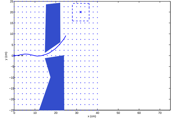
(d) t=36s . Tissue is at its most compressed state.
