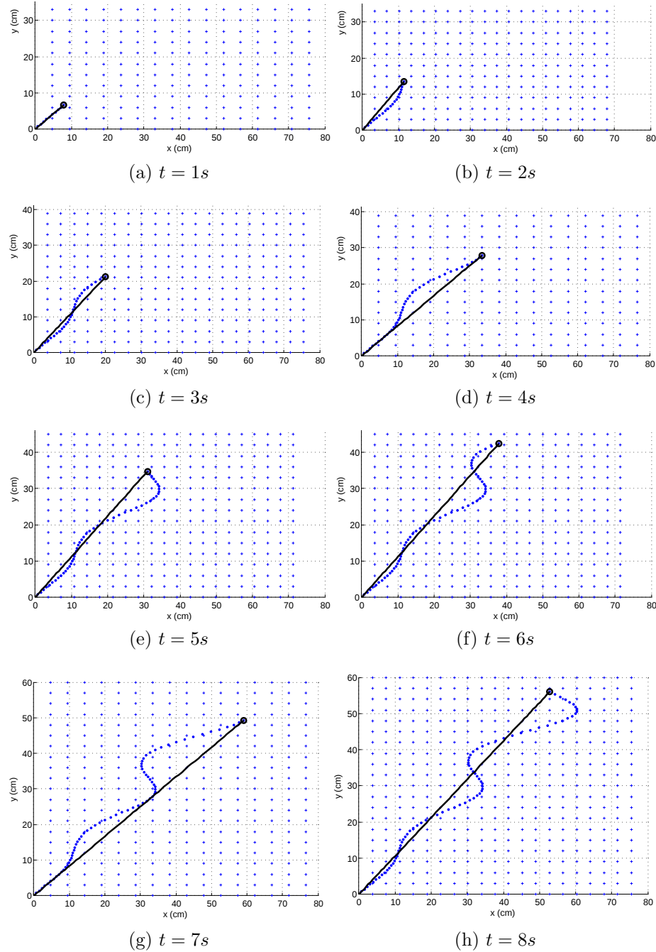
Figure 3.17: Snapshots taken in \mathbb{N}_r where the needle is inserted with 10 cm/s constant velocity for insertion under periodic motion. Tissue is denoted by blue crosses where the path followed by the tip is shown with blue dots and the needle as a solid line.
