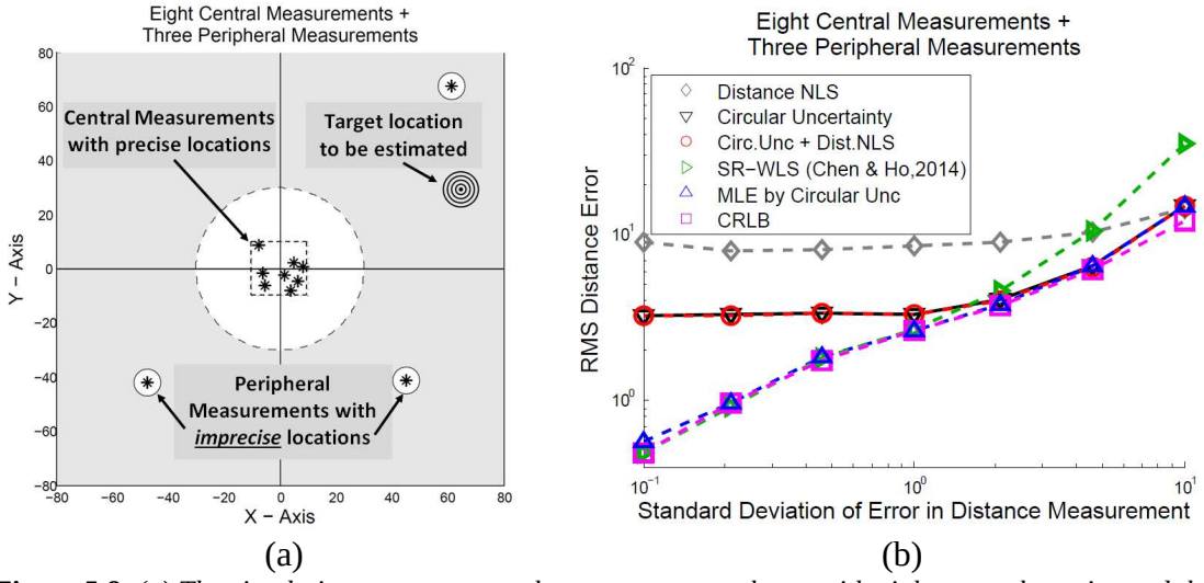
Figure 5.8. (a) The simulation setup - a sample measurement scheme with eight central precise and three peripheral imprecise measurements, (b) the RMS distance errors for various localization methods
