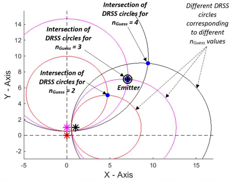
Figure 4.8. Intersection of DRSS circles for different n_{\text{Guess}} values
