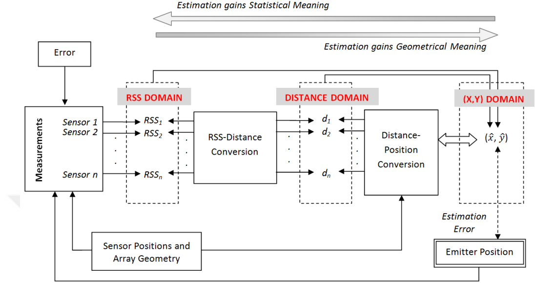
Figure 4.1. Flowchart of RSS based Localization
