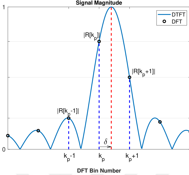
Figure 2.1: Magnitude DTFT and DFT magnitude spectrum of the complex sinusoidal signal with frequency \omega = \frac{2\pi(k_p + \delta)}{N} .
