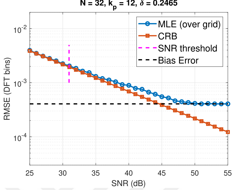
Figure 2.3: RMSE vs SNR plot for MLE with frequency \omega = \frac{2\pi(12+0.2465)}{32} .
