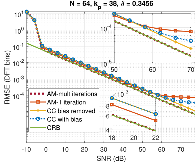
Figure 2.6: Comparison of different fine frequency estimation methods with frequency \omega = \frac{2\pi(38+0.3456)}{64} .
