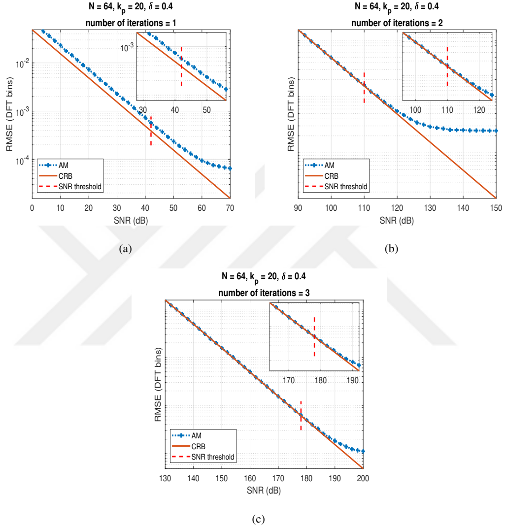
Figure 2.8: AM algorithm simulation results for different iterations where N = 64 and f = \frac{20+0.4}{64} : (a) 1 iteration, (b) 2 iterations, (c) 3 iterations.
