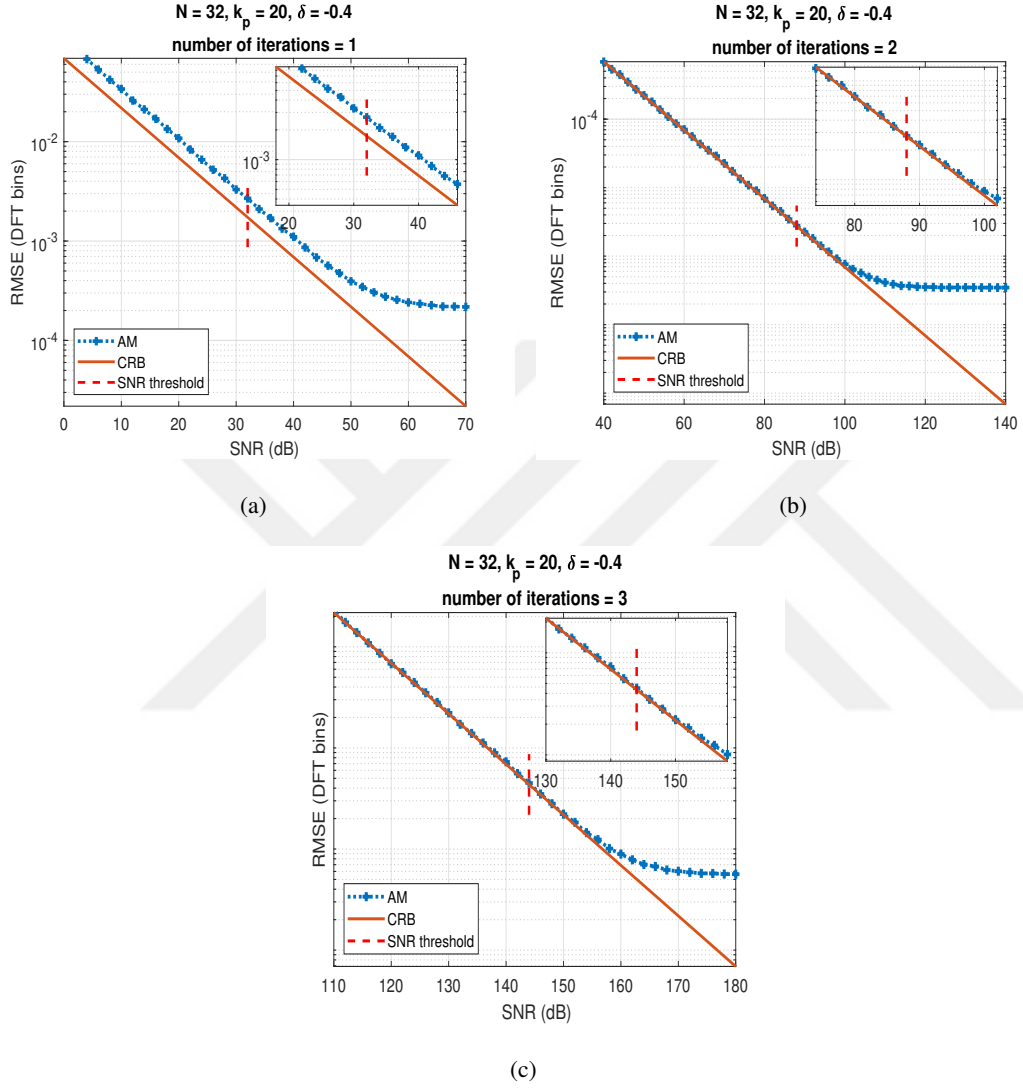
Figure 2.9: AM algorithm simulation results for different iterations where N = 32 and f = \frac{20-0.4}{32} : (a) 1 iteration, (b) 2 iterations, (c) 3 iterations.
