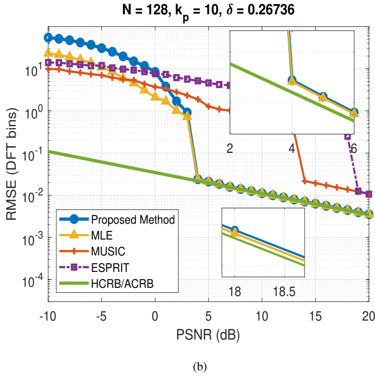
Figure 5.6: RMSE comparison of the proposed method with other methods where f_0 = \frac{10+0.26736}{128} , L = 4 and A_1 = 2A_2 = \frac{10}{3}A_3 = 10A_4 : (a) model order selection is made, (b) model order is given.
