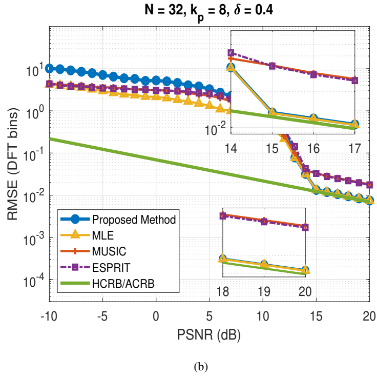
Figure 5.3: RMSE comparison of the proposed method with other methods where f_0 = \frac{8+0.4}{32} , L = 2 and A_1 = 5A_2 : (a) model order selection is made, (b) model order is given.
