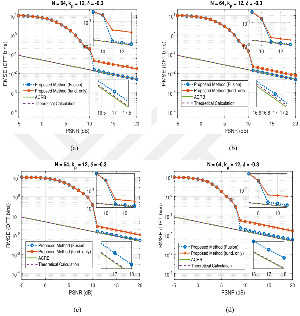
Figure 3.2: Performance of the Proposed Estimator: f_0 = \frac{12-0.3}{64} and L = 4 (a) A_1 = A_2 = A_4 and A_3 = 0 , (b) A_2 = A_3 and A_1 = A_4 = 0 , (c) A_2 = A_3 = A_4 and A_1 = 0 , (d) A_1 = A_3 = A_4 and A_2 = 0 .
