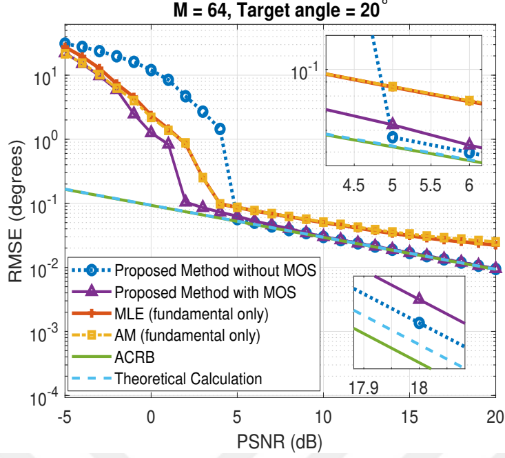
Figure 5.7: Performance comparison of proposed method with conventional methods where \omega^s = \pi \sin(20^\circ) = 2\pi \frac{10.9446}{64} , L = 3 and A_1 = 2A_2 = 4A_3 .
