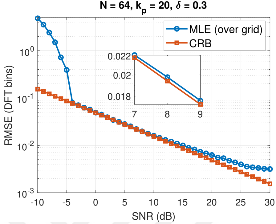
Figure 2.2: RMSE vs SNR plot for MLE with frequency \omega = \frac{2\pi(20+0.3)}{64} .
