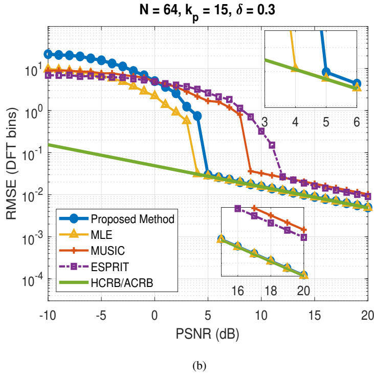
Figure 5.4: RMSE comparison of the proposed method with other methods where f_0 = \frac{15+0.3}{64} , L = 3 and A_1 = 2A_2 = \frac{10}{3}A_3 : (a) model order selection is made, (b) model order is given.
