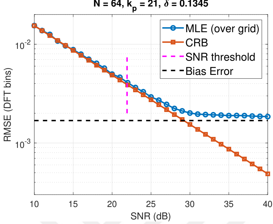
Figure 2.4: RMSE vs SNR plot for MLE with frequency \omega = \frac{2\pi(21+0.1345)}{64} .
