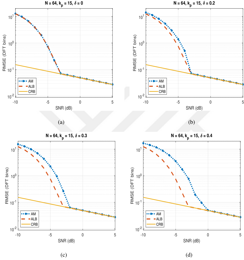
Figure 2.10: AM algorithm simulation results and approximate lower bound for different \delta values where N = 64 and k_p = 15 : (a) \delta = 0 , (b) \delta = 0.2 , (c) \delta = 0.3 , (d) \delta = 0.4 .
