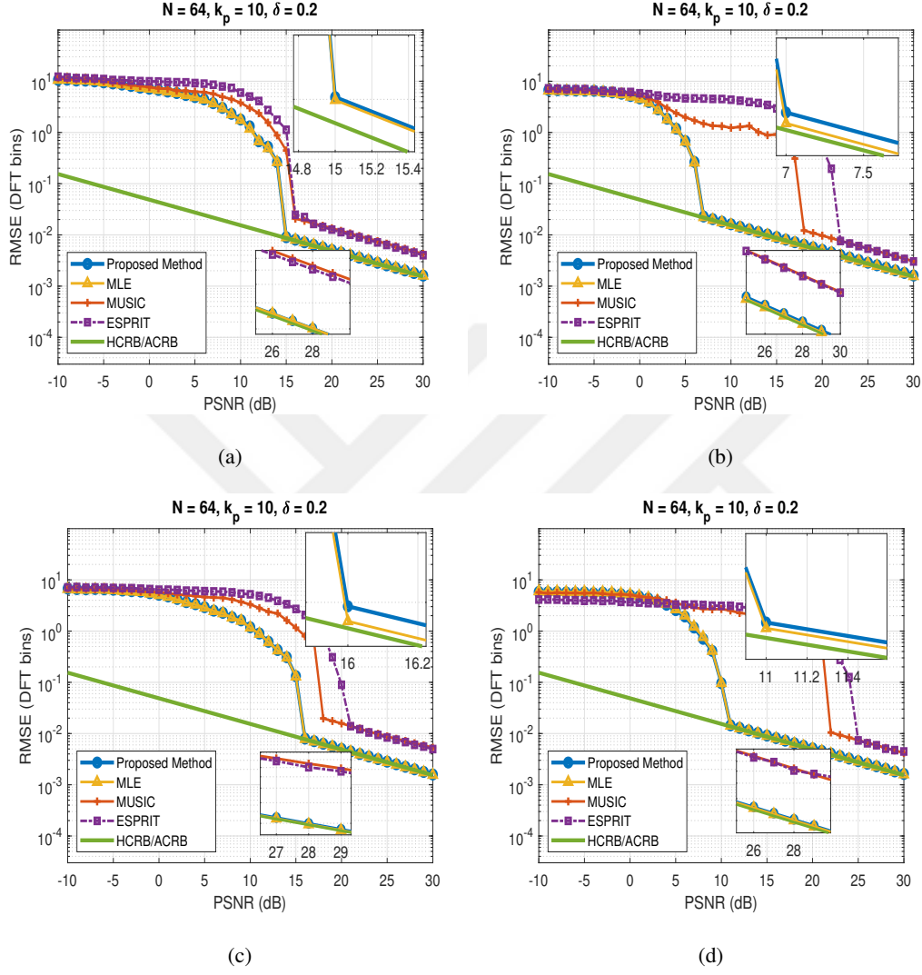
Figure 5.2: RMSE comparison of the proposed method with other methods where f_0 = \frac{10+0.2}{64} : (a) L = 2 and 5A_1 = A_2 , (b) L = 3 and 5A_1 = A_2 = A_3 , (c) L = 3 and 5A_1 = 5A_2 = A_3 , (d) L = 4 and 5A_1 = 5A_2 = A_3 = A_4 .
