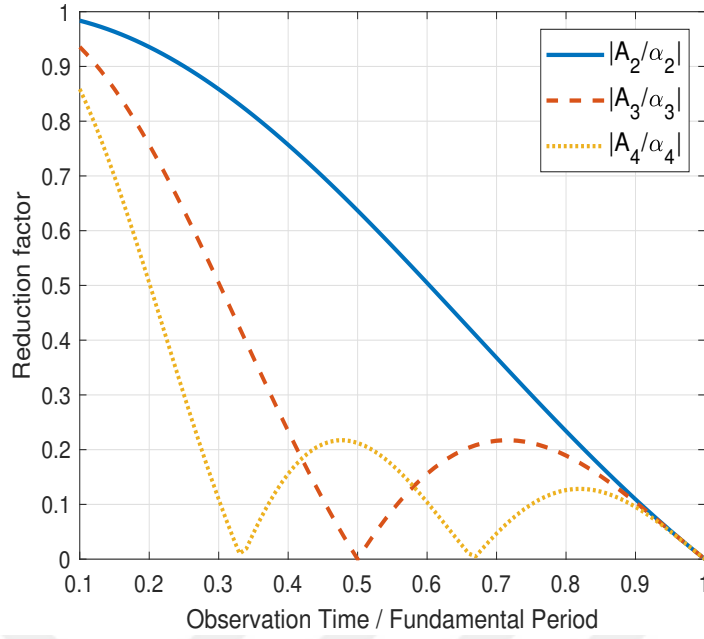
Figure 4.2: Reduction factor of second, third and fourth harmonics ( \omega_0 = 2\pi/200 ).
