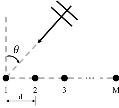
Figure 4.1: Uniform Linear Array Structure.
