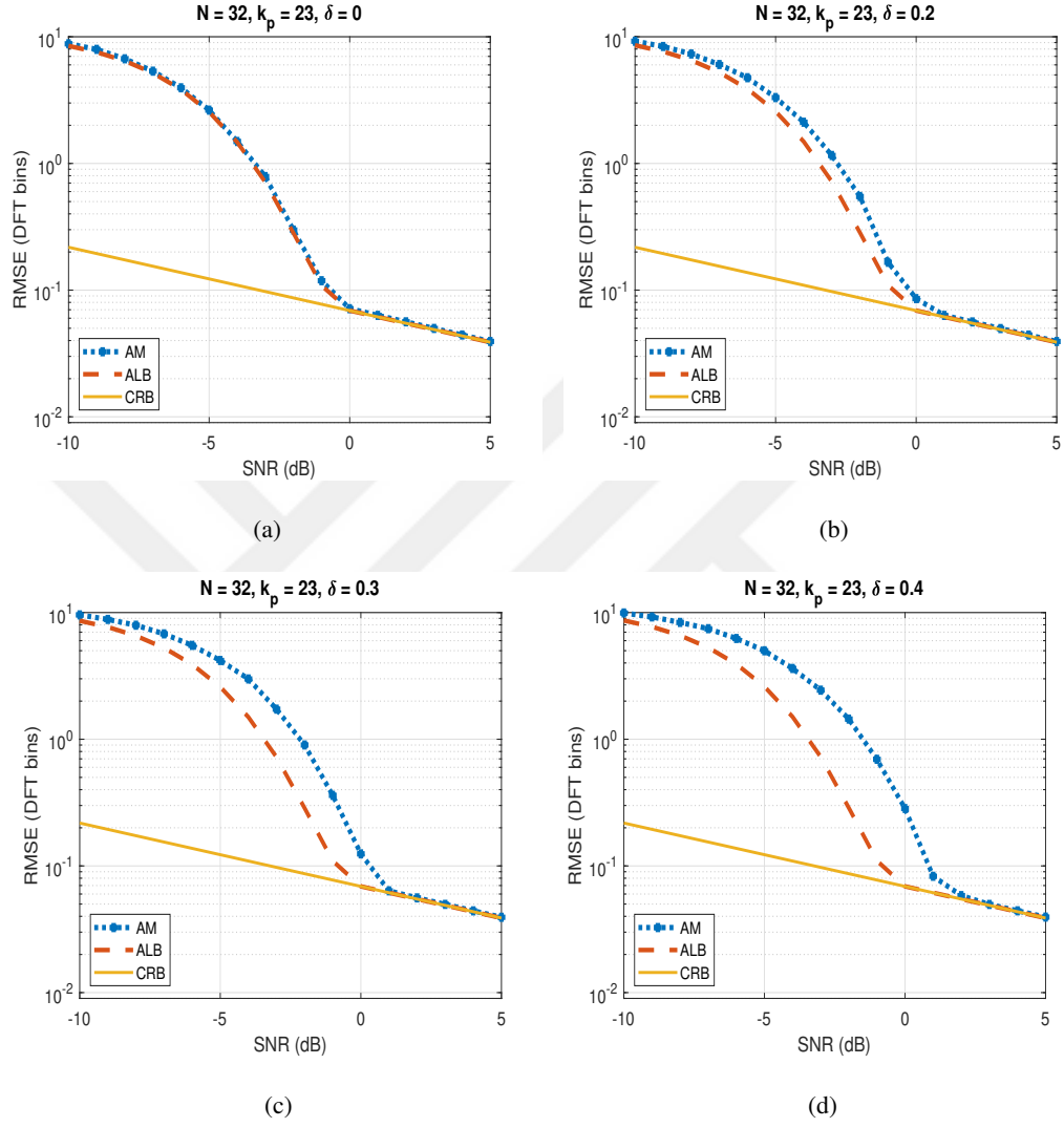
Figure 2.11: AM algorithm simulation results and approximate lower bound for different \delta values where N = 32 and k_p = 23 : (a) \delta = 0 , (b) \delta = 0.2 , (c) \delta = 0.3 , (d) \delta = 0.4 .
