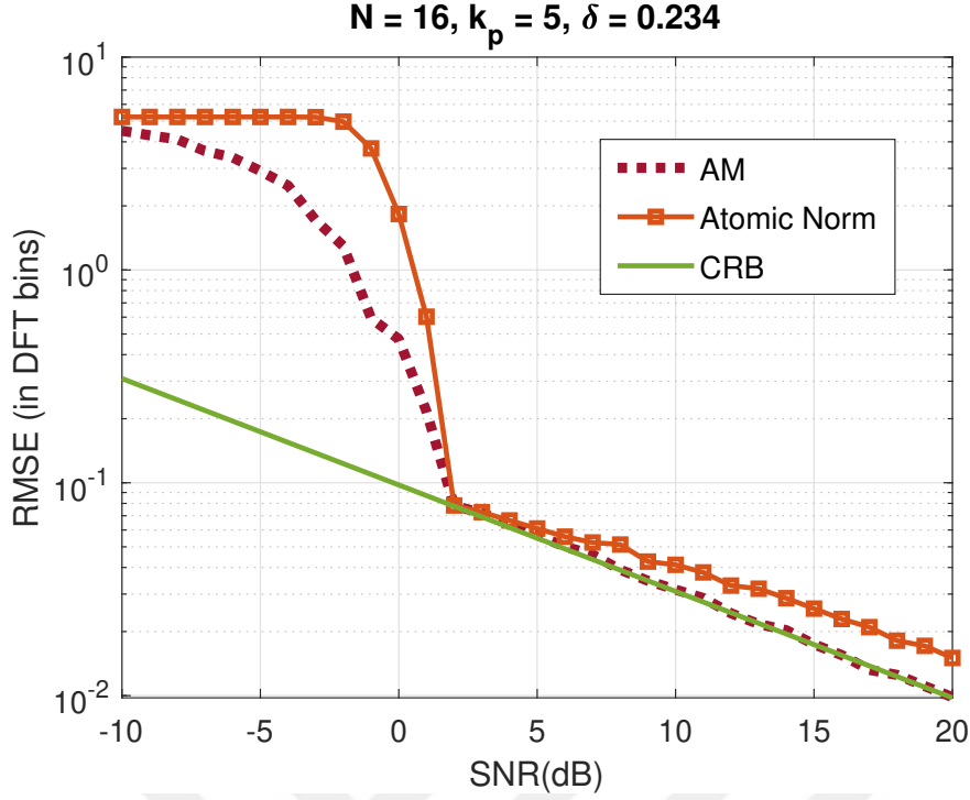
Figure B.1: RMSE and SNR plots for AM and ADMM with Prony's Method with frequency \omega = \frac{2\pi(5+0.2345)}{16} .
