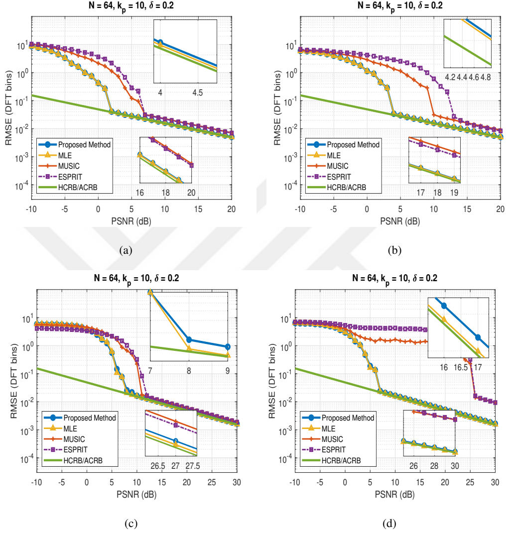
Figure 5.1: RMSE comparison of the proposed method with other methods where f_0 = \frac{10+0.2}{64} : (a) L = 2 and A_1 = 2A_2 , (b) L = 3 and A_1 = 2A_2 = 4A_3 , (c) L = 4 and A_1 = A_2 = A_3 = A_4 , (d) L = 3 and A_1 = 10A_2 = A_3 .
