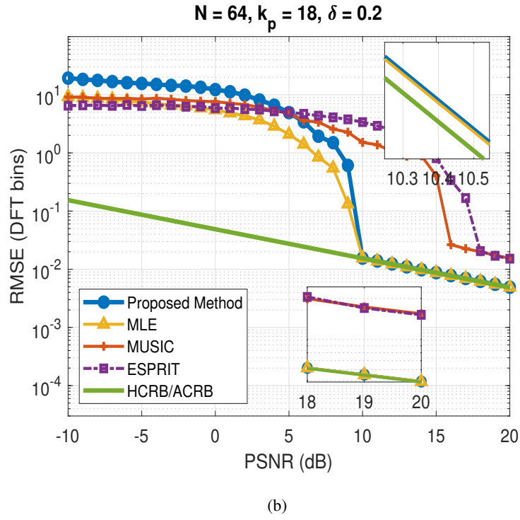
Figure 5.5: RMSE comparison of the proposed method with other methods where f_0 = \frac{18+0.2}{64} , L = 3 and A_1 = 5A_2 = 10A_3 : (a) model order selection is made, (b) model order is given.
