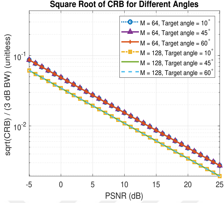
Figure 4.4: Square Root of CRB normalized to 3 dB beamwidth of ULA array for different target angles and total number of sensors ( d = \lambda/2 ).
