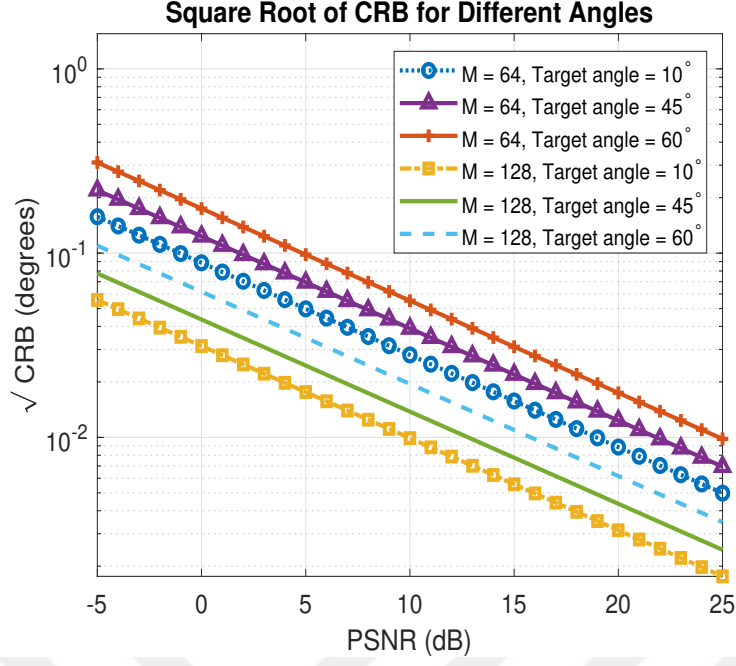
Figure 4.3: Square root of CRB for different target angles and total number of sensors ( d = \lambda/2 ).
