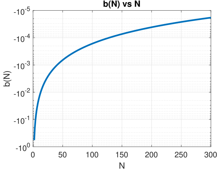
Figure 2.7: g'(\delta) = b(N) vs N
