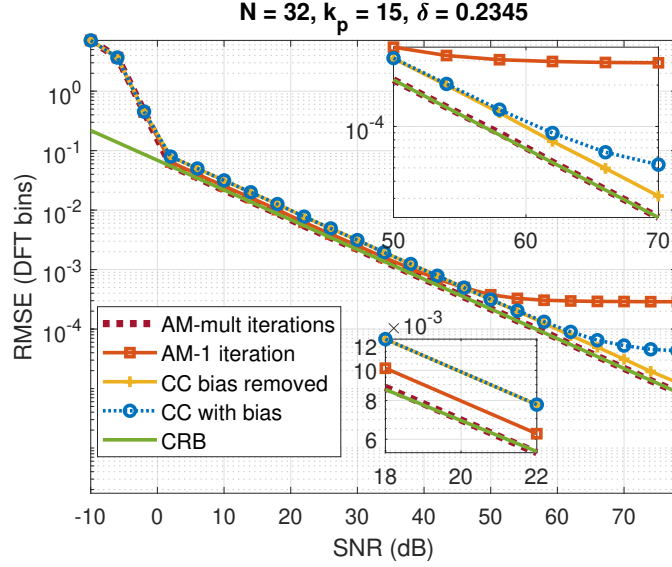
Figure 2.5: Comparison of different fine frequency estimation methods with frequency \omega = \frac{2\pi(15+0.2345)}{32} .
