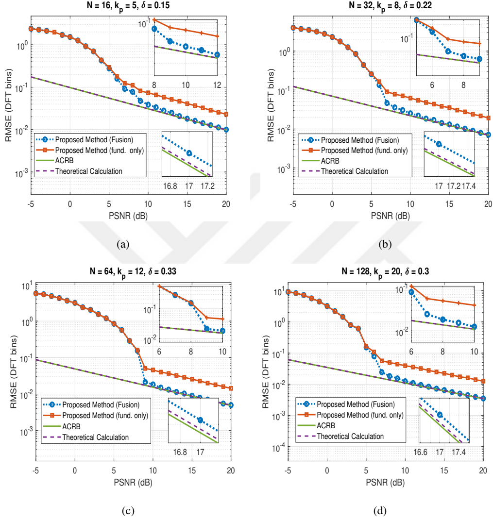
Figure 3.1: Performance of the Proposed Estimator: (a) f_0 = \frac{5+0.15}{16} , L = 2 and A_1 = A_2 , (b) f_0 = \frac{8+0.22}{32} , L = 3 and A_1 = A_2 = 2A_3 , (c) f_0 = \frac{12+0.33}{64} , L = 4 and A_1 = A_2 = 2A_3 = 4A_4 , (d) f_0 = \frac{20+0.3}{128} , L = 5 and A_1 = A_2 = 2A_3 = 2A_4 = 4A_5 .
