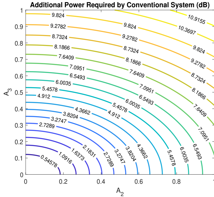
Figure 4.5: Additional power in dB required by the conventional DOA system ( A_1 = 1, A_2 = A_3 = 0 ) to operate at the CRB of the system utilizing three harmonics ( A_1 = 1, A_2 \in [0, 1], A_3 \in [0, 1] )
