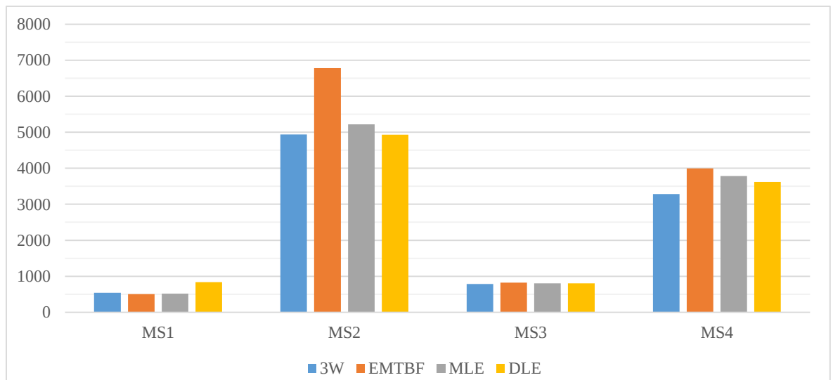
Figure 38 Average MSE Scores
