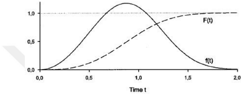
Figure 7 CDF F(t) and PDF f(t) versus Time [43]
