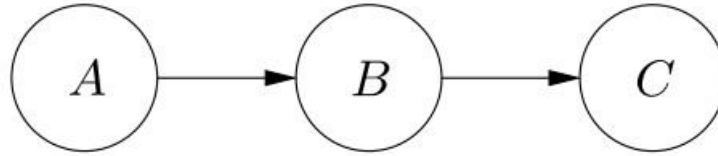
Figure 3 Serial Connection in BNs [21]
