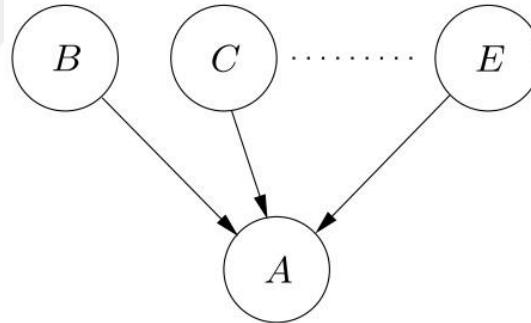
Figure 5 Converging Connection in BNs [21]
