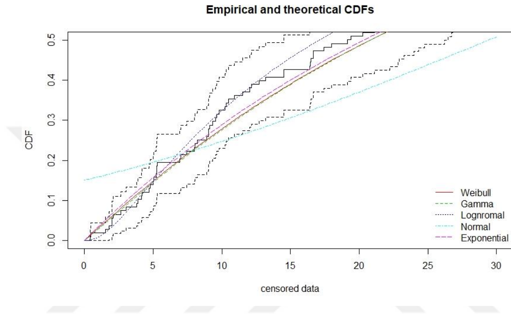
Figure 23 MS3 MLE Distributions Plot-1
