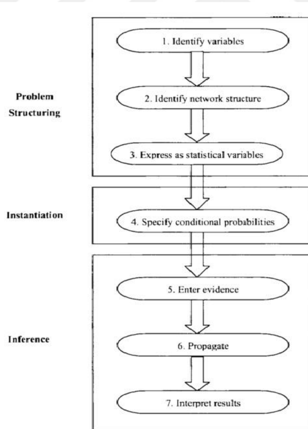
Figure 6 Flowchart of Stages for Building and Using a BN Model [36].
