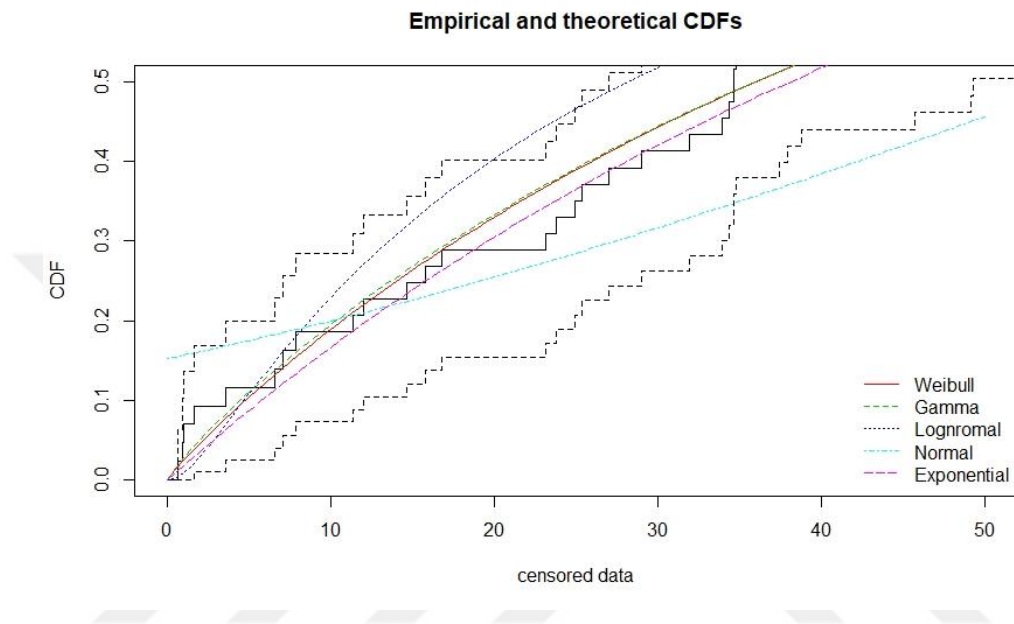
Figure 26 MS4 MLE Distributions Plot-1
