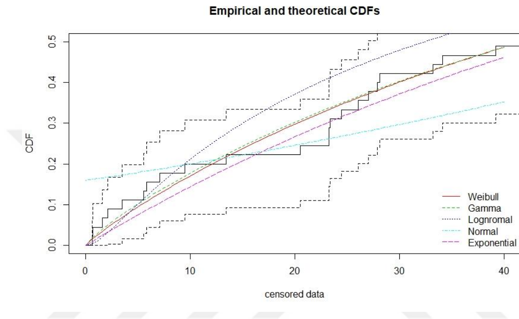
Figure 20 MS2 MLE Distributions Plot-1
