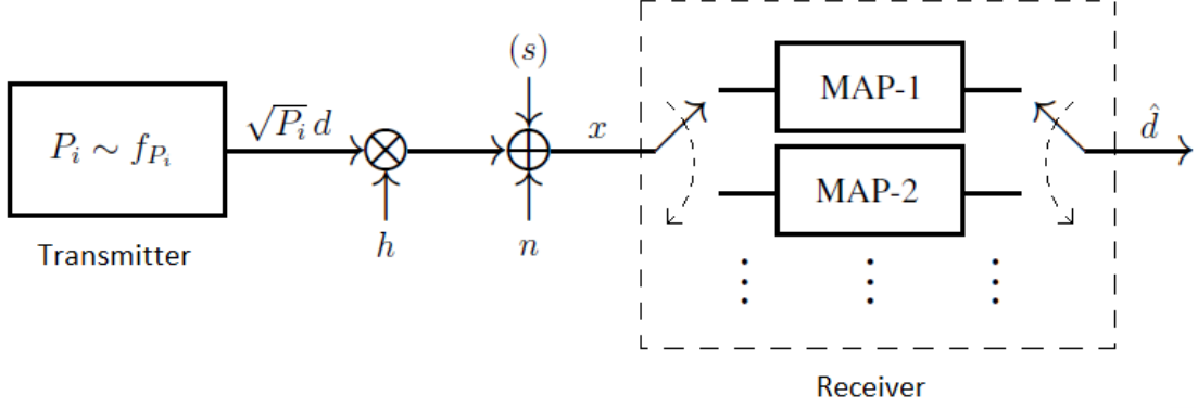
Figure 2.1: Basedband model of the communications system for the secondary users. The secondary transmitter generates a signal, the power P_i of which is determined according to the PDF f_{P_i} for i \in \{0, 1\} . The information signal, \sqrt{P_i} d is multiplied with the complex channel coefficient h , and it is corrupted by additive noise n . Also, if primary users exist, their faded signals, denoted by s , interfere with the desired signal. The secondary receiver can perform randomization among multiple MAP detectors, each of which is optimized according to a possible power level of the transmit signal.
