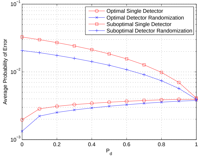
Figure 2.13: Average probability of error versus P_d for different approaches when \sigma = 0.1 , P_{av,0} = 1.0 and P_{av,1} = 0.1 .
