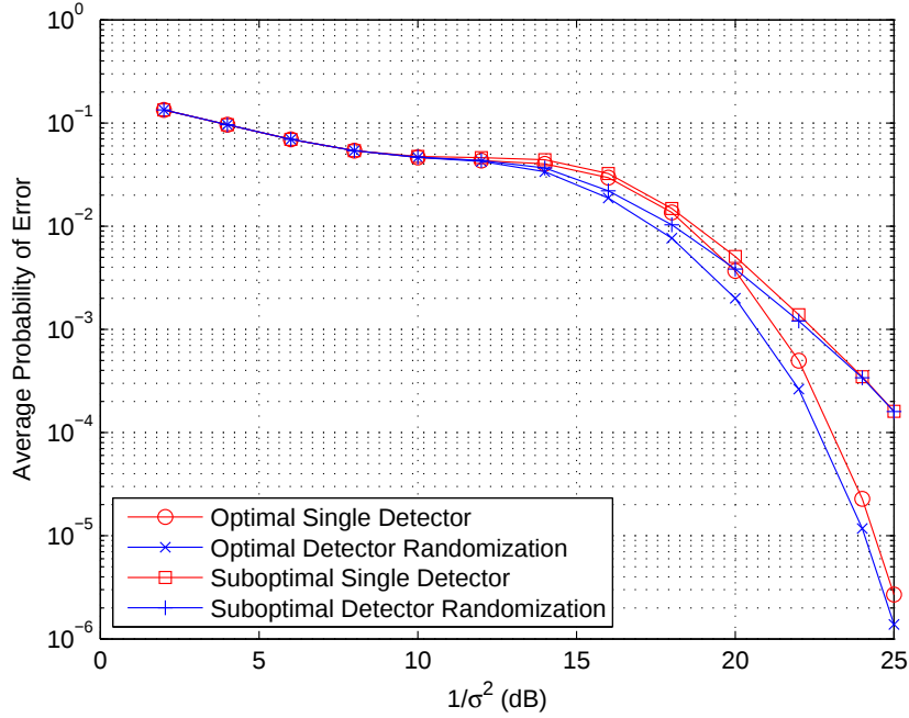
Figure 2.2: Average probability of error versus 1/\sigma^2 for different approaches when P_{av,0} = 1.3 and P_{av,1} = 0.4 .
