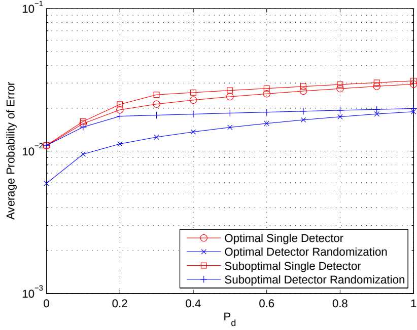
Figure 2.4: Average probability of error versus P_d for different approaches when \sigma = 0.15 , P_{av,0} = 1.3 and P_{av,1} = 0.4 .
