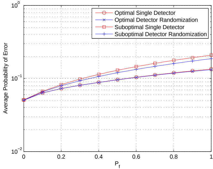
Figure 2.18: Average probability of error versus P_f for different approaches when \sigma = 0.25 , P_{av,0} = 1.0 and P_{av,1} = 0.1 .
