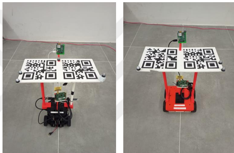
Figure 5.3 Turtlebot Burger and Rosbot 2.0
