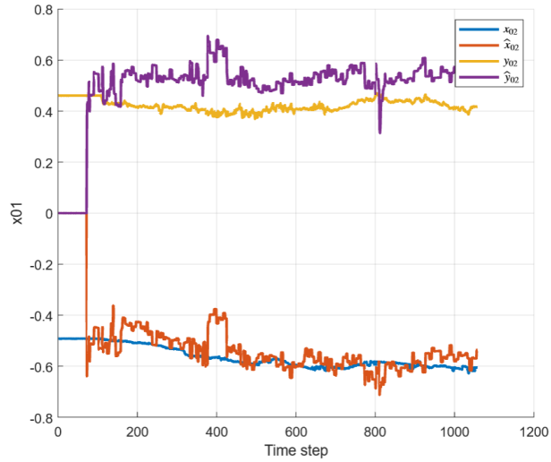
Figure 5.7 x and y positions estimation and ground truths of second ground robot.
