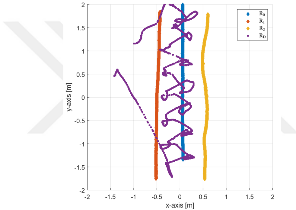
Figure 5.8 Ground robots and drone positions in a real experiment.
