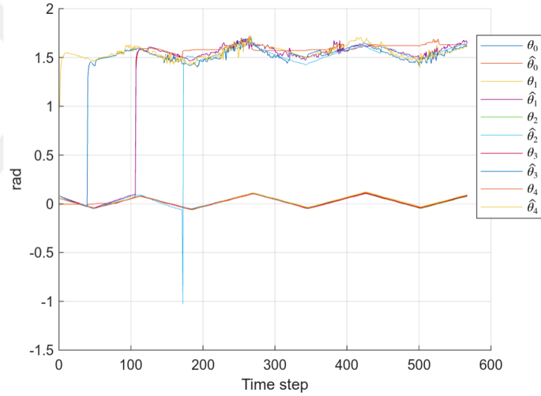
Figure 4.11 Exact heading values and EKF estimation headings of the ground robots.
