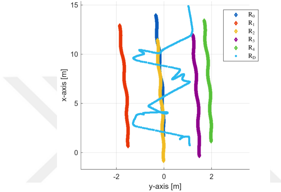
Figure 4.8 Ground robots and drone positions in simulation.
