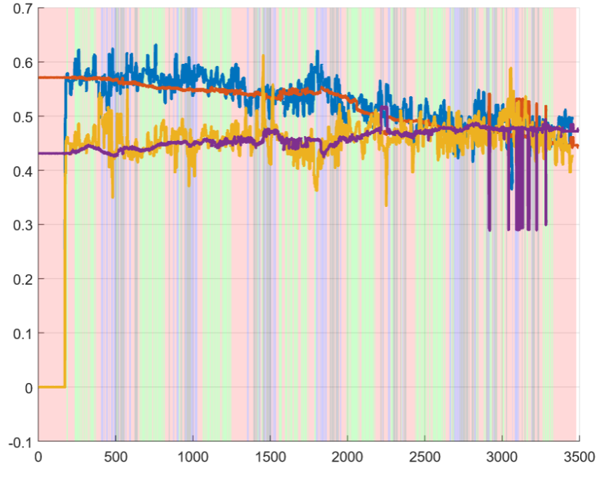
Figure 5.9 x and y positions estimation and ground truths of first ground robot.
