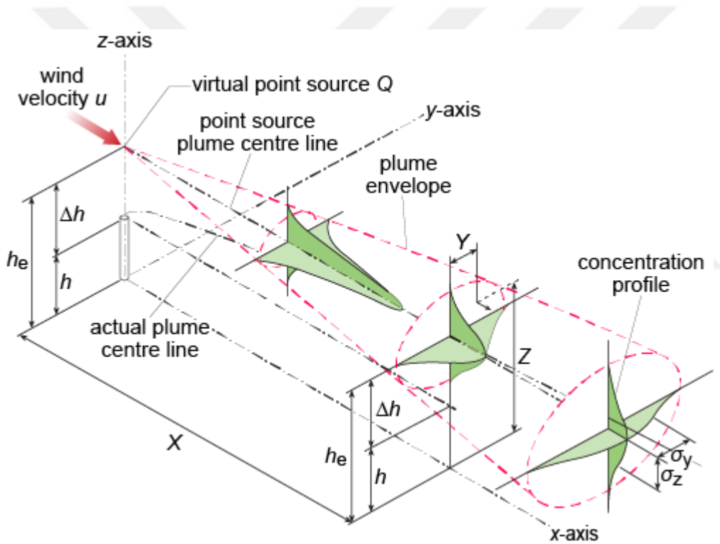
Figure 2.19. Gaussian Dispersion Model (Nesaratnam and Taherzadeh, 2014).
