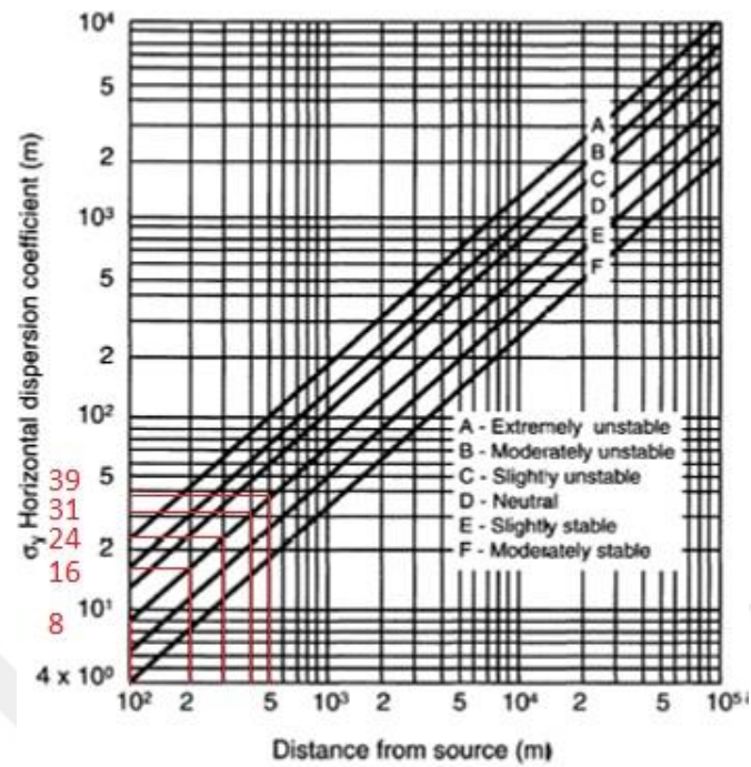
Figure 5.10. Horizontal dispersion coefficient, \sigma_y , vs. Downwind distance, x (Godish, 2004).
