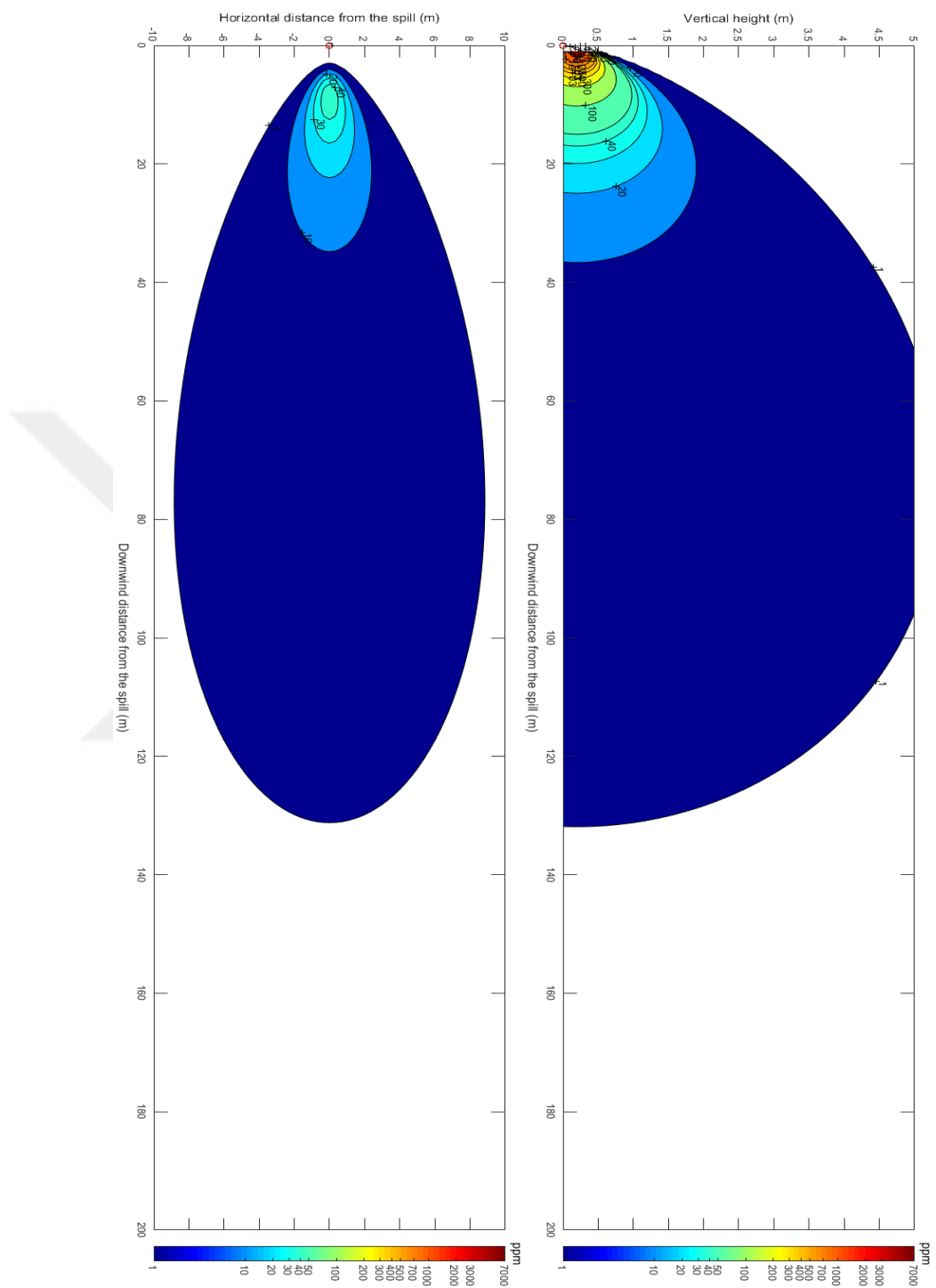
Figure 5.13. Vapor Concentration vs. Downwind Distance at 10 °C Temperature
