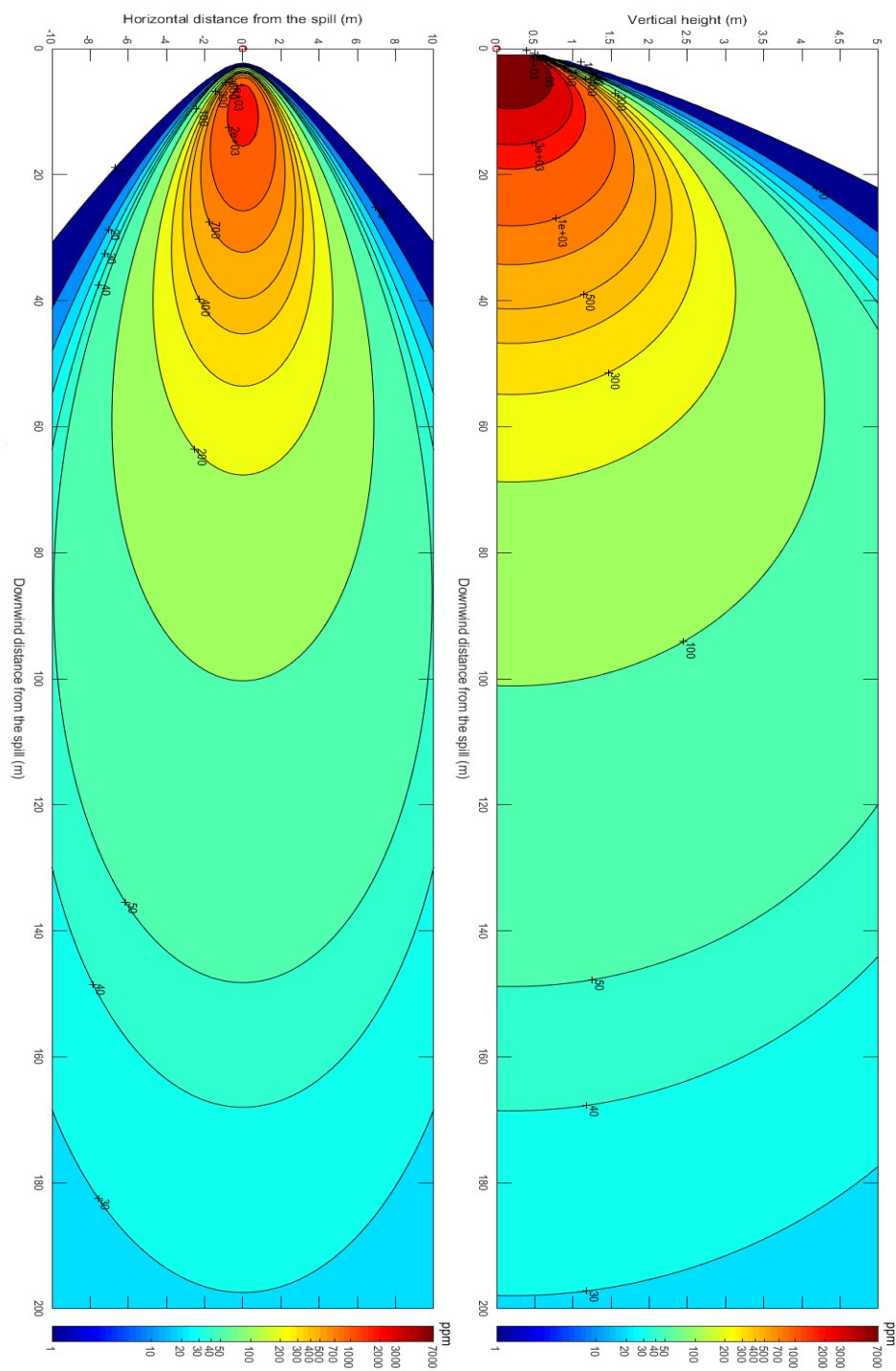
Figure 5.15. Vapor Concentration vs. Downwind Distance at 0.5 m/s Wind Speed
