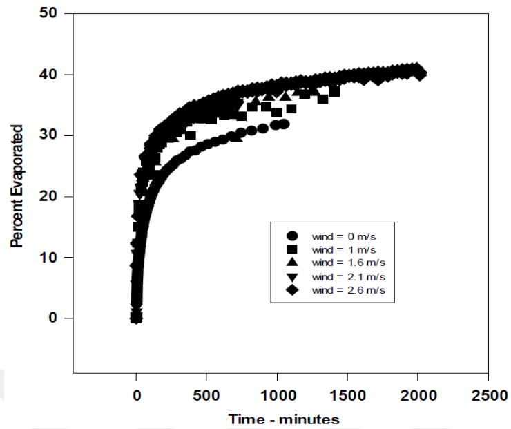
Figure 2.9. Evaporation Rates of ASMB versus Various Wind Speed (Fingas 2013).
