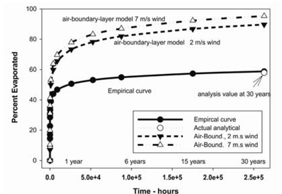
Figure 2.14. Evaporation Rate Modelling of Pembina Crude Oil with Air-layer-boundary Equation (like equation (33)) versus Real Data and Experimental Curve (Fingas, 2013)
