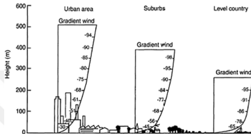
Figure 2.17. Effect of Urban, Suburbs and Rural Areas on Wind Speed (Turner, 1994)
