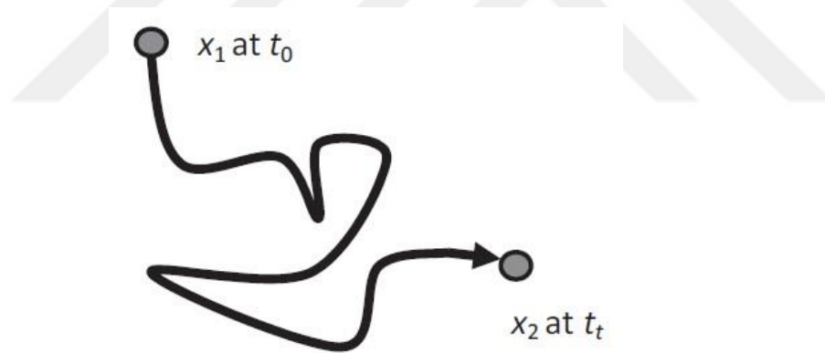
Figure 2.25. Movement of a Particle in the Random Walk Model (Vallero, 2014)
