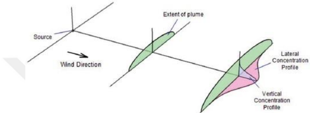
Figure 2.20. Non-buoyant Gaussian Dispersion from a Ground Source (Pursuer et al., 2016).
