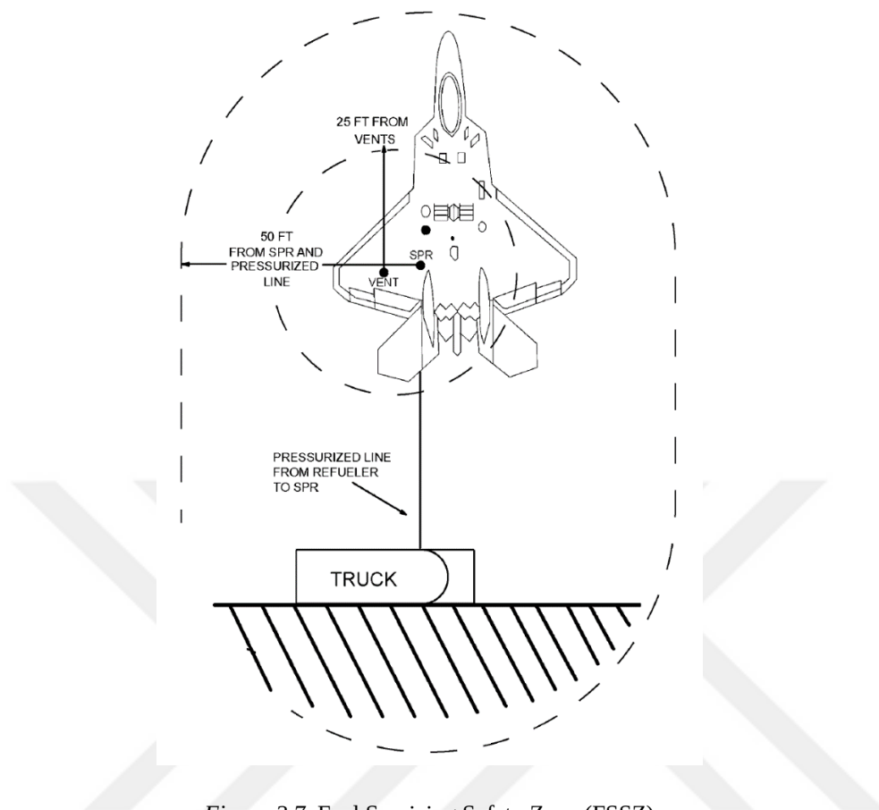
Figure 2.7. Fuel Servicing Safety Zone (FSSZ)
