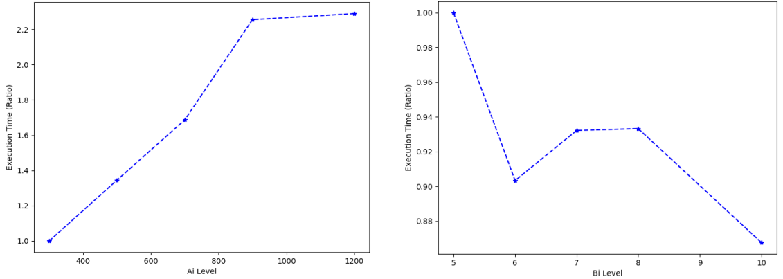
Figure 3.1 Effect of A_i and B_i on the execution time of Gurobi.
