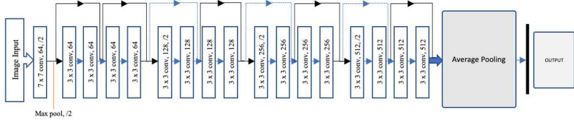
Figure 4.11. ResNet-18 Architecture.
