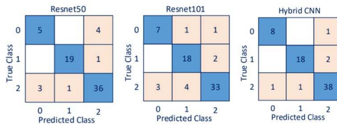
Figure 5.4. Confusion matrices
