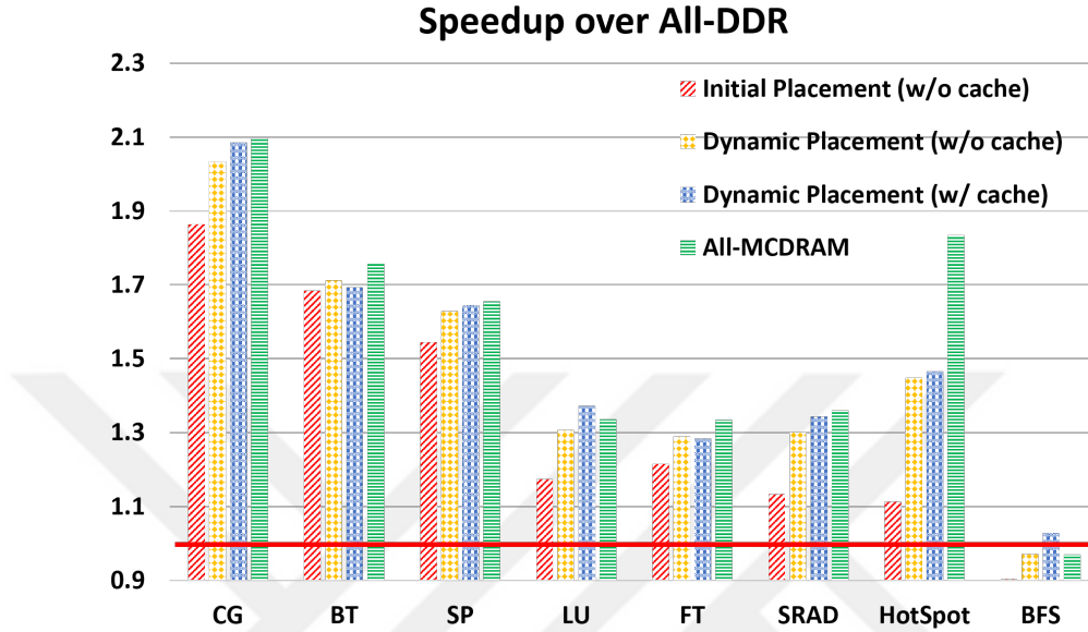
Figure 6.2: Speedup achieved by the object placement conducted by our tool against All-DDR mode. Red line shows the baseline. All values below 1 indicate degraded performance.
