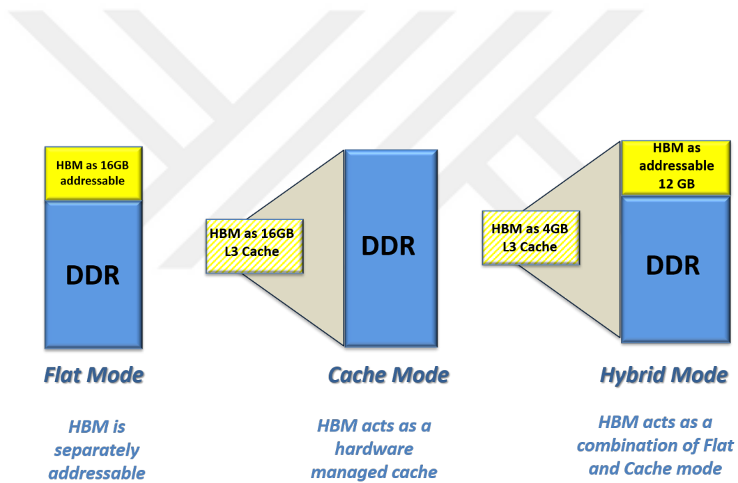
Figure 2.4: Intel KNL memory modes.
