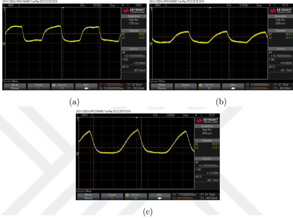
Figure 3.1: Photo-diode response for the screen flickering between black and white background at 60Hz, 120Hz, 240Hz. (a) This is response for 60Hz refresh rate where high corresponds to the white frame and low corresponds to the black frame. Cursors on screen show the period of one cycle of flicker where the frequency is measured as 29.94Hz. Note that one cycle of flicker has two frames (black and white) so the refresh rate of monitor is 2 \times 29.94 . (b) This is the response for 120 Hz. The frequency of one cycle of flicker is measured as 59.98 and refresh rate becomes 119.96Hz. (c) This is response for 240Hz. The frequency of one cycle of flicker is measured as 119.90Hz and refresh rate becomes 239.8Hz.
