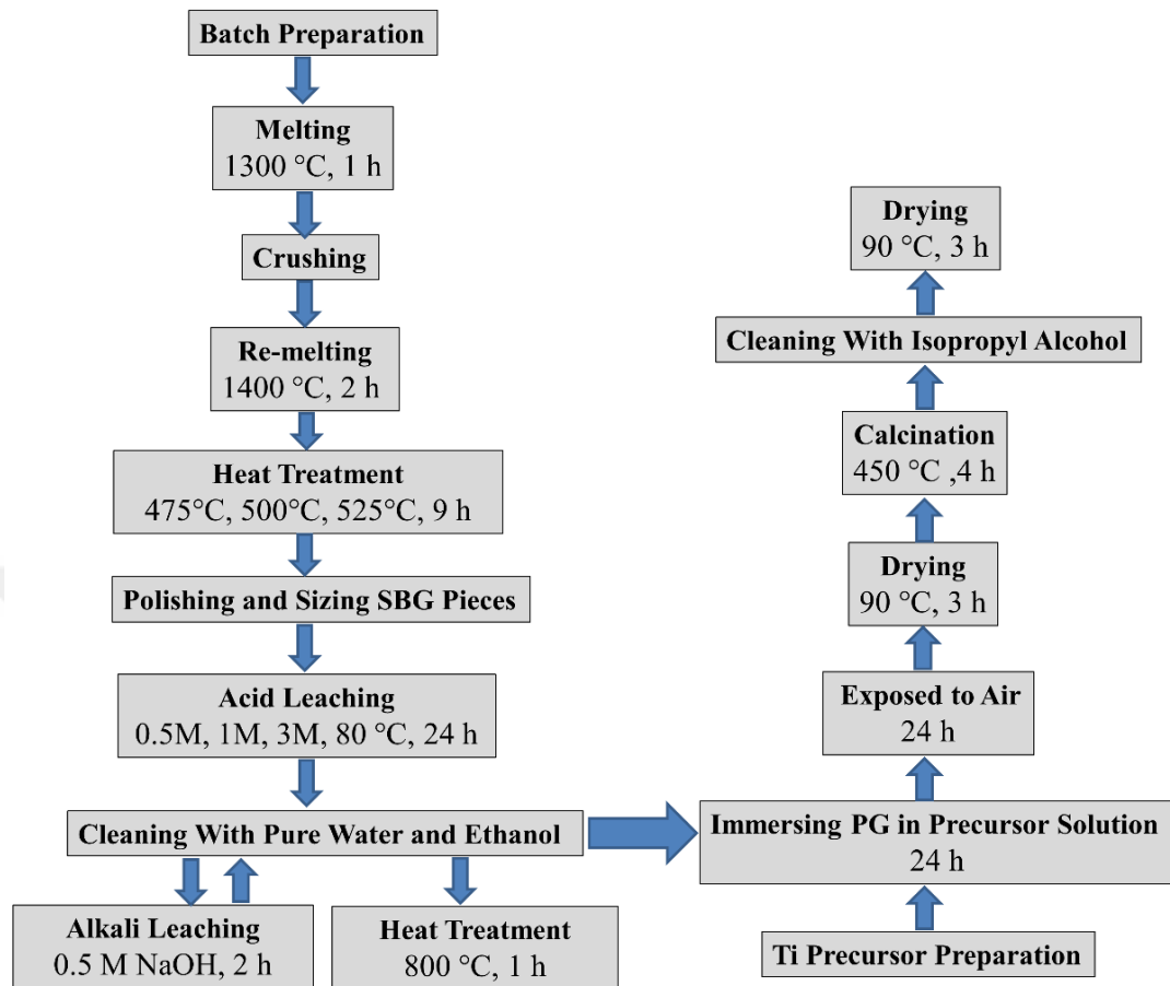
Figure 3.2. The steps in the PG production processes and \text{TiO}_2 crystallization within the PG.
