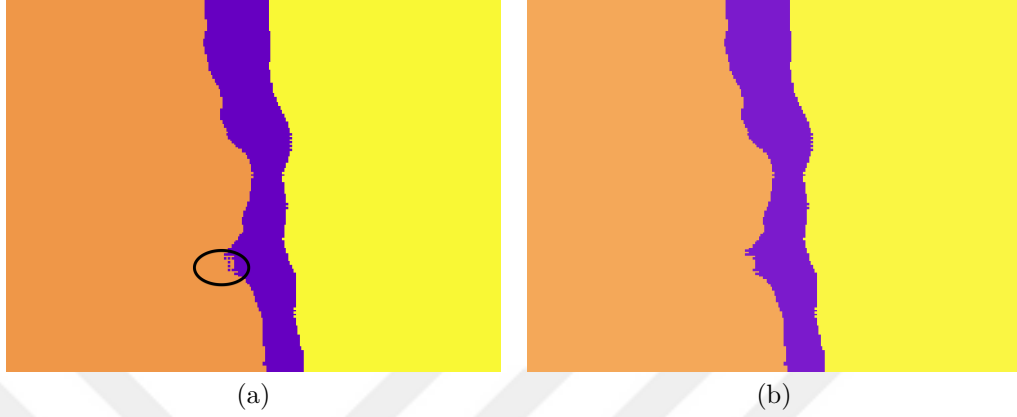
Figure 3.12: Illustration of the post-processing step on a sample image: (a) Resulting regions after the remapping operation. The circled area includes small regions that are byproducts of the remapping procedure. (b) Resulting segmentation after the extra small regions are eliminated by clean-up.
