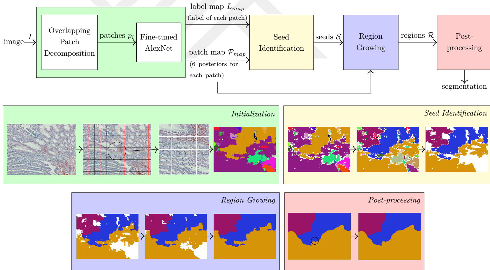
Figure 3.8: Schematic overview of Tier 2. Steps and terms are explained in the subsections of Section 3.2.
