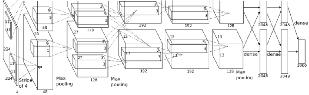
Figure 3.2: The AlexNet model defined in [29]. Used model parameters are given in Table 3.1. This image is used under the knowledge of NIPS Proceedings and permission of one of the copyright owner authors: Alex Krizhevsky.
