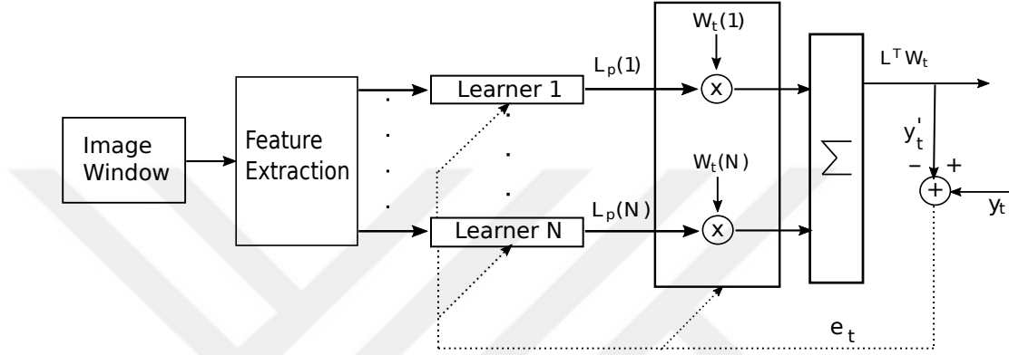
Figure 3.4: Mixture of learners block diagram.
