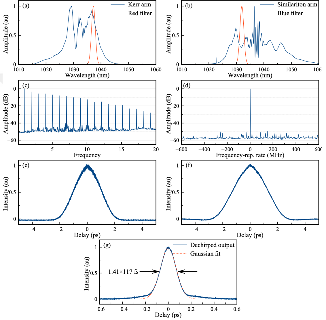
Figure 5.3: Harmonically mode-locked state at 1.007 GHz ((67 th harmonic): (a) spectrum at the output of the Kerr arm and the subsequent filter, (b) spectrum at output of the similariton arm and the subsequent filter, (c) radio frequency spectrum spanning 20 GHz, (d) radio frequency spectrum centered around the first line showing a supermode suppression of 50 dB, (e) intensity autocorrelation trace at the output of the Kerr arm, (f) Intensity autocorrelation trace at the output of the similariton arm (laser output), (g) Intensity autocorrelation trace of de-chirped laser output (similariton arm)
