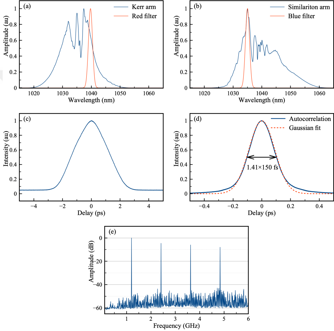
Figure 5.1: Harmonically mode-locked state at 1.208 GHz ( 83^{rd} harmonic): (a) spectrum at the output of the Kerr arm and the subsequent filter, (b) spectrum at the output of the similariton arm and the subsequent filter, (c) intensity autocorrelation trace of the laser output (from the similariton arm), (d) intensity autocorrelation trace of de-chirped laser output showing a pulse duration of 150 fs, (e) radio frequency spectrum showing a supermode suppression ratio of \sim 45 dB
