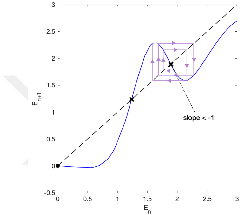
Figure 4.10: The evolution towards a period-doubled state. The pulse energy is unstable here because the slope is less than -1. The arrows show a trajectory starting from a perturbation from this unstable fixed point, which diverges away from it and converges to a period-doubled state.
