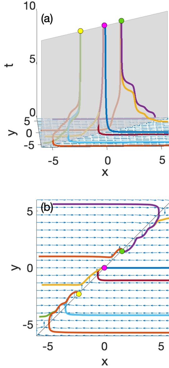
Figure 2.1: Behavior of a nonlinear dissipative dynamical system, \dot{x} = 20(y - x) , \dot{y} = \sin(xy) - 0.4y . (a) shows the evolution in time from multiple initial conditions. (b) shows the same trajectories projected onto the 2-dimensional phase space. This system is dissipative, which allows it to have attractors. The attractors shown are three stable fixed points, marked by yellow, pink, and green dots; these points attract all trajectories in their respective basins of attraction. Note also that x approaches the x = y line much faster than y approaches the fixed points; x is slaved to the order parameter y so that the dynamics is effectively one-dimensional.
