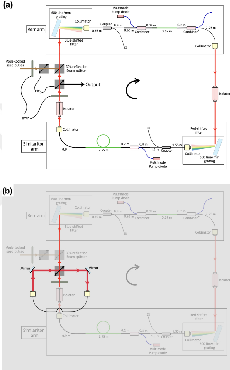
Figure 3.2: (a) detailed schematic representation of our Mamyshev oscillator. The green lines represent Yb-doped gain fibers with a 10\mu\text{m} core diameter; the thick (thin) black lines represent passive fibers with 10\mu\text{m} ( 6\mu\text{m} ) core diameter; the thick blue lines represent multimode fibers carrying the pump. The combiner with an asterisk is used as a pump stripper and a mode-field adaptor. PBS: polarizing beam splitter; HWP: half waveplate; (b) detailed schematic representation of the orthogonally polarized secondary loop. The cavity is shaded to highlight the elements of the secondary loop. The secondary loop is used for pulse interaction experiments only
