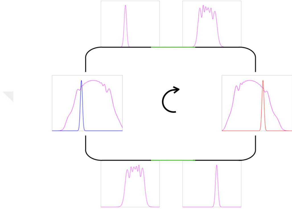
Figure 3.1: illustration of the working principle of a Mamyshev oscillator. There are two non-overlapping spectral filters. After each filter, the pulse experiences gain to compensate the filtering and other losses, and nonlinearity, for its spectrum to broaden and reach the next filter. With insufficient nonlinearity, the light can not survive both filters.
