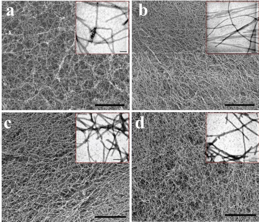
Figure 2.3 SEM images of LN-PA/GAG-PA (a), LN-PA/E-PA (b), K-PA/GAG-PA (c) and K-PA/E-PA (d) show nanofiber networks resembling the fibrous ECM structure. Scale bars are 3 \mu\text{m} in length. STEM images of all PA nanofibers formed at pH 7.4 are given in inner frames of panels a, b, c and d. Scale bars are 100 nm in length.
