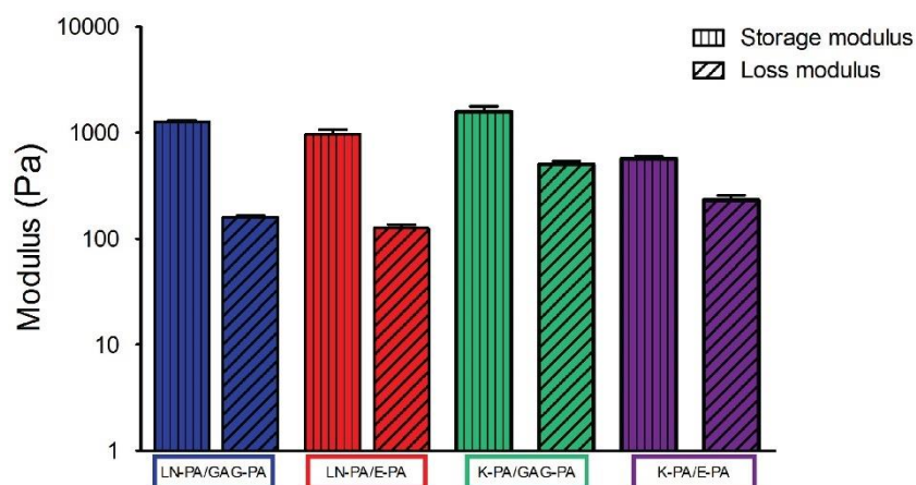
Figure 2. 5 Mechanical properties of PA gels measured by oscillatory rheology. Rheology results showed gelation as a result of nanofibrous network formation by all combinations at pH 7.4.
