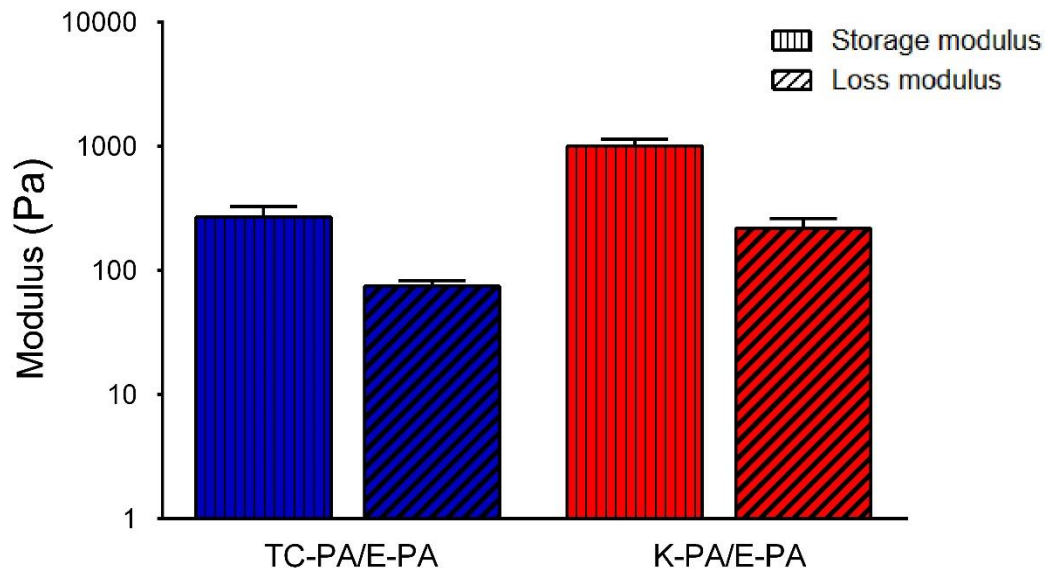
Figure 5. 7 Mechanical properties of PA gels characterized by oscillatory rheology.
