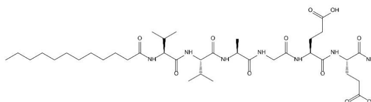
Figure 4. 2 Chemical structures of PA molecules.
