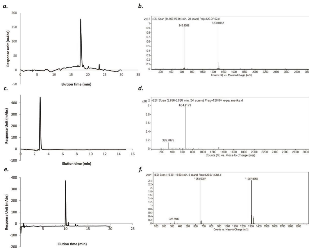
Figure 5.3 LC and MS of PA molecules used. LC results verify the purity of TC-PA (a), E-PA (c) and K-PA (e). MS of PA-TC (b), [M+H]^+ (calculated): 1290.81 [M+H]^+ (observed): 1290.81 [M+2H]^{+2/2} (calculated): 645.91 [M+2H]^{+2/2} (observed): 645.91. MS of PA-E (d), [M-H]^- (calculated): 654.42 [M-H]^- (observed): 654.42, [M-2H]^{-2/2} (calculated): 326.71 [M-2H]^{-2/2} (observed): 326.71. MS of PA-K (f), [2M+H]^+ (calculated): 1307.96 [2M+H]^+ (observed): 1307.98 [M+H]^+ (calculated): 654.48 [M+H]^+ (observed): 654.51 [M+2H]^{+2/2} (calculated): 327.74 [M+2H]^{+2/2} (observed): 327.75
