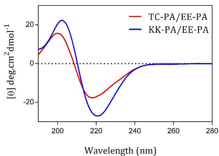
Figure 4. 5 CD spectra of TC-PA/EE-PA and KK-PA/EE-PA nanofibers.
