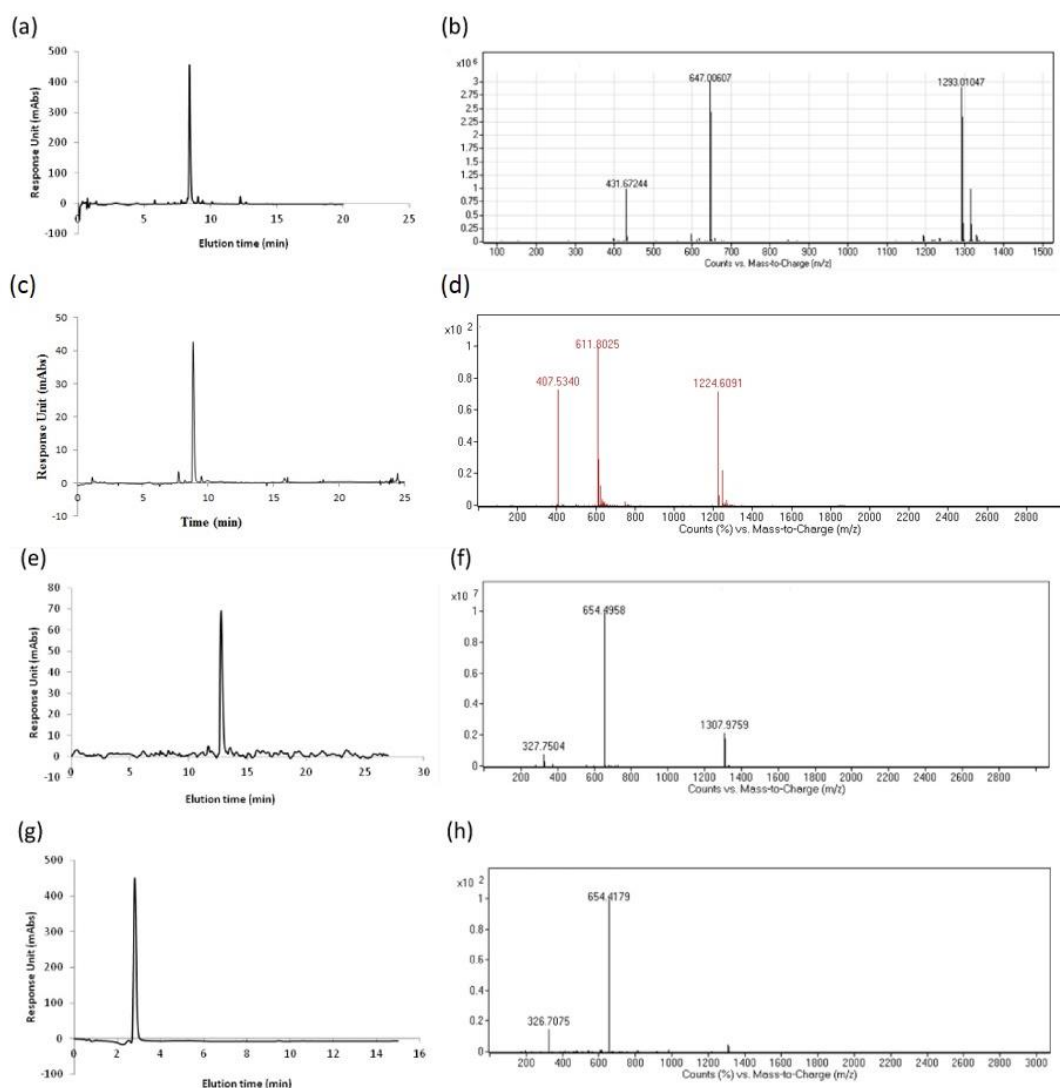
Figure 3. 2 LC-MS of LN-PA (a,b), GAG-PA (c,d), K-PA (e,f) and E-PA (g,h). Mass spectrometry of LN-PA; [M+H]^+ (calculated): 1292.93, [M+H]^+ (observed): 1293.01, [M+2H]^{+2/2} (calculated): 646.96, [M+2H]^{+2/2} (observed): 647.01, [M+3H]^{+3/3} (calculated): 431.64, [M+3H]^{+3/3} (observed): 431.67. Mass spectrometry of GAG-PA; [M-H]^- (calculated): 1225.59, [M-H]^- (observed): 1224.61, [M-2H]^{-2/2} (calculated): 612.29, [M-2H]^{-2/2} (observed): 611.80, [M-3H]^{-3/3} (calculated): 407.86, [M-3H]^{-3/3} (observed): 407.53. Mass spectrometry of K-PA; [2M+H]^+ (calculated): 1307.96, [2M+H]^+ (observed): 1307.98, [M+H]^+ (calculated): 654.48, [M+H]^+ (observed):
