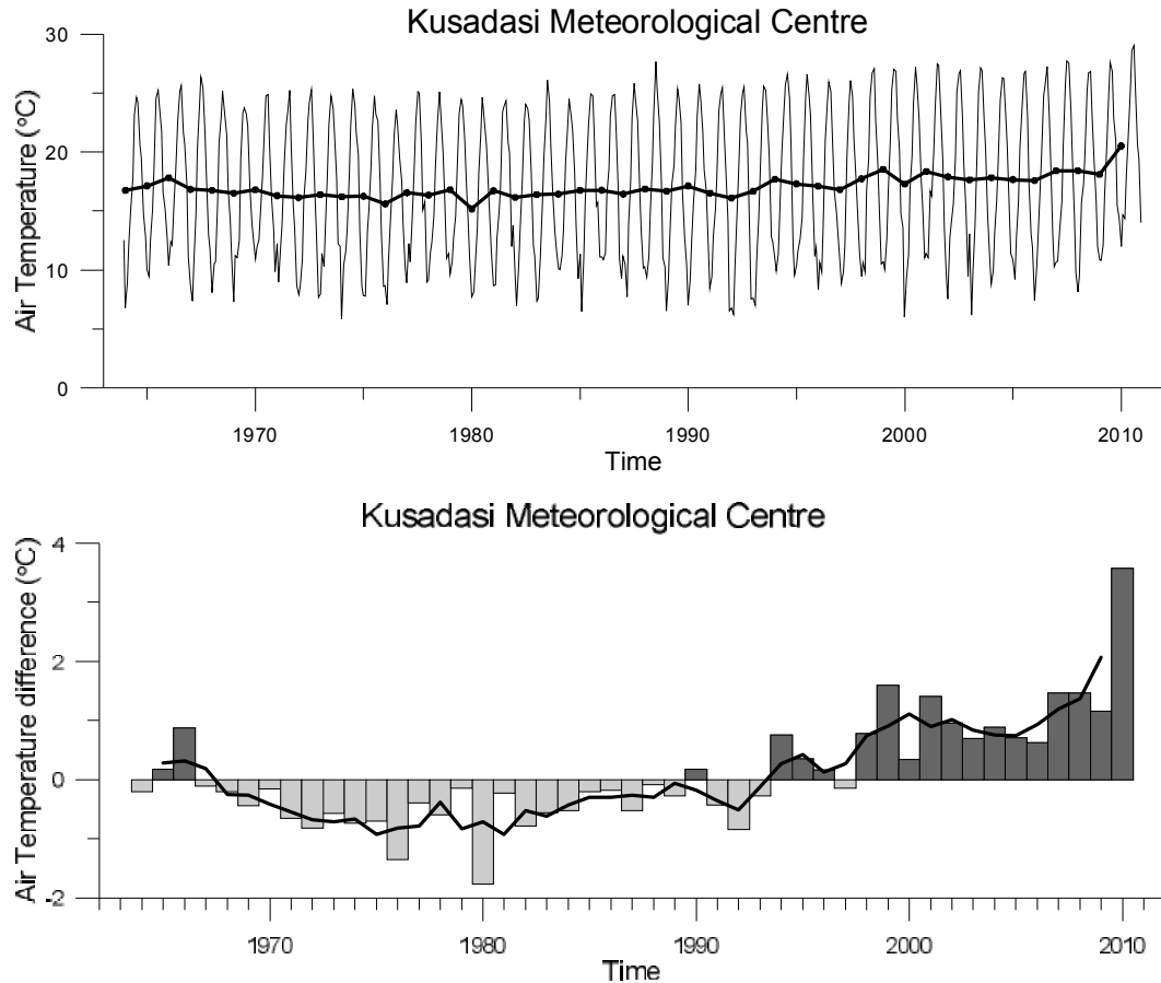
Figure 3.58 Time series of monthly average (thin line) and annual mean (thick line) air temperature (°C) (top), and yearly anomaly time series (bars) with moving averages (thick line) (bottom) for the Kuşadası Bay.
