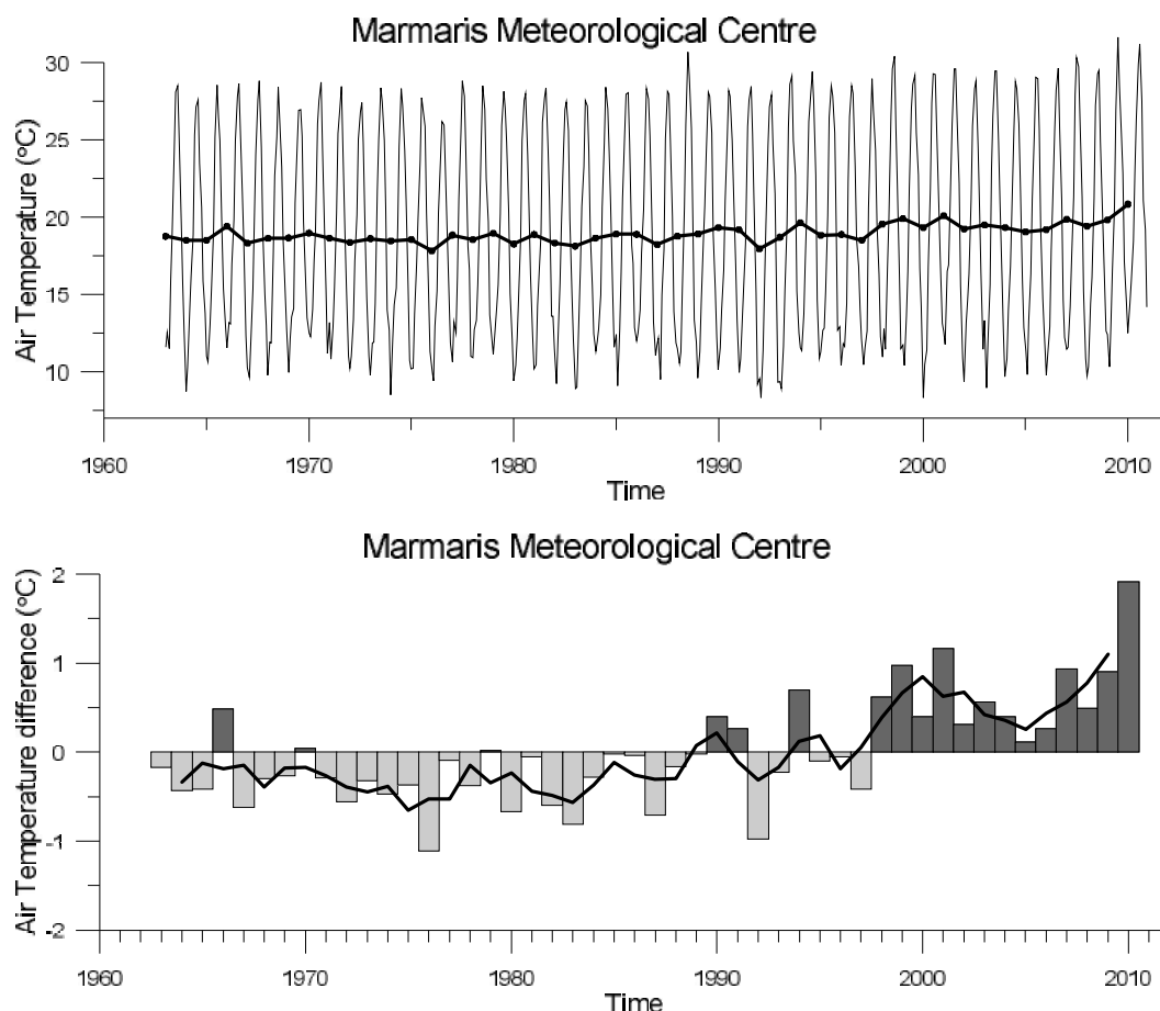
Figure 3.77 Time series of monthly average (thin line) and annual mean (thick line) air temperature (°C) (top), and yearly anomaly time series (bars) with moving averages (thick line) (bottom) for the Gökova Bay.
