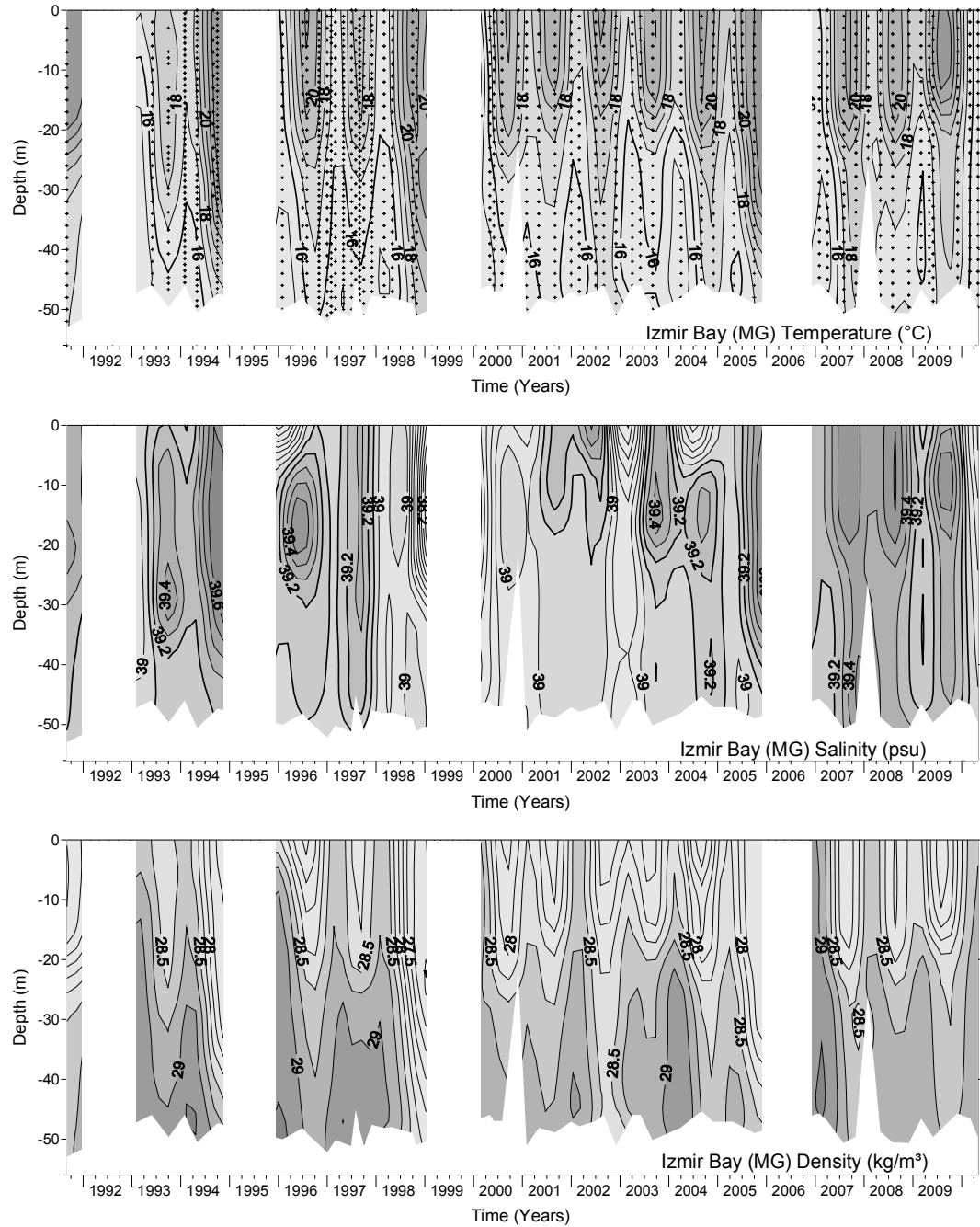
Figure 3.48 b Temporal evaluations of temperature, salinity and density fields of İzmir Middle Gyre region starting from summer 1991 up to spring 2010. The areas in white represent where data was not collected.
