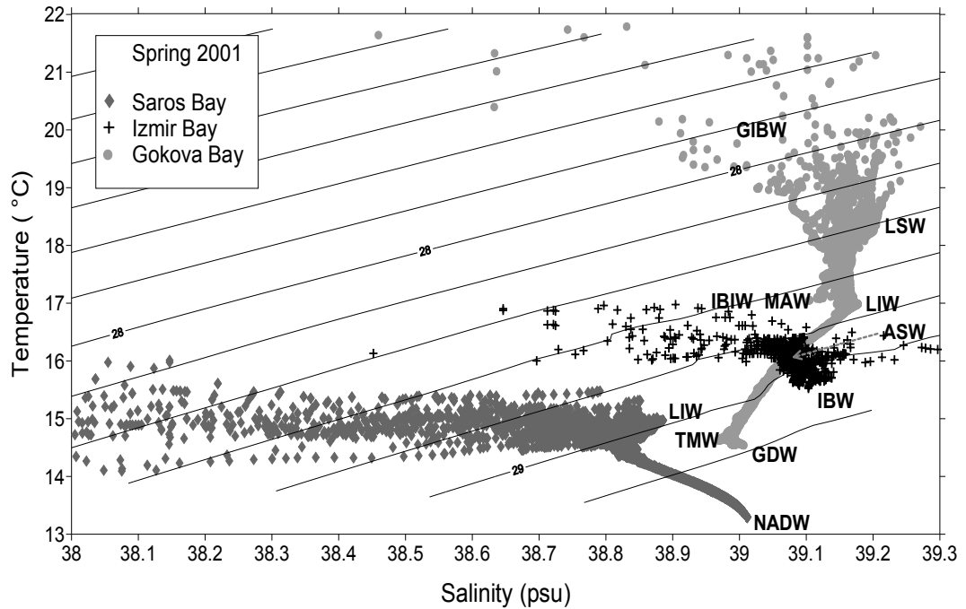
Figure 4.8 T-S diagram of spring 2001.
