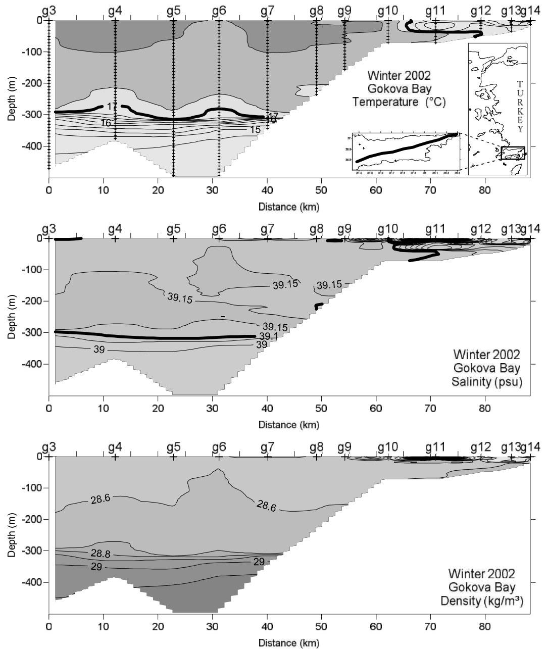
Figure 3.92 The salinity vertical section along the long axis of Gökova bay in winter 2002.
