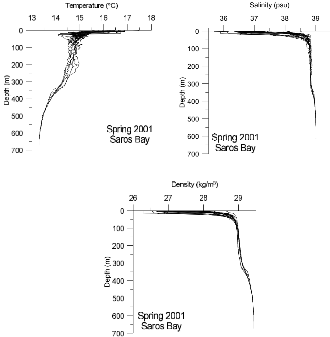
Figure 3.11 Temperature, salinity and density profiles of Saros bay in spring 2001.
