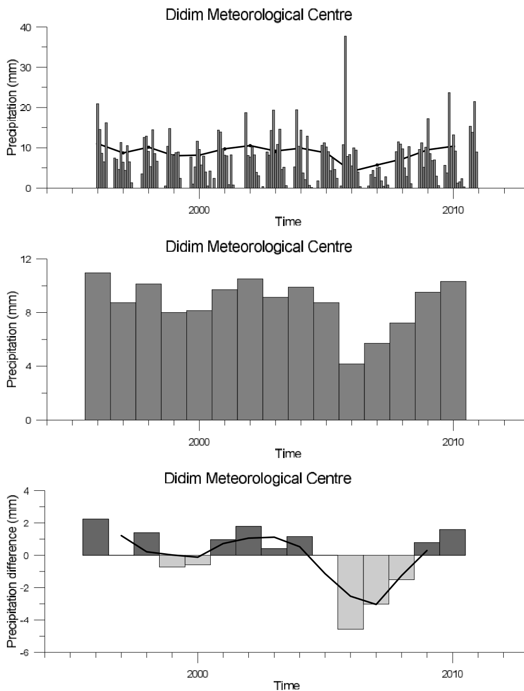
Figure 3.70 Time series of monthly averaged (top), annual mean precipitation (center) and yearly anomaly time series (bars) with moving averages (thick line) (bottom) for the Güllük Bay.
