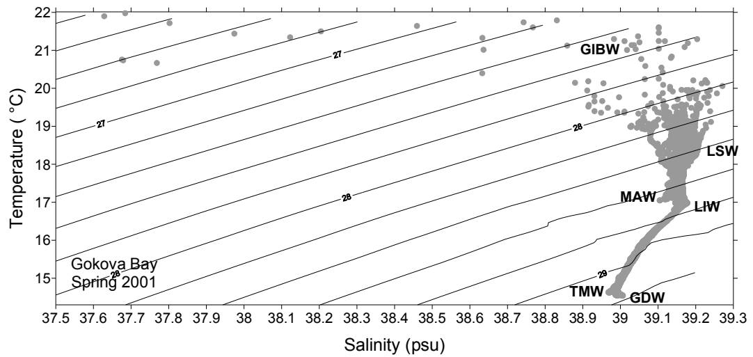
Figure 3.89 T-S diagram of spring 2001 (Gökova Bay).
