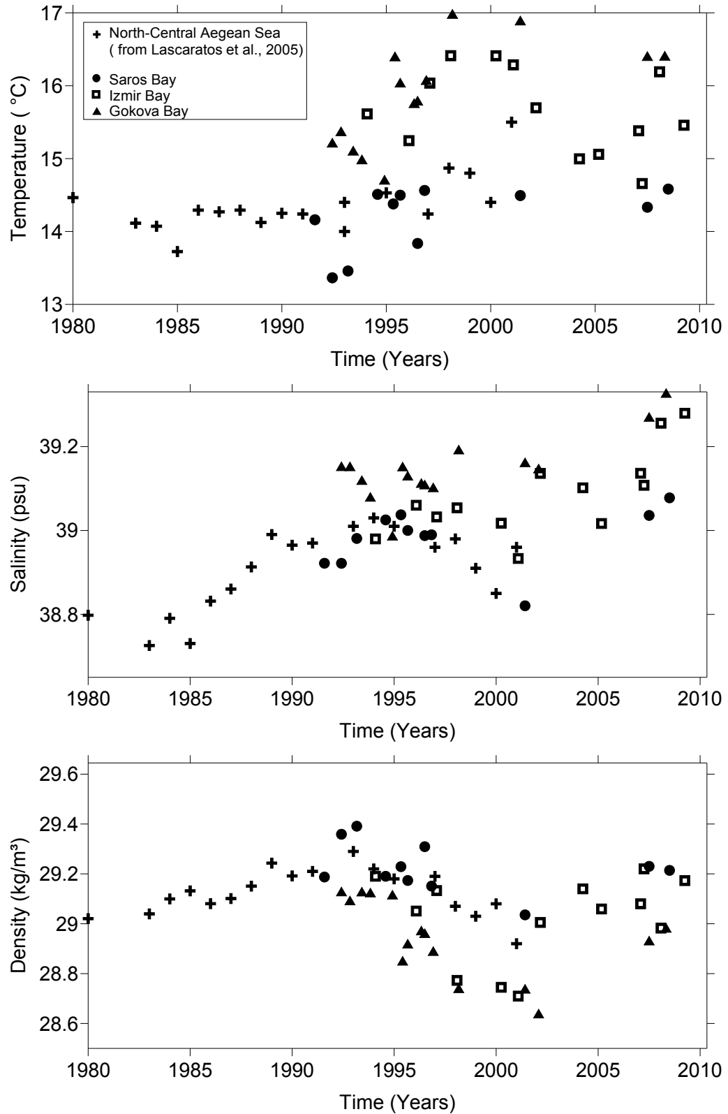
Figure 4.1 Time evolution of mean integrated values of temperature, salinity and density in the 100–300 dbar layer in the North-Central Aegean Sea (after Velaoras, D. and Lascaratos, A., 2005) in the Saros and in the Gökova Bay. İzmir Bay is very shallow area. The İzmir data is selected only for winter period from deep part of the Bay to rid of the influence of the seasonal variations.
