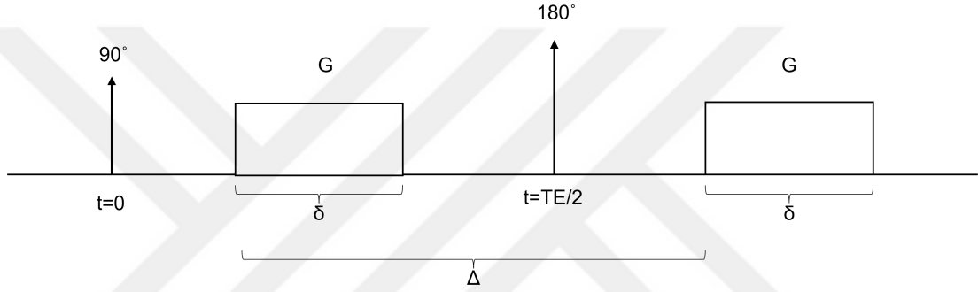
Figure 2.1: The spin-echo diffusion MRI sequence. This sequence incorporates two diffusion-sensitizing gradient pulses, one before and one after the 180° refocusing RF pulse.
