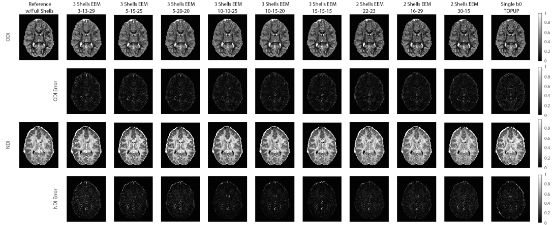
Figure 4.3: ODI and NDI maps constructed with NODDI analysis using the undersampled multi-shell HARDI data at R=2 , shown for one of the subjects. The absolute error image for each metric was computed with respect to the reference metric maps obtained with the original 89 diffusion-weighted gradient direction.
