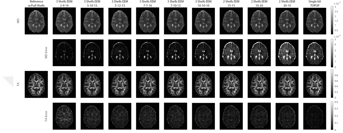
Figure 4.4: MD and FA maps, obtained through DTI analysis of the undersampled multi-shell HARDI data for R=3 . The metric maps and error images are shown for one of the subjects. The absolute error images compares the performances of undersampling strategies with respect to the reference, fully sampled case.
