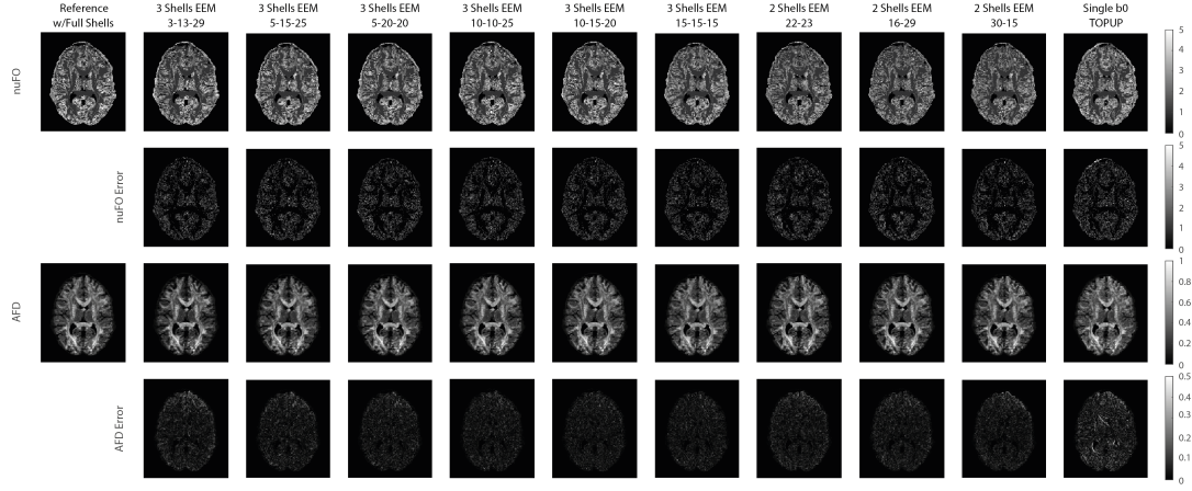
Figure 4.2: nuFO and AFD maps obtained from MSMT-CSD analysis using the undersampled multi-shell HARDI data at R=2 for one of the subjects. Each metric map is shown with the corresponding absolute error image computed with respect to the reference metric maps with the original 89 diffusion-weighted gradient directions.
