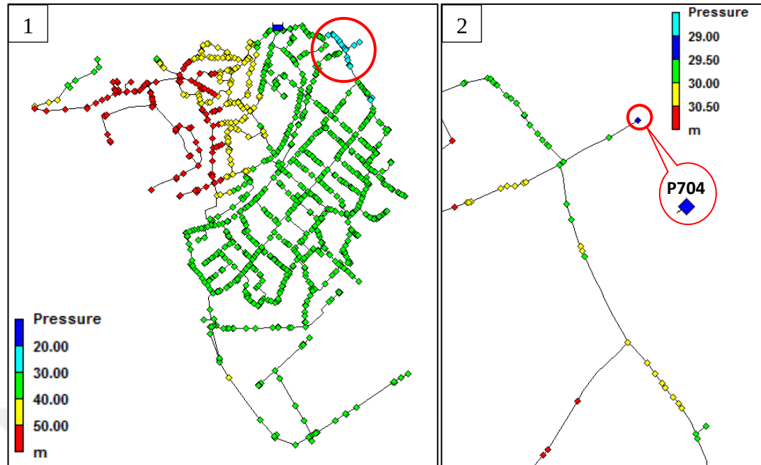
Figure 4.35. The location of the CP related to the least predicted pressure in the PSA (assuming -25% decrease of non-leakage flow) during winter season. CP (P704), on 15.01.2016 at 12:00 AM; min. pressure = 29.60 m, \Sigma Q_{(75\% \times \text{non-leakage}) + (\text{leakage})} = 69.46 \text{ m}^3/\text{h} and pressure upstream PRV = 32.05 m
