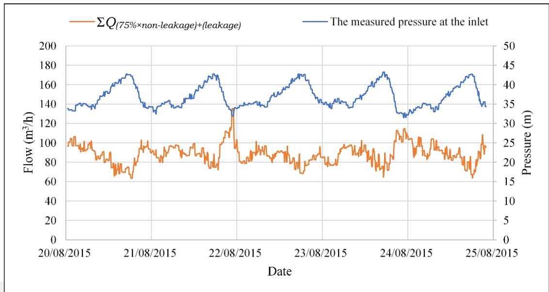
Figure 3.20. The pressure measured at the inlet vs. \Sigma Q_{(75\% \times \text{non-leakage}) + (\text{leakage})} , (August 20 – 25, 2015)
