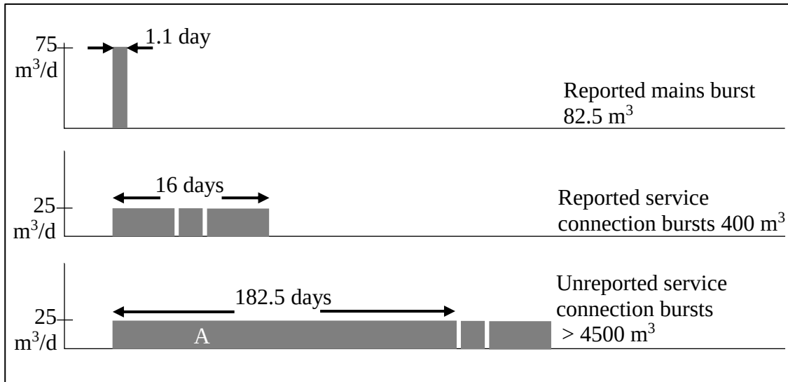
Figure 2.7. The effect of runtime on the volume of leaked water, (Pilcher et al. 2007)
