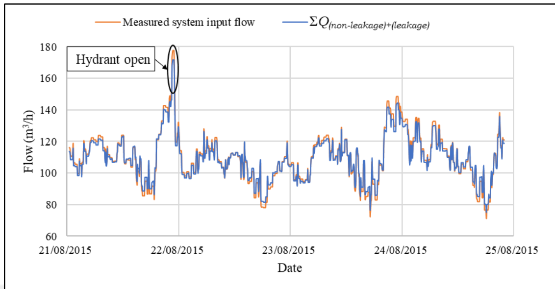
Figure 4.4. The measured system input flow vs. ( \Sigma Q_{(non-leakage)+(leakage)} ) at roughness R=57 , MAE = 1.67\text{m}^3/\text{h} and RMSE = 2\text{ m}^3/\text{h} (August 21-25, 2015)
