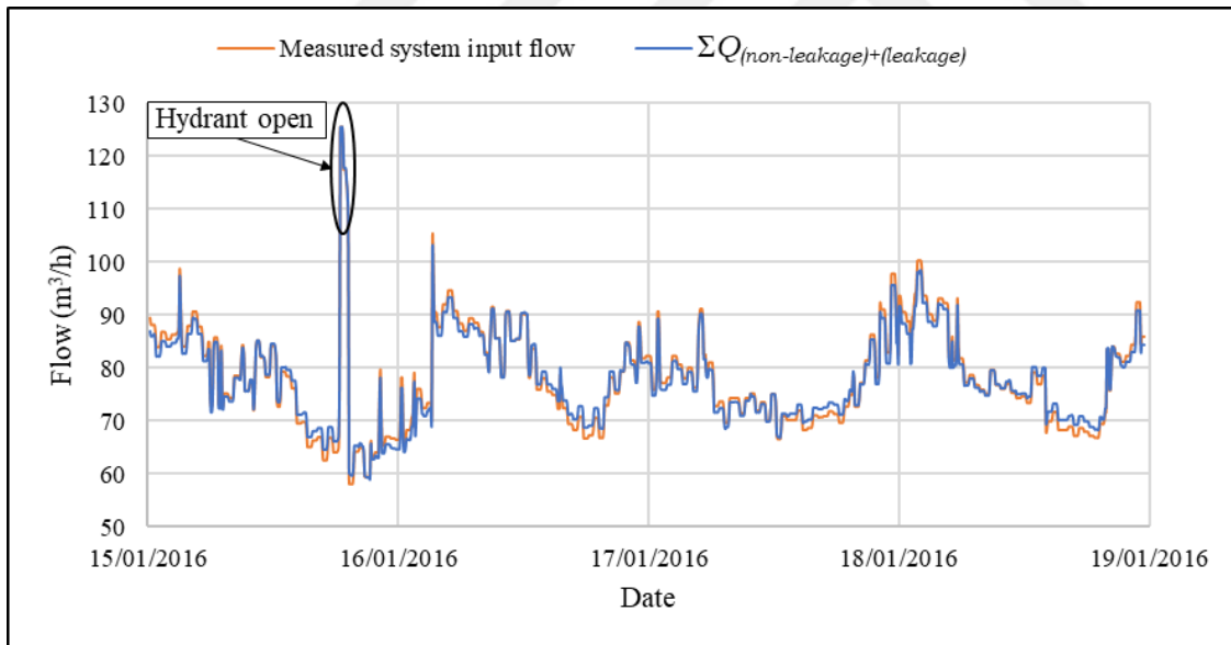
Figure 4.10. The measured system input flow vs. (\Sigma Q_{(non-leakage)+(leakage)}) at roughness R = 58 , MAE = 1.113 \text{ m}^3/\text{h} and RMSE = 1.286 \text{ m}^3/\text{h} (January 15 - 19, 2016)
