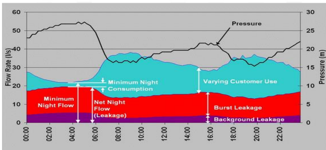
Figure 2.9. Leakage modeling based on MNF, (Pilcher et al. 2007)
