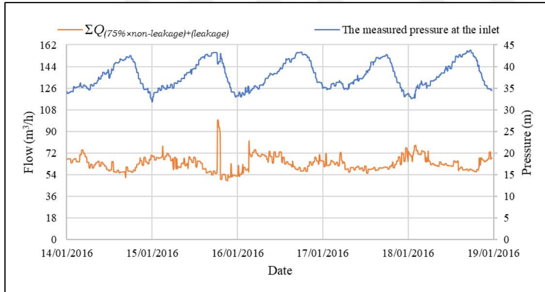
Figure 3.22. The pressure measured at the inlet vs \Sigma Q_{(75\% \times \text{non-leakage}) + (\text{leakage})} , (January 14 – 19, 2016)
