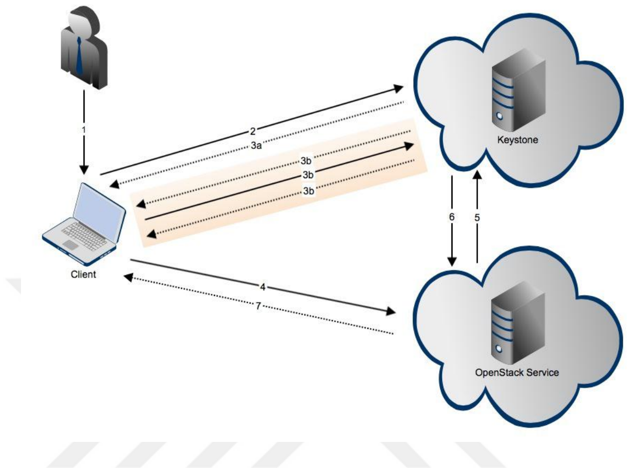
Figure 4.4 The authentication process for ‘regular’ username/password login.
