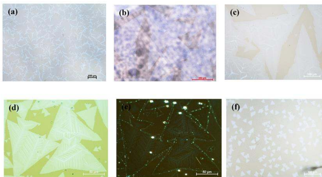
Figure 3.4. Optical images of MoS 2 grown on glass substrates: (a) continuous film, (b) MoS 2 crystals with domain sizes averaging 800 \mu\text{m} , (c) 400 \mu\text{m} edged crystals, (d) 150 \mu\text{m} MoS 2 flakes, (e) Dark field image illustrating amalgamation and second layer nucleation, (f) Tiny crystals, ~40 \mu\text{m} , at low concentrations of metallic precursor and furthest from the precursors
