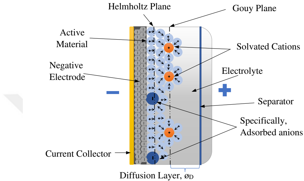
Figure 2.6. A model of the supercapacitor double layer (adapted from Bockris, 1963)
