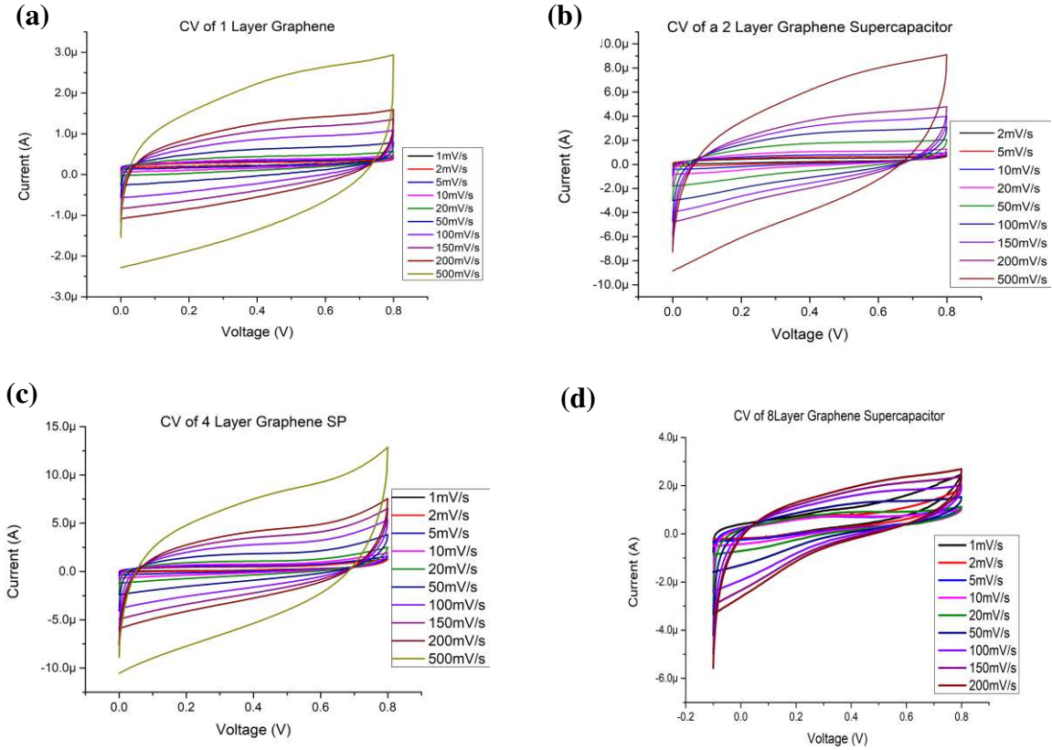
Figure 4.3. CV of different layers of Graphene: (a) 1layer graphene ( \sim 0.63 nm), (b) 2-layer graphene ( \sim 2 \times 0.63 nm), (c) 4-layer ( \sim 4 \times 0.63 nm), (d) 8 layers of graphene ( \sim 8 \times 0.63 nm).
