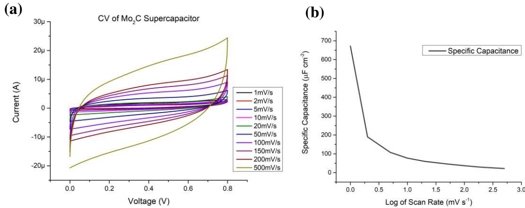
Figure 4.7. CV results: (a) CV at different scan rates, (b) specific capacitance obtained from different scans
