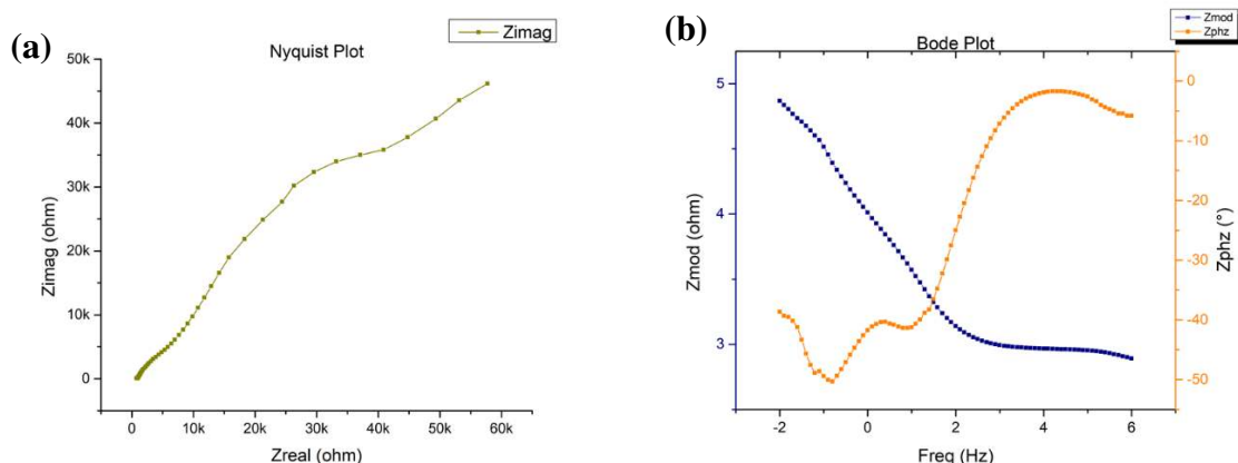
Figure 4.8. EIS of \text{Mo}_2\text{C} . (a). Nyquist plot. (b). Bode plot
