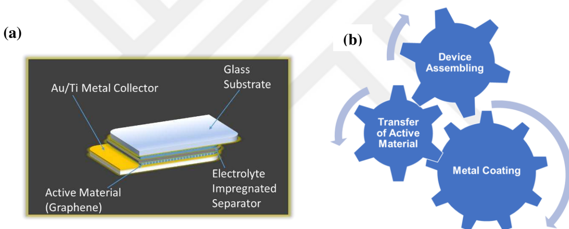
Figure 4.1. Supercapacitor's construct: (a) schematic of an EDLC, (b) fabrication process flow
