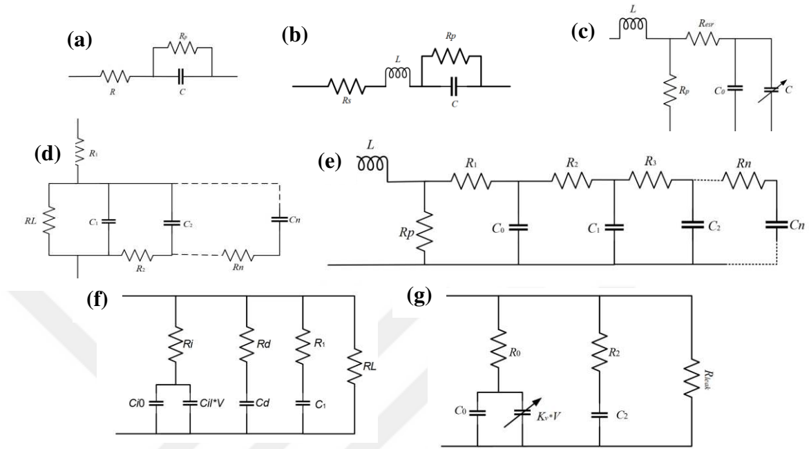
Figure 2.7. Equivalent circuit models of a supercapacitor: (a) simplest model of an SC, (b) simplest model with inductive effect considered, (c) Cultura and Salameh model, (d) the latter model, (e) the transmission line model, (f) Zubieta model and (g) the two-branch model (Zhang L., 2018)
