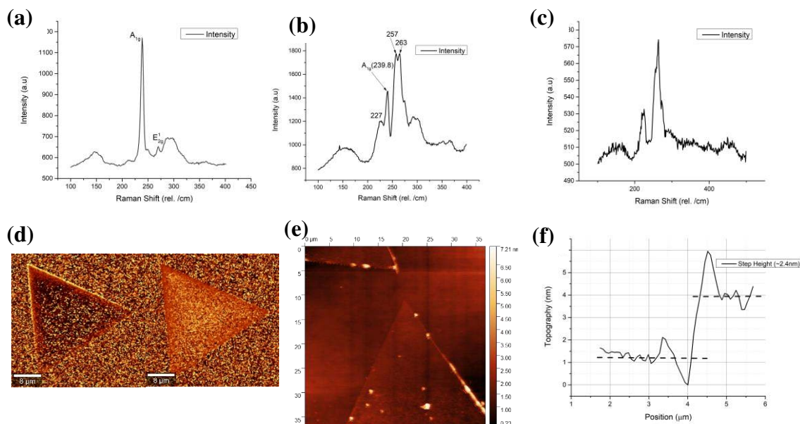
Figure 3.7. Optical characterization of MoSe 2 : (a) Raman spectra indicating monolayer 2H MoSe 2 , (b) Raman spectra taken from a MoSe 2 , with a star morphology, (c) Raman of MoSe 2 grown on glass substrate, (d) Raman image scan with peak filtering, (e) AFM of MoSe 2 transferred onto Si/SiO 2 substrates, (f) Step height results extracted from the AFM image results.
