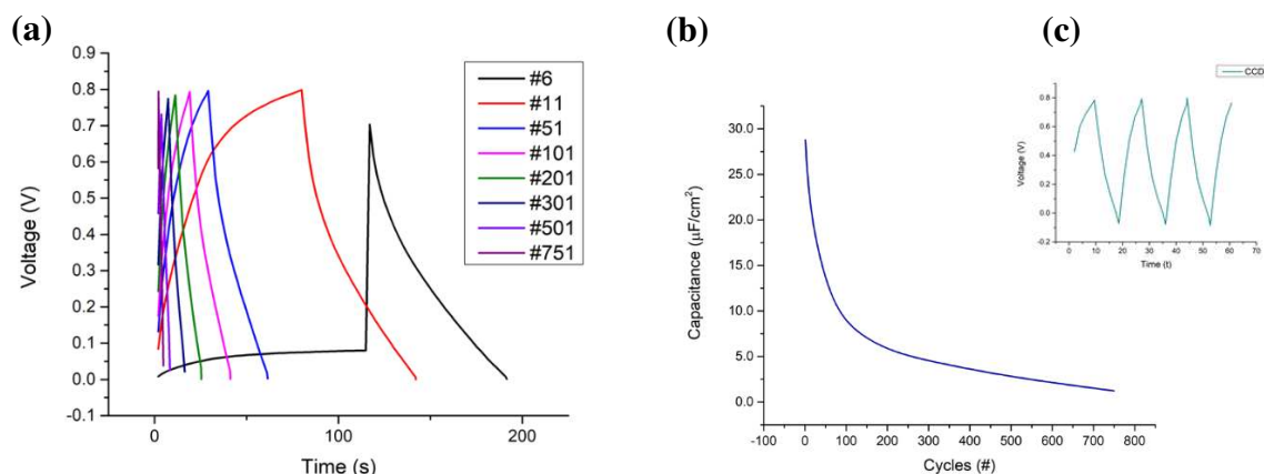
Figure 4.9. CCD of \text{Mo}_2\text{C} based SC: (a) Charge discharge curves after a random number of cycles, (b) Curve of capacitance (calculated from the discharge curve) vs. cycle number, indicating the capacitors retention capability, (c) Continuous CCCD for the first four charge discharge cycles.
