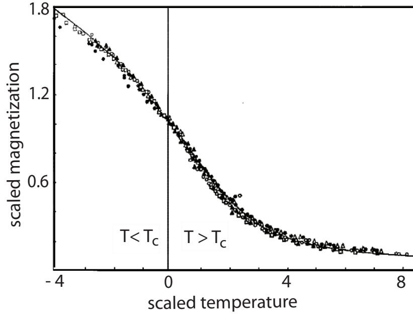
Figure 1.2: The experimental data of the magnetization for five elements showing the universal behavior: The data of CrBr 3 (lattice anisotropy), EuO (second-neighbor interactions), Ni (itinerant-electron ferromagnet), YIG (ferrimagnet), and Pd 3 Fe (ferromagnetic alloy). All data are consistent with the scaled function given by three dimensional Heisenberg model.
