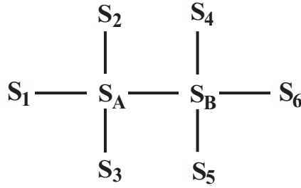
Figure 2.1: Spin configuration of the model: Spins used in H(S_A, S_B) are shown.
