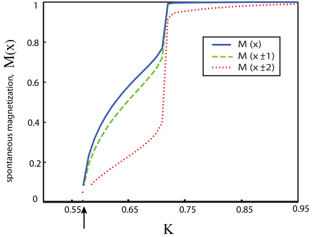
Figure 3.7: The longitudinal segregation of the Metropolis rate for \ell = L/10 : The critical behavior is expected to be obtained at K = 0.57 which is shown by the arrow.
