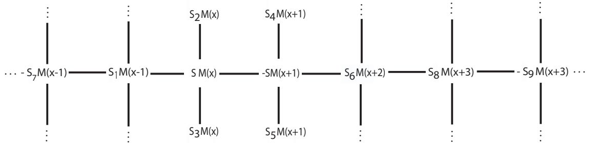
Figure 3.4: The nearest neighbor spins and the corresponding magnetization: S is one of the “+” and the “-” of the configuration we interpreted in Figure 3.3.
