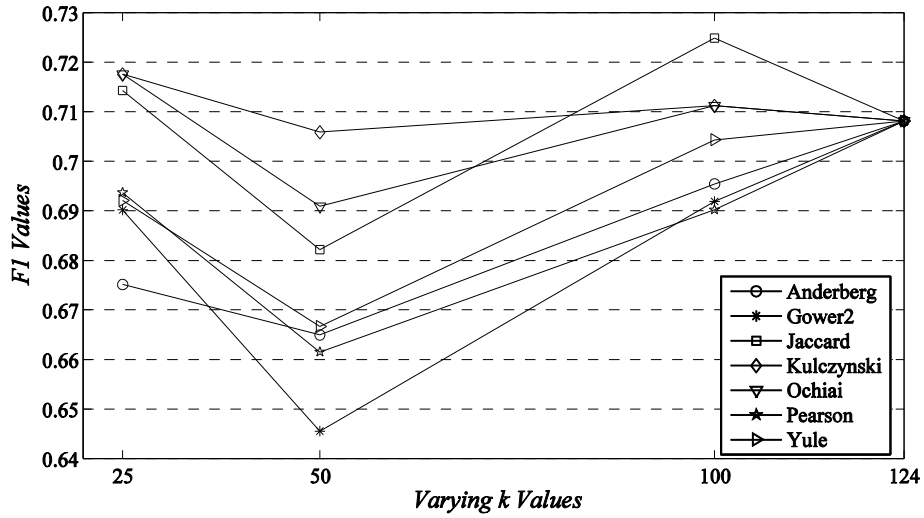
Figure 9. F1 values with varying k values (ML & n = 124 )
