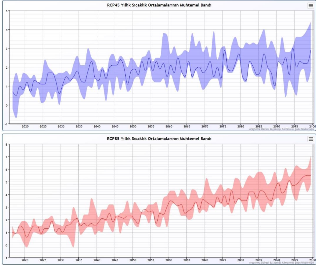
Figure 2.1. Average Temperature Change Projections Between the Period of 2016-2100 for Turkey according to RCP4.5 and RCP8.5 emission scenarios (General Directorate of Meteorology, 2020)
