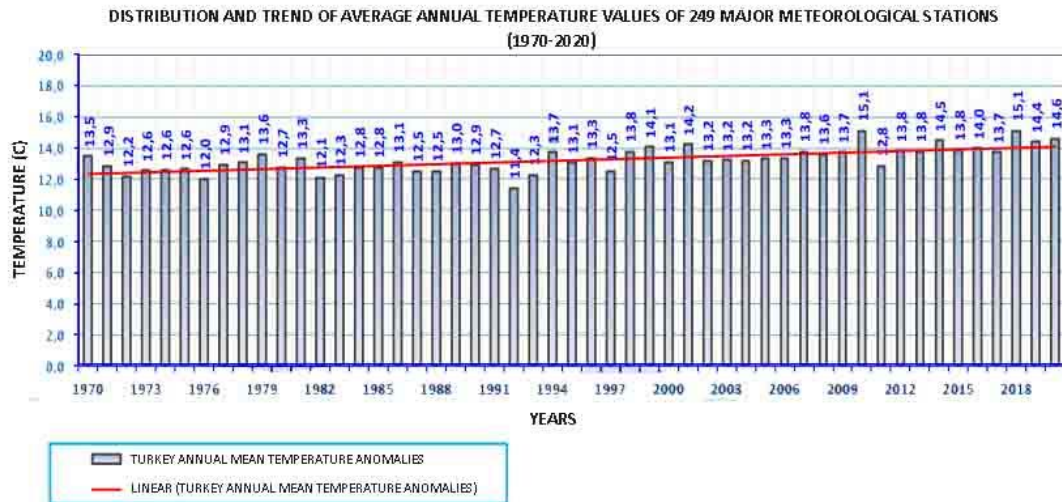
Figure 1.3. Turkey annual mean temperature anomalies between 1970 - 2020 (General Directorate of Meteorology,2021)
