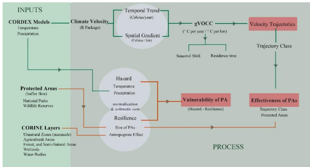
Figure 3.1. Data and Methodology flowchart that used in study
