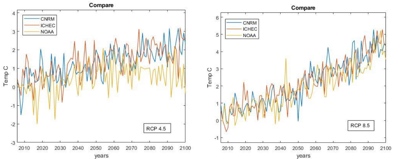
Figure 3.3. Comparison of 3 CORDEX models future scenarios regarding RCP4.5 and RCP8.5
