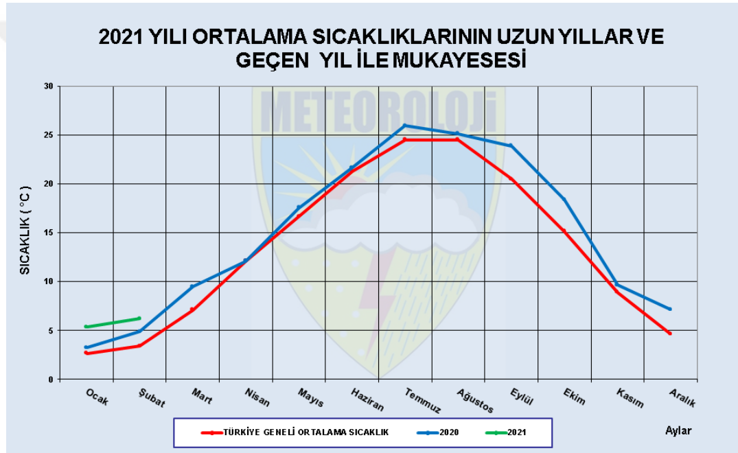
Figure 1.4. 2021 and past years average monthly temperature anomalies (General Directorate of Meteorology,2021)
