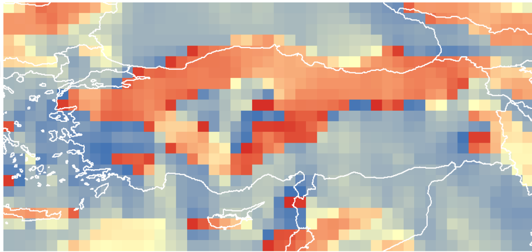
Figure 3.14. The angle of velocity of climate change for the 2000-2100 period.
