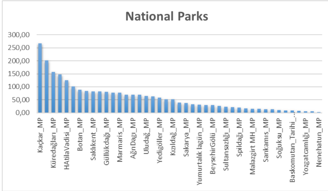
Figure 4.7. Residence Time of National Parks from higher to lower (diameter of the equivalent circle (km), and residence time (years) as the ratio D/v_{el} )
