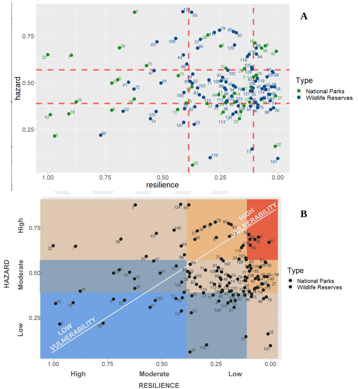
Figure 4.5. Vulnerability of Protected Areas in Turkey. Graph A shows National Parks (green) and Wildlife Reserves (blue) vulnerability level. Graph B shows the vulnerability classes that divided into five according to quartiles
