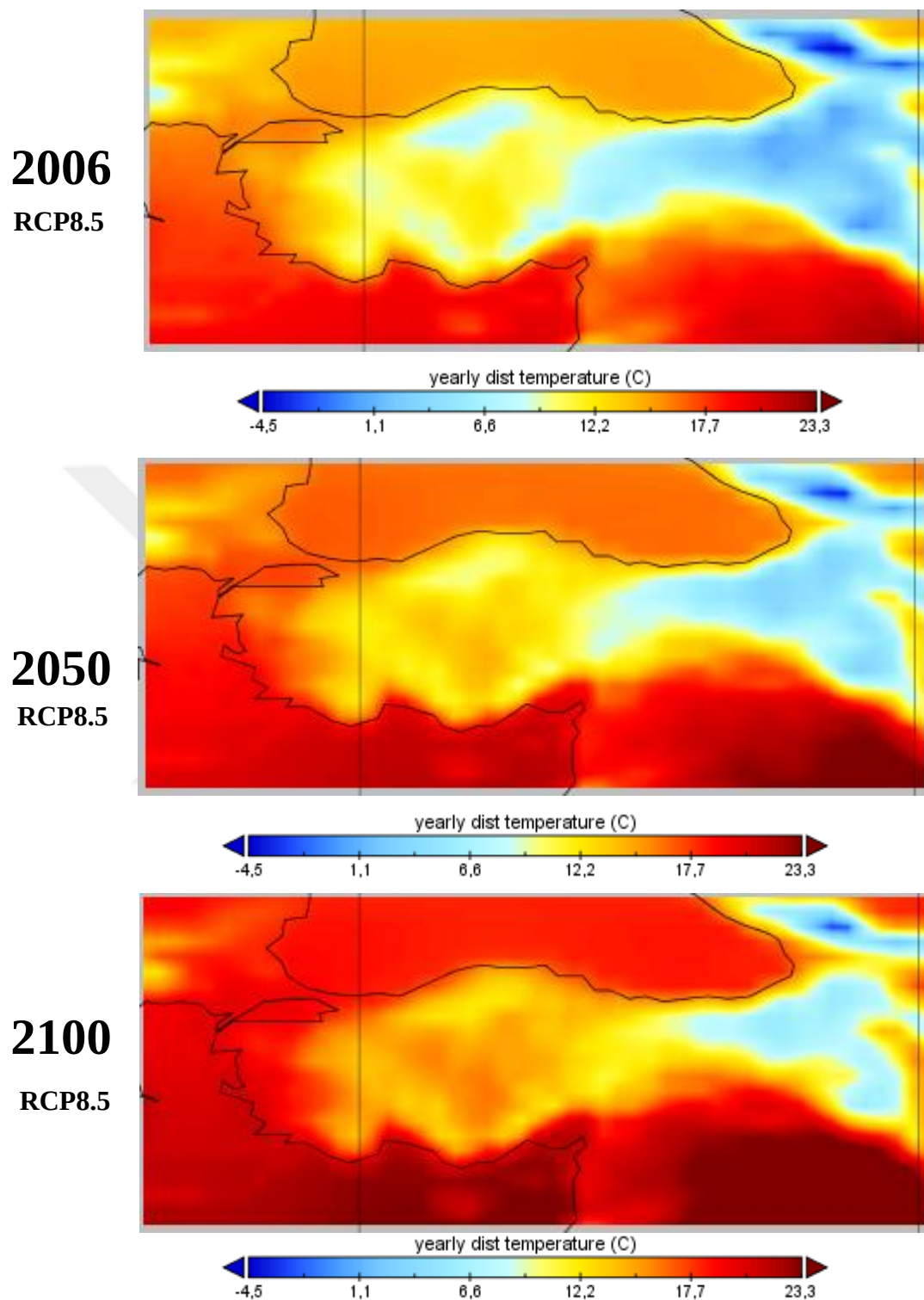
Figure 3.8. ICHEC-EC-EARTH Annual Average Temperature
