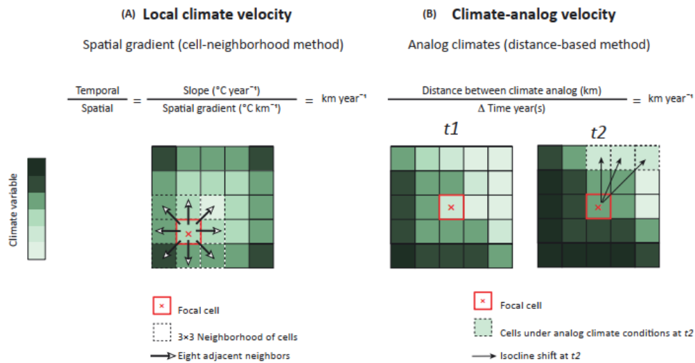
Figure 2.3. Calculation of (A) Local Climate / Gradient based and (B) Climate-Analog Velocities / Distance based (Brito-Morales et al, 2018).
