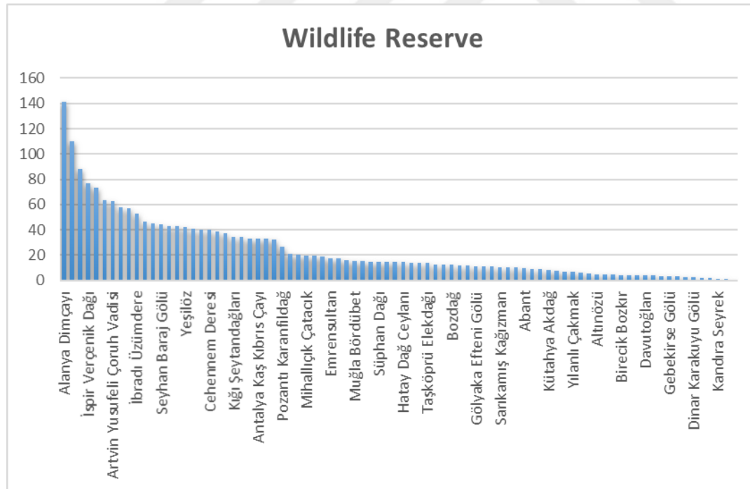
Figure 4.8. Residence Time of Wildlife Reserves from higher to lower (diameter of the equivalent circle (km), and residence time (years) as the ratio D/v_{el} )
