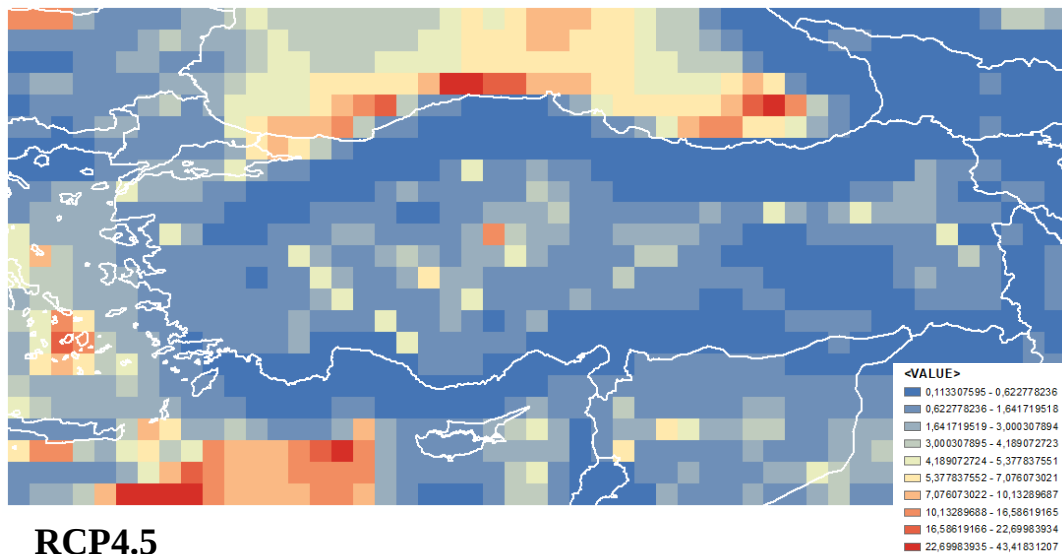
Figure 3.14. The angle of velocity of climate change for the 2000-2100 period.
