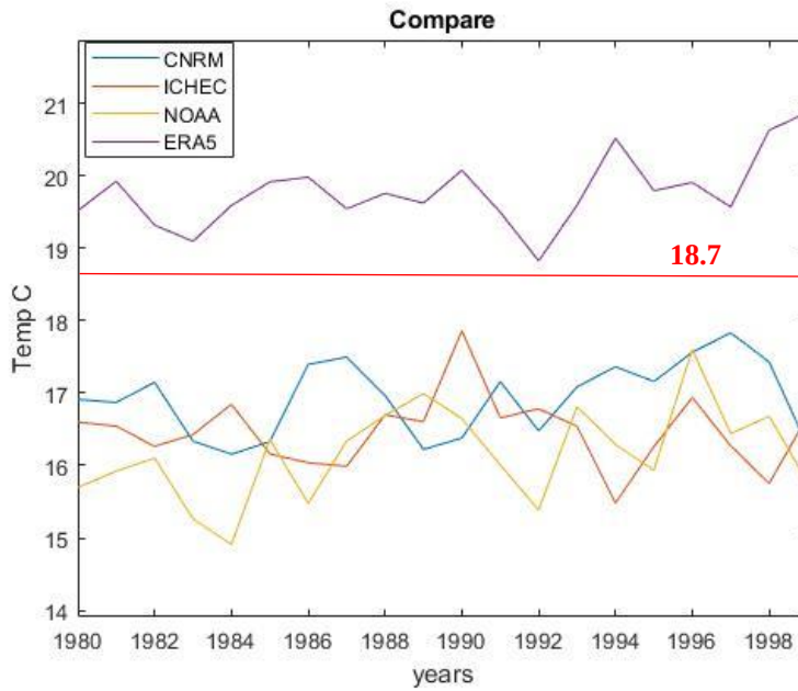
Figure 3.2. Comparison of the annual temperatures from ERA5, CORDEX models, and Meteorological Station in a historical period between 1980-2000
