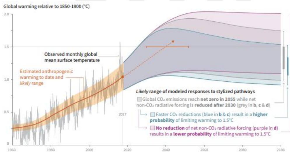
Figure 1.1. Observed global temperature change and modeled responses to stylized anthropogenic emission and forcing pathways (Source: IPCC Report)
