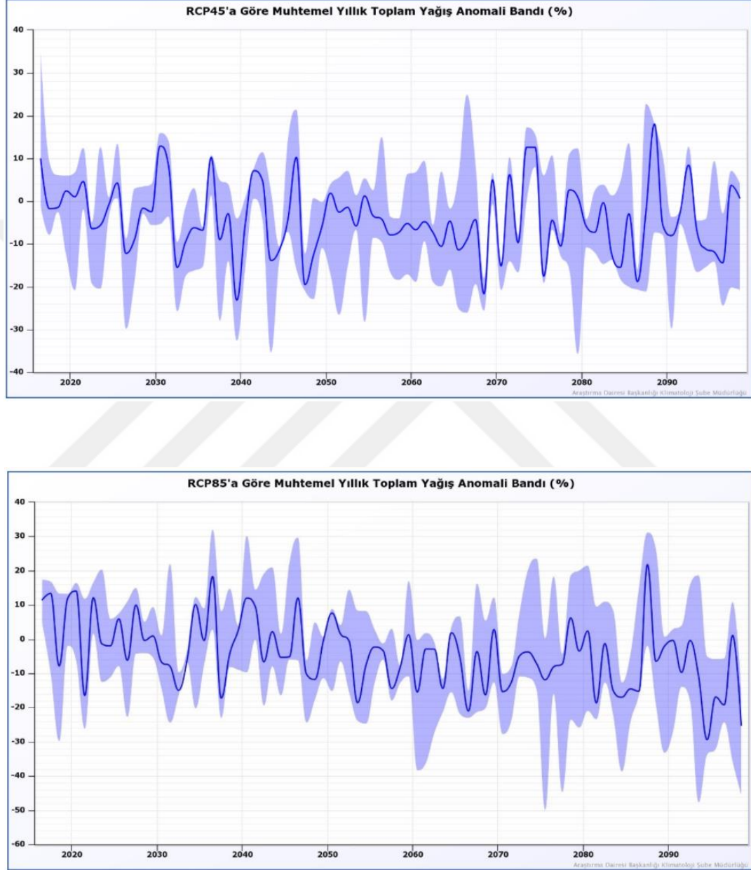
Figure 2.2. Turkey RCP4.5 and RCP8.5 Average Precipitation Change Projections Between the Period of 2016-2100 (General Directorate of Meteorology, 2020)
