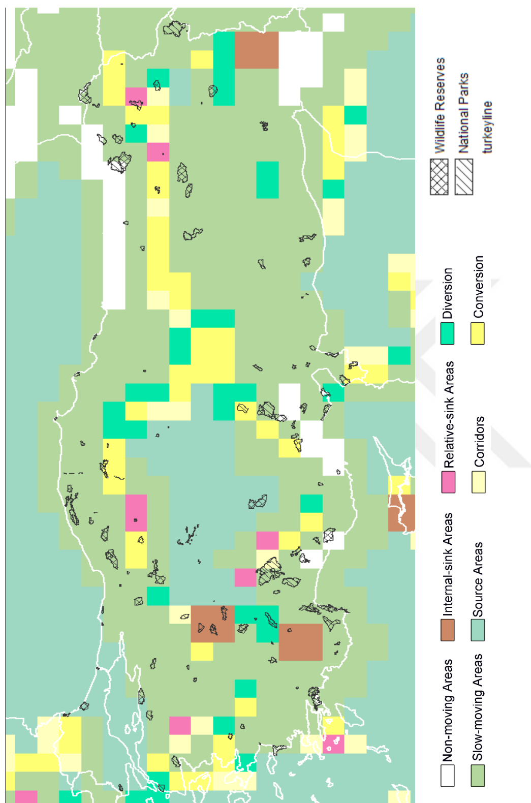
Figure 4.6. Protected Areas with trajectory classes
