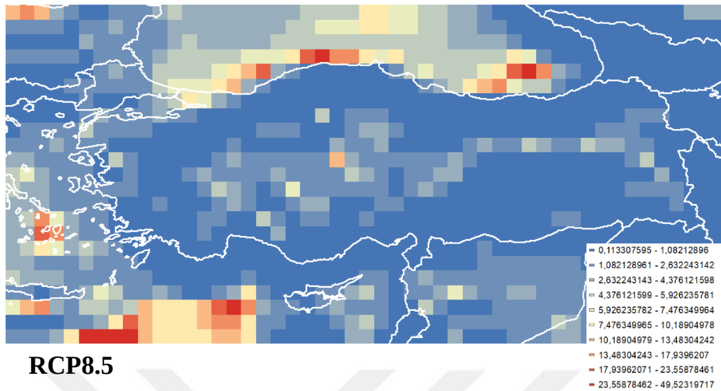
Figure 3.15. According to CNRM-CERFACS-CNRM-CM5-Cordex Model, Magnitude velocity of climate change for 2000-2100 period (km/yr) for RCP 4.5 and RCP8.5 emission scenarios. Colors (blue: lower, red: higher) show degree level which form base angle for velocity trajectories.
