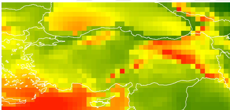
Figure 4.10. Spring seasonal shift is shown for April. A shows spring seasonal rate of temperature change (C/ month). B shows seasonal shift for April (day/decade)
