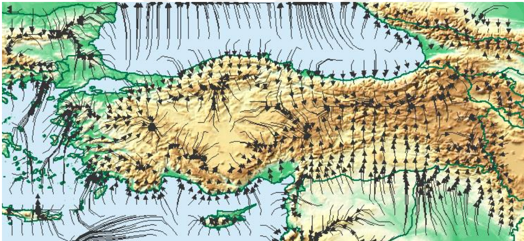
Figure 4.3. The elevation map of Turkey with velocity trajectories. Arrows represent trajectories that computed as regards velocity level.
