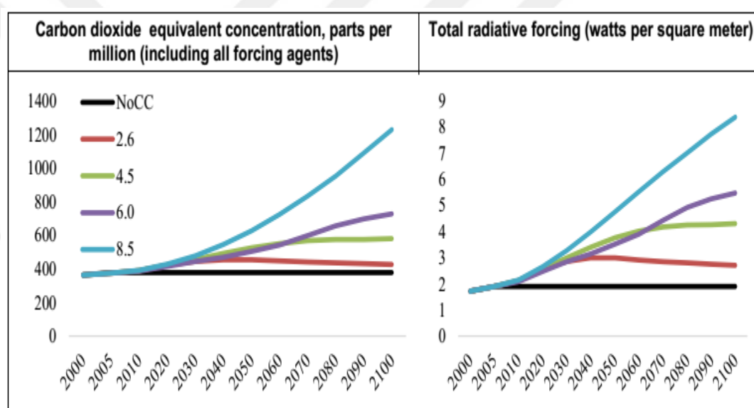
Figure 1.8. Probable \text{CO}_2 concentration and radiative forcing by RCP
