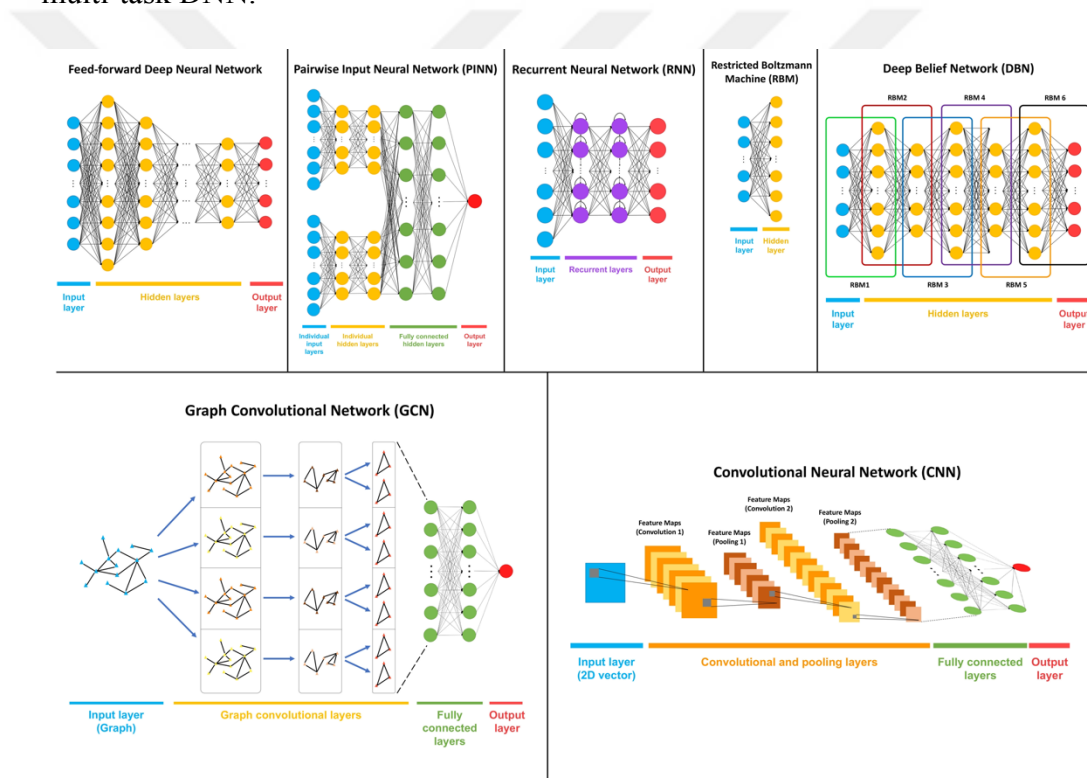
Figure 2.3. Schematic representations of different deep neural network (DNN) architectures frequently used in the literature (Adapted from our publication [7]).
