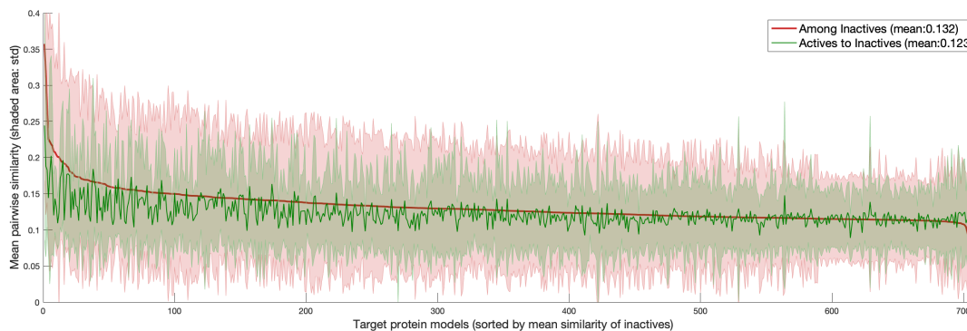
Figure 4.3. Target-based (x-axis) average pairwise compound similarity (y-axis) curves for intra-group (among inactives) and inter-group (actives to inactives) similarities with error bands for 704 DEEPScreen targets.
