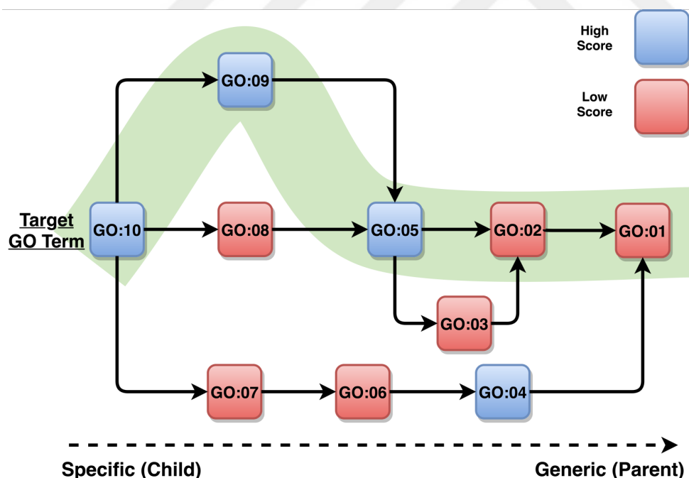
Figure 3.3. Post-processing of a prediction (GO:10) for a query protein sequence on a hypothetical GO DAG. Each box corresponds to a different GO term, with identification numbers written inside. The blue colored boxes represent GO terms
