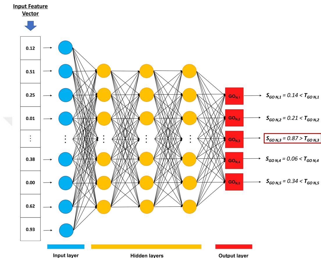
Figure 3.1. The representation of an individual multi-task feed-forward DNN model of DEEPred. Here, each task at the output layer (i.e., red squares) corresponds to a different GO term. In the example above, a query input vector is fed to the trained model N and a score greater than the pre-defined threshold is produced for GO_{N,3} , which is marked as a prediction. (Adapted from our publication [191])
