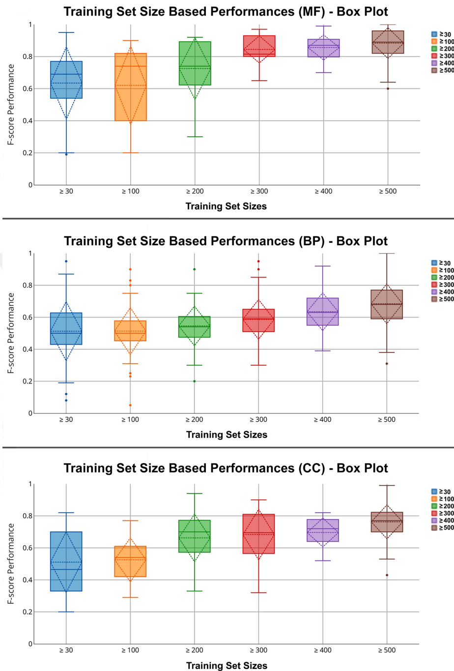
Figure 3.4. Box plots for training dataset size specific performance evaluation. Each box plot represents variance, mean and standard deviations of F1-score values (vertical axis) for models with differently sized training datasets (horizontal axis),
