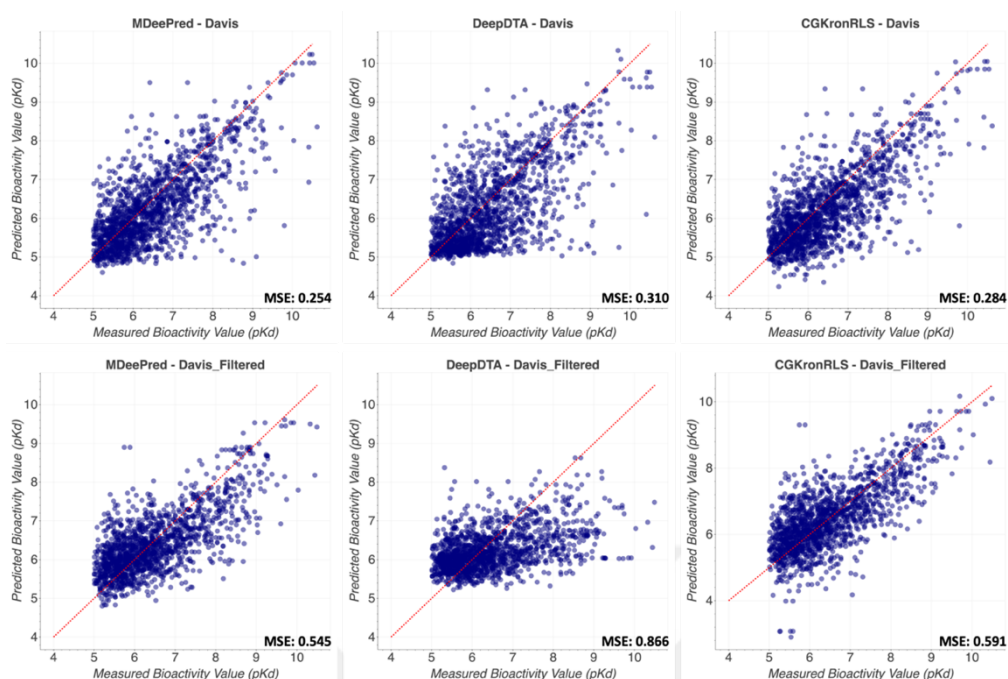
Figure 5.3. Measured (true) vs. predicted binding affinity plots for MDDeePred, DeepDTA and CGKronRLS, on Davis and the filtered Davis datasets
