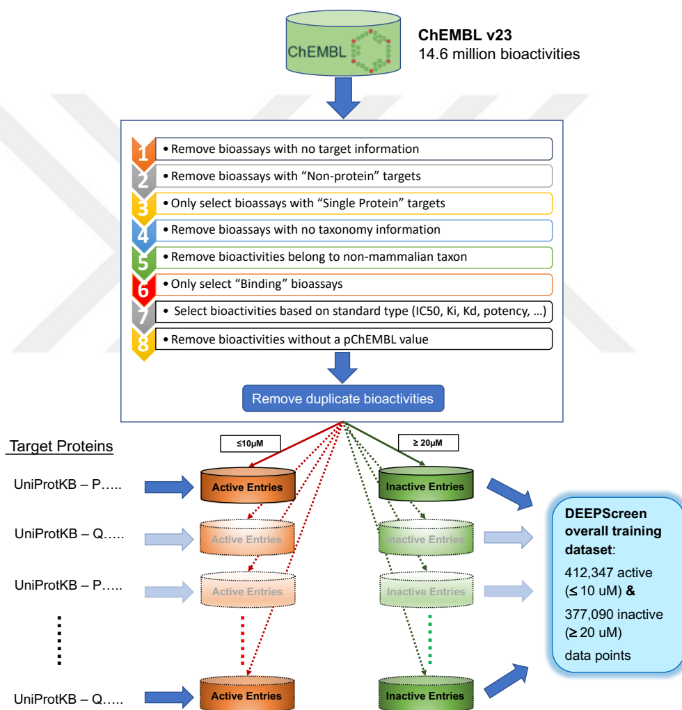
Figure 4.1. Data filtering and processing steps to create the training dataset of each target protein model. Predictive models were trained for 704 target proteins, each of which have at least 100 known active ligands in the ChEMBL database.
