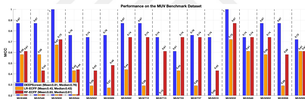
Figure 4.5. Predictive Performance evaluation and comparison of DEEPScreen against the state-of-the-art DTI prediction approaches, on scaffold-split benchmarks: (a) Bar plots of MCC values on representative targets dataset; (b) Bar plots of MCC values on the MUV dataset.
