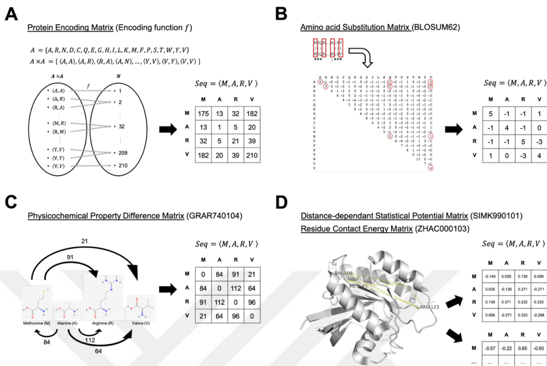
Figure 5.1. Construction of multi-channel input protein feature vectors for an example of 4 amino acid peptide sequence: "M A R V", using the protein encoding matrix (a), substitution scoring matrix (b), physicochemical property difference matrix (c), statistical potential and residue contact energy matrices (d). For the channels except the protein encoding, corresponding 20-by-20 AAindex matrices are used to construct 500-by-500 or 1000-by-1000 2-D feature matrix of the input proteins.
