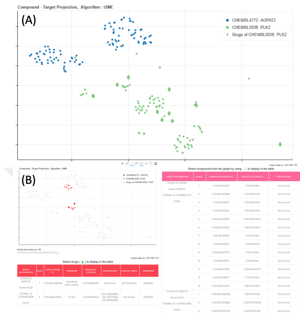
Figure 6.1. Interactive output of the iBioProVis framework. (A) Embedding output without user selection. (B) The same embedding output (including tables) after user selection of compounds. Visual clusters and the nodes in close vicinity may indicate the same or similar target proteins.
