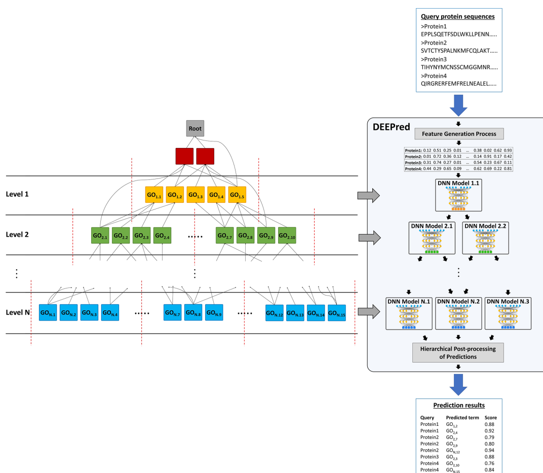
Figure 3.2. Illustration of the GO-level-based architecture of DEEPred on a simplified hypothetical GO DAG. We omitted highly generic GO terms (shown with red colored boxes) at the top of the GO hierarchy (e.g., GO:0005488 - Binding) from our models, since they are less informative and their training datasets are highly
