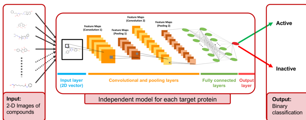
Figure 4.2. Illustration of the deep convolutional neural network structure of DEEPScreen, where the sole input is the 2-D structural images of the drugs and drug candidate compounds (generated from the SMILES representations as a data pre-processing step). Each target protein has an individual prediction model with specifically optimized hyper-parameters (please refer to the Methods section). For each query compound, the model produces a binary output either as active or inactive, considering the interaction with the corresponding target.
