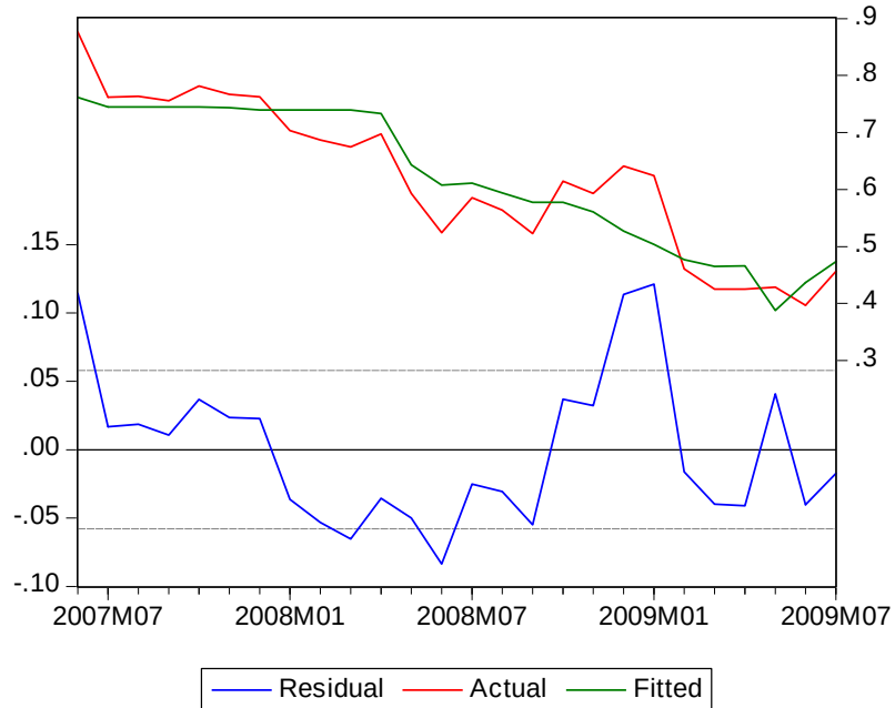
Figure 17: Graph of Residuals, Actual and Fitted Line
