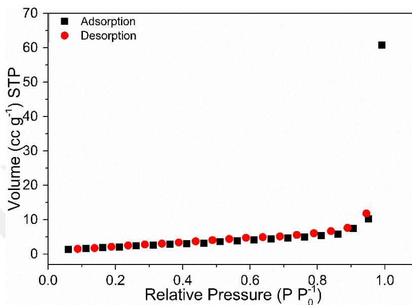
Figure A.1. N 2 adsorption – desorption isotherm of CuCr 2 O 4 nanoparticles
