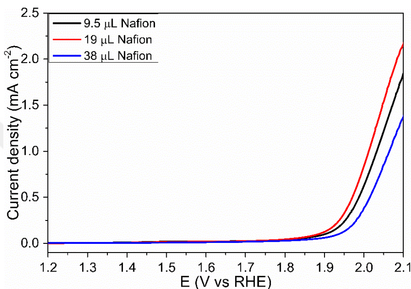
Figure B.1. Polarization curves of \text{CuCr}_2\text{O}_4 nanoparticles with different amount of Nafion ® in 0.1 M KOH at a scan rate of 5 \text{ mV s}^{-1}
