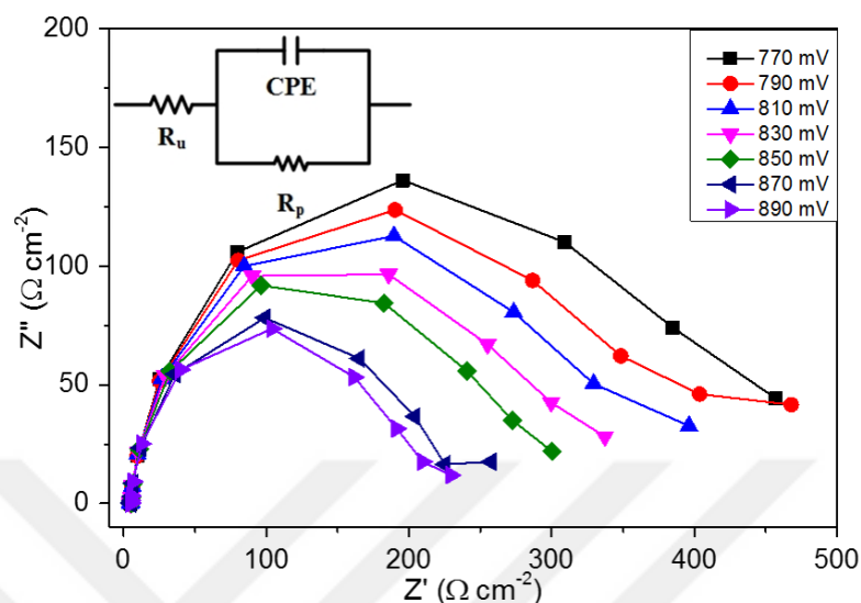
Figure 5.30. Nyquist plots of \text{CuCr}_2\text{O}_4 nanoparticles at various overpotential values in 0.1 M KOH
