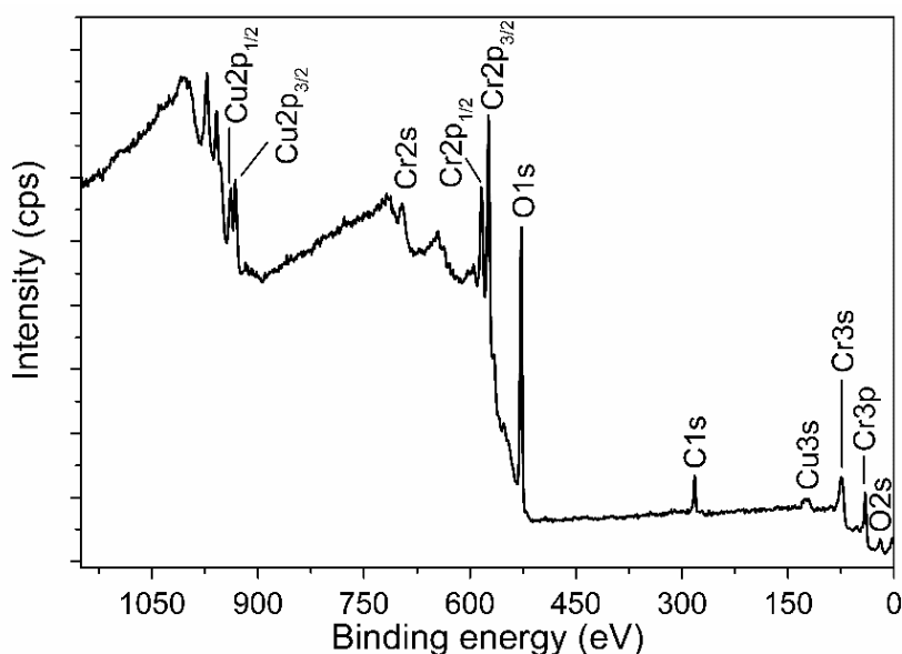
Figure 5.5. XPS survey spectrum of CuCr 2 O 4 nanoparticles
