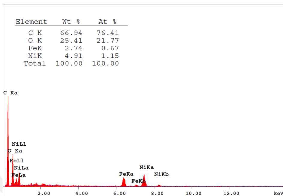
Figure 5.15. EDX spectrum of \text{NiFe}_2\text{O}_4\text{-NiO} nanoparticles
