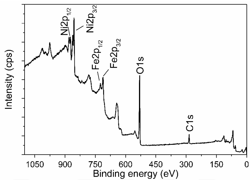
Figure 5.17. XPS survey spectrum of NiFe 2 O 4 -NiO nanoparticles
