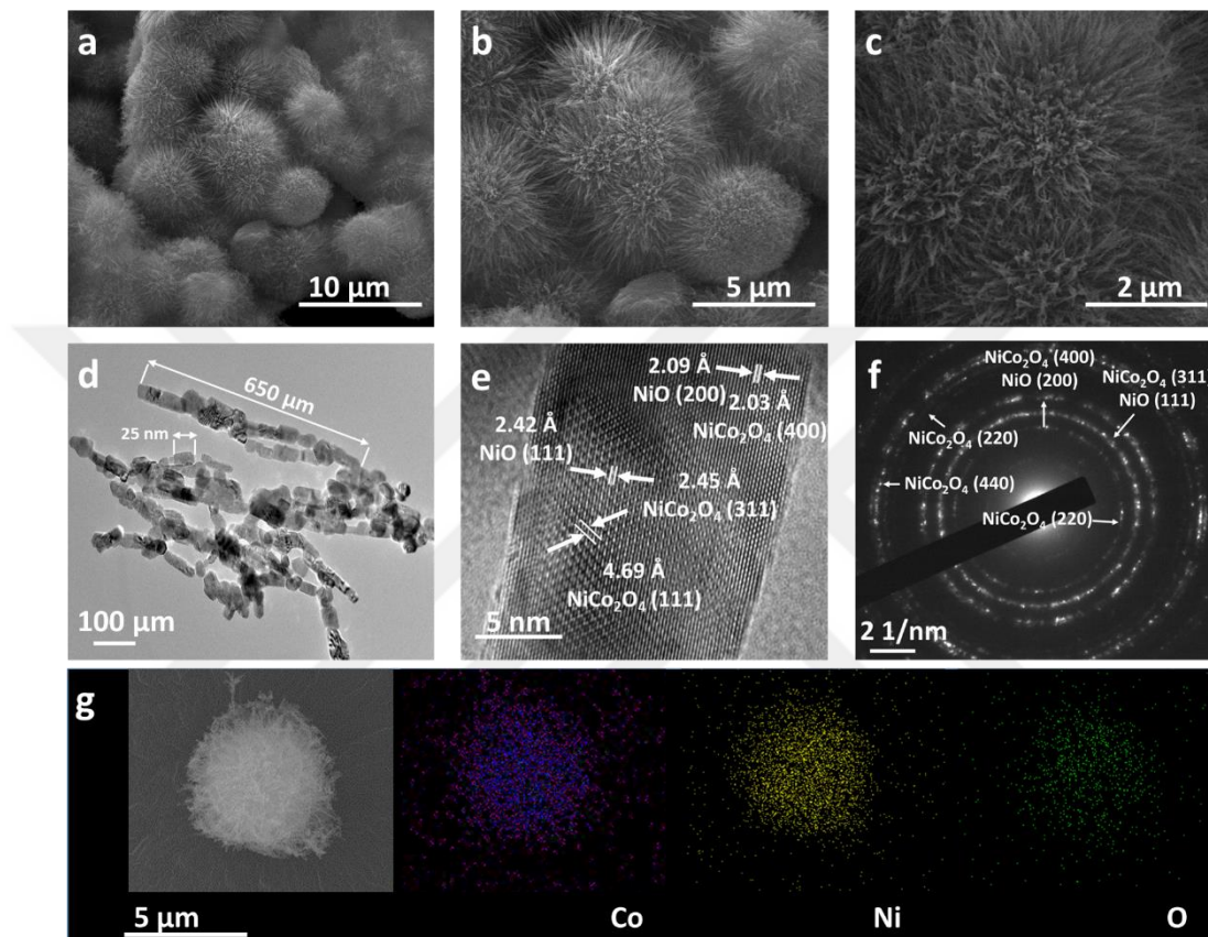
Figure 5.21. (a-c) SEM and (d-e) TEM images at different magnification, (f) SAED pattern and (g) Element mapping (Co (blue), Ni (yellow), O (green)) of U-NiCo microspheres
