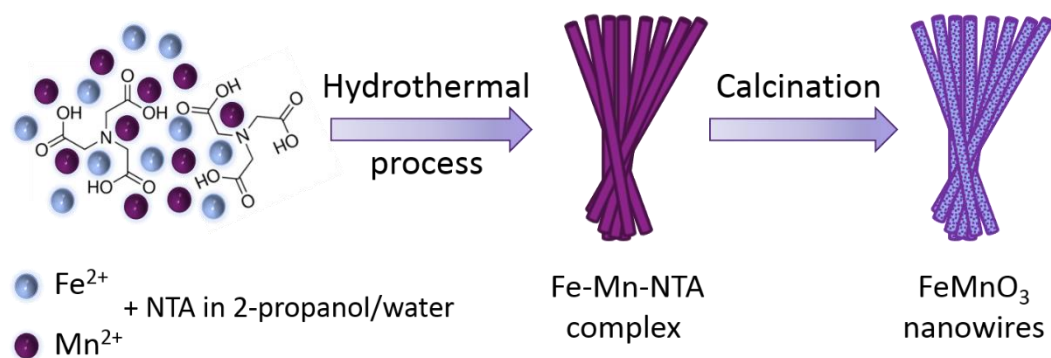
Figure 5.7. Illustration for the formation of FeMnO 3 nanowires
