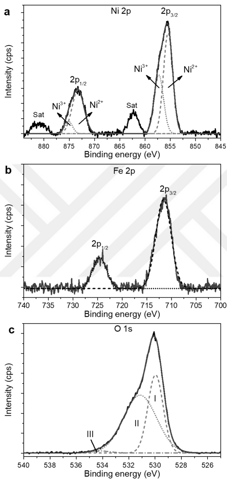
Figure 5.18. XPS (a) Ni 2p, (b) Fe2p and (c) O 1s spectra \text{NiFe}_2\text{O}_4\text{-NiO} nanoparticles
