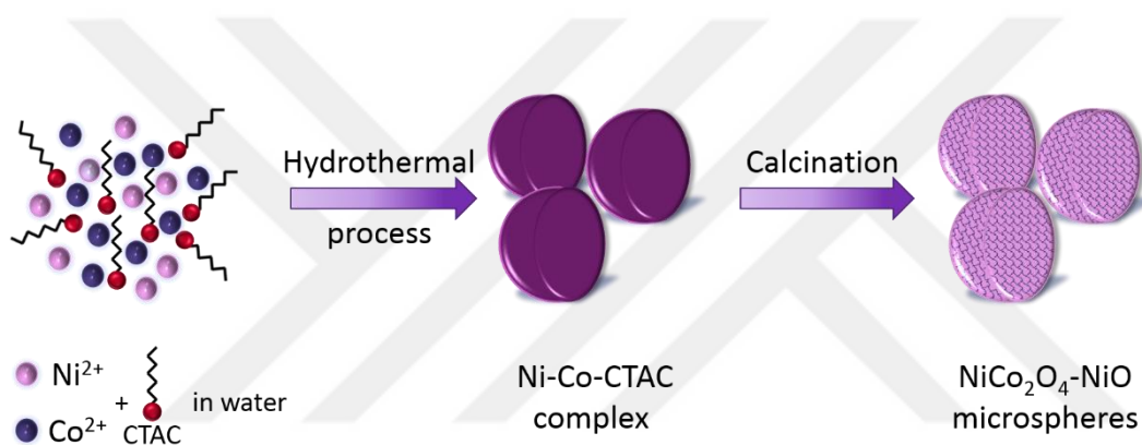
Figure 5.20. Illustration for the formation of CTAC stabilized \text{NiCo}_2\text{O}_4 -NiO microspheres
