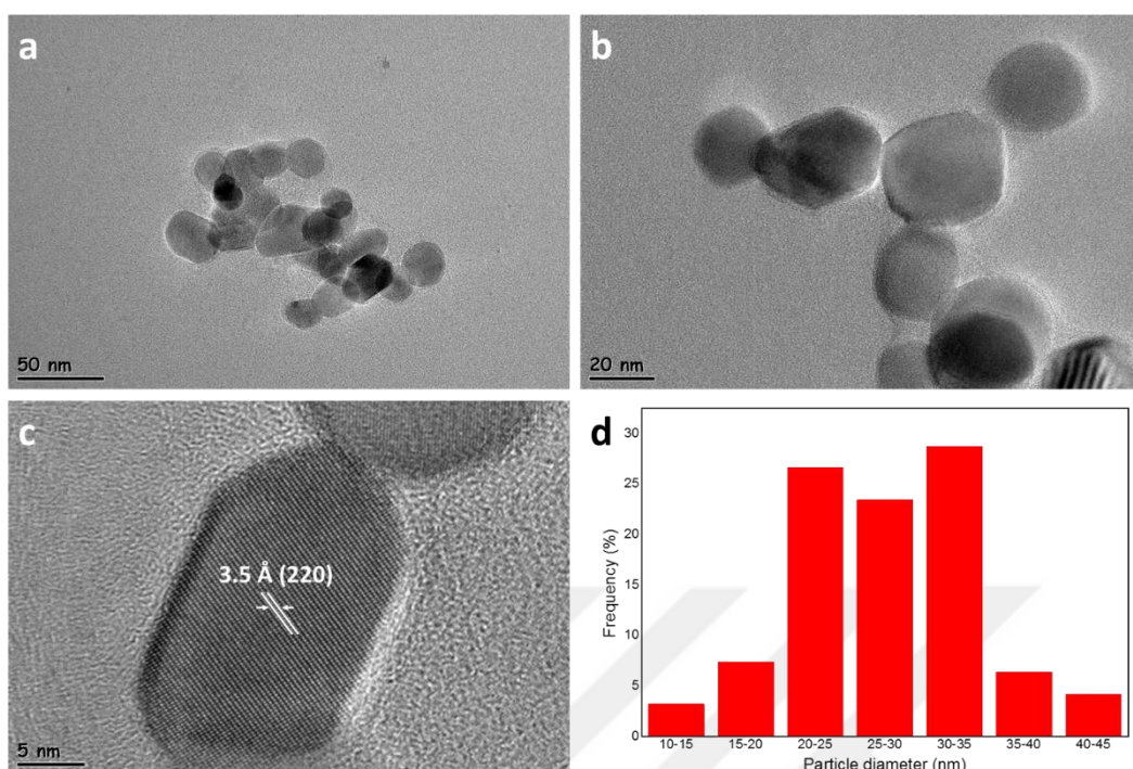
Figure 5.2. (a-c) TEM images and (d) particle size distribution graph of \text{CuCr}_2\text{O}_4 nanoparticles
