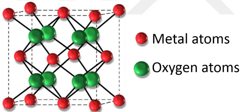
Figure 2.4. Unit cell of fluorite structure (green circles: oxygen atoms, red circles: transition metal atoms)
