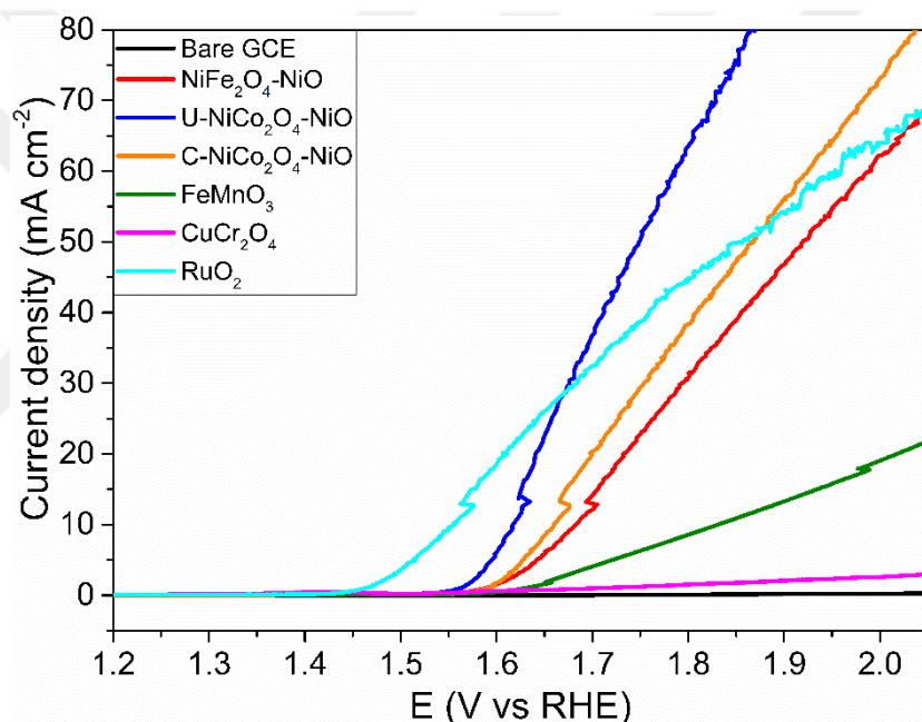
Figure 5.48. Polarization curves of bare GCE, \text{CuCr}_2\text{O}_4 nanoparticles, \text{FeMnO}_3 nanowires, \text{NiFe}_2\text{O}_4\text{-NiO} nanoparticles, \text{NiCo}_2\text{O}_4\text{-NiO} microspheres and \text{RuO}_2 in 0.1 M KOH solution at a scan rate of 5 \text{ mV s}^{-1}
