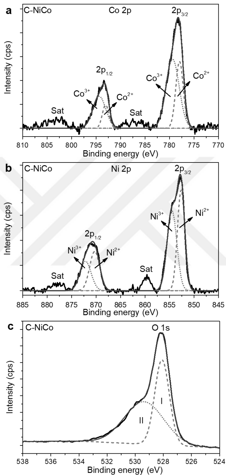
Figure 5.28. XPS (a) Co 2p, (b) Ni 2p and (c) O 1s spectra of C-NiCo microspheres
