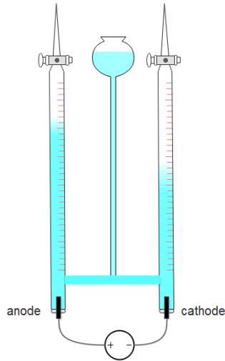
Figure 4.3. Schematic representation of a Hoffmann electrolysis apparatus
