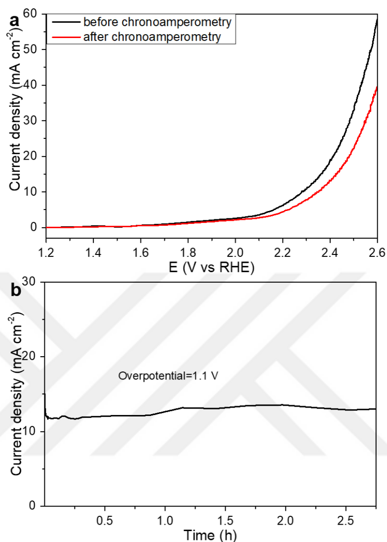
Figure 5.32. (a) Polarization curves before and after chronoamperometric electrolysis at \eta=1.1 V and (b) the change current density during chronoamperometry
