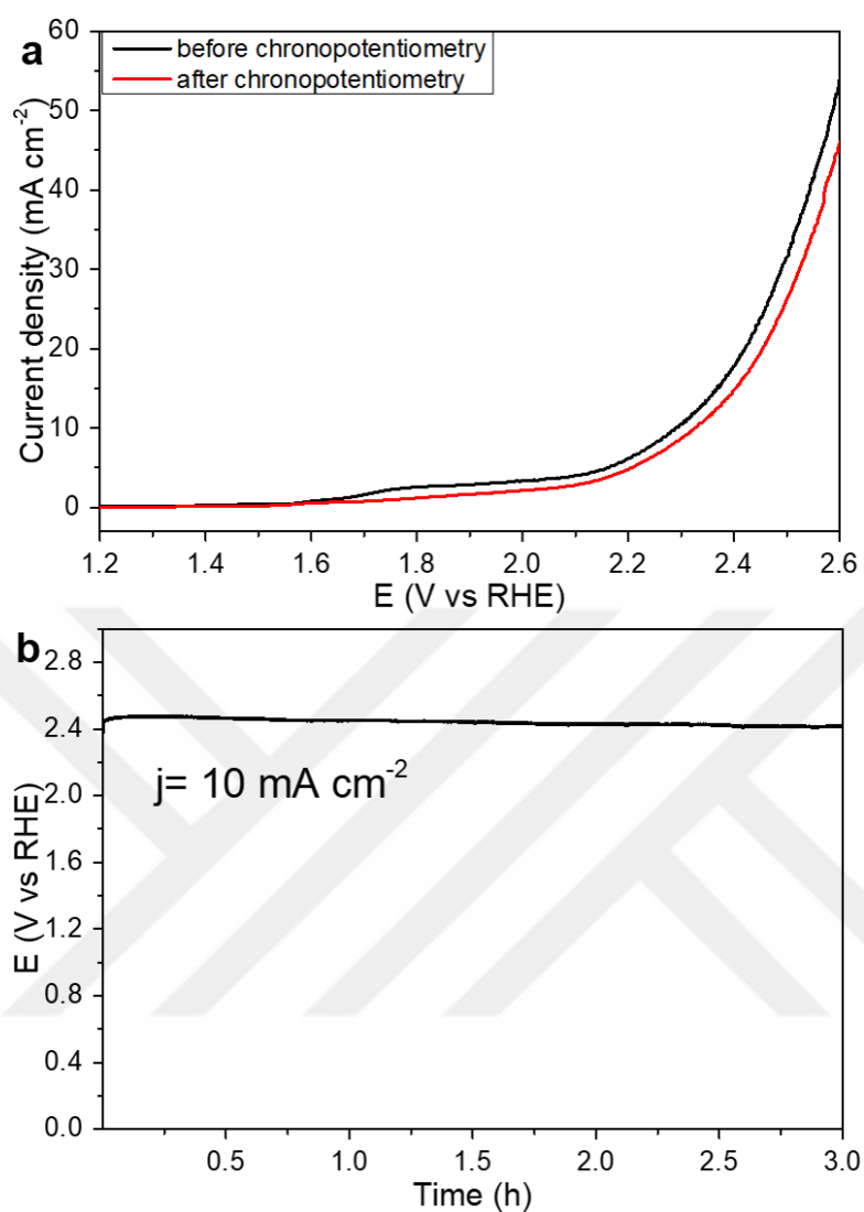
Figure 5.31. (a) Polarization curves before and after chronopotentiometric electrolysis at j=10 \text{ mA cm}^{-2} and (b) the change in potential during chronopotentiometry in 0.1 M KOH
