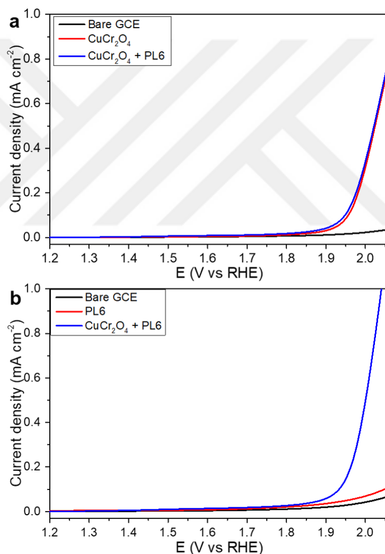
Figure B.2. Polarization curves of bare GCE, \text{CuCr}_2\text{O}_4 nanoparticles and \text{CuCr}_2\text{O}_4 nanoparticles mixed with PL6 in 0.1 M KOH at a scan rate of 5 \text{ mV s}^{-1}
