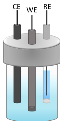
Figure 4.2. Schematic representation of a standard three-electrode system used for the electrochemical studies of electrodes modified with nanomaterials
