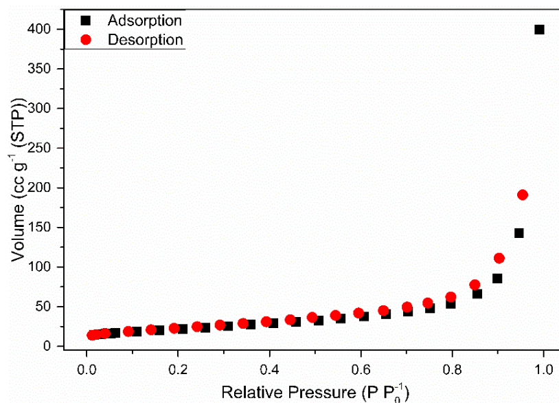
Figure A.2. N 2 adsorption – desorption isotherm of NiFe 2 O 4 -NiO nanoparticles
