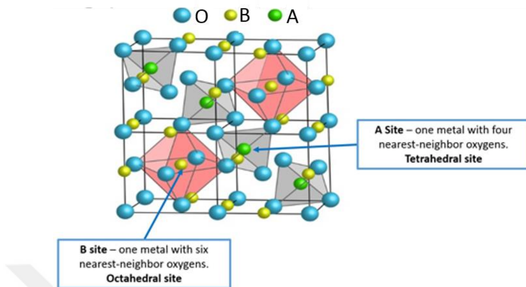
Figure 2.7. Unit cell of spinel structure (green circles: A cations, yellow circles: B cations and blue circles: oxygen atoms)
