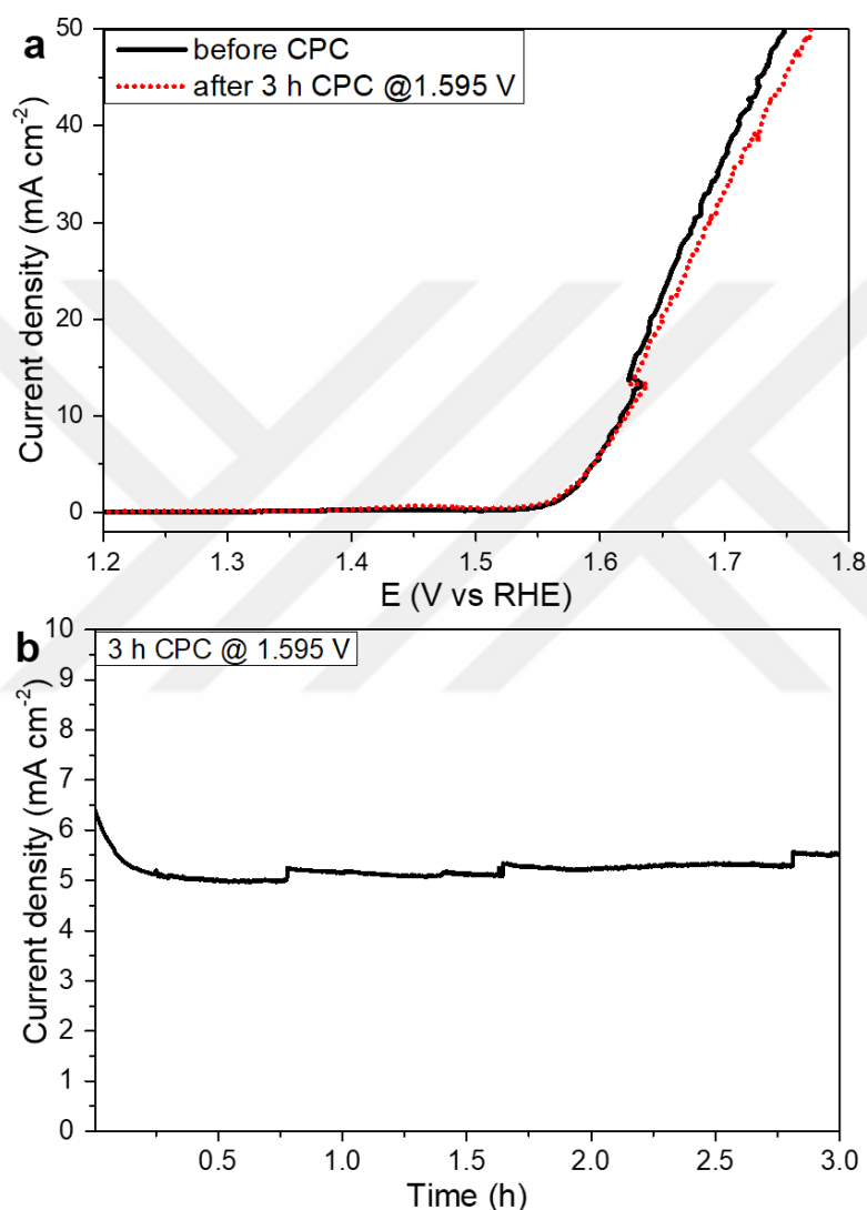
Figure 5.46. (a) Polarization curves of U-NiCo microspheres recorded before and after controlled potential electrolysis at overpotential corresponding to initial current density of 5 \text{ mA cm}^{-2} and (b) The change in current density during electrolysis in 0.1 \text{ M KOH}
