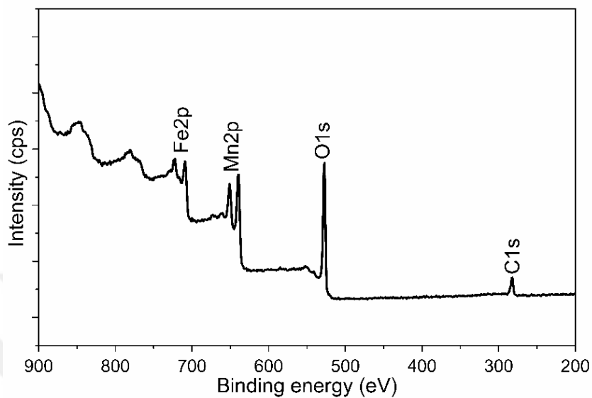
Figure 5.11. XPS survey spectrum of FeMnO 3 nanowires
