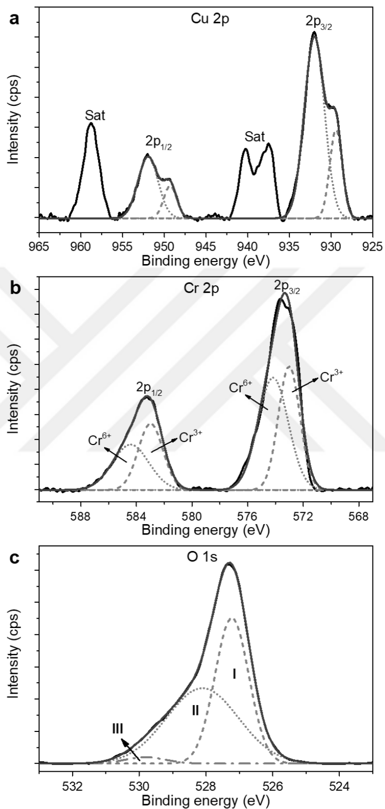
Figure 5.6. XPS (a) Cu 2p, (b) Cr 2p and (c) O 1s spectra of \text{CuCr}_2\text{O}_4 nanoparticles
