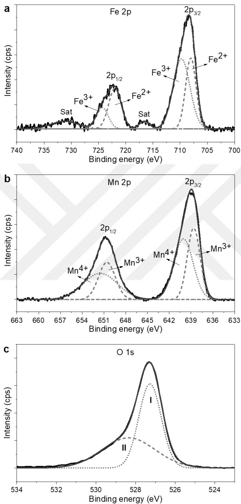
Figure 5.12. XPS (a) Fe 2p, (b) Mn 2p and (c) O 1s spectra of FeMnO_3 nanowires
