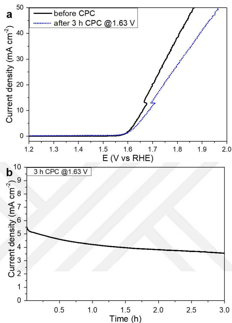
Figure 5.47. (a) Polarization curves of C-NiCo microspheres recorded before and after controlled potential electrolysis at overpotential corresponding to initial current density of 5 \text{ mA cm}^{-2} and (b) The change in current density during electrolysis in 0.1 M KOH
