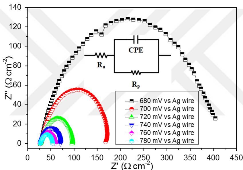
Figure 5.35. Nyquist plots for the FeMnO 3 -FTO electrodes at different overpotentials
