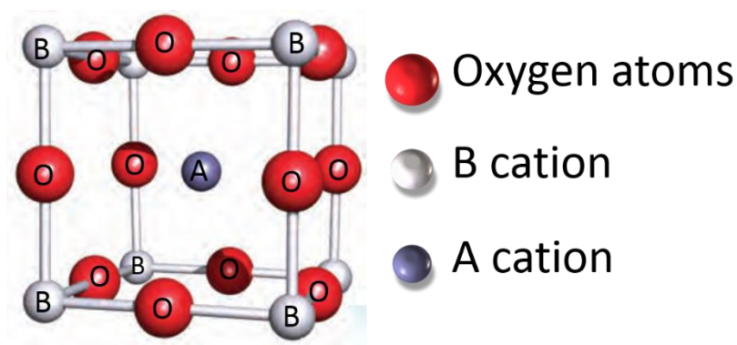
Figure 2.8. Unit cell of perovskite ( \text{ABO}_3 ) structure (red circles: oxygen atoms, purple circle: A cation and pale grey circles: B cations) (modified from 34 )
