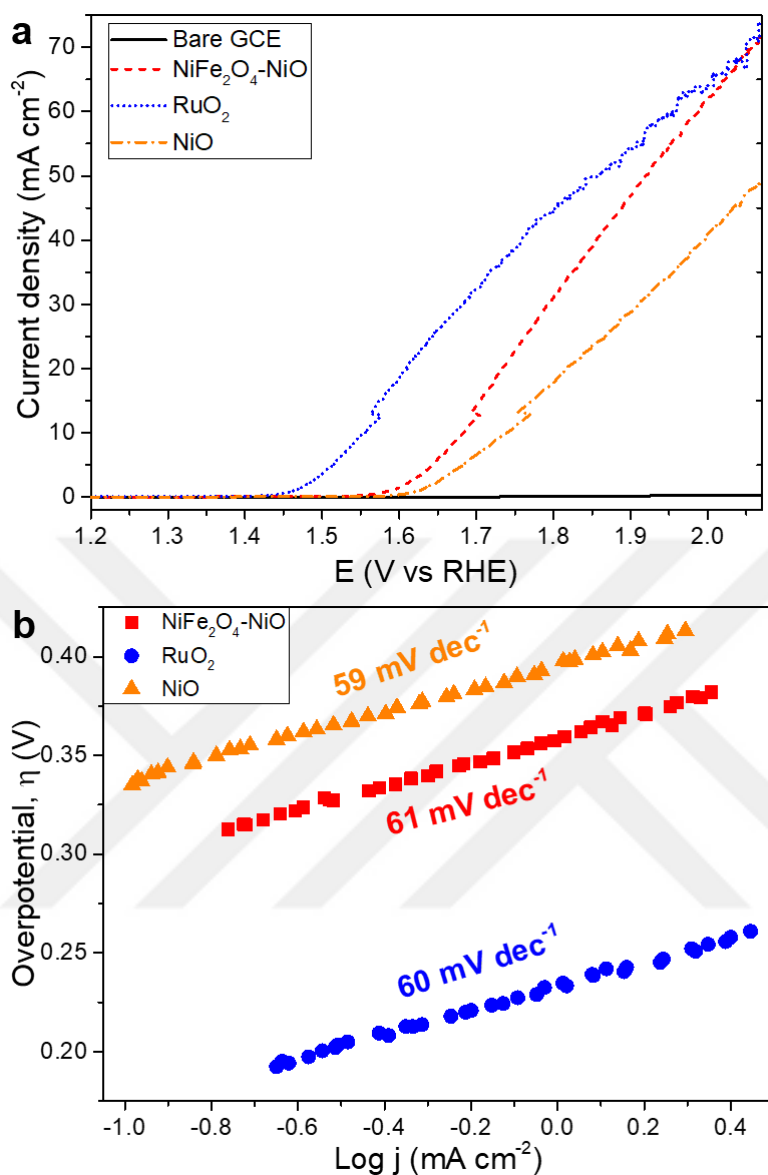
Figure 5.38. (a) Polarization curves of bare GCE, NiFe 2 O 4 -NiO nanoparticles, NiO and RuO 2 in 0.1 M KOH at a scan rate of 5 mV s -1 and (b) The corresponding Tafel plot obtained from polarization curves
