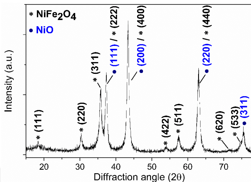
Figure 5.16. XRD pattern of \text{NiFe}_2\text{O}_4 - \text{NiO} nanoparticles
