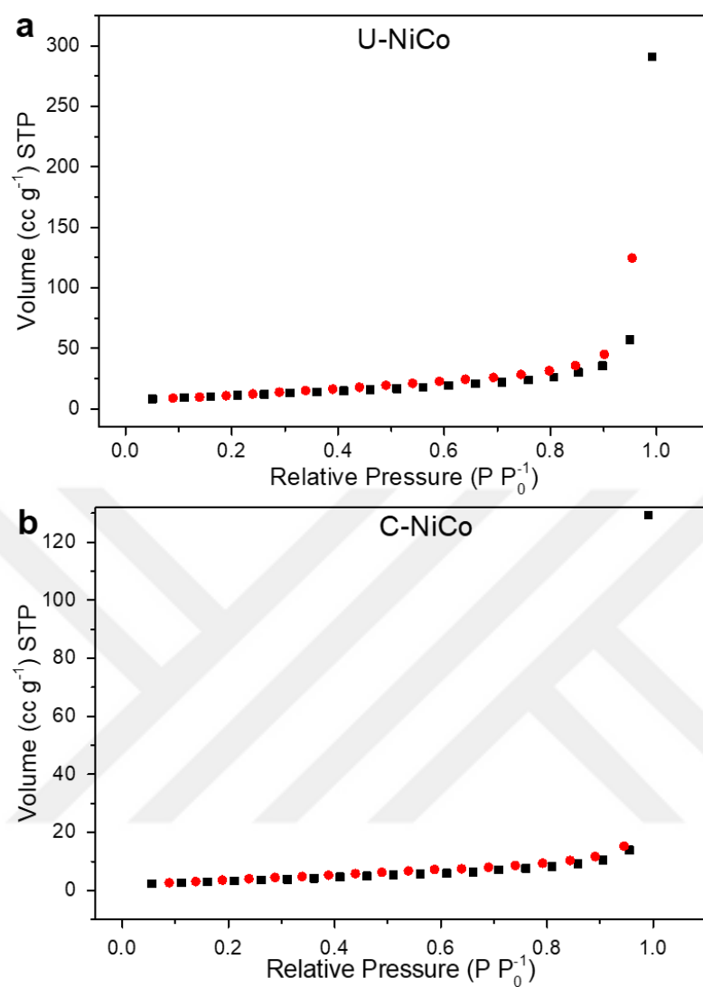
Figure A.3. N 2 adsorption – desorption isotherms of (a) U-NiCo and (b) C-NiCo microspheres
