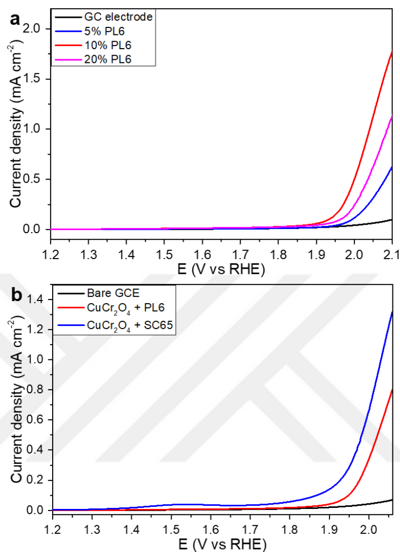
Figure B.3. Polarization curves of CuCr 2 O 4 nanoparticles obtained with (a) different carbon loadings and (b) different carbon materials in 0.1 M KOH at a scan rate of 5 mV s -1
