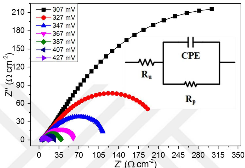
Figure 5.40. Nyquist plots of \text{NiFe}_2\text{O}_4/\text{NiO} nanoparticles at various overpotentials (inset shows the equivalent circuit diagram)
