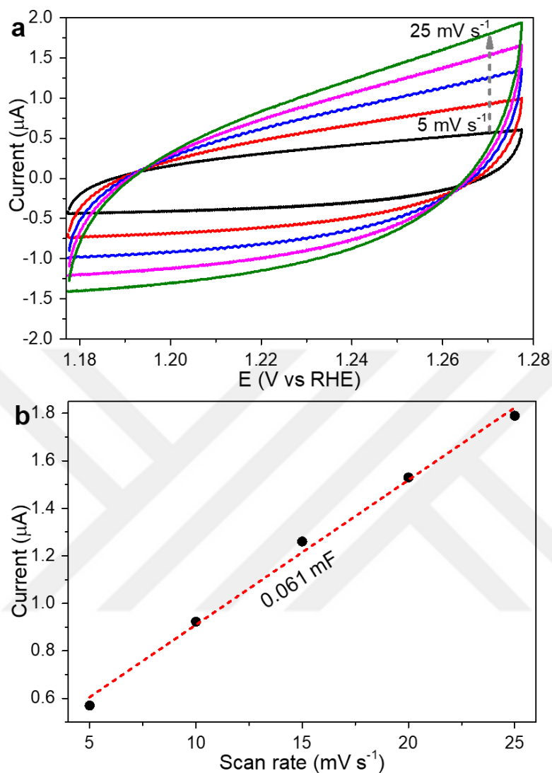
Figure 5.39. (a) CVs of NiFe 2 O 4 -NiO nanoparticles measured at different scan rate from 5 to 25 mV s -1 and (b) Plot of current at 1.27 V (vs RHE) vs scan rate
