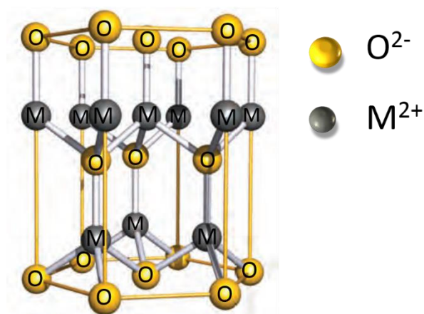
Figure 2.2. Unit cell of wurtzite structure (yellow circles: oxygen atoms, grey circles: transition metal atoms) (modified from 34 )
