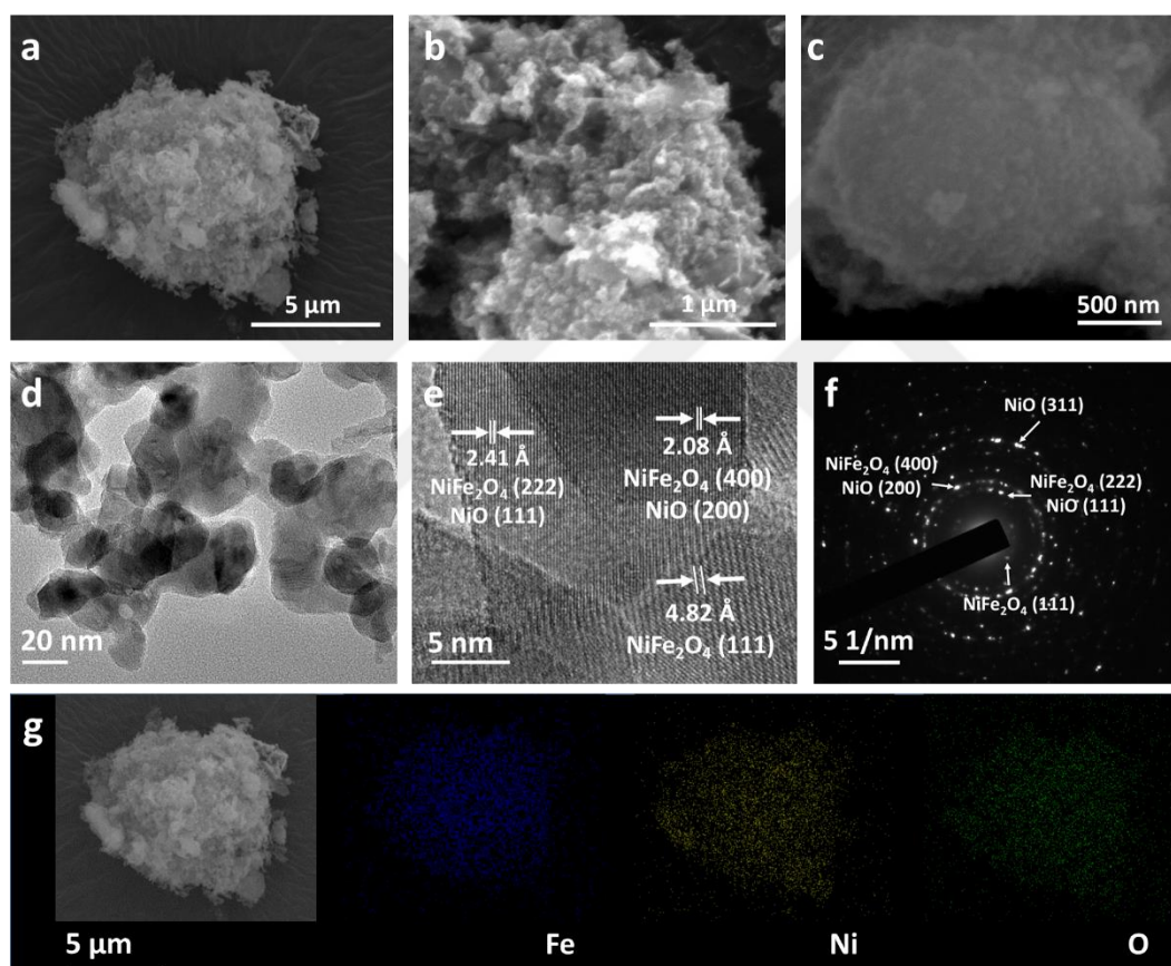
Figure 5.14. (a-c) SEM and (d-e) TEM images at different magnifications, (f) SAED pattern and (g) element mapping (Fe (blue), (Ni (yellow), O (green)) of \text{NiFe}_2\text{O}_4\text{-NiO} nanoparticles
