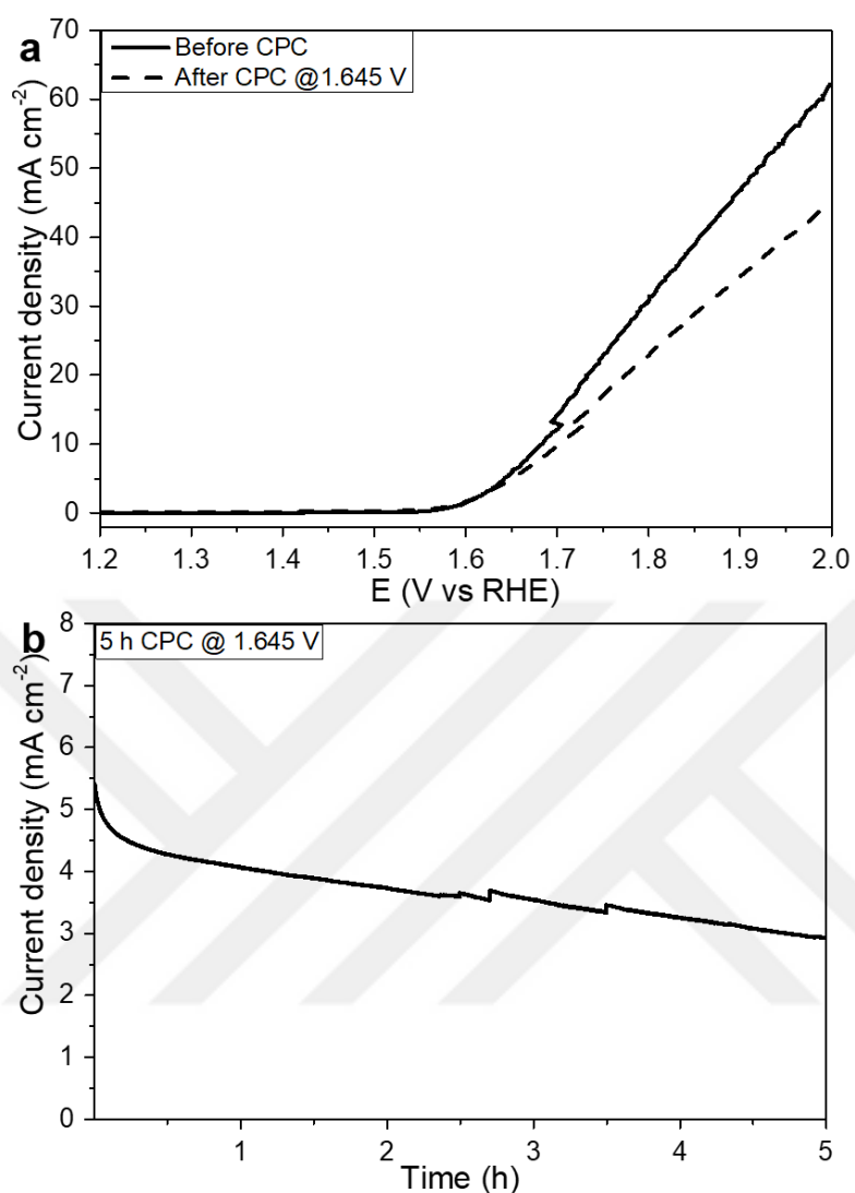
Figure 5.41. (a) Polarization curves of NiFe 2 O 4 -NiO nanoparticles recorded before and after controlled potential electrolysis at overpotential corresponding to initial current density of 5 mA cm -2 and (b) Change in current density during electrolysis in 0.1 M KOH
