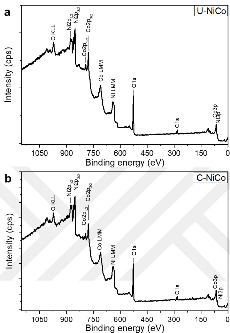
Figure 5.26. XPS Survey spectra of (a) U-NiCo and (b) C-NiCo microspheres
