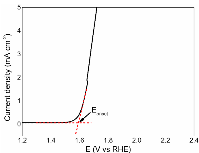
Figure 3.3. Determination of onset potential from a polarization curve
