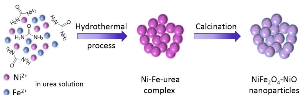
Figure 5.13. Illustration for the formation of \text{NiFe}_2\text{O}_4 -NiO nanoparticles
