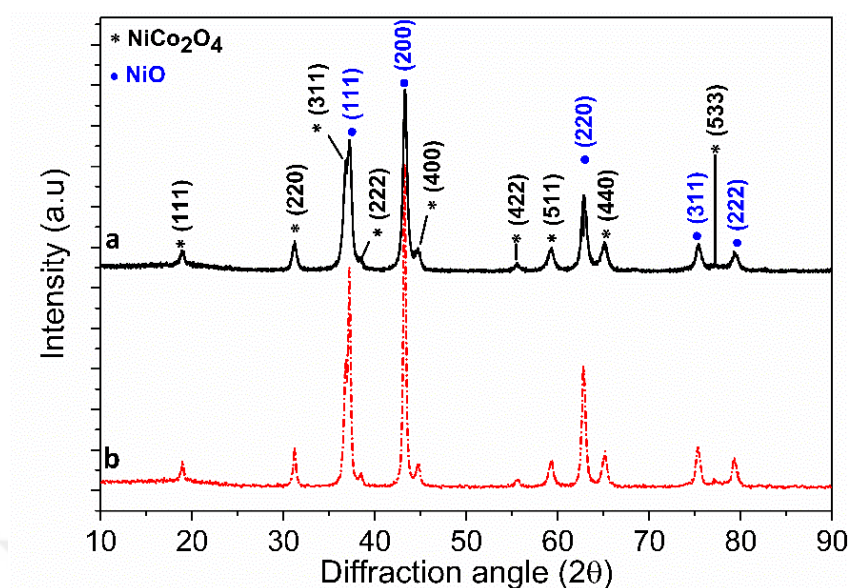
Figure 5.25. XRD patterns of (a) U-NiCo and (b) C-NiCo microspheres
