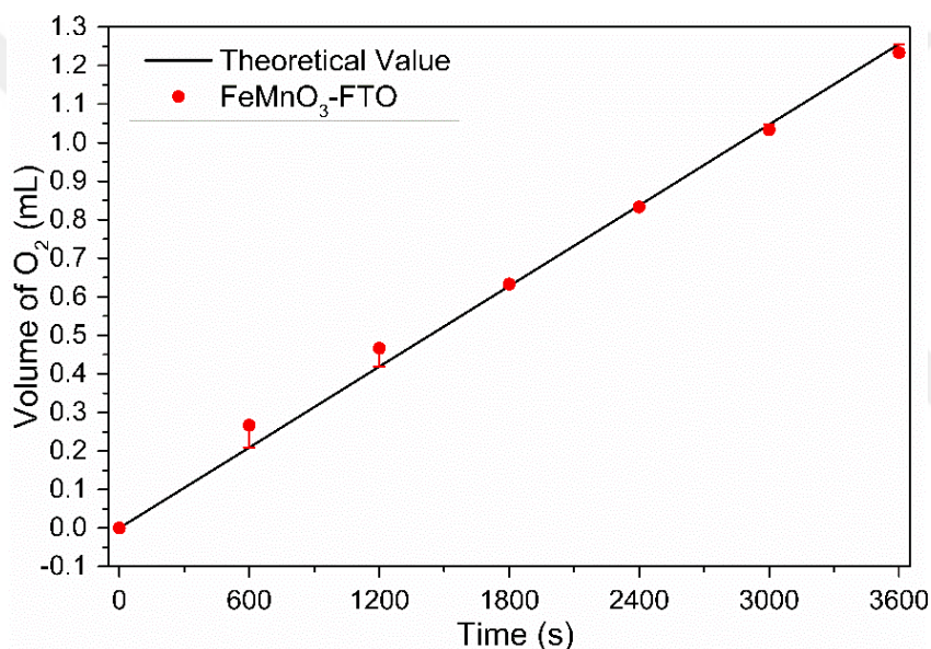
Figure 5.37. Plot of \text{O}_2 volume vs time during the electrolysis of water using \text{FeMnO}_3 -FTO electrode
