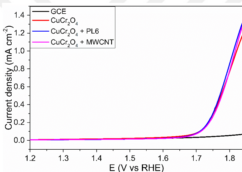
Figure B.4. Polarization curves of \text{CuCr}_2\text{O}_4 nanoparticles and \text{CuCr}_2\text{O}_4 nanoparticles mixed with PL6 and MWCNT in 0.1 M KOH at a scan rate of 5 \text{ mV s}^{-1}
