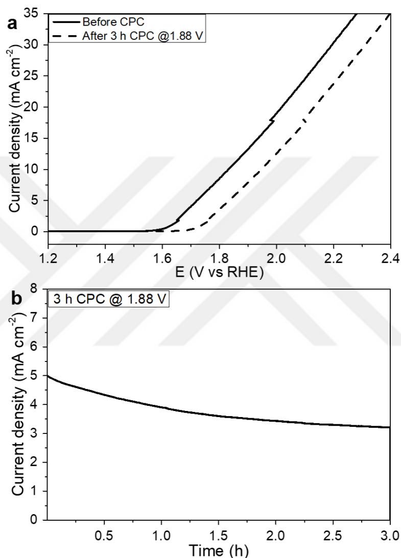
Figure 5.36. (a) Polarization curve of FeMnO 3 -FTO electrode before and after controlled potential electrolysis at overpotential corresponding to initial current density of 5 \text{ mA cm}^{-2} and (b) Change in current density during electrolysis in 0.1 M KOH
