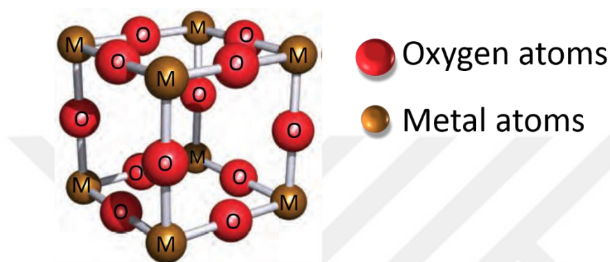
Figure 2.6. Unit cell of ReO 3 structure (red circles: oxygen atoms, gold circles: transition metal atoms) (modified from 34 )
