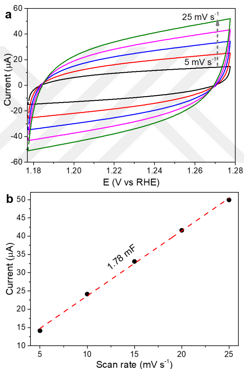
Figure 5.34. (a) CVs of \text{FeMnO}_3 nanowires measured at different scan rates from 5 to 25 \text{ mV s}^{-1} and (b) Plot of current at 1.27 V (vs RHE) vs scan rate
