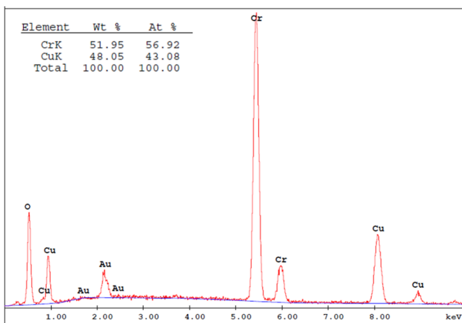
Figure 5.3. EDX spectrum of \text{CuCr}_2\text{O}_4 nanoparticles
