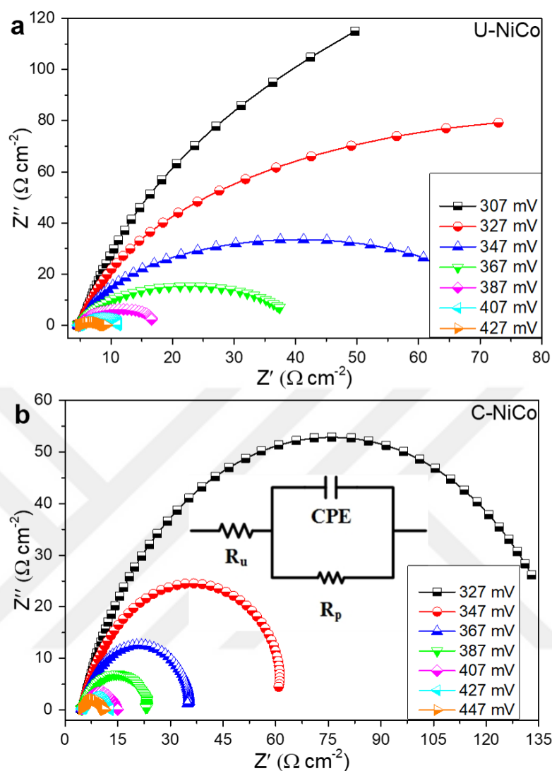
Figure 5.45. Nyquist plots of (a) U-NiCo and (b) C-NiCo microspheres at various overpotentials (inset shows the equivalent circuit diagram)
