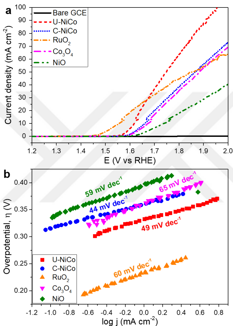
Figure 5.42. (a) Polarization curves of bare GCE, \text{NiCo}_2\text{O}_4 -NiO microspheres, \text{RuO}_2 , \text{Co}_3\text{O}_4 and NiO in 0.1 M KOH at a scan rate of 5 \text{ mV s}^{-1} and (b) The corresponding Tafel plots obtained from polarization curves
