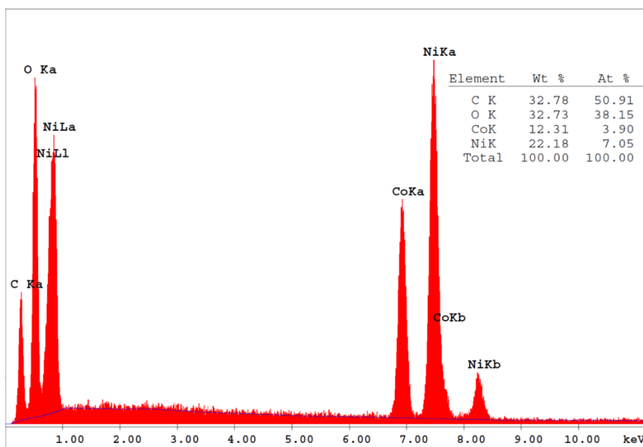
Figure 5.22. EDX spectrum of U-NiCo microspheres
