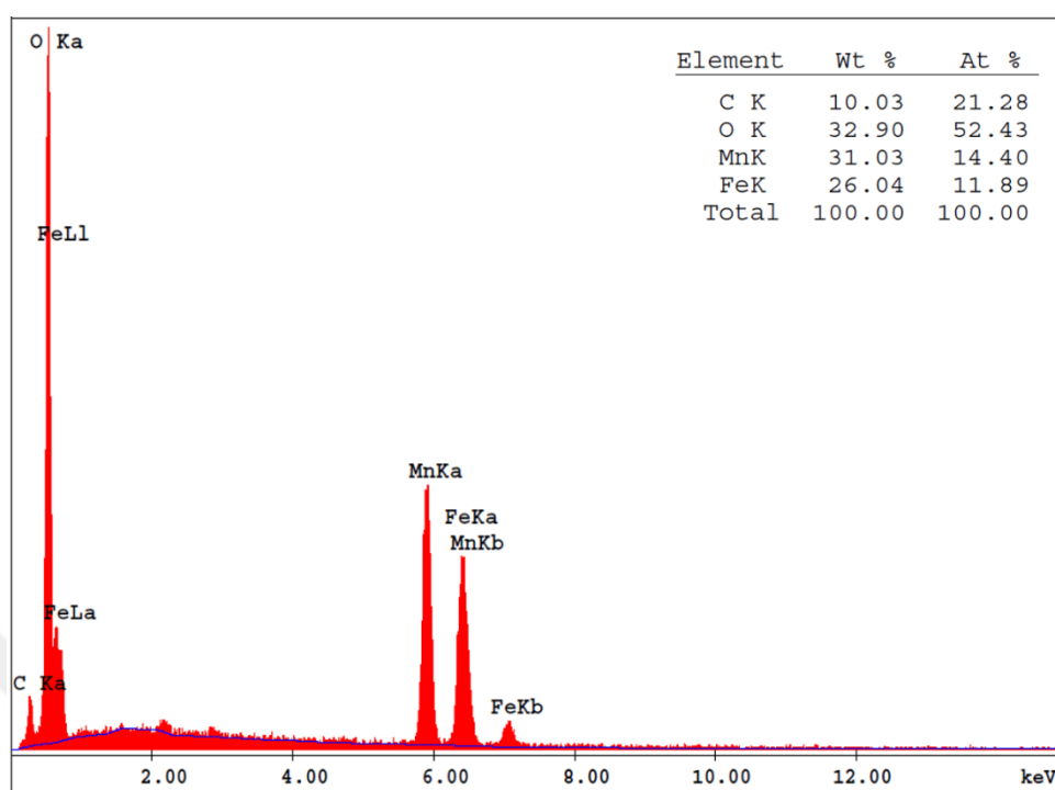
Figure 5.9. EDX spectrum of FeMnO 3 nanowires
