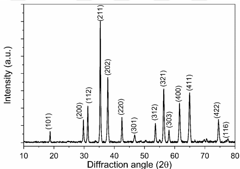
Figure 5.4. XRD pattern of \text{CuCr}_2\text{O}_4 nanoparticles (JCPDS 34-0424)
