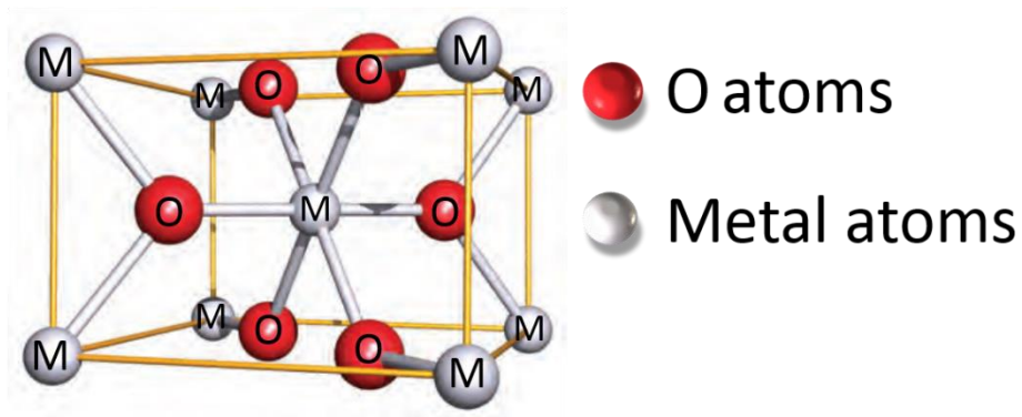
Figure 2.3. Unit cell of rutile structure (red circles: oxygen atoms, pale grey circles: transition metal atoms) (modified from 34 )
