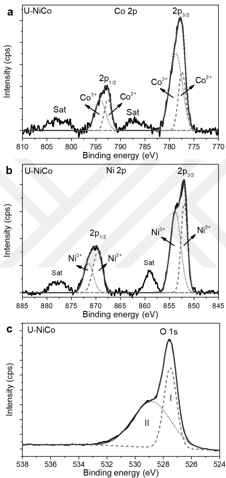
Figure 5.27. XPS (a) Co 2p, (b) Ni 2p and (c) O 1s spectra of U-NiCo microspheres
