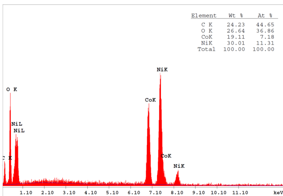
Figure 5.24. EDX spectrum of C-NiCo microspheres
