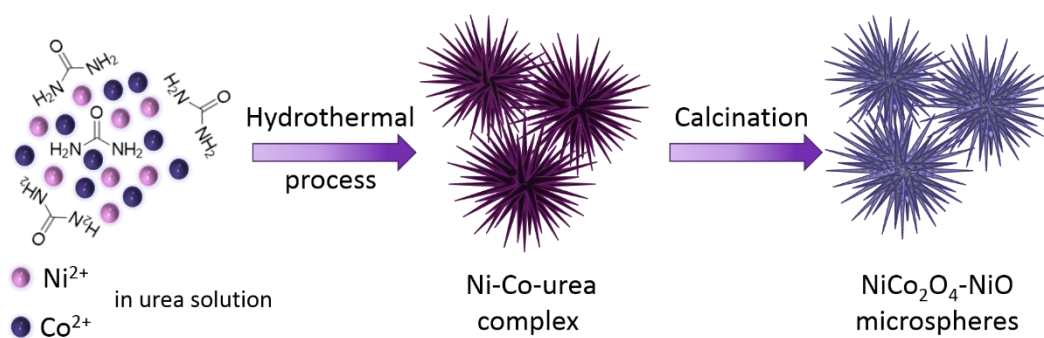
Figure 5.19. Illustration for the formation of urea stabilized \text{NiCo}_2\text{O}_4 -NiO microspheres
