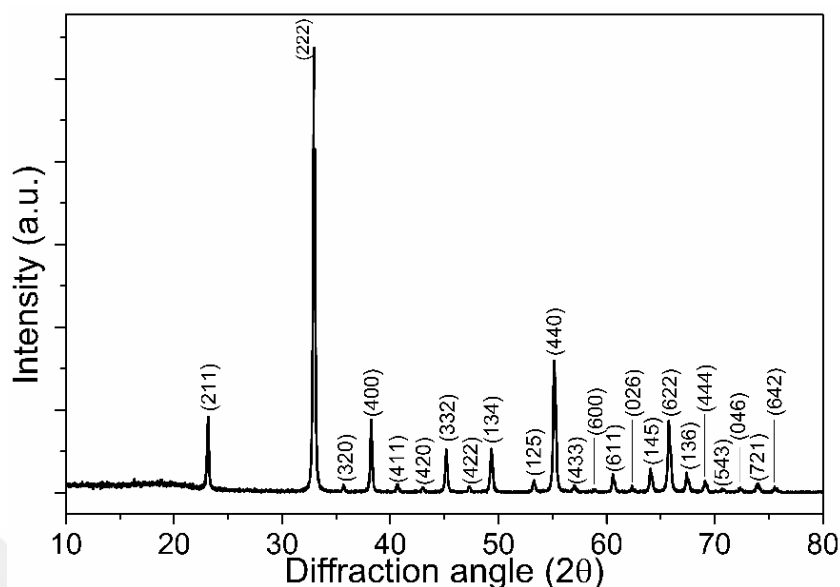
Figure 5.10. XRD pattern of FeMnO 3 nanowires (PDF number 01-076-0076)
