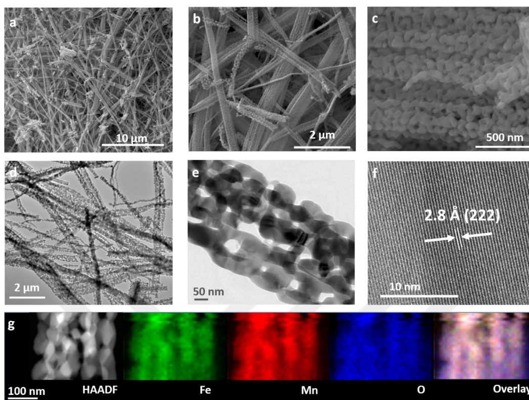
Figure 5.8. (a-c) SEM images and (d-f) TEM images at different magnifications, (g) HAADF-STEM image and element mapping (Fe (green), Mn (red) and O (blue)) of FeMnO 3 nanowires
