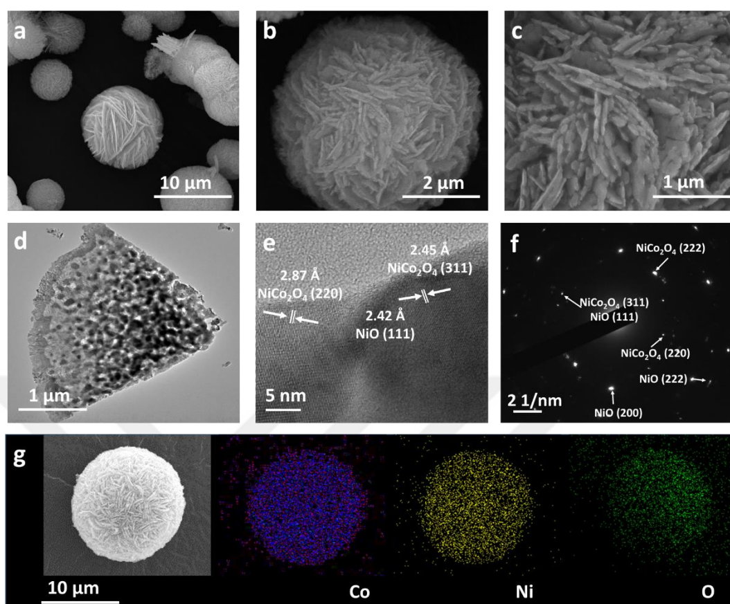
Figure 5.23. (a-c) SEM and (d-e) TEM images at different magnifications, (f) SAED pattern and (g) Element mapping (Co (blue), Ni (yellow), O (green)) of C-NiCo microspheres
