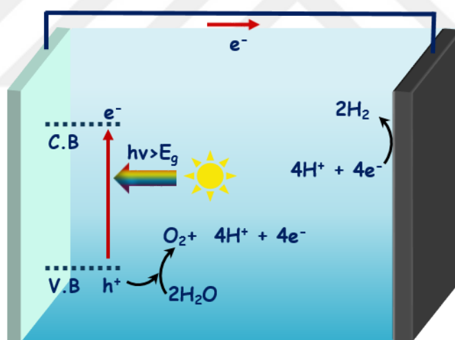
Figure 3.1. Schematic representation of photoelectrochemical water oxidation
