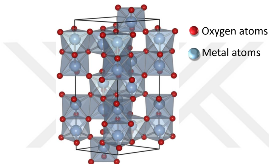
Figure 2.5. Corundum structure of TMOs ( M_2O_3 ) (red circles: oxygen atoms, blue circle: transition metal atoms occupying the octahedral cavity formed by O^{2-} ions) (modified from 32 )
