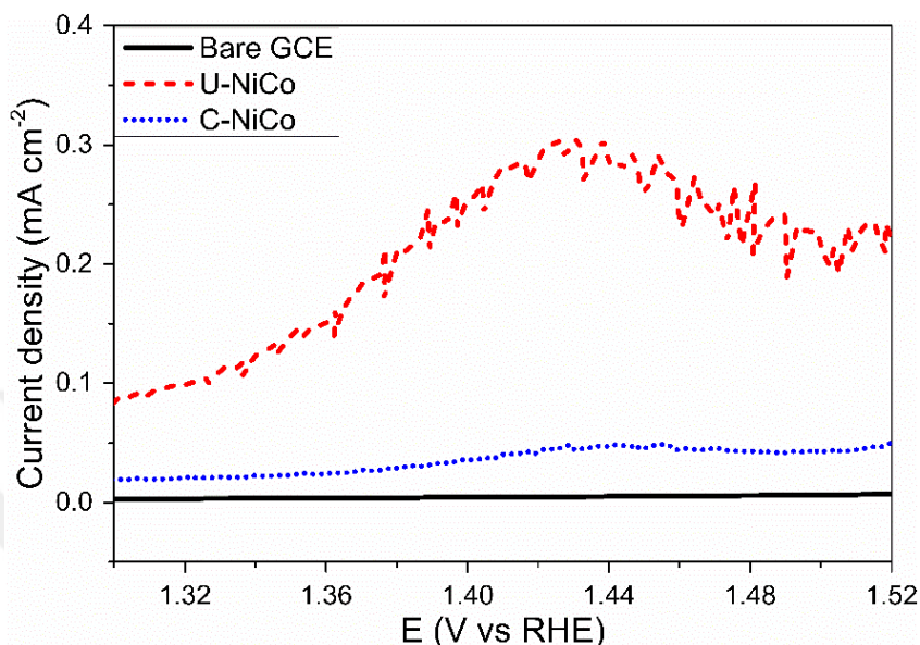
Figure 5.43. Polarization curves (in 1.30-1.52 V range) of bare GCE, U- and C-NiCo microspheres in 0.1 M KOH at a scan rate of 5 mV s -1
