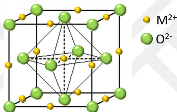
Figure 2.1. Unit cell of rock salt structure (green circles: oxygen atoms, yellow circles: transition metal atoms)
