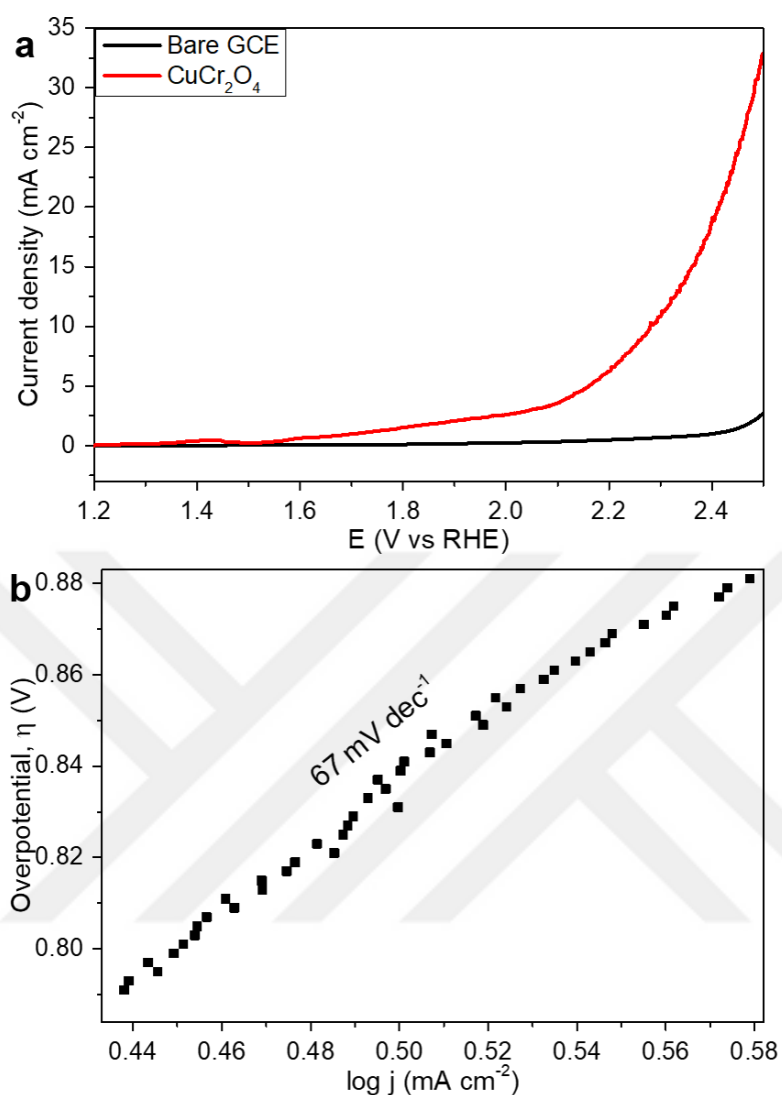
Figure 5.29. (a) Polarization curves of bare GCE and CuCr 2 O 4 nanoparticles in 0.1 M KOH at a scan rate of 5 mV s -1 and (b) The corresponding Tafel plot obtained from polarization curve
