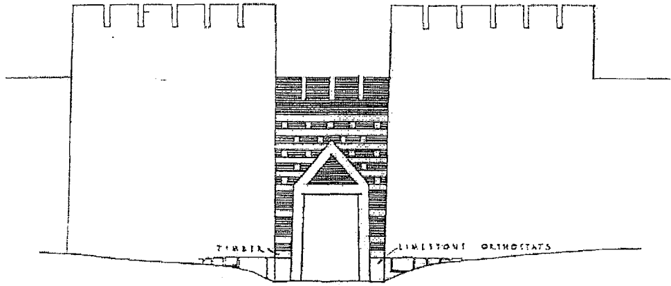
SUGGESTED NORTH ELEVATION, SHEDDING NAIL-TIMBERING
