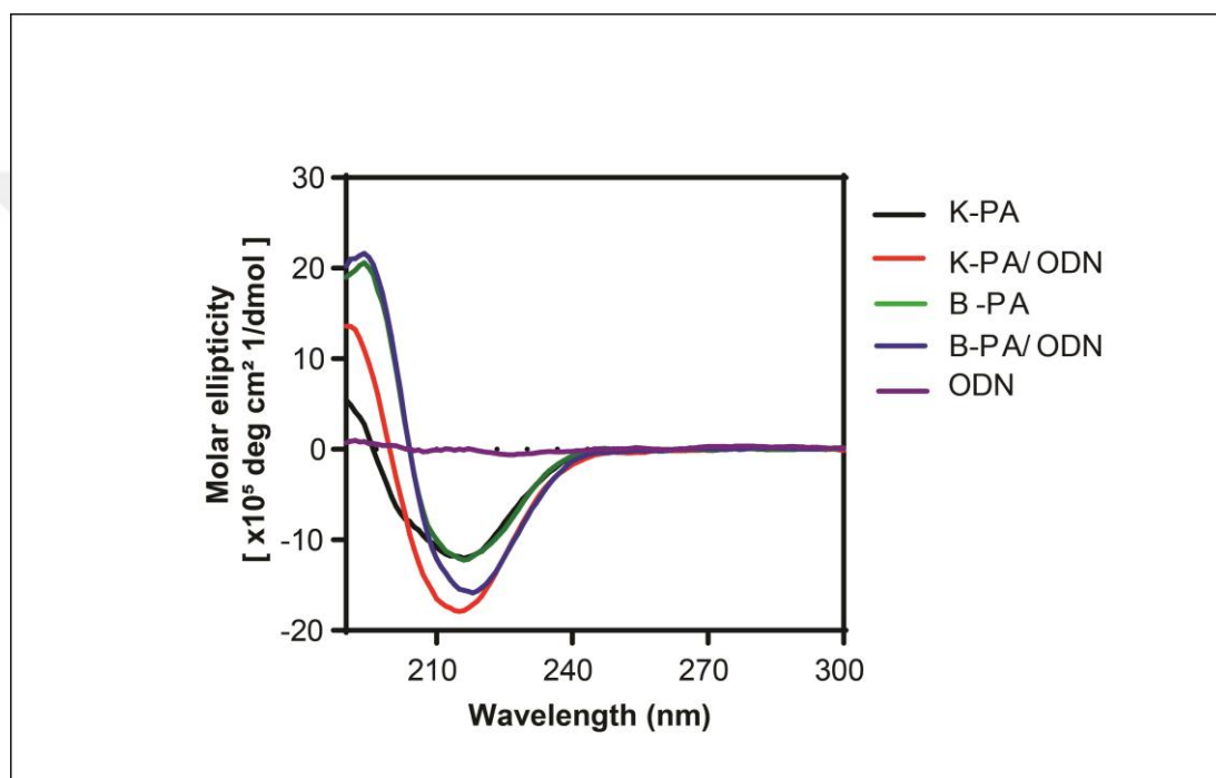
Figure 2.4 Structural characterization of PA/ODN nanostructures. CD spectra of ODN, PAs and PA/ODN complexes.
