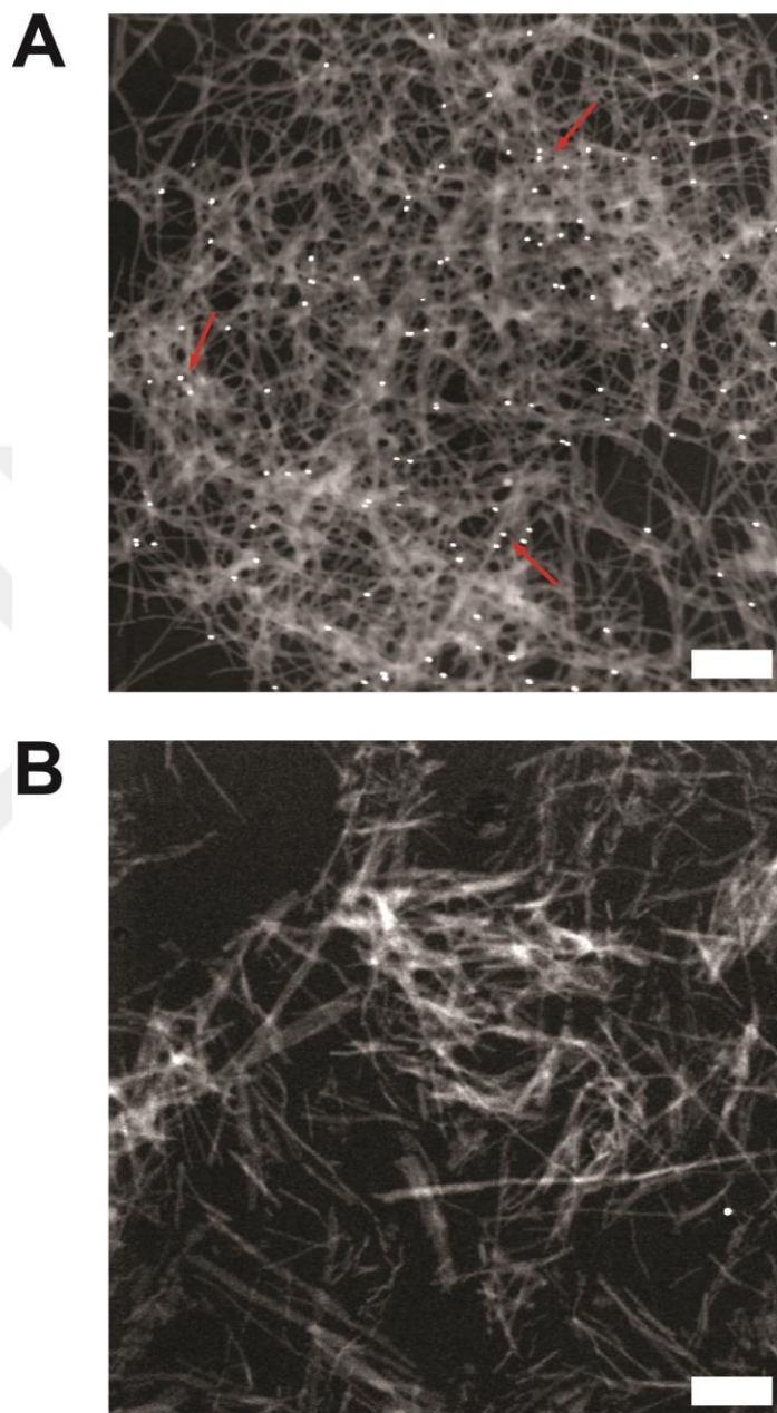
Figure 2.8 Antigen-bearing B-PA/ODN nanostructures. (A) STEM image of anti IgG-gold labeled B-PA/ODN + OVA nanostructures. Scale bar is 500 nm. (B) STEM image of anti IgG-gold labeled B-PA/ODN + OVA nanostructures without anti-Ovalbumin addition. Scale bar is 500 nm. (Shiny dots show gold nanoparticles)
