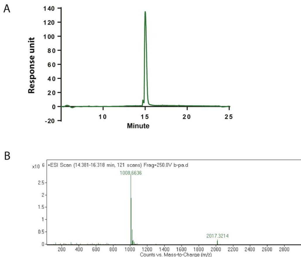
Figure 2.3 Characterization of B-PA. (A) LC chromatogram of B-PA molecule at 220 nm. (B) Mass spectrometry analysis of B-PA. [M+H]^+ (calculated) = 1008.38, [M+H]^+ (observed) = 1008.66
