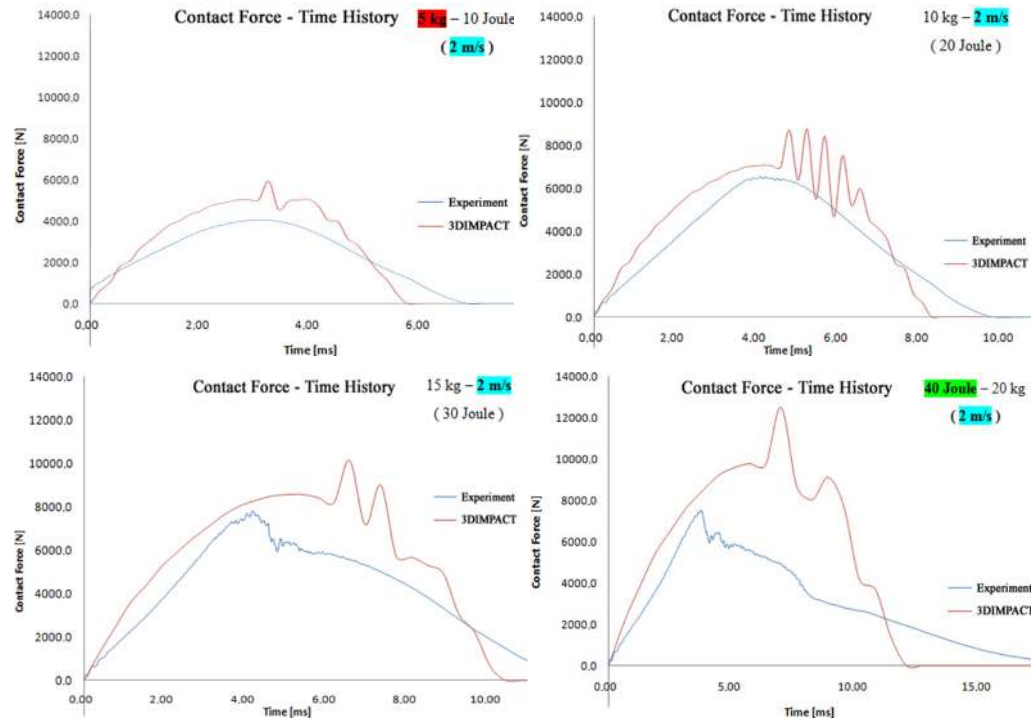
Figure 5.24 The contact force-time overlaid histories for equal impact velocity for [0^\circ/30^\circ/60^\circ/90^\circ] s.
