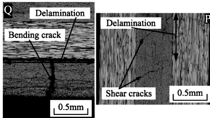
Figure 3.10 Cross-sectional micrographs, showing bending and shear cracks. (Takeda, Minakuchi & Okabe, 2004)
