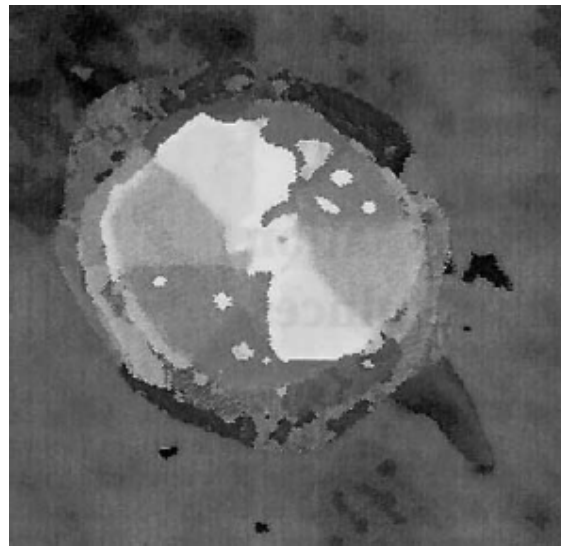
Figure 3.12 Ultrasonic C-Scan of a [45^\circ_2, 0^\circ_2, -45^\circ_2, 90^\circ_2]_s , 7.1 J impacted laminate. (Guinarda, Allixb, Gue'dra-Degeorgesa & Vineta, 2000)
