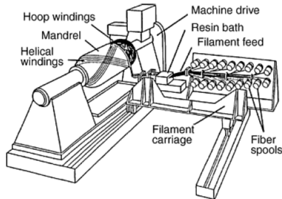
Figure 2.9 Filament winding machine. (Miracle & Donaldson, 2001)
