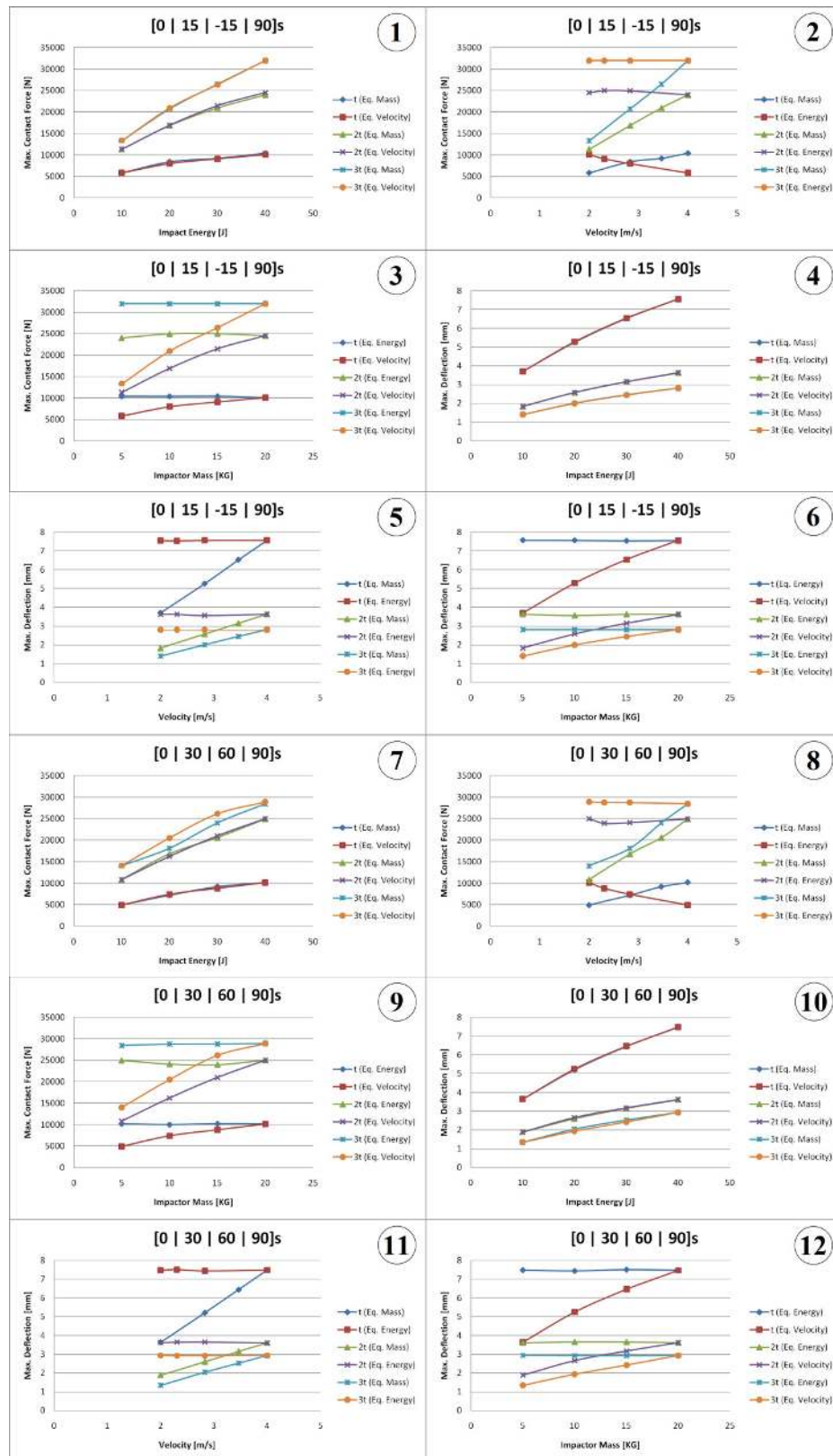
Figure 5.26 Multiple diagrams for thickness effect on max. contact force &amp; deflection.
