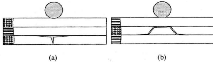
Figure 3.9 Tensile or bending crack (a), and the shear crack (b). (Abrate, 1999)
