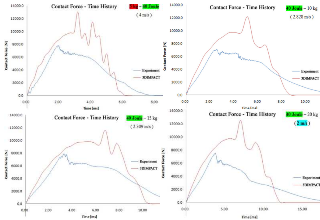
Figure 5.23 The contact force-time overlaid histories for equal impact energy for [0^\circ/30^\circ/60^\circ/90^\circ] s.
