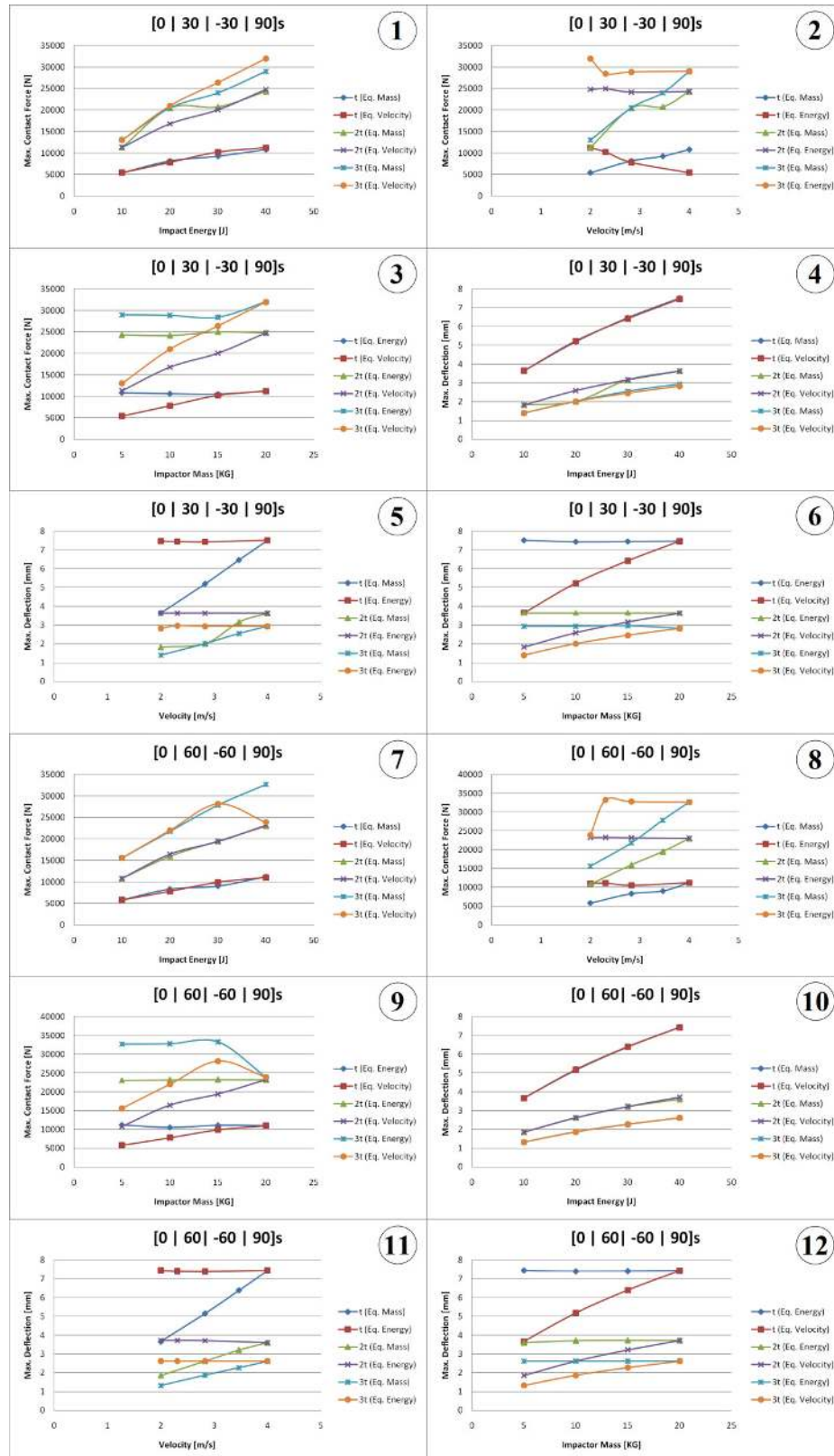
Figure 5.27 Multiple diagrams for thickness effect on max. contact force &amp; deflection.
