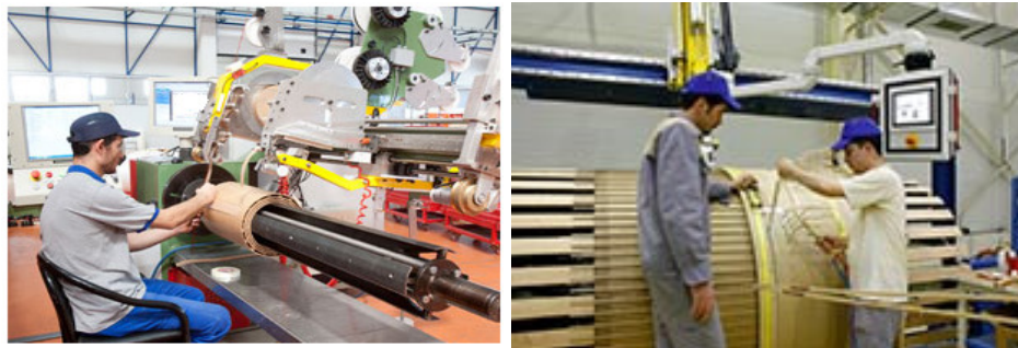
Figure 4.7 Winding production.
