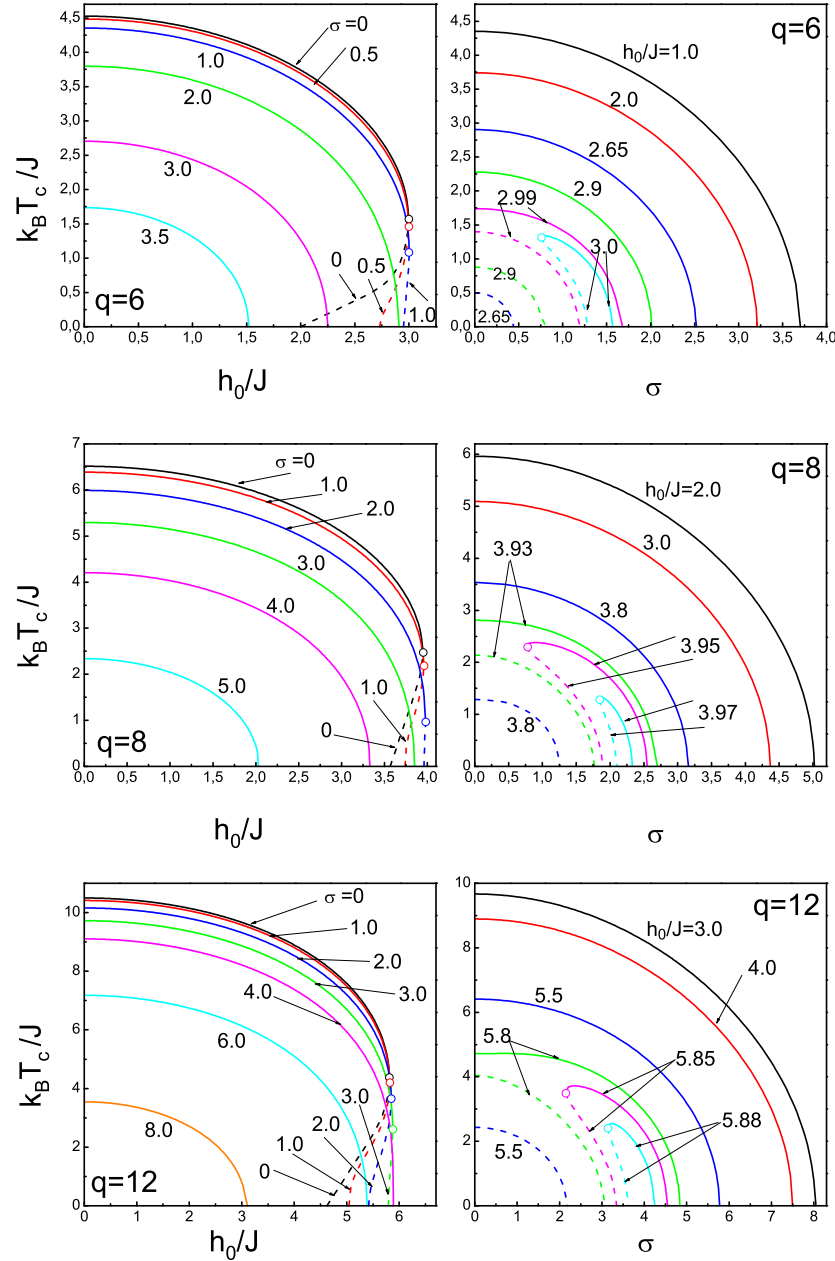
Figure 5.14 Phase diagrams of the system for a double-Gaussian random-field distribution with q = 6, 8 , and 12 in (k_B T_c/J - h_0/J) and (k_B T_c/J - \sigma) planes.
