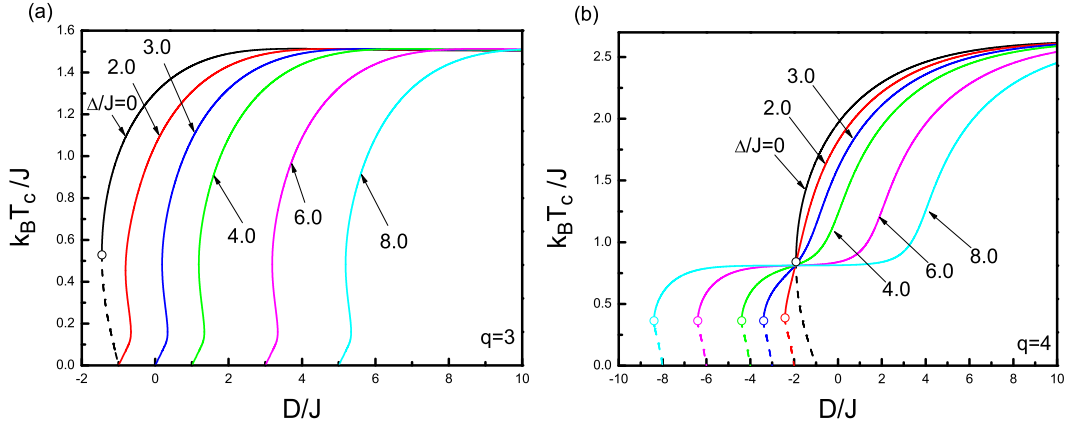
Figure 5.7 Phase diagrams of the system in a (k_B T_c / J - D/J) plane corresponding to random crystal field distribution defined in Eq. (5.3.6) for (a) q = 3 , (b) q = 4 . The numbers on each curve denote the value of \Delta/J . The open circles represent the tricritical points, and the solid and dashed lines correspond to second- and first-order phase transitions, respectively.
