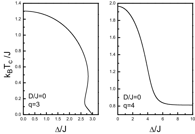
Figure 5.6 Phase diagrams of the system in a (k_B T_c / J - \Delta/J) plane for a bimodal crystal field distribution corresponding to Eq. (5.3.6) with D/J = 0.0 . Left and right-hand side panels are plotted for q = 3 and q = 4 , respectively.
