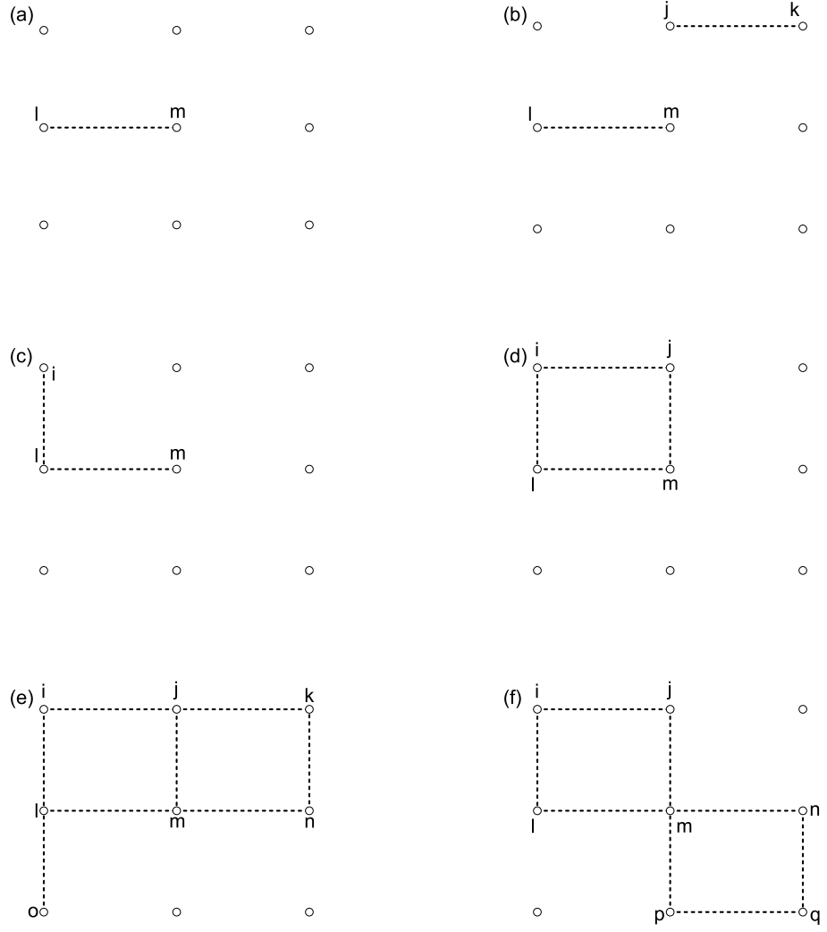
Figure 3.1 Graphs on the square lattice, each of which corresponds to a product of spins in the sum in Eq. (3.2.3): (a) s_l s_m , (b) s_l s_m s_j s_k , (c) s_i s_l^2 s_m , (d) s_i^2 s_j^2 s_l^2 s_m^2 , (e) s_i^2 s_j^3 s_k^2 s_l^3 s_m^3 s_n^2 s_o , (f) s_i^2 s_j^2 s_l^2 s_m^4 s_n^2 s_p^2 s_q^2 . Only (d) and (f), where the number of bonds at each vertex is even, give a nonzero contribution to the partition function, (Yeomans, 2000).
