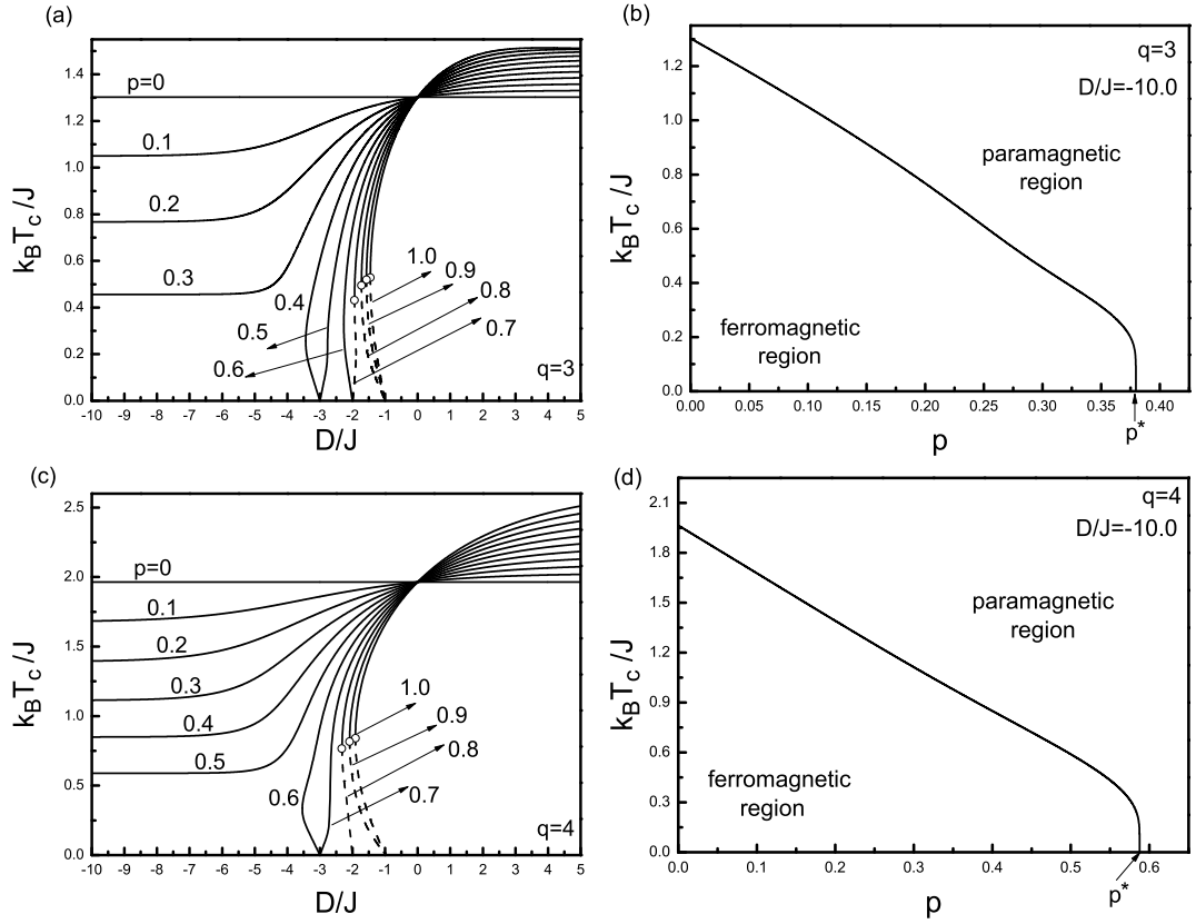
Figure 5.3 (a) Phase diagrams of the system for q = 3 in a (k_B T_c/J - D/J) plane corresponding to dilute crystal field distribution defined in Eq. (5.3.5). The solid and dashed lines correspond to second- and first-order phase transitions, respectively. The open circles denote the tricritical points, and the numbers on each curve represent the value of concentration p . (b) Phase diagrams of the system for q = 3 in a (k_B T_c/J - p) plane with a selected value of the crystal field D/J = -10.0 . (c) Phase diagrams of the system for q = 4 in a (k_B T_c/J - D/J) plane corresponding to dilute crystal field distribution defined in Eq. (5.3.5). The solid and dashed lines correspond to second- and first-order phase transition, respectively. The open circles refer to the tricritical points, and the numbers on each curve represent the value of concentration p . (d) Phase diagrams of the system for q = 4 in a (k_B T_c/J - p) plane with a selected value of the crystal field D/J = -10.0 .
