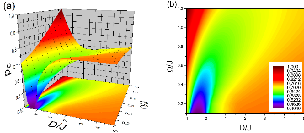
Figure 5.2 Variation of the bond percolation threshold p_c with crystal field D/J and transverse field \Omega/J . (a) 3D contour plot surface, (b) projection on (\Omega/J-D/J) plane.
