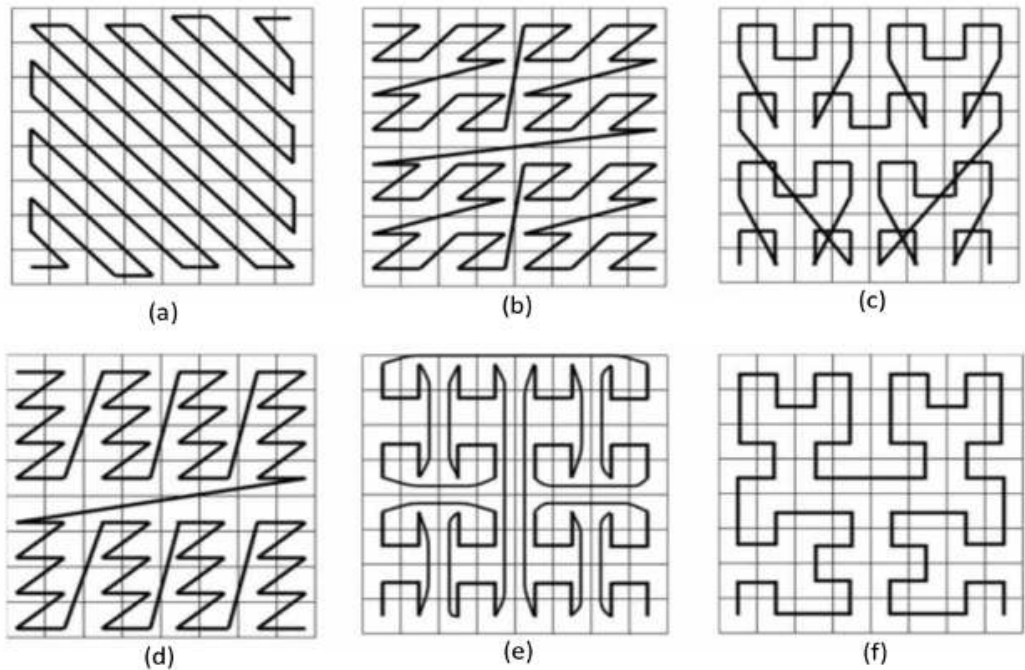
Figure 3.6. Six different space-filling curves that can be used in the transformation phase.
