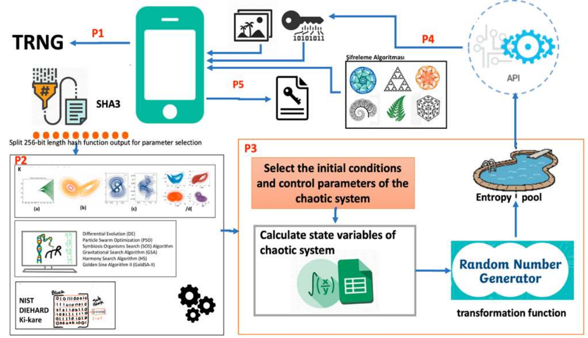
Figure 3.1. The general view of the proposed architecture.
