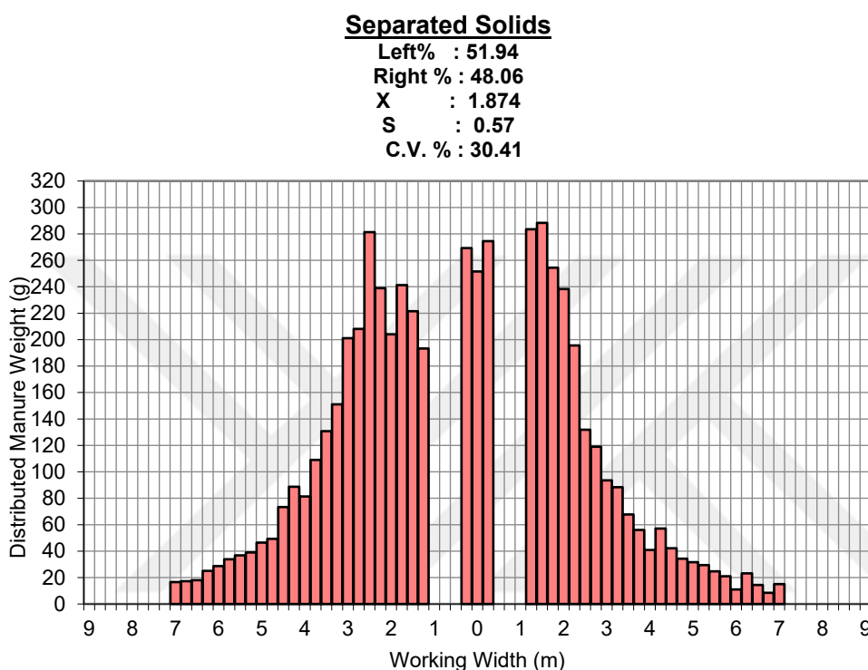
Figure 4.2. Transverse distribution, optimum working width, standard deviation after folding technique and coefficient of variation.
