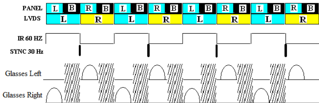
Figure 5.1 Sync Signal
