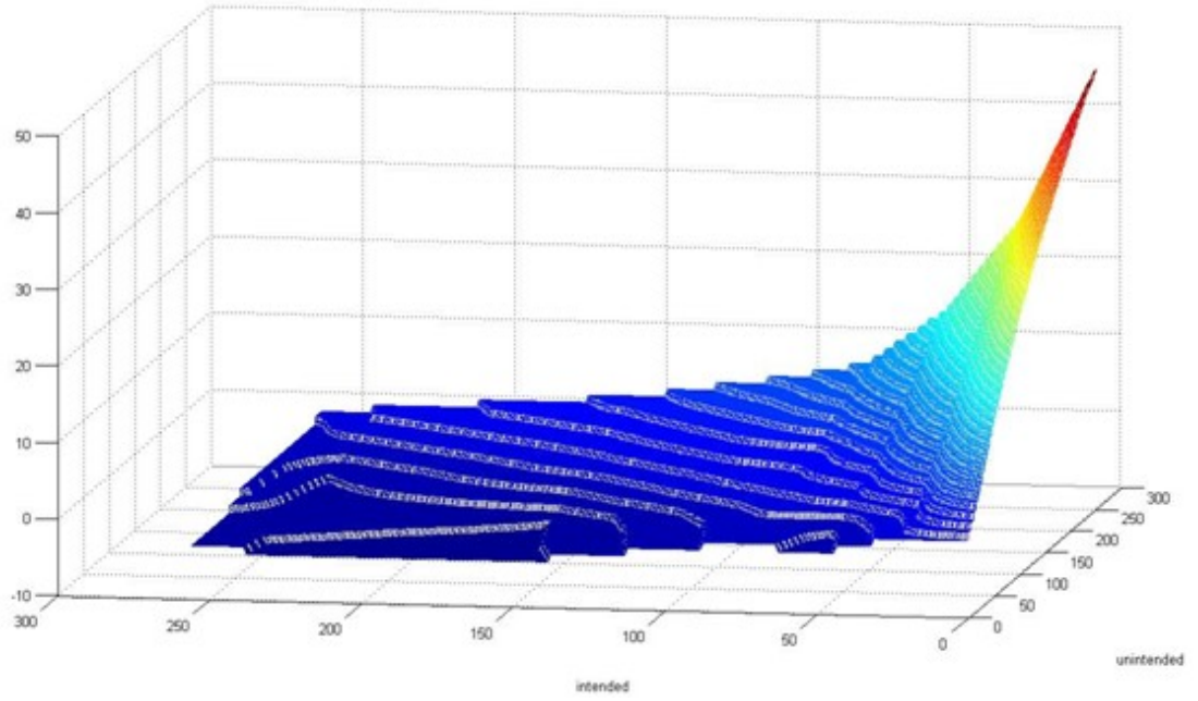
Figure 5.7 Graphical illustration of table 4.2: Crosstalk Characteristics
