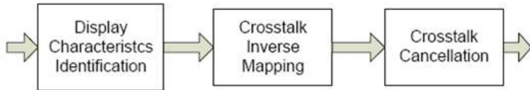
Figure 5.3 Algorithm Overview
