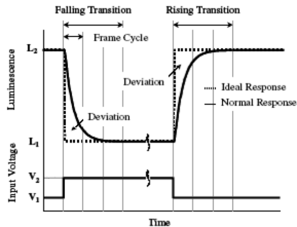
Figure 2.5 LCD Response time waveform
