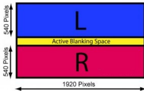
Figure 2.16 Structure of a 1080p top-bottom 3D
