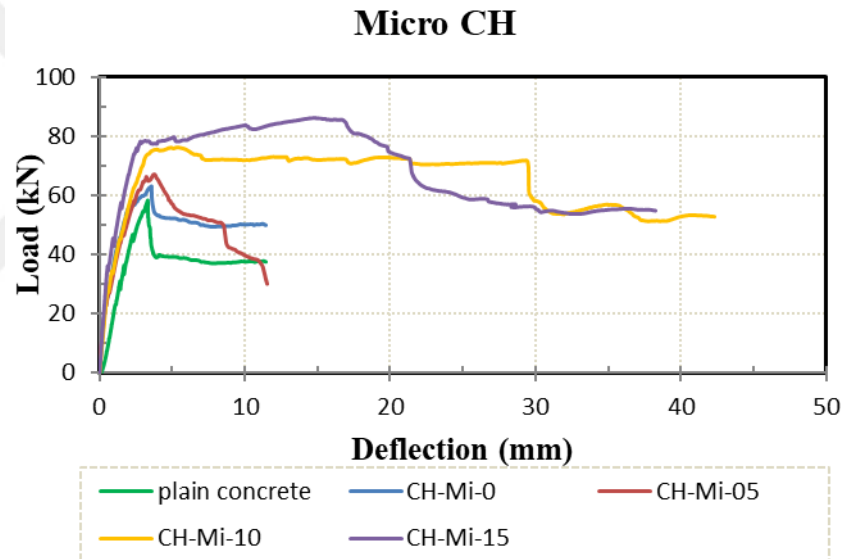
Figure 5.10 Load – Deflection curve
