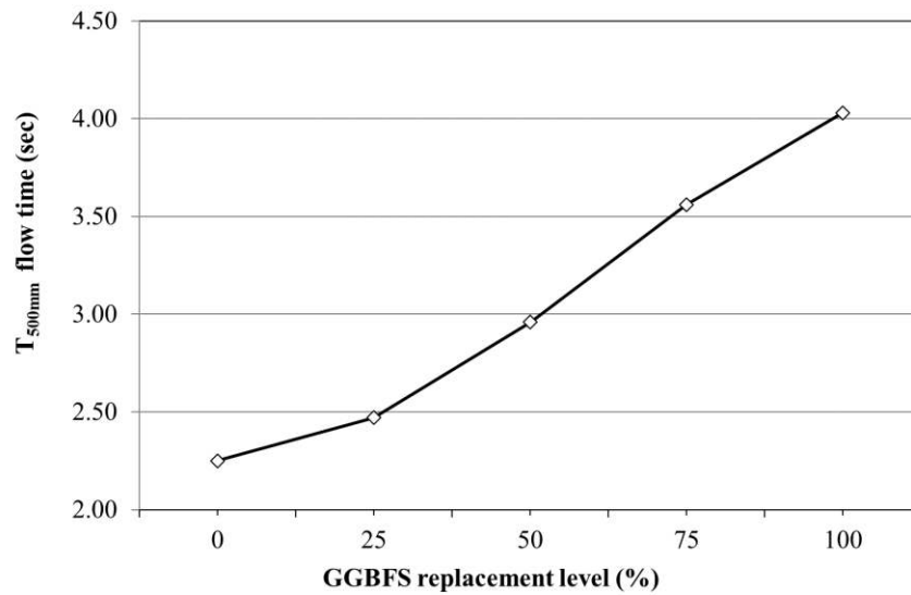
Figure 4.2 Effect of GGBFS level on T_{500\text{mm}} flow time values
