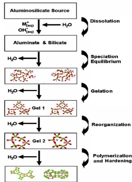
Figure 2.5 Conceptual model for geopolymerization [36].
