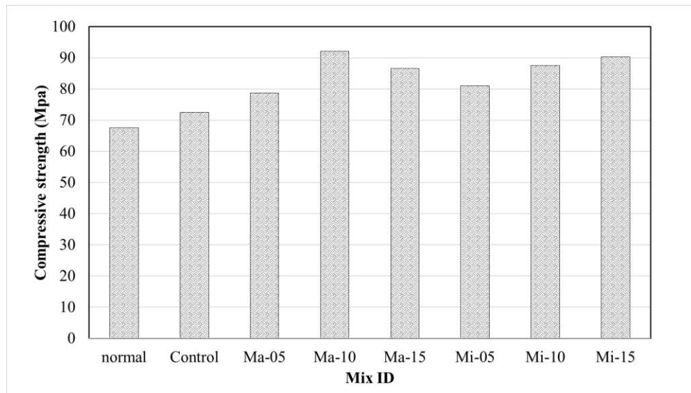
Figure 5.1 Compressive strength
