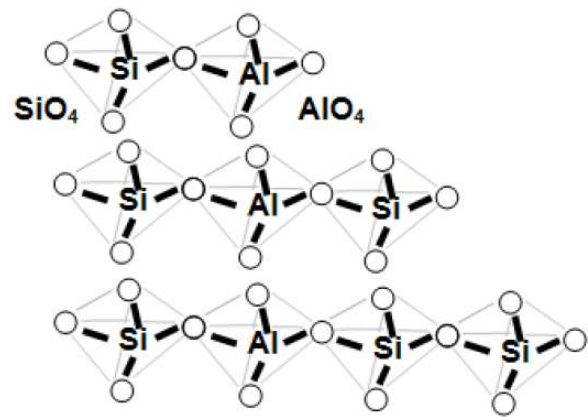
Figure 2.3 Common types of polysialates
